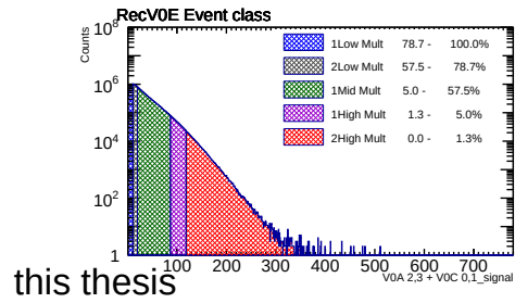
(h) Rec.MC, V0E event estimator.
