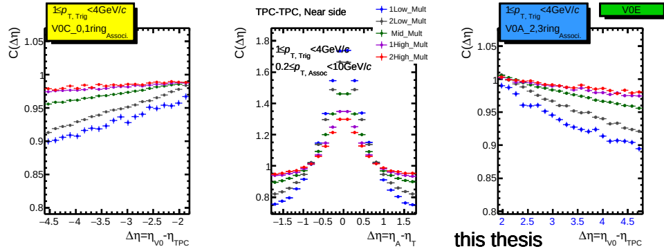
(d) ALICE experimental data, V0E event estimator, near side.
