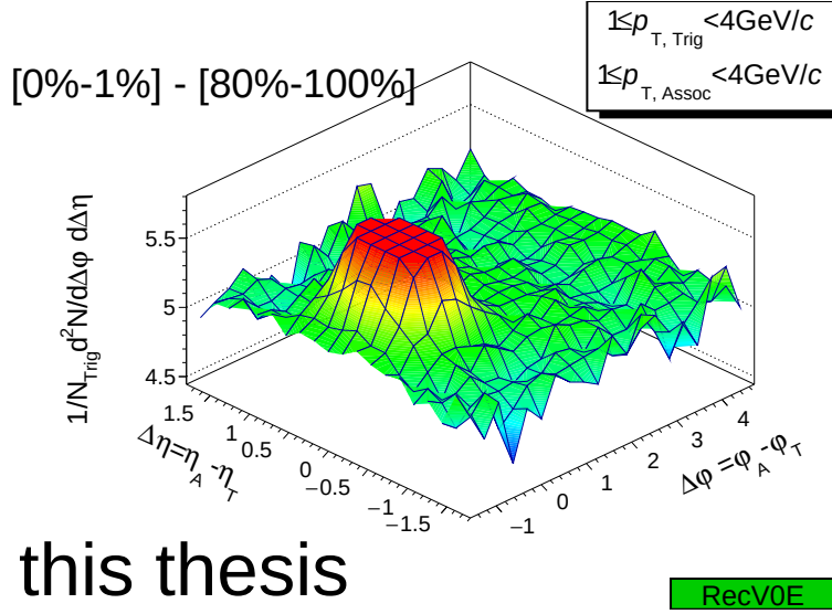
(b) Rec.MC, V0E event estimator.
