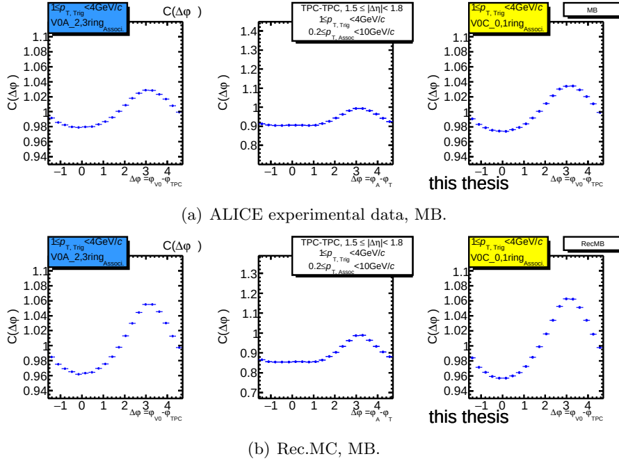
Figure 4.26: 1-D dihadron correlation functions of V0A-TPC, TPC-TPC and V0C-TPC in pp collisions at \sqrt{s} = 7 TeV in long range approximate 1.9 < \Delta\eta < 4.8 , 1.5 \leq |\Delta\eta| < 1.8 and -1.8 < \Delta\eta < -4.6 are shown for the minimum bias (MB).
