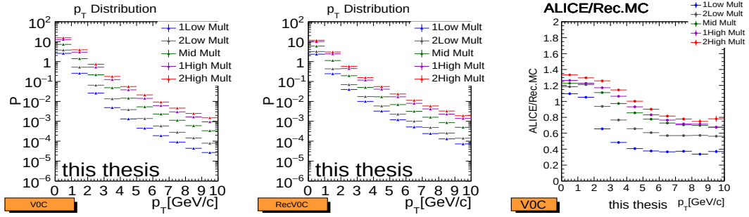
(d) ALICE experimental data, (e) Rec.MC, V0C event estimator, (f) V0C event estimator, Ratio of ALICE experimental data over Rec.MC.
