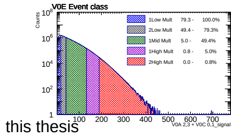
(g) ALICE experimental data, V0E event estimator.
