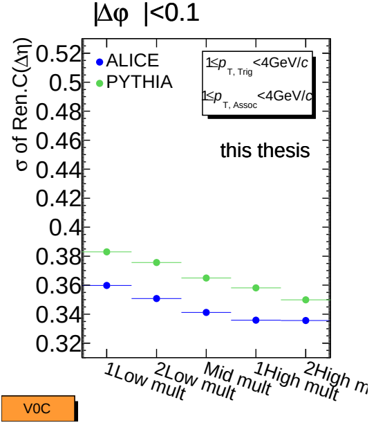
(b) ALICE experimental data, V0C event estimator.
