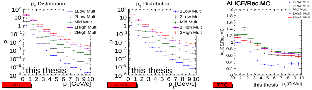
(g) ALICE experimental data, (h) Rec.MC, TPC event estimator, (i) TPC event estimator, Ratio of ALICE experimental data over Rec.MC.
