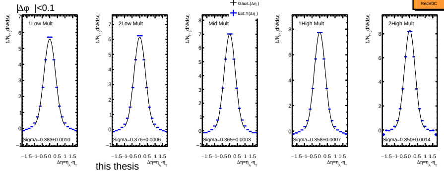
(b) Rec.MC data, V0C event estimator.
