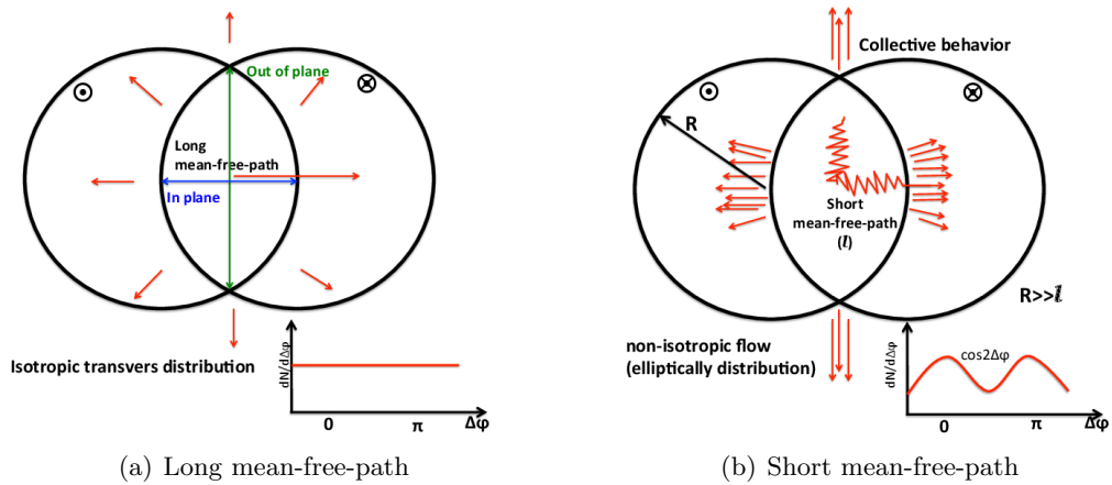
Figure 1.8: The difference between long- and short mean-free-path evolutions in transvers plane are shown.
