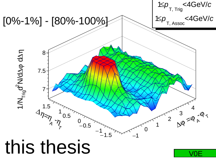
(a) ALICE experimental data, V0E event estimator.
