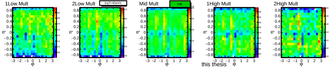
(d) ALICE experimental data, V0E event estimator, \varphi and \eta distributions for the 5 multiplicity classes.
