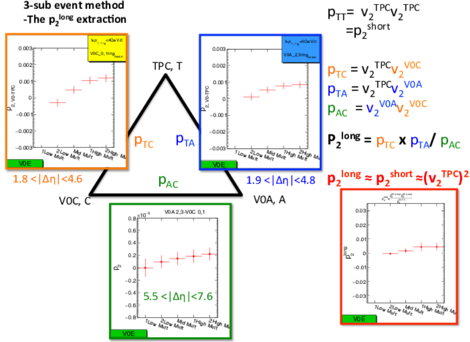
Figure 3.15: p_2^{\text{long}} extraction in long range \Delta\eta .
