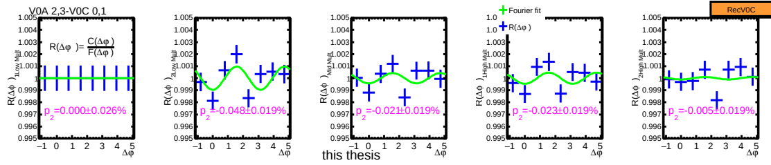
(b) Rec.MC, V0C event estimator.
