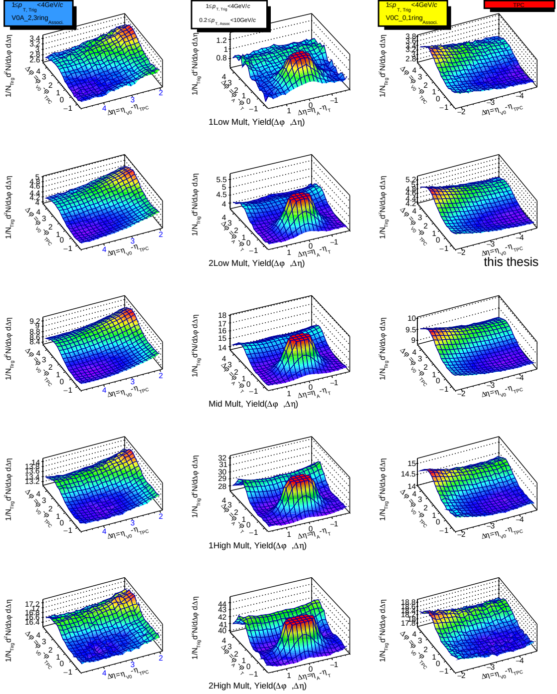
Figure F.3: ALICE experimental data, TPC event estimator, particle yield per trigger particle of V0A-TPC, TPC-TPC and V0C-TPC correlations are shown for the 5 multiplicity classes.
