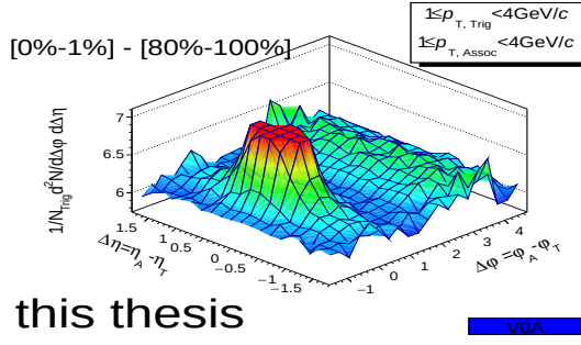
(a) ALICE experimental data, V0A event estimator.
