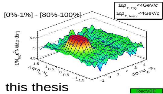
(h) Rec.MC, V0E event estimator.
