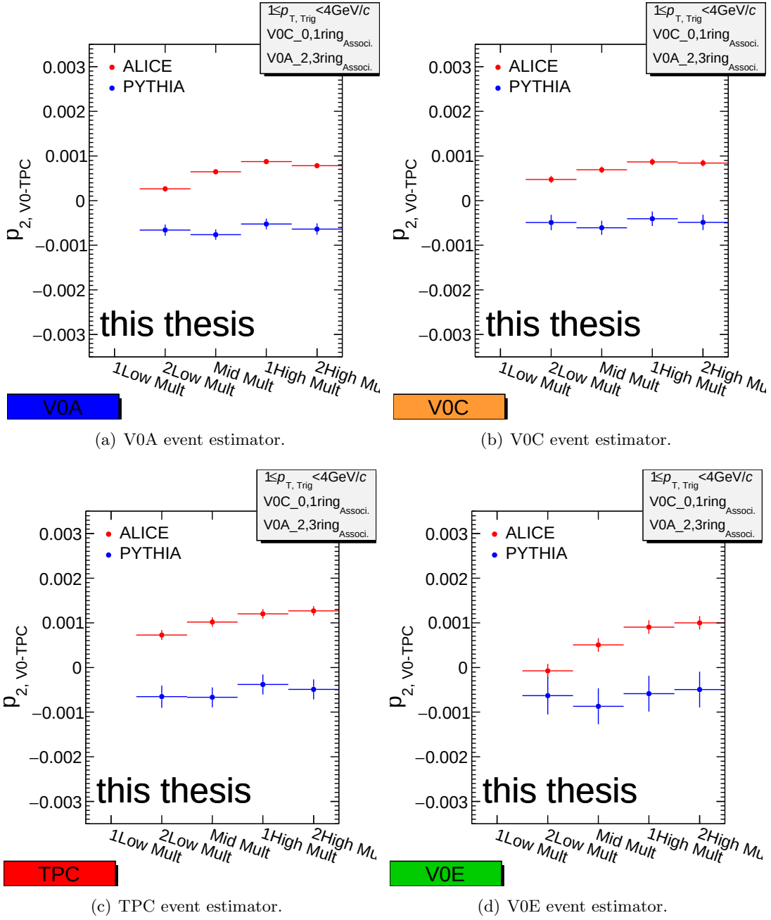
Figure 4.32: Product of two p_2 parameters (for trigger and associate particles) of TPC-V0 C(\Delta\varphi) correlation with respect to the lowest multiplicity are shown for the 5 multiplicity classes.
