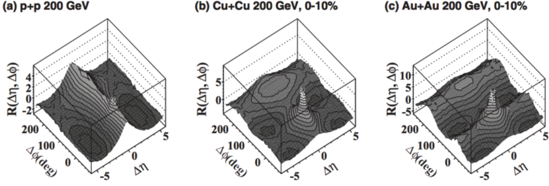
Figure 1.11: 2-D Two-particle angular correlation functions for (a) p + p , the central 10% (b) \text{Cu} + \text{Cu} and (c) \text{Au} + \text{Au} collisions at \sqrt{s} or \sqrt{s_{NN}} = 200 GeV [20].
