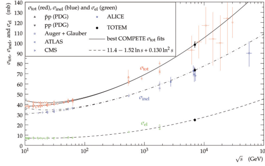
Figure 1.12: The increase with energy of the proton-proton total cross-section at \sqrt{s} = 7 TeV [4].
