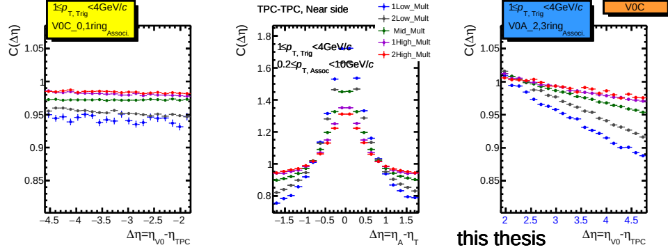
(b) ALICE experimental data, V0C event estimator, near side.
