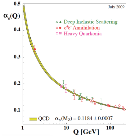
Figure 1.4: Summary of measurements of \alpha_s as a function of the respective momentum transfer Q [3].
