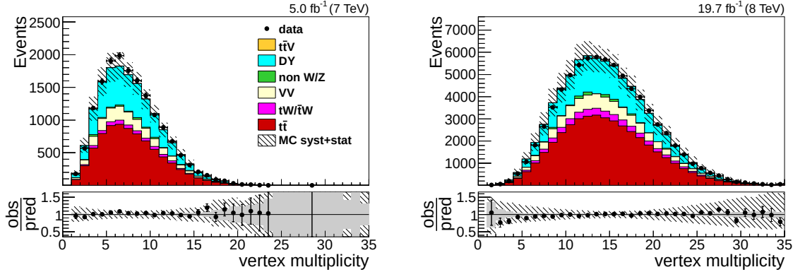
Figure 4.2: Reconstructed vertex multiplicity for \sqrt{s} = 7 \text{ TeV} (left) and \sqrt{s} = 8 \text{ TeV} (right). The hatched bands correspond to statistical and systematic uncertainties (discussed in Section 5.2) added in quadrature. The lower panels depict the ratio of observed and predicted yields. Here, the statistical uncertainty on the simulated yields is indicated by a gray shaded band. All events are required to fulfill the dilepton selection defined in Section 4.3.
