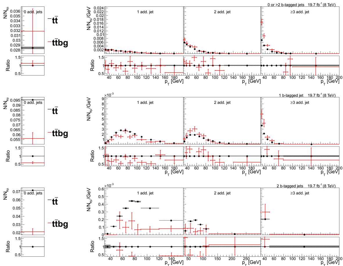
Figure 5.7: Comparison of the template shapes for the contribution from the t\bar{t} signal and t\bar{t} processes with non-dileptonic decay ( t\bar{t}b\bar{g} ). Left: total event yield for zero non-b-tagged jets (additional jets). Right: p_T of the least energetic additional jet in the event for events with one, two, and at least three additional jets. Shown are events with zero or more than two (top row), one (middle row), and two (bottom row) b-tagged jets at \sqrt{s} = 8 TeV. Each simulated contribution is normalized to the total number of selected dilepton events N_{e\mu} . The error bars and shaded bands indicate the statistical uncertainties on the simulated events yields. The lower panels depict the ratio of the t\bar{t}b\bar{g} contribution and the t\bar{t} signal contribution.
