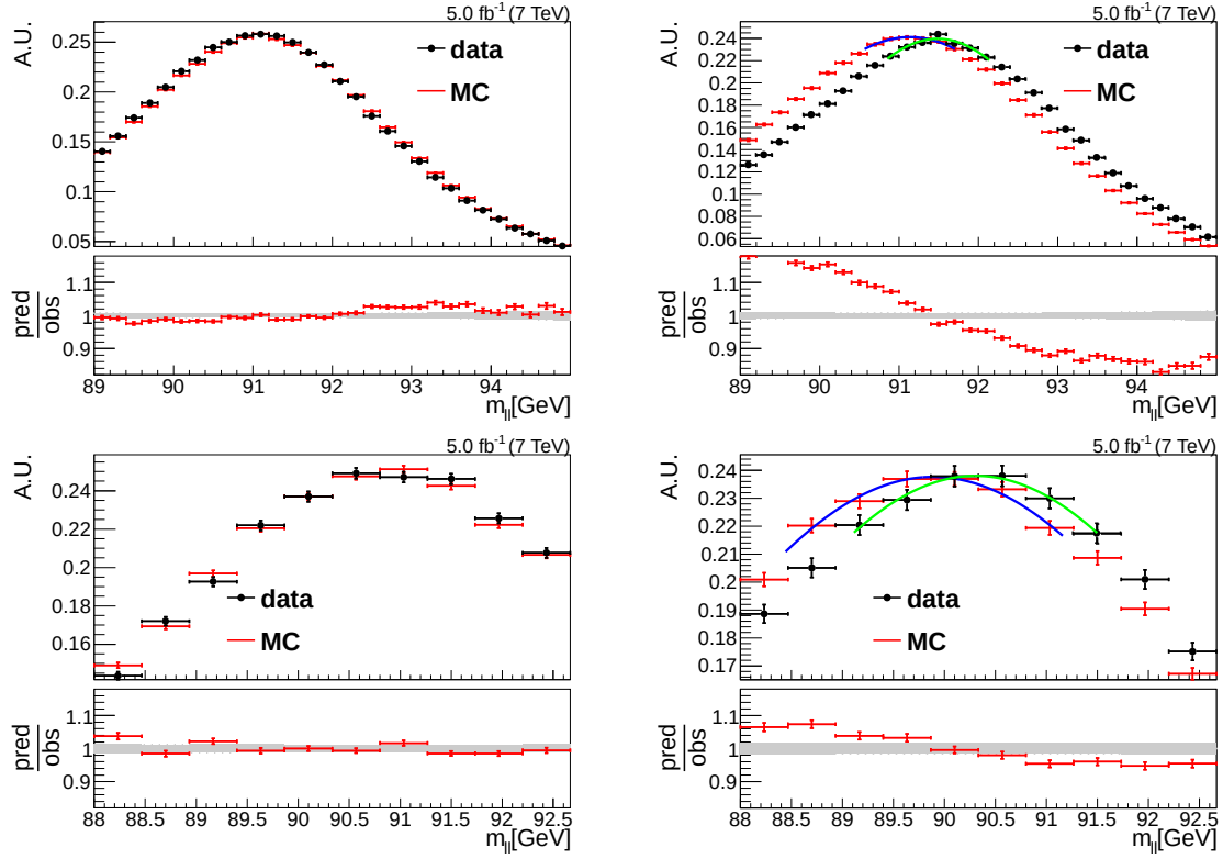
Figure 4.4: Invariant mass of muon (left) and electron (right) candidate pairs without additional lepton energy corrections at \sqrt{s} = 7\text{ TeV} normalized to 1. The upper row shows the barrel region ( |\eta| \leq 1.5 ), the lower row the endcap region ( 2.4 > |\eta| > 1.5 ). The green (blue) line corresponds to a Gaussian fitted to the data (simulation). The statistical uncertainties are indicated by error bars. The lower panel depicts the ratio of predicted and observed yields. Here, the statistical uncertainty on the data is indicated by a gray shaded band.
