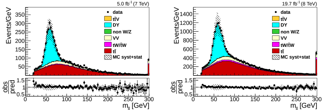
Figure 4.3: Invariant mass m_{ll} of the selected lepton candidate pair for \sqrt{s} = 7 TeV (left) and \sqrt{s} = 8 TeV (right). The hatched bands correspond to statistical and systematic uncertainties (discussed in Section 5.2) added in quadrature. The lower panels depict the ratio of observed and predicted yields. Here, the statistical uncertainty on the simulated yields is indicated by a gray shaded band.
