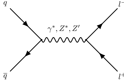
Figure 5.1: The Drell-Yan s -channel diagram that is used to calculate the scale factor per event where either the photon, Z boson or Z' boson is the propagator.
