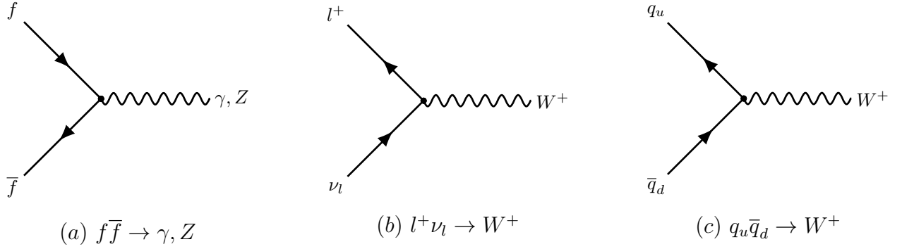
Figure 2.6: The interaction vertices involving fermions in EW theory.
