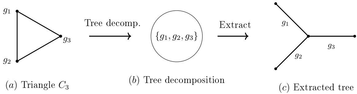
Figure 6.14: Tree decomposition (b) of the triangle C_3 (a) and the extracted graph of the tree decomposition (c).
