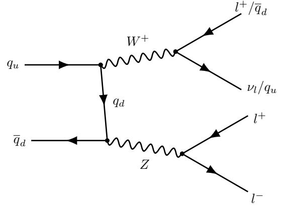
(b) Production of a Z boson and W^+ boson where the Z boson must decay leptonically.
