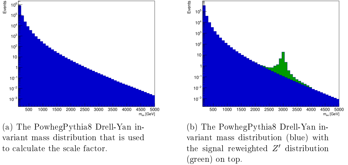
Figure 5.17: The PowhegPythia8 Drell-Yan invariant mass distribution (blue) (a) used for signal reweighting and the signal reweighted Z' (green) on top of the Drell-Yan distribution (blue) (b).
