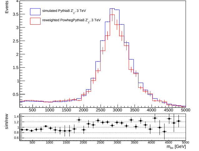
(b) Comparison between simulated (blue) and signal reweighted (red) Z'_\chi invariant mass distributions (lin)
