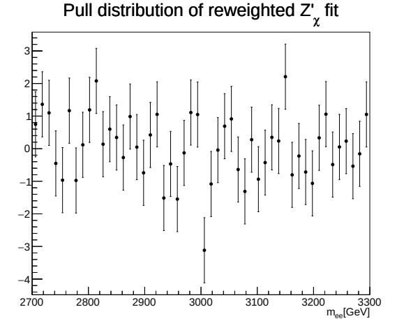
(b) Pull distribution of the reweighted Z'_\chi invariant mass fit.
