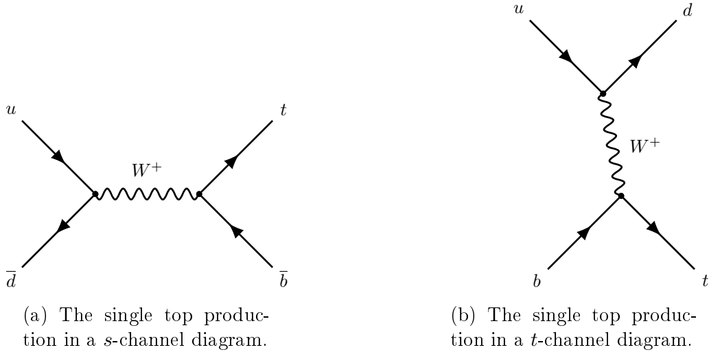
Figure 4.6: The single top production involving a s -channel (a) and t -channel (b).
