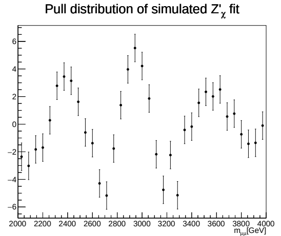
(b) Pull distribution of simulated Z'_\chi invariant mass fit.
