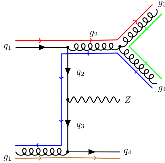
Figure 6.22: q_1 g_1 \rightarrow q_4 g_3 g_4 Z
