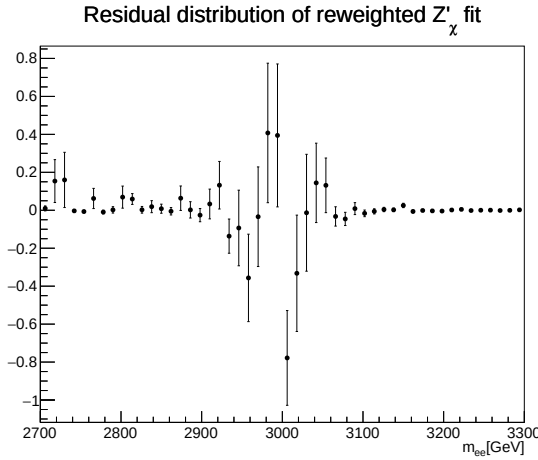
(a) Residual distribution of the reweighted Z'_\chi invariant mass fit.
