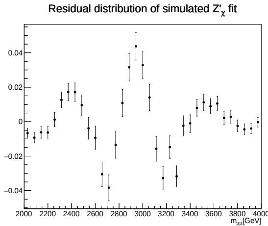
(a) Residual distribution of simulated Z'_\chi invariant mass fit.
