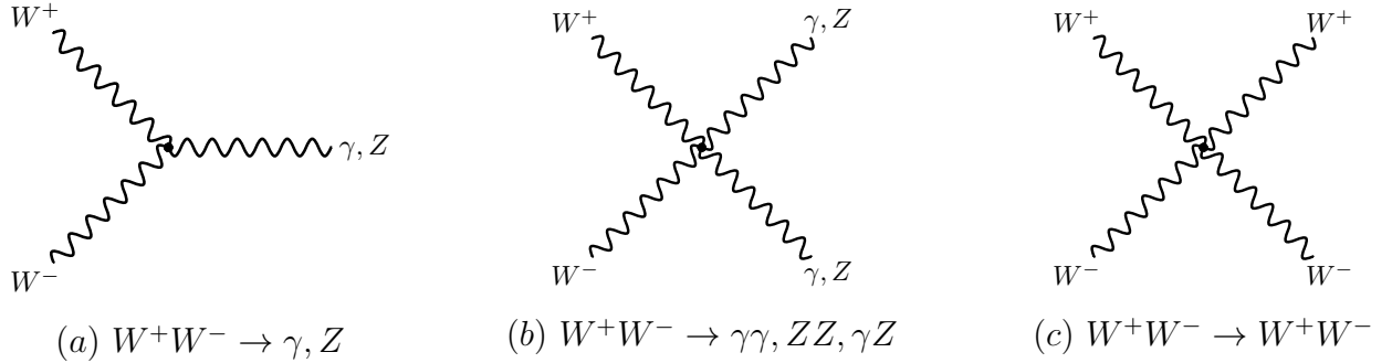
Figure 2.7: The self-interaction vertices in EW theory.
