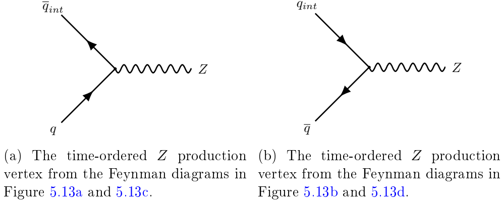
Figure 5.14: The time-ordered Z production vertices from the Feynman diagrams in Figure 5.13.
