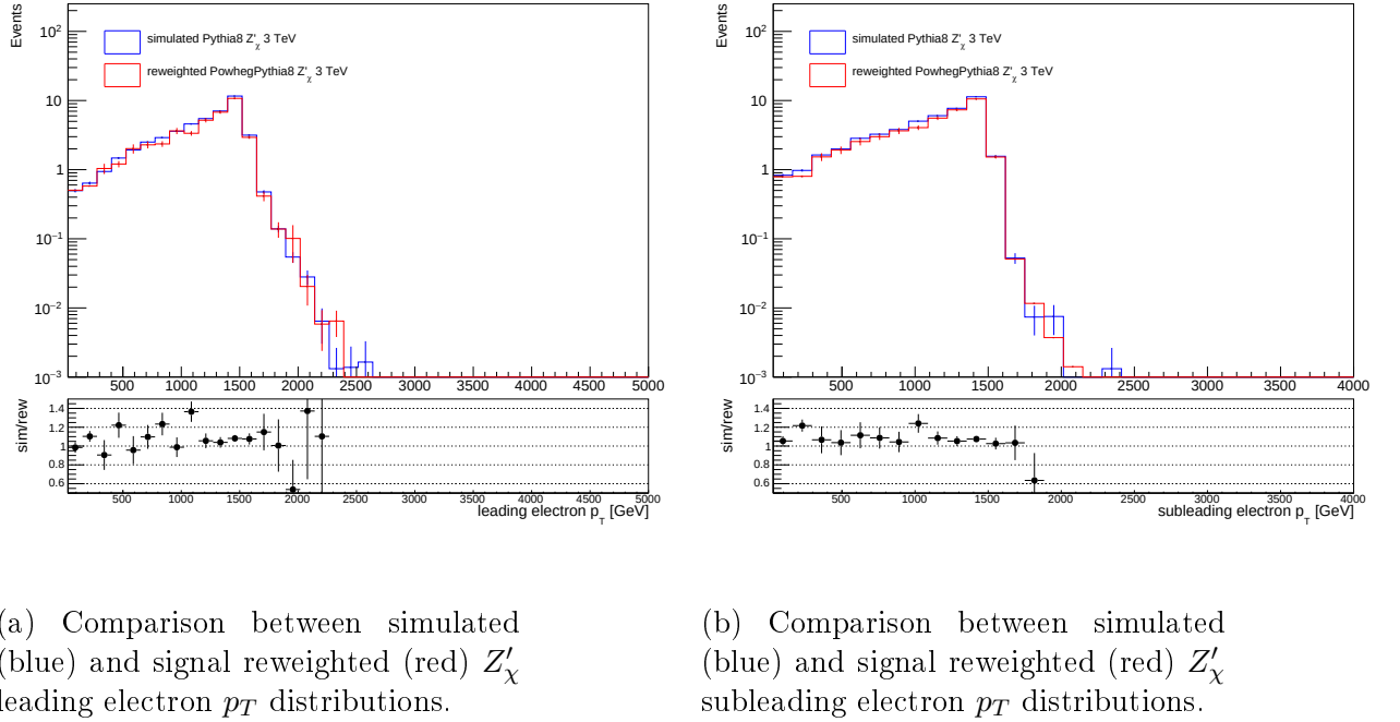
Figure 7.4: Comparison of Z'_\chi leading (a) and electron subleading (b) p_T distributions.
