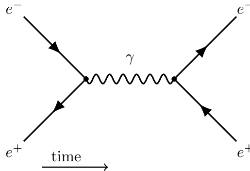
Figure 2.1: The Feynman diagram showing the process e^-e^+ \rightarrow \gamma \rightarrow e^-e^+ with the time going from left to right as indicated by the arrow.
