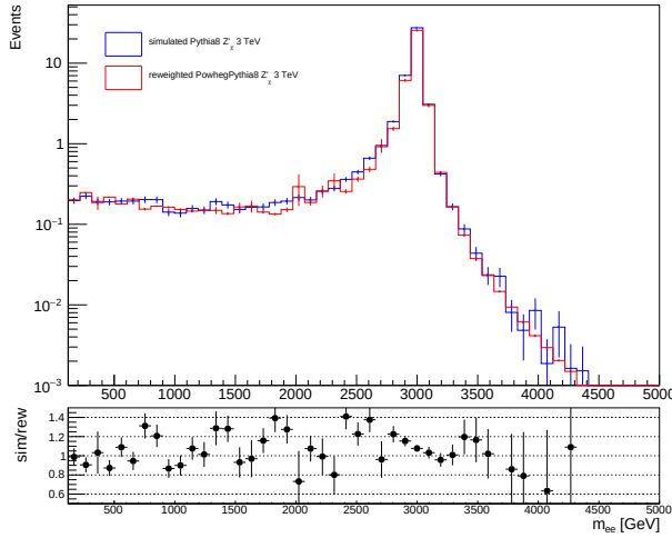
(a) Comparison between simulated (blue) and signal reweighted (red) Z'_\chi invariant mass distributions (log)
