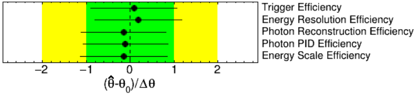
Figure 3.9: Pulls and constraints on the fitted nuisance parameters considered in the fit under the signal-plus-background hypothesis. For each NP, the fitted value represents the preferred shift with respect to the prediction in a unit of its prior uncertainty, and the fitted error represents the uncertainty after the fit in a unit of its prior uncertainty
