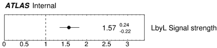
Figure 3.12: Estimation of the Light-by-Light signal strength by the fit.
