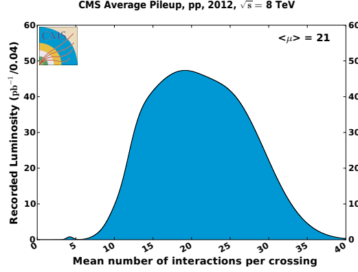
Figure 2.2: Distribution of the mean number of pp interaction per bunch crossing, as recorded at the CMS collision point in 2012 [55].
