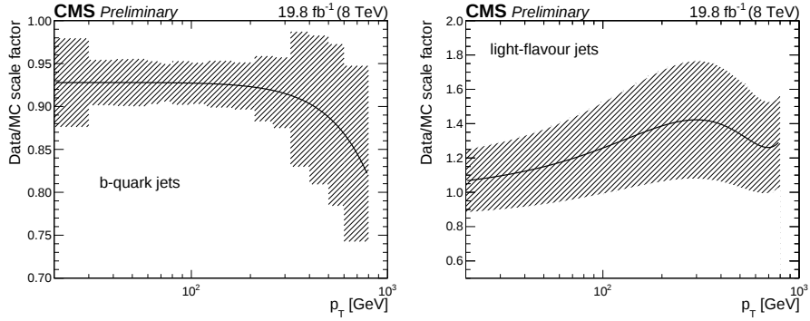
Figure 4.3: Difference in b -tagging efficiencies between data and simulation. The scale factors are derived in a single bin in jet pseudorapidity.
