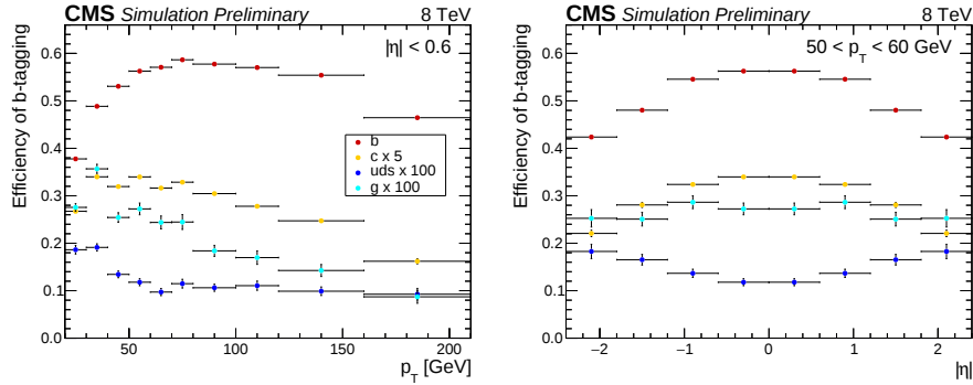
Figure 3.12: Efficiencies of b -tagging as determined from simulation.
