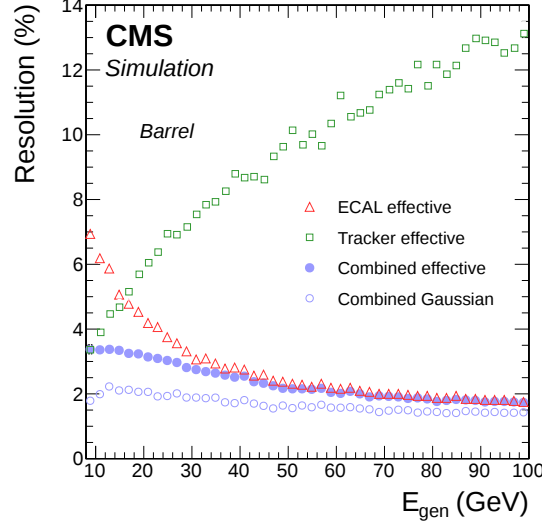
Figure 3.3: Electron momentum resolution after combining p and E_{\text{SC}} measurements, compared to estimates based on track momentum and SC energy alone [80]. Open circles correspond to the Gaussian core of the distribution.
