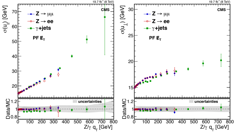
Figure 3.14: \cancel{E}_T resolution curves for parallel (left) and perpendicular (right) components of the hadronic recoil [100].
