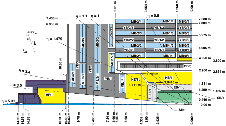
Figure 2.6: A quarter view of the CMS detector in the (y, z) plane [62].
