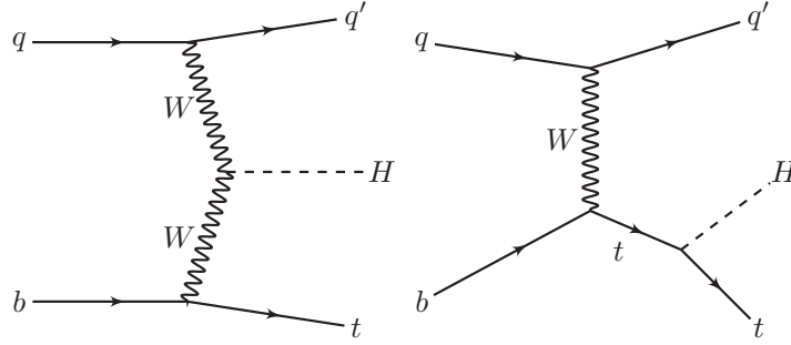
Figure 1.2: Dominant Feynman diagrams for the tH production in the t channel.
