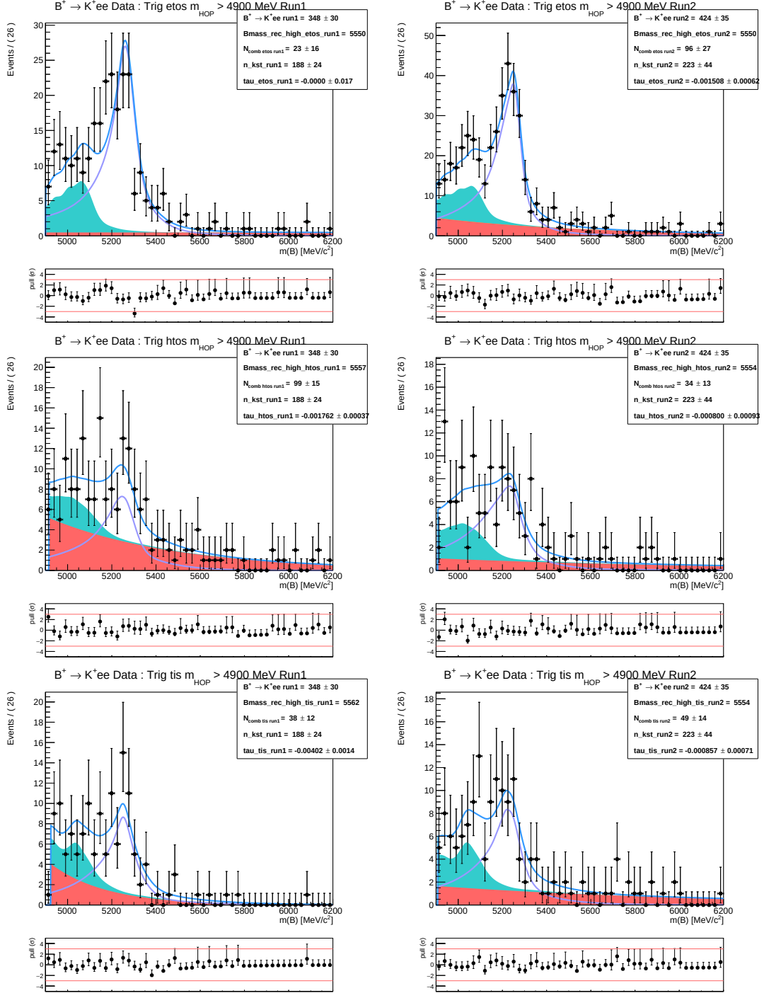
Figure 4.22: Run1 (left) and Run2 (right) mass fits to the m_{HOP} > 4900 \text{ MeV} region for B^+ \rightarrow K^+ e^+ e^- fully selected data, split into trigger categories eTOS (top), hTOS (centre), TIS (bottom). The combinatorial background is shown in red, the partially reconstructed background in teal, and the entire signal model in purple. Each individual bremsstrahlung category as a dashed blue line, and the total model as a solid blue line.
