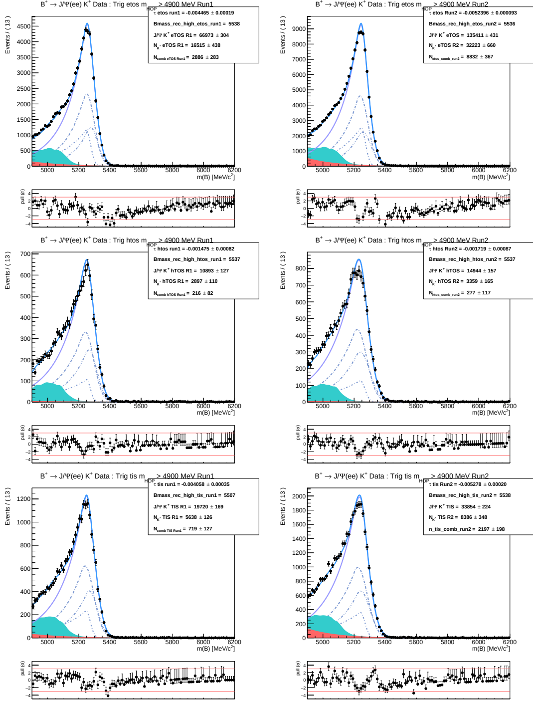
Figure 4.20: Run1 (left) and Run2 (right) fits to the m_{HOP} > 4900 MeV region for B^+ \rightarrow J/\Psi(e^+e^-)K^+ fully selected data, split into trigger categories eTOS (top), hTOS (centre), TIS (bottom). The combinatorial background is shown in red, the partially reconstructed background in teal, and the entire signal model in purple. Each individual bremsstrahlung category as a dashed blue line, and the total model as a solid blue line.
