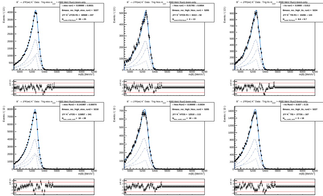
Figure A.13: Run1 (top) and Run2 (bottom) fits to the m_{HOP} > 4900 \text{ MeV} region for B^+ \rightarrow J/\Psi(e^+e^-)K^+ fully selected and mass constrained ( m_{const} > 5185 \text{ MeV} ) data, split into trigger categories eTOS (left), hTOS (centre), TIS (right). The combinatorial background would be shown in red, although the yield is compatible with zero in all cases. Each individual bremsstrahlung category as a dashed blue line, and the total model as a solid blue line.
