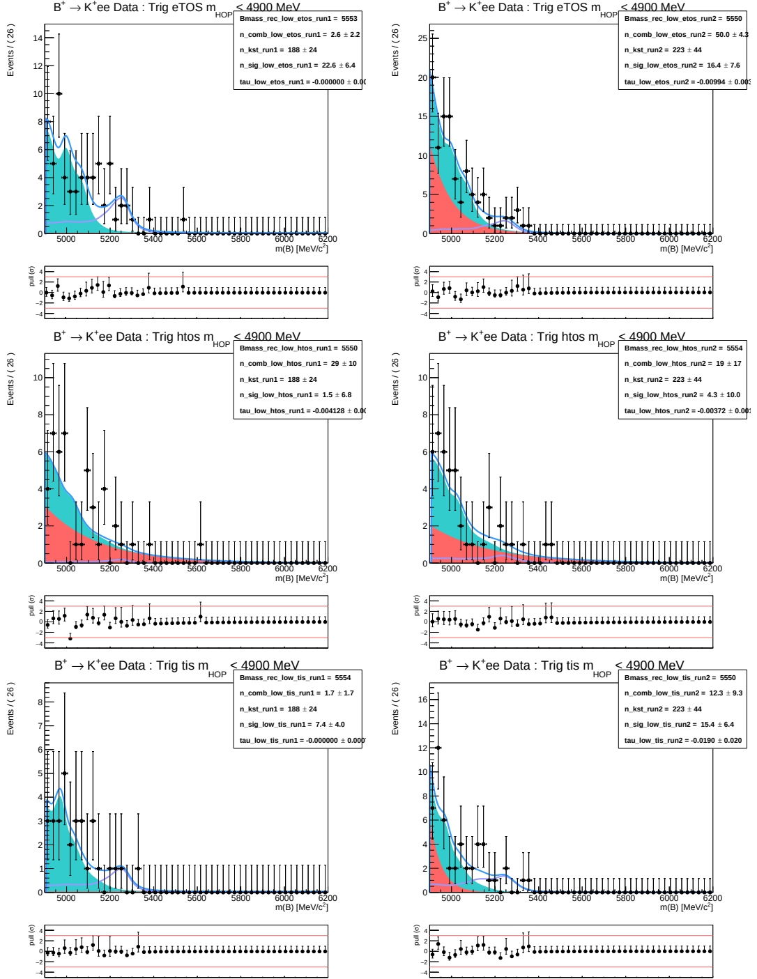
Figure 4.21: Run1 (left) and Run2 (right) mass fits to the m_{HOP} < 4900 \text{ MeV} region for B^+ \rightarrow K^+ e^+ e^- fully selected data, split into trigger categories eTOS (top), hTOS (center), TIS (bottom). The combinatorial background is shown in red, the signal leaking into the low HOP region in purple, the partially reconstructed background in teal, and the total model in blue.
