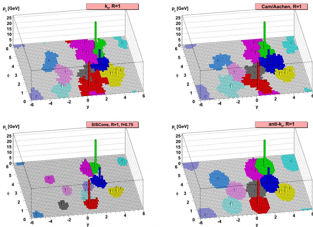
FIGURE 4.10. A sample parton-level event with many random soft jet objects, clustered with four different jets algorithms, illustrating the areas of the resulting hard jets. For k_t and Cambridge/Aachen the detailed shapes are in part determined by the specific set of ghosts used, and change when the ghosts are modified[70].
