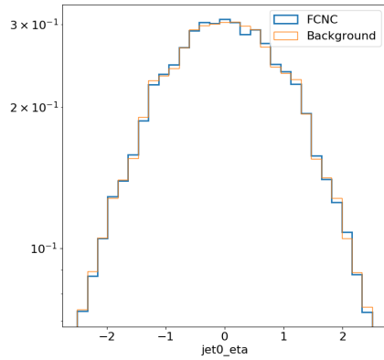
(e) \eta
