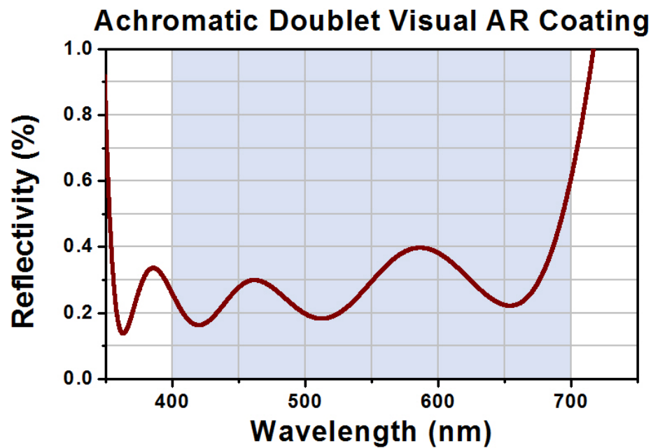
Figure B.12.: Reflectivity of the achromatic doublet used as second collimator lens.[27]
