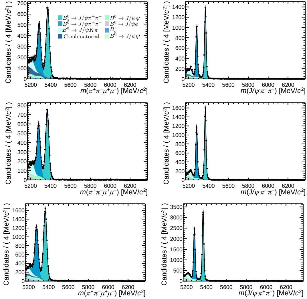
Figure 8.11: The final resonant mode invariant mass fits for the 2011+2012 (top), 2015+2016 (middle) and 2017+2018 (bottom) datasets. The left column shows the fits without the J/\psi mass constraint applied and the right plots with the J/\psi mass constraint applied.
