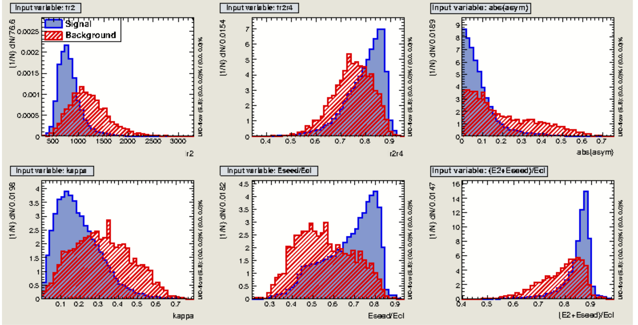
Figure II-10: Distributions of ECAL cluster shape variables (clockwise from top left): r2 , r2r4 , |asym| , \kappa , E_{seed}/E_{cl} and (E_{seed} + E_{2nd})/E_{cl} for photons (blue) and merged \pi^0 selected as photons (red) in the inner ECAL region. Figure is from Ref. [59].
