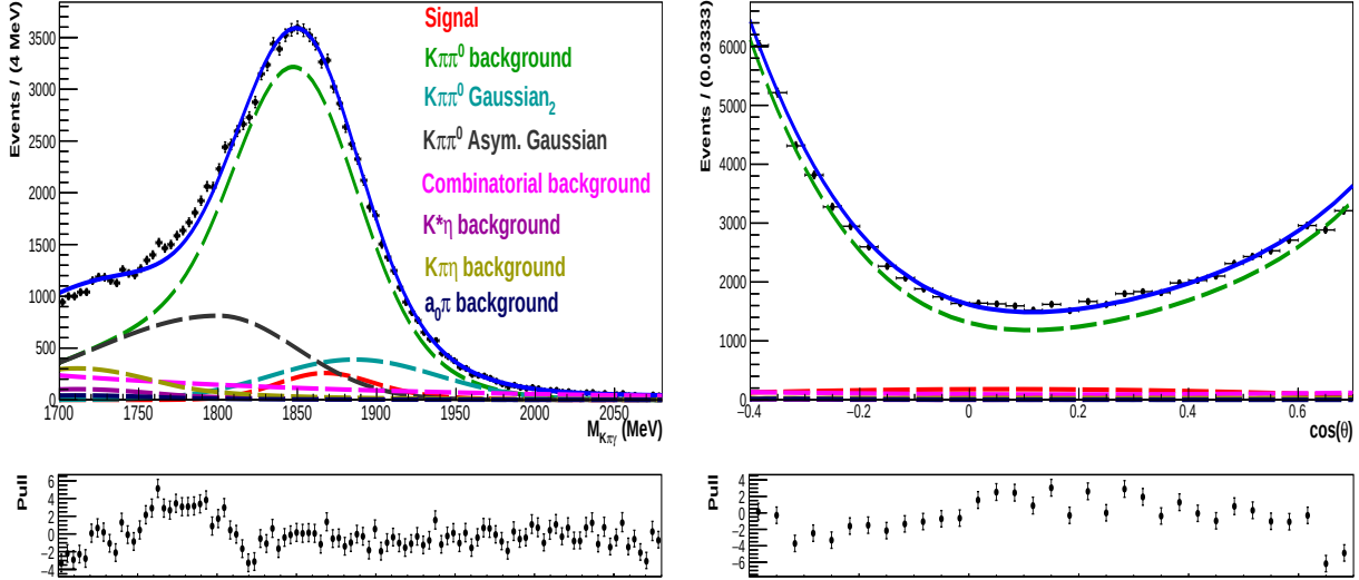
Figure V-3: (Left) M(D^0) and (right) \cos \theta projections of two-dimensional M(D^0) vs. \cos \theta fit to D^0 \rightarrow \bar{K}^{*0}\gamma candidates reconstructed in the Run-1 data in the helicity center. The \cos \theta projection is for 1805 < M(D^0) < 1924 MeV/ c^2 . No selection on IsPhoton or \gamma\text{--}\pi^0 BDT classifier is applied. Fit components are indicated in the legend.
