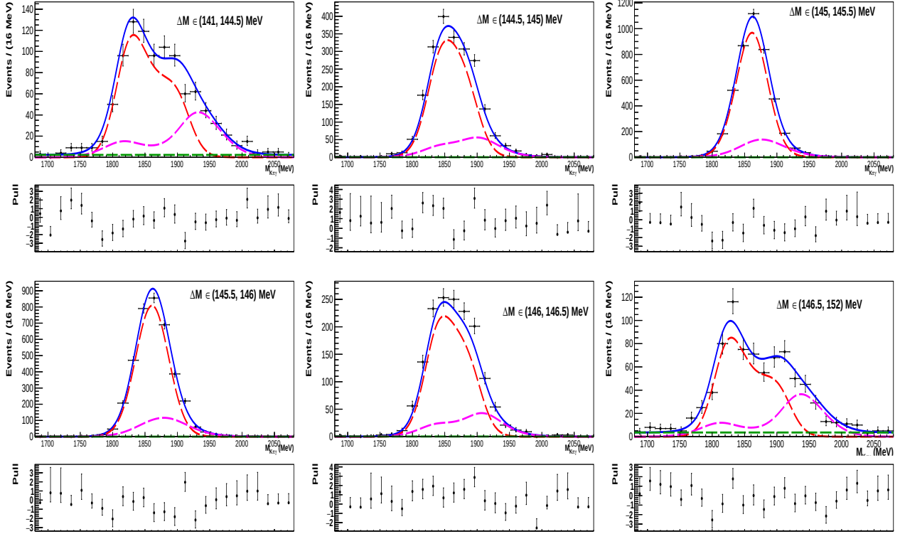
Figure IV-23: Results of two-dimensional M(D^0) - \Delta M fit performed for D^0 \rightarrow \bar{K}^{*0}\gamma simulation. M(D^0) projections are for \Delta M regions indicated in individual plots. Red and magenta lines describe G_1 and G_2 signal sub-components, green line is combinatorial background, blue line is total fit function.
