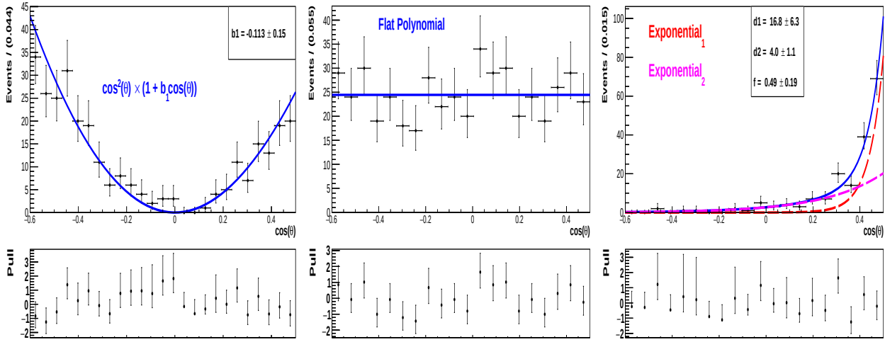
Figure IV-49 : Distributions of \cos\theta in the helicity-center region for (left) D^0 \rightarrow \rho^0 \eta decays, (middle) D^0 \rightarrow \pi^+ \pi^- \eta decays, (right) D^0 \rightarrow a_0(980)^+ \pi^- decays. Fit results are superimposed. Parameters quoted in the right figure are exponents d_1 and d_2 of two exponential functions, and fraction f of the first function.
