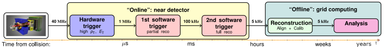
Figure II-7: A simplified scheme of the data flow from collisions to the offline storage in Run-1.
