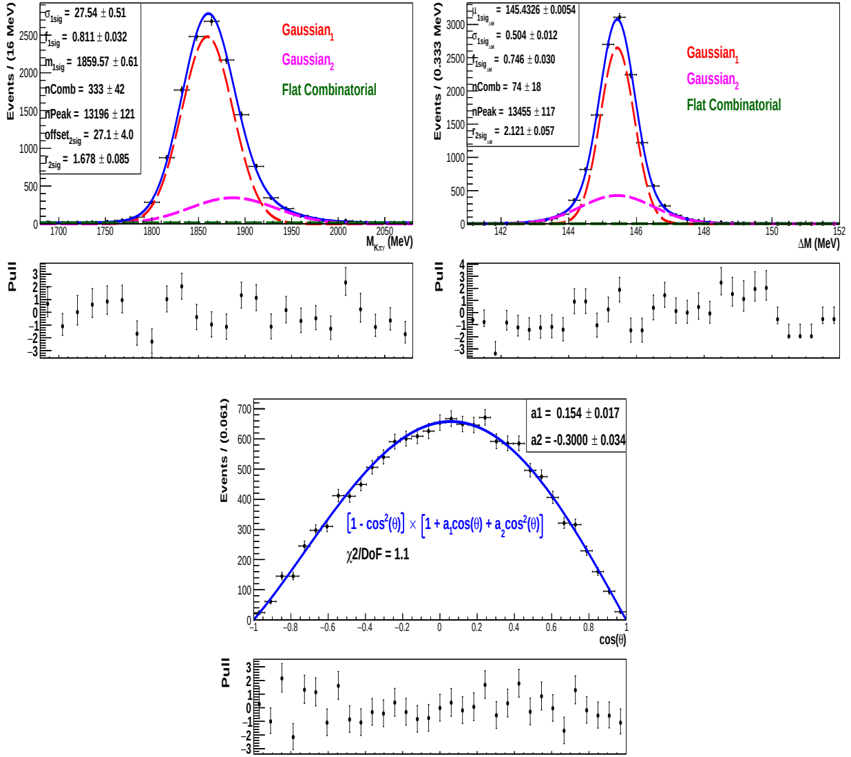
Figure IV-9: Distributions of (top left) M(D^0) , (top right) \Delta M and (bottom) \cos\theta for simulated D^0 \rightarrow \bar{K}^{*0}\gamma decays. Results of one-dimensional fits are superimposed.
