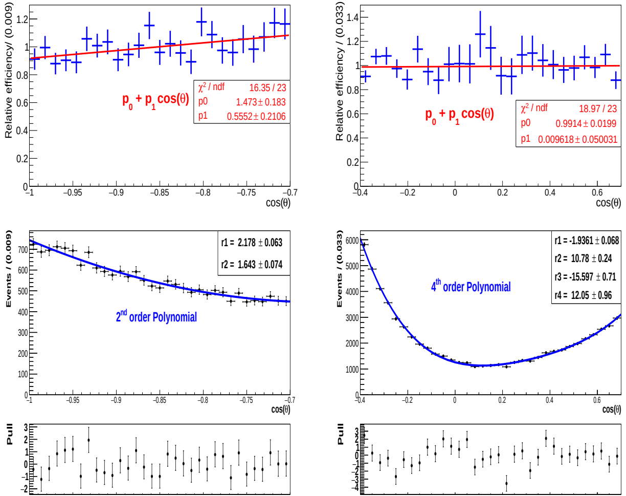
Figure IV-11 : (Top) Efficiency as a function of \cos\theta for D^0 \rightarrow \bar{K}^{*0}\pi^0 simulation sample in (top left) helicity-edge and (top right) helicity-center regions. (Bottom) Theoretical \cos\theta distribution in (bottom left) helicity-edge and (bottom right) helicity-center regions generated with the BaBar model for the D^0 \rightarrow K^-\pi^+\pi^0 decay. Results of fits are superimposed.
