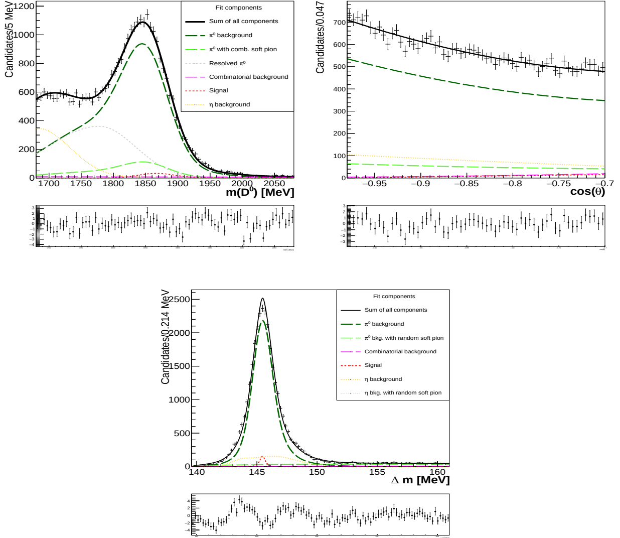
Figure V-4: (Top left) M(D^0) , (top right) \cos \theta and (bottom) \Delta M projections of three-dimensional fit to D^0 \rightarrow \bar{K}^{*0} \gamma candidates, with \text{IsPhoton} > 0.86 , reconstructed in the Run-1 data in the helicity-edge region -0.97 < \cos \theta < -0.7 . These projections are in the full fit region. Fit components are indicated in the legend.
