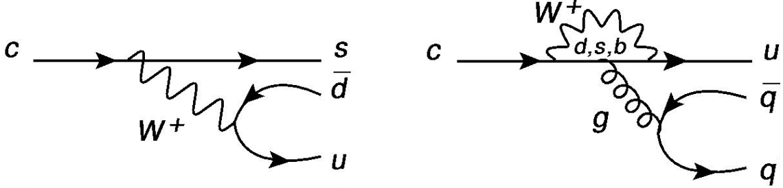
Figure I-2: Diagrams for charm-quark transitions occurring through (left) tree-level c \rightarrow sW^+ process, followed by W^+ boson coupling to u\bar{d} pair, and (right) loop-level c \rightarrow u process with d , s or b quark entering the loop. This loop process is a QCD penguin, with emitted gluon g coupling to q\bar{q} quark pair.
