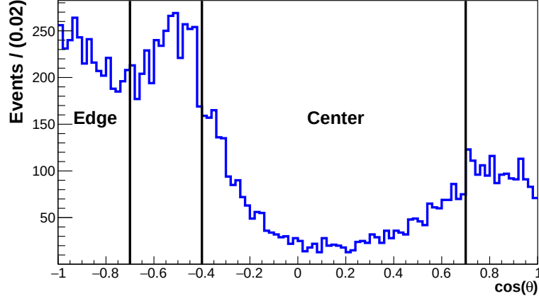
Figure III-3 : Distribution of \cos\theta in D^0 \rightarrow K^-\pi^+\pi^0 simulation sample passing the D^0 \rightarrow \bar{K}^{*0}\gamma signal selection. Edge and central helicity regions are indicated.
