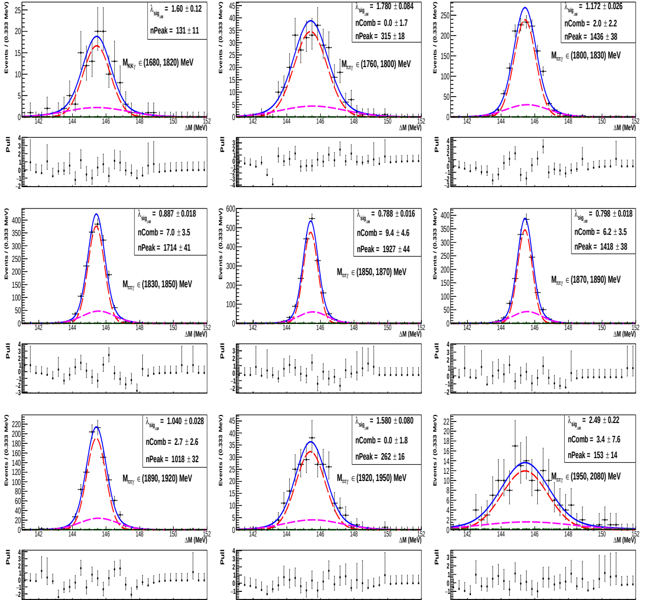
Figure IV-50: Results of \Delta M fits in M(D^0) bins performed using the D^0 \rightarrow \rho^0 \gamma simulation sample. Considered M(D^0) regions, as well as fitted \lambda values are indicated in individual figures.
