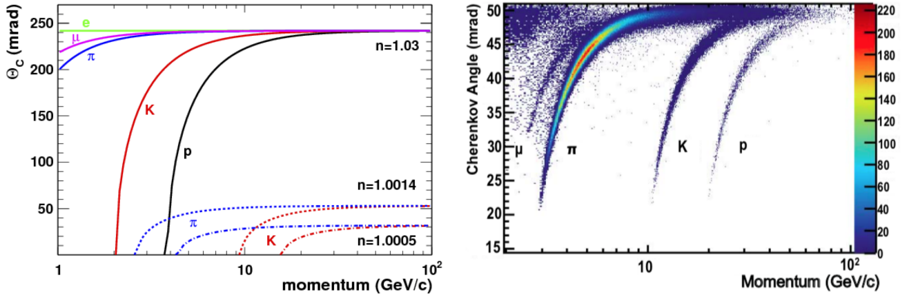
Figure II-3: (Left) Cherenkov angle as a function of momentum for different particle species, and for the three radiators used in RICH1 and RICH2. (Right) Response of the gas radiator in RICH1 to charged particles; the Cherenkov angle is measured with the Run-1 data. Figures are from Ref. [48].
