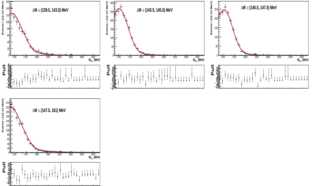
Figure IV-27 : Results of two-dimensional M(D^0) – \Delta M fit performed for D^0 \rightarrow \bar{K}^{*0}\eta simulation. M(D^0) projections are for \Delta M regions indicated in individual plots. Red line describes \eta component, green line is combinatorial background, blue line is total fit function.
