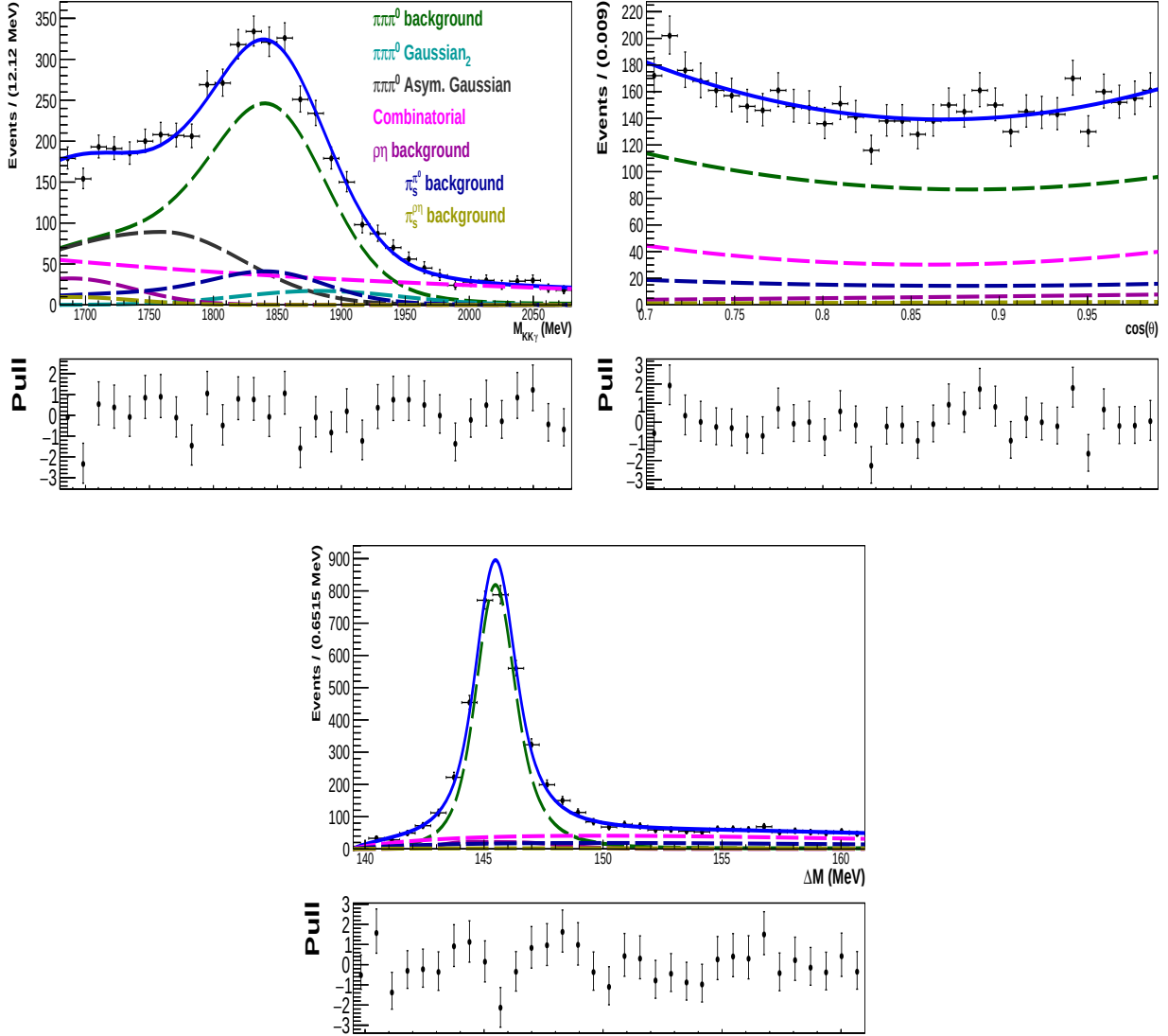
Figure V-22: (Top left) M(D^0) , (top right) \cos \theta and (bottom) \Delta M projections of three-dimensional fit to D^0 \rightarrow \rho^0 \gamma candidates, with \text{IsPhoton} > 0.95 , reconstructed in the Run-1 data in the helicity-edge region, \cos \theta > 0.7 . These projections are in the full fit region. Fit components are indicated in the legend.
