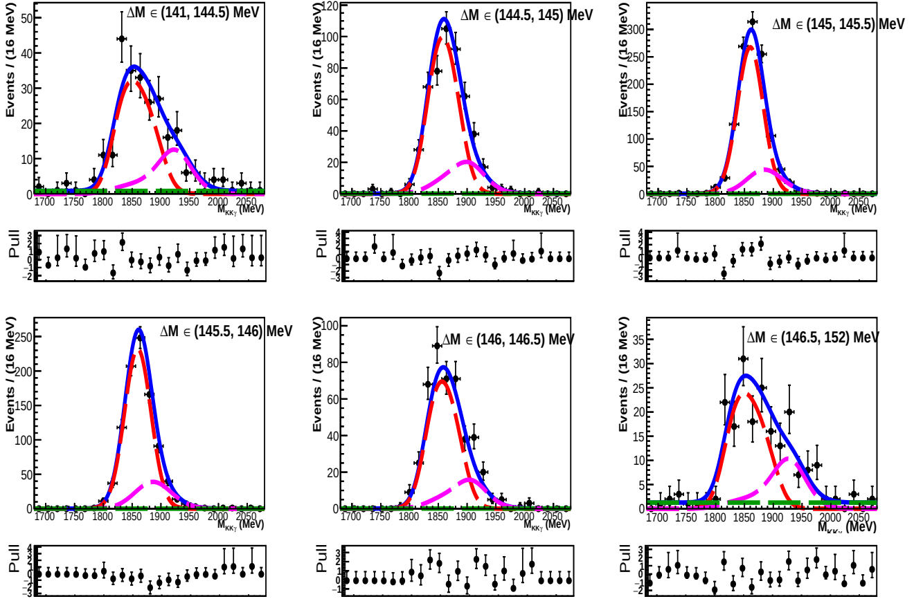
Figure IV-38: Results of two-dimensional M(D^0) – \Delta M fit performed for D^0 \rightarrow \phi\gamma simulation. M(D^0) projections are for \Delta M regions indicated in individual plots. Red and magenta lines describe G_1 and G_2 signal sub-components, green line is combinatorial background, blue line is total fit function.
