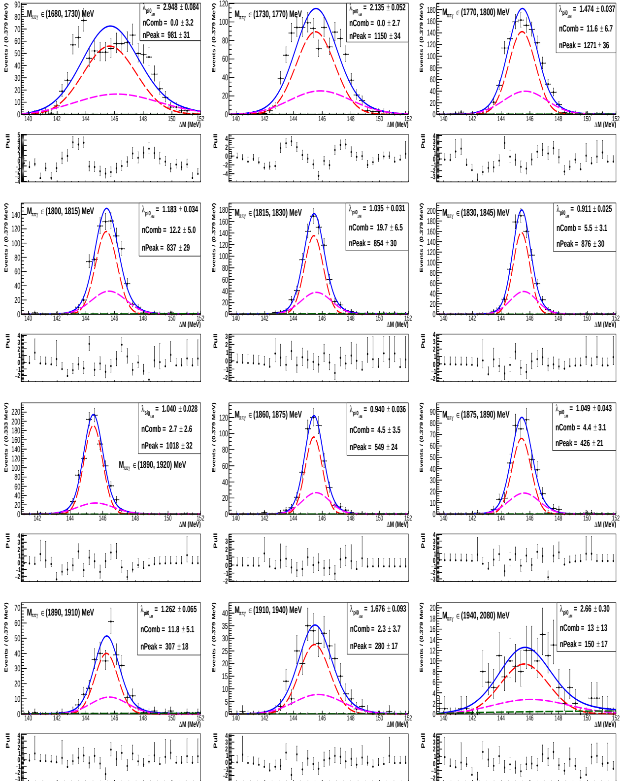
Figure IV-52: Results of \Delta M fits in M(D^0) bins performed using the D^0 \rightarrow \rho^0 \pi^0 simulation sample. Considered M(D^0) regions, as well as fitted \lambda values are indicated in individual figures.
