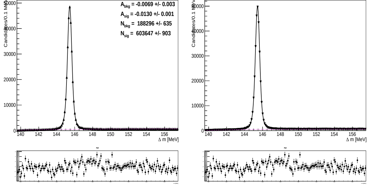
Figure VII-2 : \Delta M distribution for (left) \pi_s^+ -tagged D^0 \rightarrow \pi^+\pi^- and (right) \pi_s^- -tagged \bar{D}^0 \rightarrow \pi^-\pi^+ candidates in the Run-1 data before kinematic reweighing. Results of the simultaneous fit are superimposed; black line shows the total fit, dashed magenta line shows combinatorial background.
