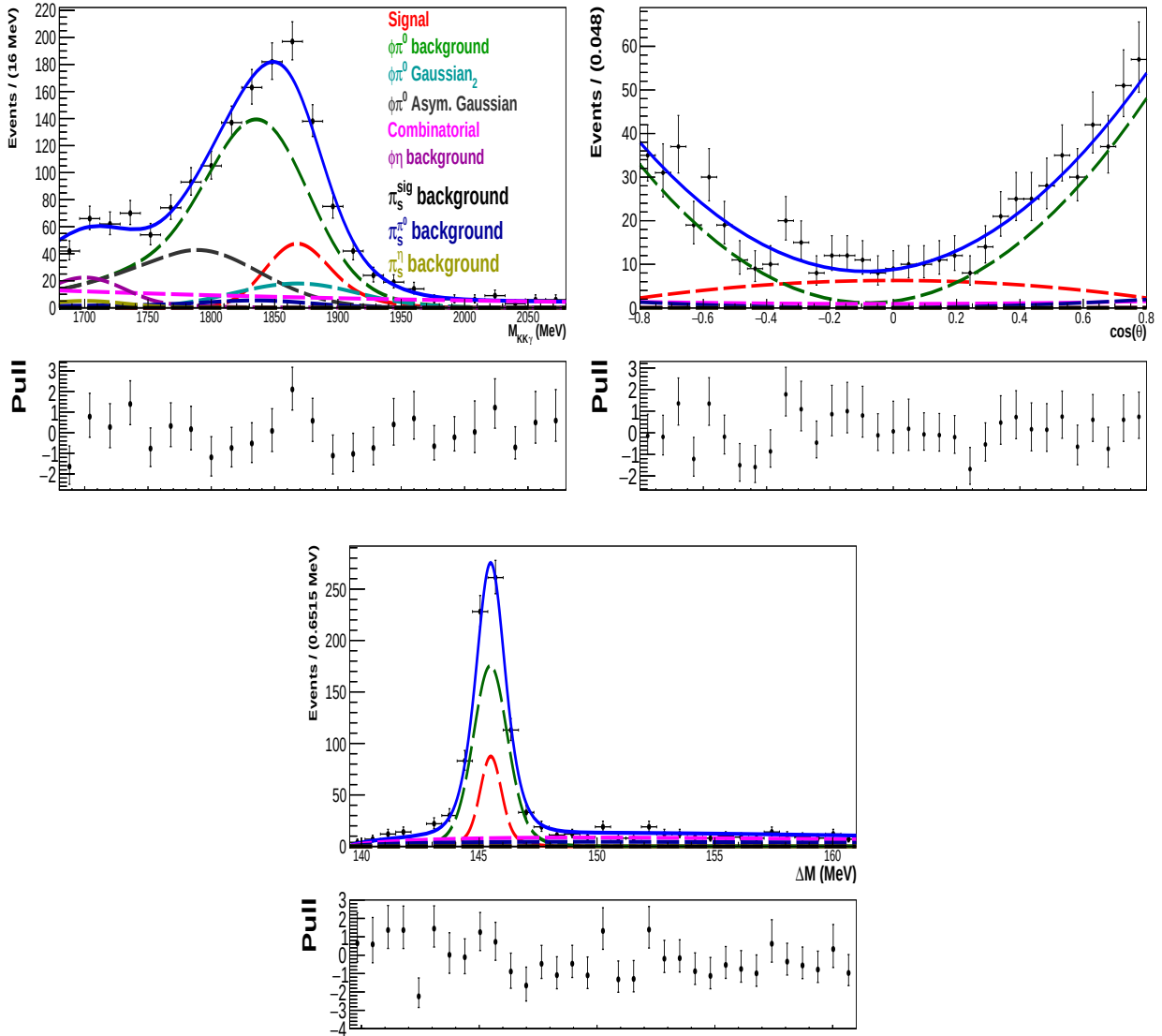
Figure V-17: (Top left) M(D^0) , (top right) \cos\theta and (bottom) \Delta M projections of three-dimensional fit to D^0 \rightarrow \phi\gamma candidates, with IsPhoton > 0.85, reconstructed in the Run-1 data in the helicity center |\cos\theta| < 0.8 . These projections are in the signal-enhanced region. Fit components are indicated in the legend.
