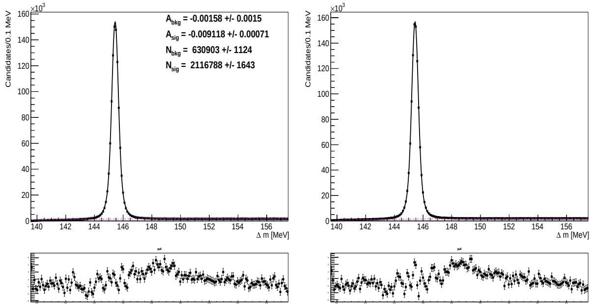
Figure VII-1: \Delta M distribution for (left) \pi_s^+ -tagged D^0 \rightarrow K^+K^- and (right) \pi_s^- -tagged \bar{D}^0 \rightarrow K^-K^+ candidates in the Run-1 data before kinematic reweighing. Results of the simultaneous fit are superimposed; black line shows the total fit, dashed magenta line shows combinatorial background.
