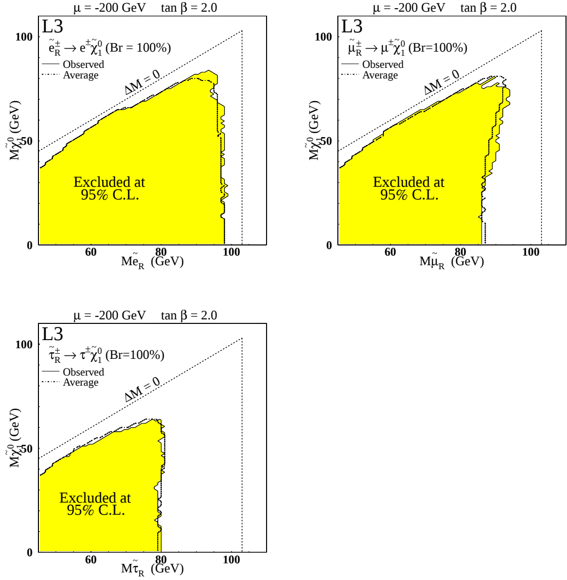
Figure 6.13: Excluded region at 95% C.L. in the M_{\tilde{\chi}_1^0} - M_{\tilde{l}} plane, for three scalar lepton flavors.
