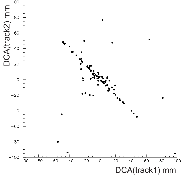
Figure 7.4: Since cosmic rays are recognized as two outgoing particles, they can be found along the band near DCA(track1) + DCA(track2) = 0 .
