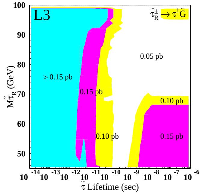
Figure 7.9: Model independent limit on the production cross section of \tilde{\tau} at \sqrt{s} = 205 GeV, as a function of M_{\tilde{\tau}} and its lifetime.
