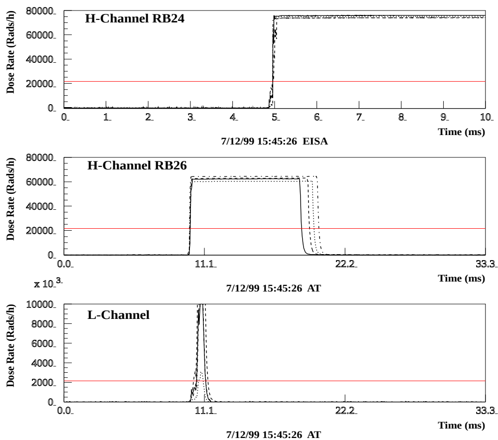
Figure 4.6: The waveform of a typical category a event (this is also an a* event).
