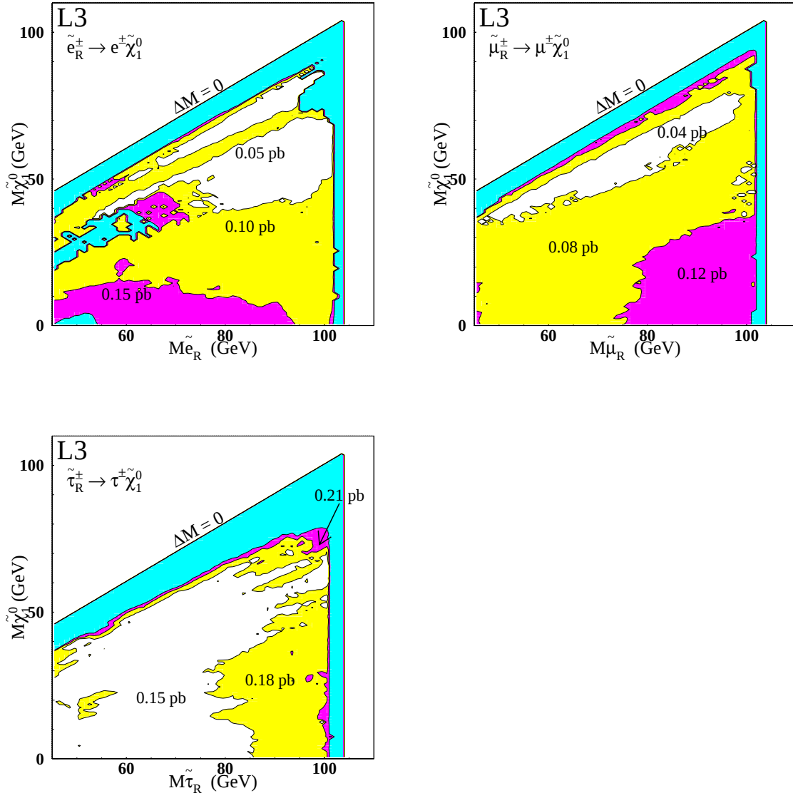
Figure 6.12: Model independent limit on the production cross section at \sqrt{s} = 205 \text{ GeV} , in the M_{\tilde{\chi}_1^0} - M_{\tilde{l}} plane, for all three scalar lepton flavors.
