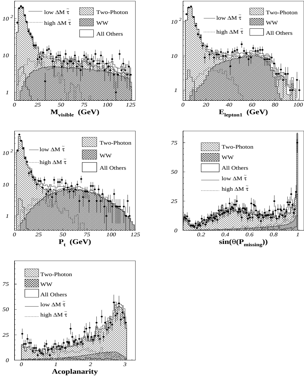
Figure 6.4: Data and Monte Carlo simulation agreement on important variables: after pre-selection for scalar \tau . Plots shown are for the data sample of 1999. The simulated \tilde{\tau} signals with M_{\tilde{\tau}} = 80 \text{ GeV} and \Delta M = 6 \text{ GeV} (low), and with \Delta M = 45 \text{ GeV} (high) are also shown.
