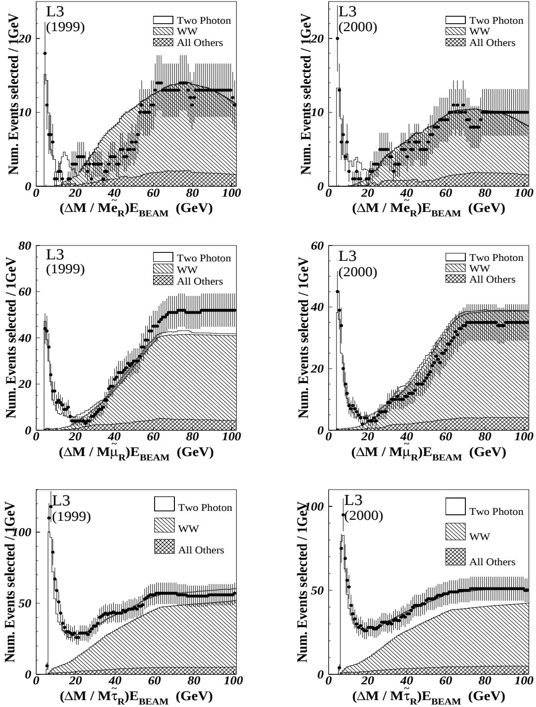
Figure 6.11: Selected data events and expected background level as a function of the parameter Z = (\Delta M / M_{\tilde{l}_R}) \times E_{beam} , for \tilde{e} , \tilde{\mu} , \tilde{\tau} selection using data from 1999 and 2000.
