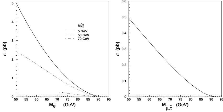
Figure 2.3: The production cross section of the sleptons, as a function of the slepton mass, at \sqrt{s} = 189 \text{ GeV} . The cross section of the selectron depends on the mass of the LSP, due to the t-channel contribution.
