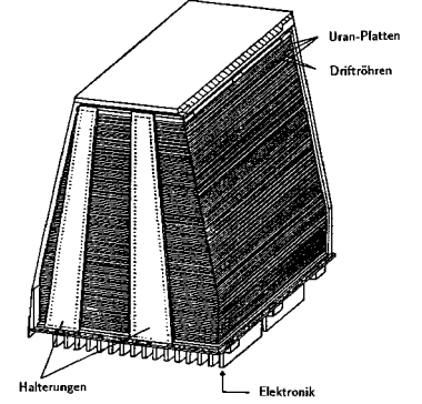
Figure 3.18: A barrel module of the L3 hadron Calorimeter.
