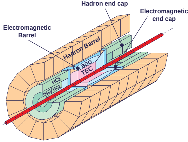
Figure 3.17: A perspective view of the L3 hadron Calorimeter (HCAL).
