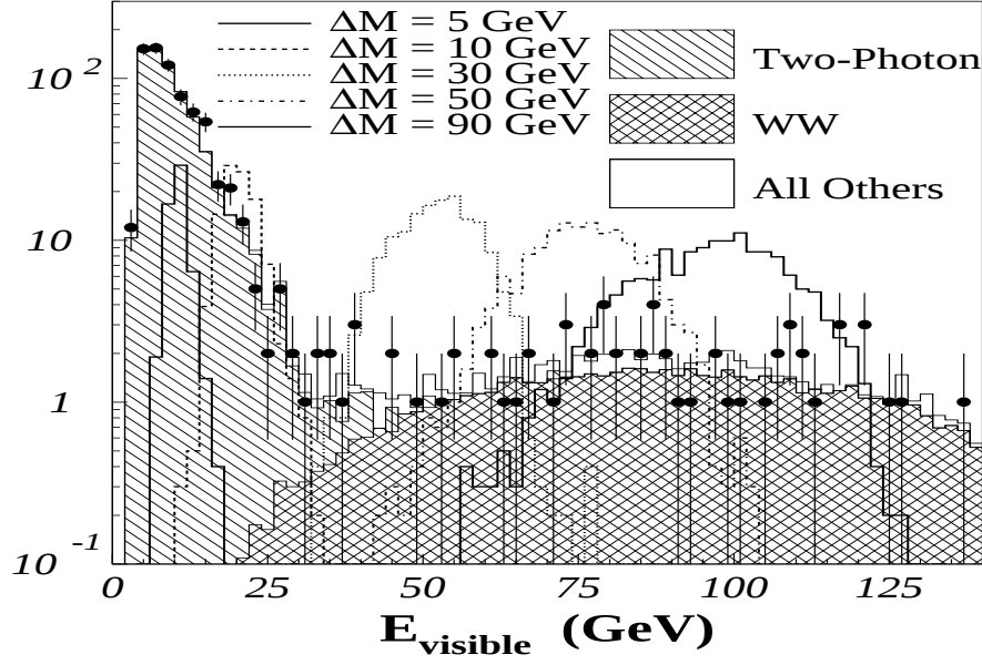
Figure 6.1: Distribution of the total visible energy of a scalar electron signal ( M_{\tilde{e}} = 80 \text{ GeV} ), as a function of \Delta M , compared with the same distribution from the data and the simulated Standard Model background processes.
