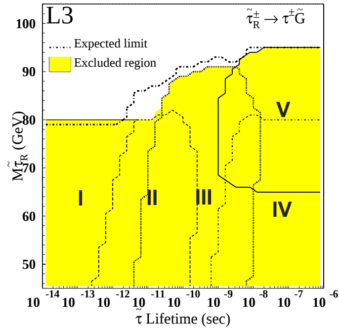
Figure 7.10: Excluded region at 95% C.L. in the M_{\tilde{\tau}} –lifetime plane for \tilde{\tau} , using different selections for: I, prompt decay; II, short decay length; III, medium decay length; IV, long decay length using kinematic cuts only; and V, long decay length using dE/dx information.
