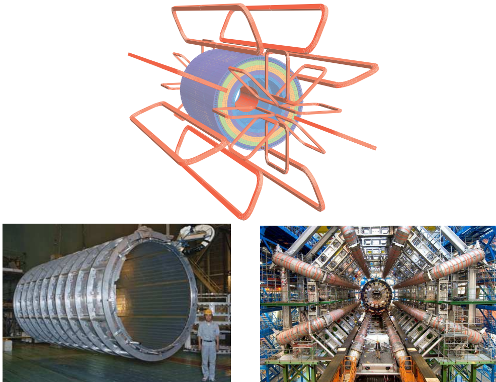
Fig. 3.3: A schematic diagram of the ATLAS magnet system (top), a photograph of the solenoid (left), and a photograph of the ATLAS magnet system (right) are shown. Those are taken from Reference [11].
