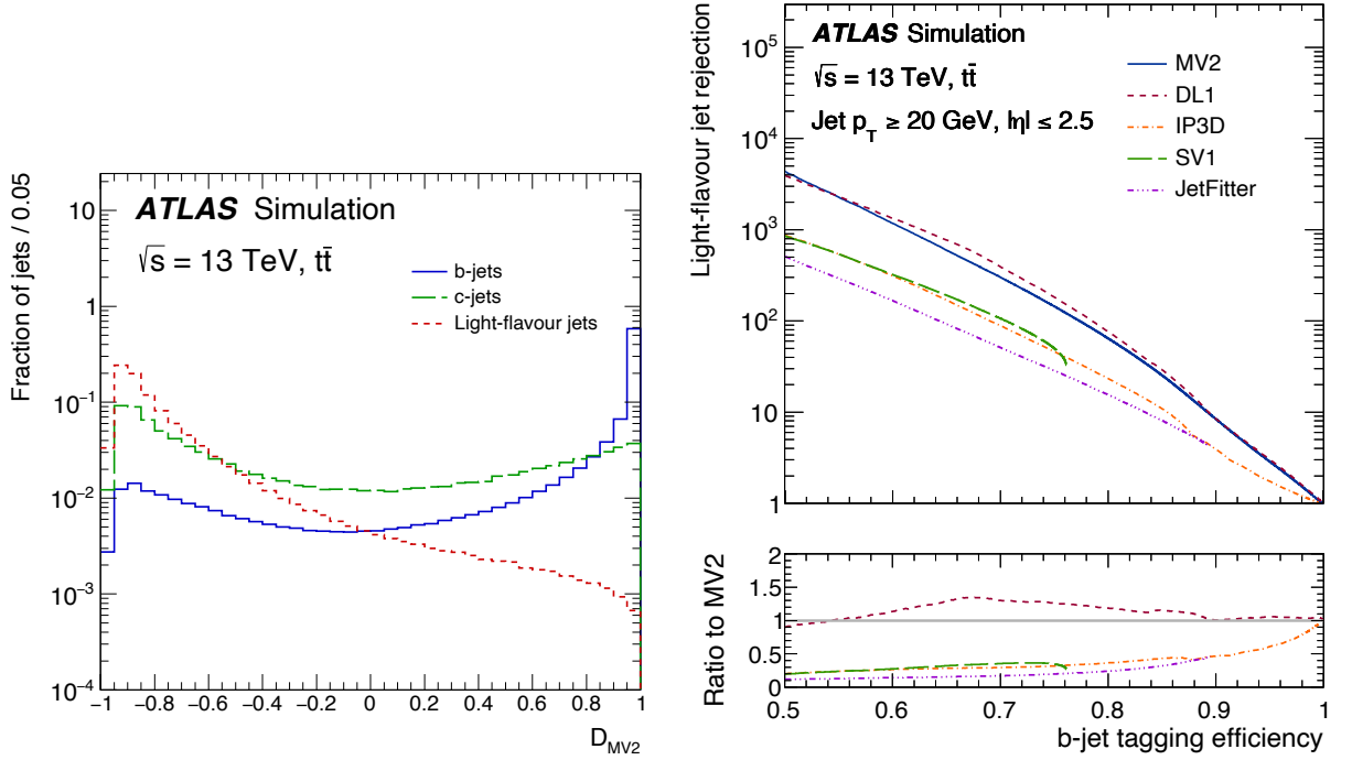
Fig. 4.17: The MV2 outputs (left) and light jet rejections as a function of b-jet tagging efficiency are shown [97]. The MV2 output has discrimination power for not only light jets but also c-hadron jets as shown in the left plot. The right plot represents the MV2 performed much better than its inputs, IP3D, SV1, and JETFITTER. Although the DL1 which uses deep neural network instead of BDT of MV2 has superior light-flavor jet rejection than that of MV2, we have chosen to use MV2 because the calibration for DL1 takes a longer time than that of MV2.
