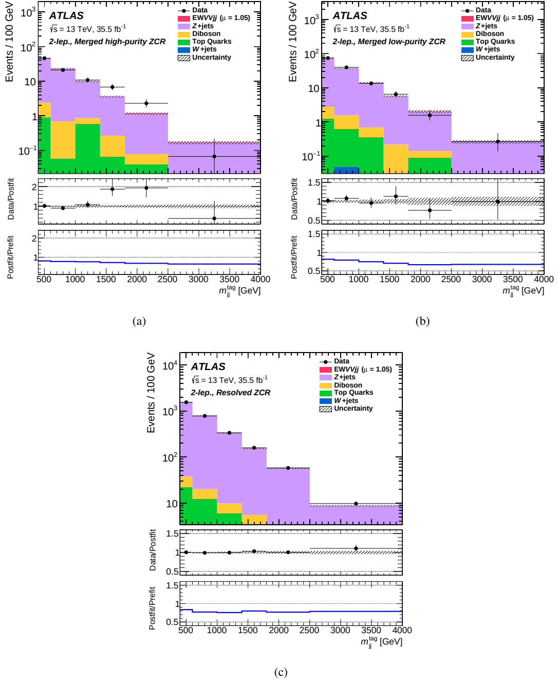
Fig. 6.24: Comparisons of the observed data and expected background distributions of m_{jj}^{\text{tag}} of the Z + jets control regions in the 2-lepton channel: (a) high-purity and (b) low-purity merged signal regions; (c) the resolved signal region. The background contributions after the global likelihood fit are shown as filled histograms. The signal is shown as a filled histogram on top of the fitted backgrounds normalized to the signal yield extracted from the observed data ( \mu = 1.05 ), but it is not visible due to its small contribution. The middle pane shows the ratios of the observed data to the post-fit signal and background predictions. The uncertainty in the total prediction, shown as bands, combines statistical and systematic contributions. The bottom pane shows the ratios of the post-fit and pre-fit background predictions.
