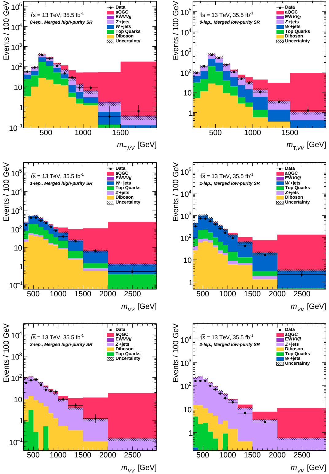
Fig. 7.6: m_{VV} distribution at boosted signal region for 0-lepton HP (top left), 0-lepton LP (top right), 1-lepton HP (middle left), 1-lepton LP (middle right), 2-lepton HP (bottom left), and 2-lepton LP (bottom right) before the fit. Since the normalization factors obtained by the fit are not applied, histograms for MC simulations have approximately 10-20% greater than the observed data. histograms for MC simulations match the observed data when the fit is performed to obtain limits.
