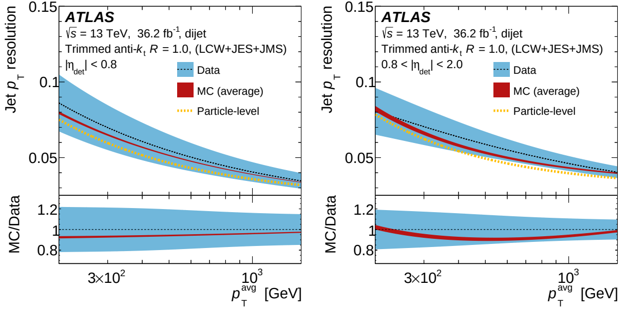
Fig. 5.9: The p_T dependences on jet p_T resolutions at |\eta| < 0.8 (left) and |\eta| > 0.8 (right) regions. The three lines represent the fit results with Equation 5.12 for the observed data (black dashed line), MC simulations (dark red line), and the particle-level (yellow dashed line) which is the resolutions directly calculated from \Delta R -matched truth jet. The widths of lines denote statistical uncertainty in itself. Agreements with the MC simulations and Particle-level support validity of this method. The blue band stands for the combined systematic uncertainties.
