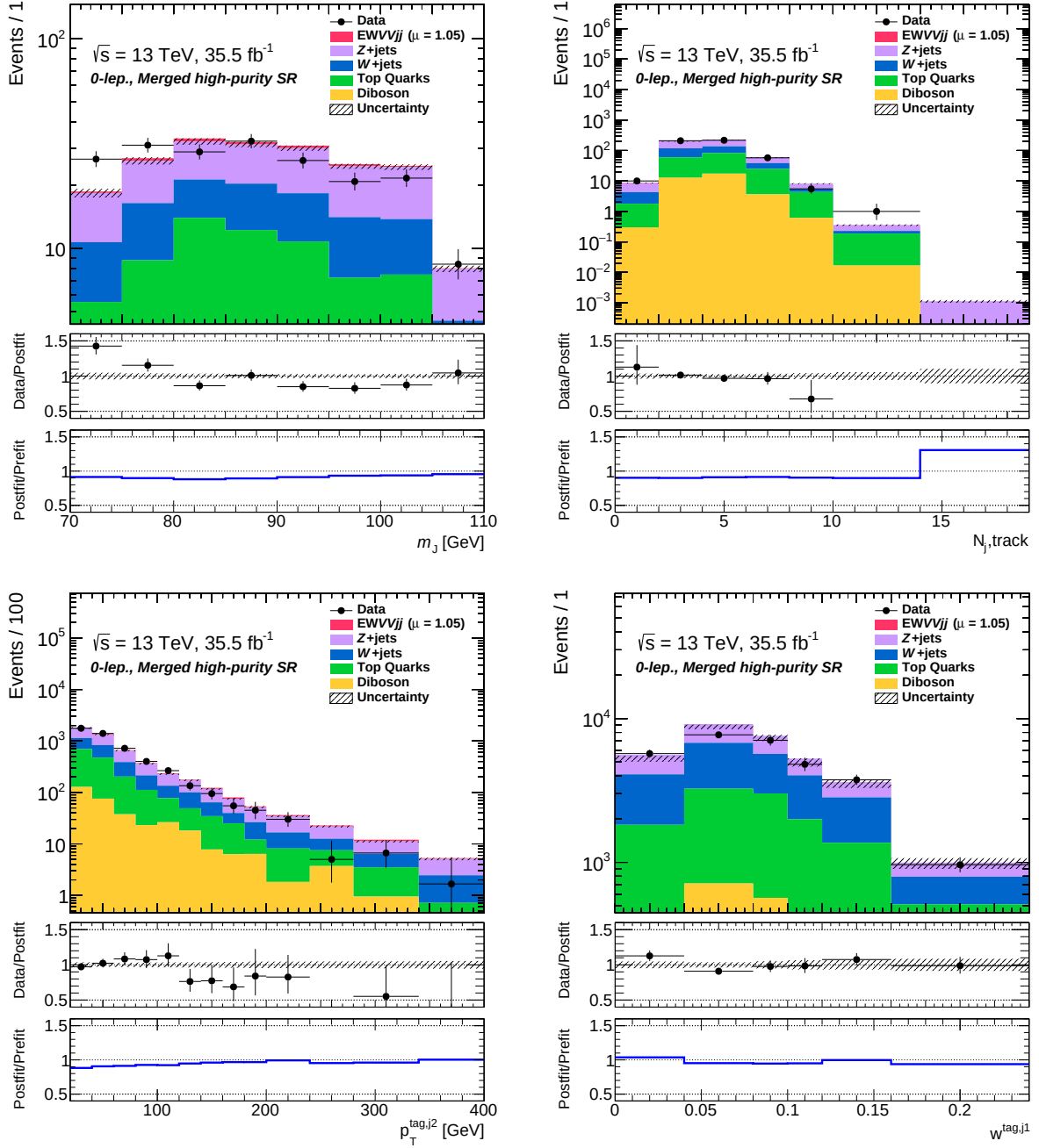
Fig. B.2: Distributions of variables used in the BDT training in the merged high-purity region for the 0-lepton channel applying post-fit uncertainties are shown.
