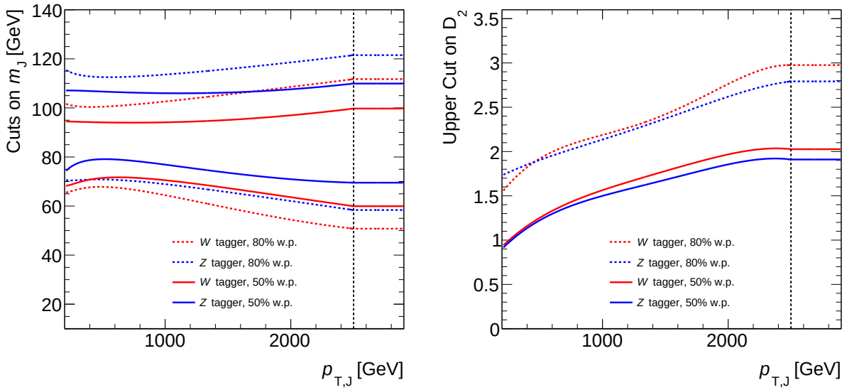
Fig. 5.17: The thresholds of the mass window cuts (left) and the upper cut on D_2 (right) with respect to p_T of a large-R jet are shown. The red and blue (dashed) lines represent 50% (80%) cut thresholds for W and Z boson-tagging. Above the vertical dashed line on p_T = 2500 GeV, the cut thresholds become constants because there is not enough statistics above p_T = 2500 GeV in MC simulated events to define cut thresholds.
