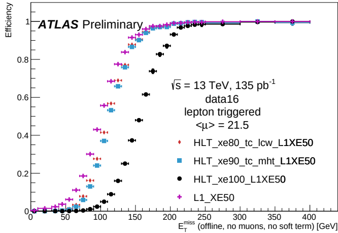
Fig. 4.20: The E_T^{\text{miss}} trigger efficiency with respect to single lepton triggered events corrected in 2016 [100] is shown. The blue square is the one which used in this thesis.
