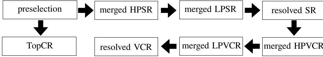
Fig. 6.7: The ordering of the categorization is illustrated. The events passed the preselection are subsequently imposed on criteria in the ordering of allows if those do not pass the previous criteria.
