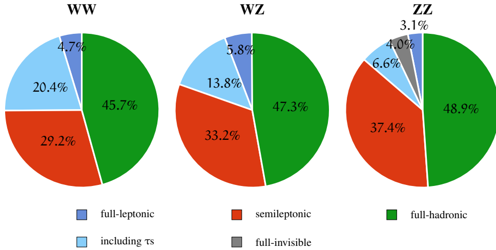
Fig. 2.4: Pie charts representing ratios of each final state are shown. The full-leptonic includes WW \rightarrow l\nu l\nu , WZ \rightarrow l\nu ll , and ZZ \rightarrow ll ll/\bar{l}\nu l\nu , where l and \nu represent charged leptons ( e/\mu ) and neutrinos ( \nu_e/\nu_\mu/\nu_\tau ), and spectator quarks coming from protons are not explicitly shown. The including \tau s represents final states including one or more \tau s. The full-invisible represents ZZ \rightarrow \nu\nu\nu\nu . The semileptonic includes WW \rightarrow l\nu q\bar{q} , WZ \rightarrow l\nu q\bar{q}/ll q\bar{q} , and ZZ \rightarrow ll q\bar{q}/\nu\nu q\bar{q} . The full-hadronic includes WW/WZ/ZZ \rightarrow qq\bar{q}\bar{q} .
