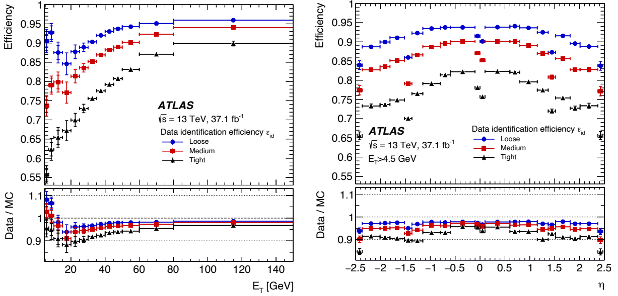
Fig. 4.5: Electron identification efficiencies for E_T (left) and \eta (right) measured in the observed data with Z \rightarrow ee events are shown [77]. The Loose and Tight identification criteria are used in this analysis for the additional electron veto and leptonically decaying W/Z boson reconstruction, respectively. The discrepancy shown in the bottom pane for each plot is corrected in dedicated calibration described in Section 4.3.3.
