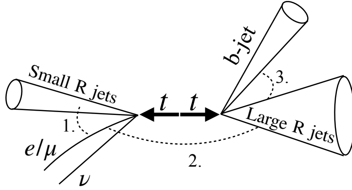
Fig. 9.4: A schematic graph of a selected topology for t\bar{t} events is shown. Three angular cuts, 1.: \Delta R(\text{small-R jet, lepton}) < 1.5 , 2.: \Delta\phi(\text{large-R jet, lepton}) > 2.3 , and 3.: \Delta R(\text{b-jet, large-R jet}) > 1.5 are applied.
