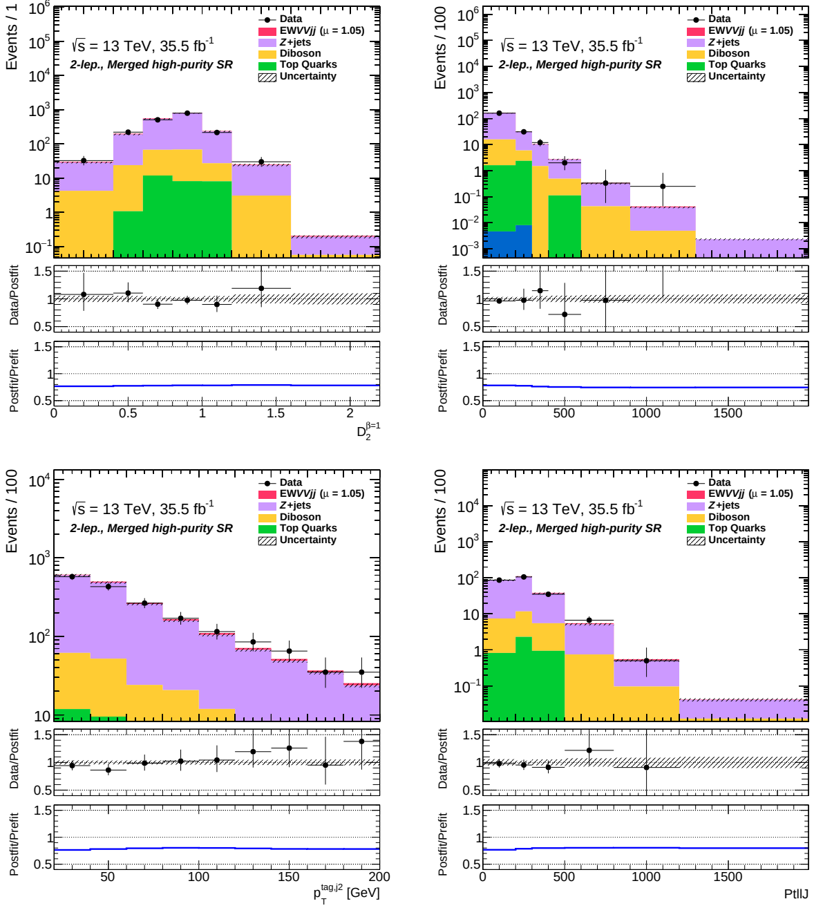
Fig. B.15: Distributions of variables used in the BDT training in the merged high-purity region for the 2-lepton channel applying post-fit uncertainties are shown.
