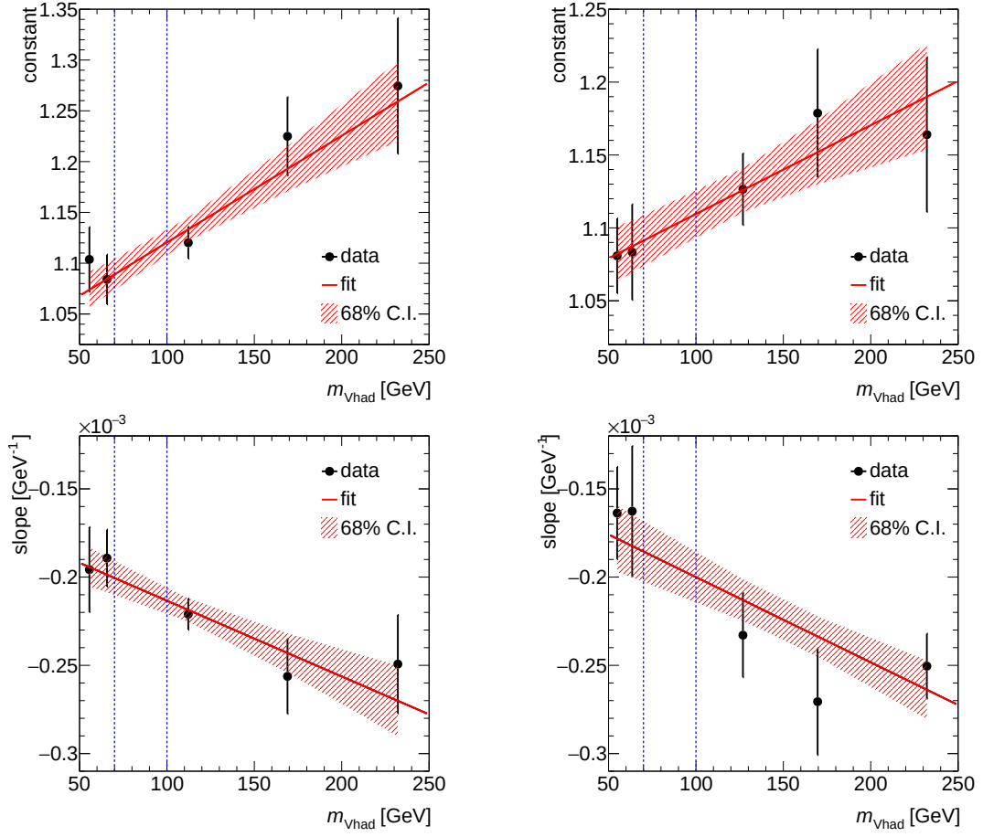
Fig. 6.14: Constants (top) and slopes (bottom) of the reweighting functions as a function of m_{\text{Vhad}} for resolved (left), for merged (right) regions are shown. The red band represents the 68% confidence interval of the linear fit. Regions surrounded by the blue lines roughly correspond to the SR, and the constants and slopes at the center of those blue lines are used for the m_{\text{jj}}^{\text{tag}} reweighting.
