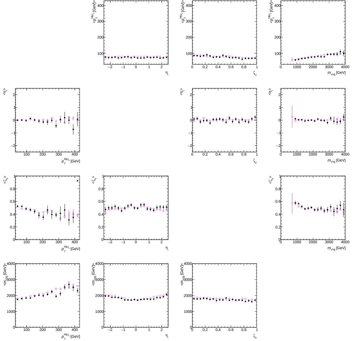
Fig. C.9: The correlations between BDT input variables for the 1-lepton merged signal region are shown. The magenta and black marker represent the MC prediction and observed data. The \langle X \rangle represents mean of the variable X distribution. Only statistical uncertainty in the mean is shown.
