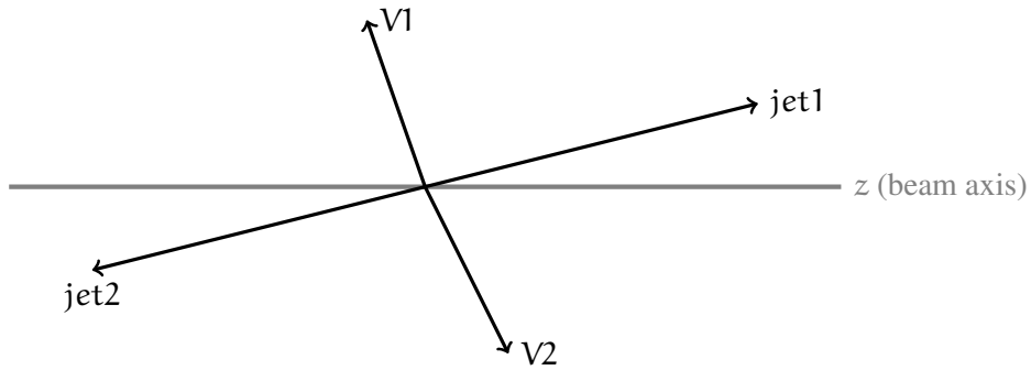
Fig. 6.1: A schematic diagram of a typical VBS topology in the experimental system.
