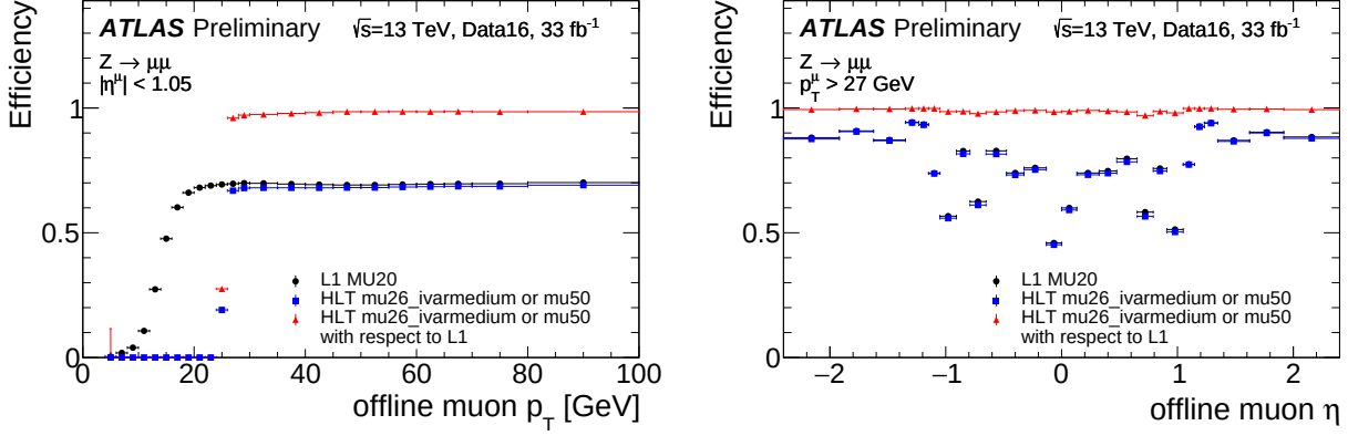
Fig. 4.12: Muon trigger efficiencies as a function of p_T (left) and \eta measured in the 2016 data with Z \rightarrow \mu\mu events are shown [84]. Triggers shown in Table 4.2 are combined by the logical “OR”. The efficiencies are given with respect to offline “Medium” identified muon candidate. The trigger efficiency of the HLT mu26_ivarmedium is sharply turned on around its threshold, and it reached a plateau with a 70% efficiency. The efficiency losses come from L1 trigger inefficiency.
