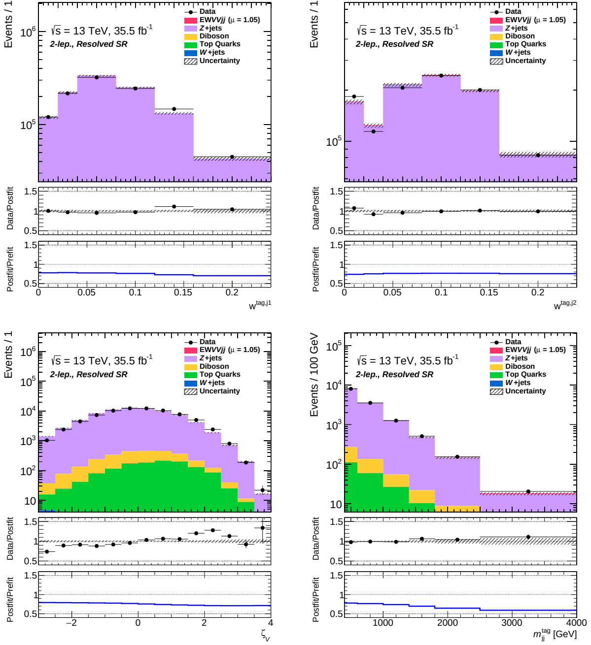
Fig. B.21: Distributions of variables used in the BDT training in the resolved region for the 2-lepton channel applying post-fit uncertainties are shown.
