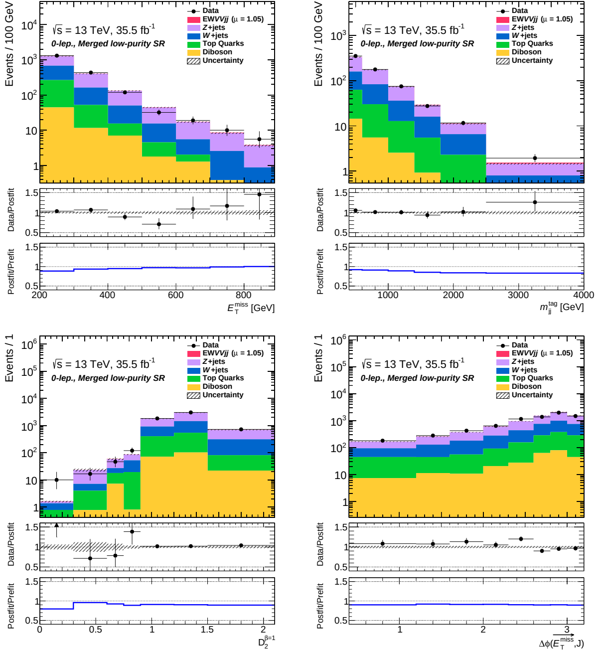
Fig. B.4: Distributions of variables used in the BDT training in the merged low-purity region for the 0-lepton channel applying post-fit uncertainties are shown.
