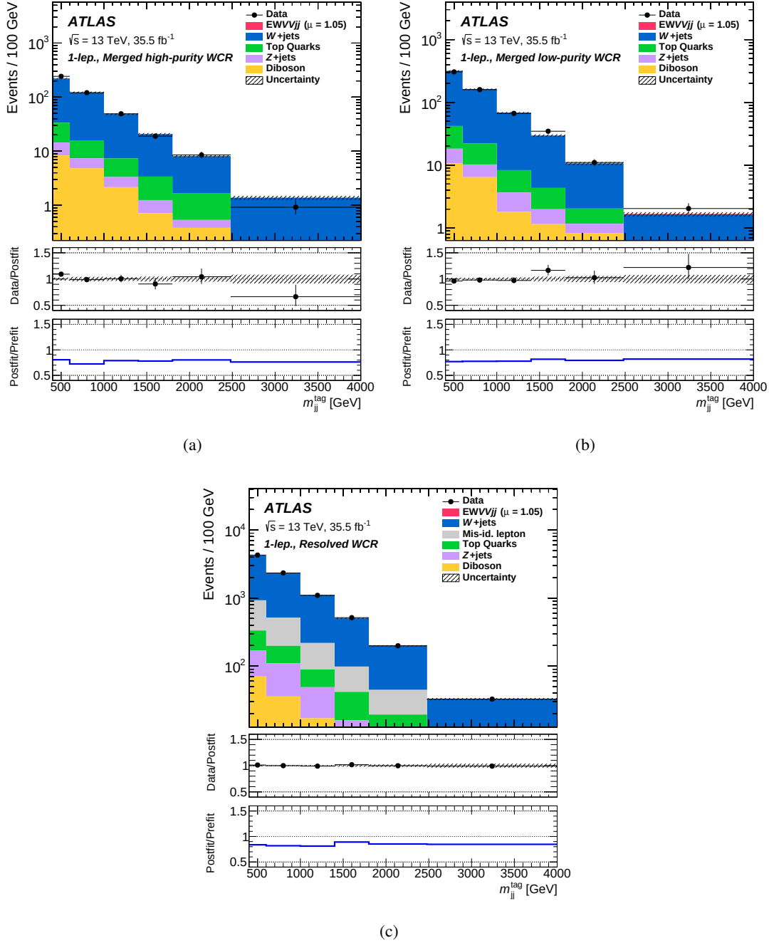
Fig. 6.23: Comparisons of the observed data and expected background distributions of m_{jj}^{\text{tag}} of the W+jets control regions in the 1-lepton channel: (a) high-purity and (b) low-purity merged signal regions; (c) the resolved signal region. The background contributions after the global likelihood fit are shown as filled histograms. The signal is shown as a filled histogram on top of the fitted backgrounds normalized to the signal yield extracted from the observed data ( \mu = 1.05 ), but it is not visible due to its small contribution. The middle pane shows the ratios of the observed data to the post-fit signal and background predictions. The uncertainty in the total prediction, shown as bands, combines statistical and systematic contributions. The bottom pane shows the ratios of the post-fit and pre-fit background predictions.
