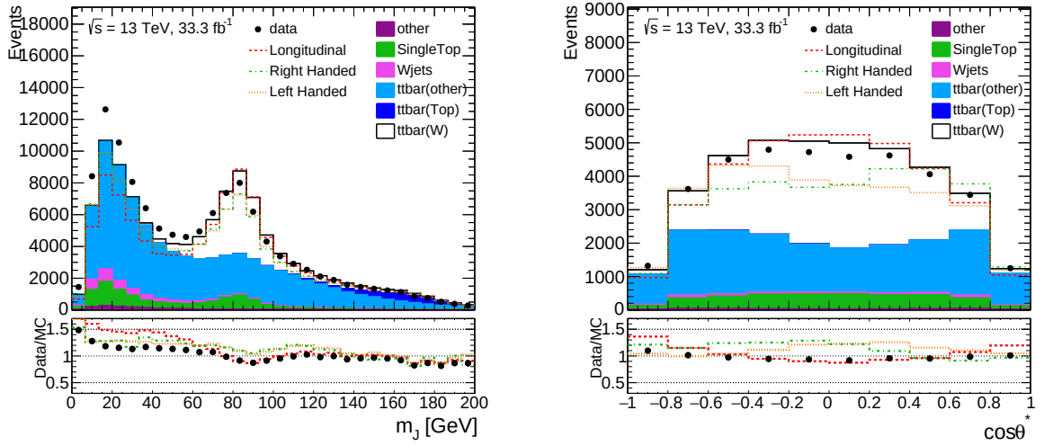
Fig. 9.5: Comparisons between data and MC simulated events for large-R jet mass (left) and \cos\theta^* (right) distributions. The discrepancy at the lower region most likely comes from multi-jets events.
