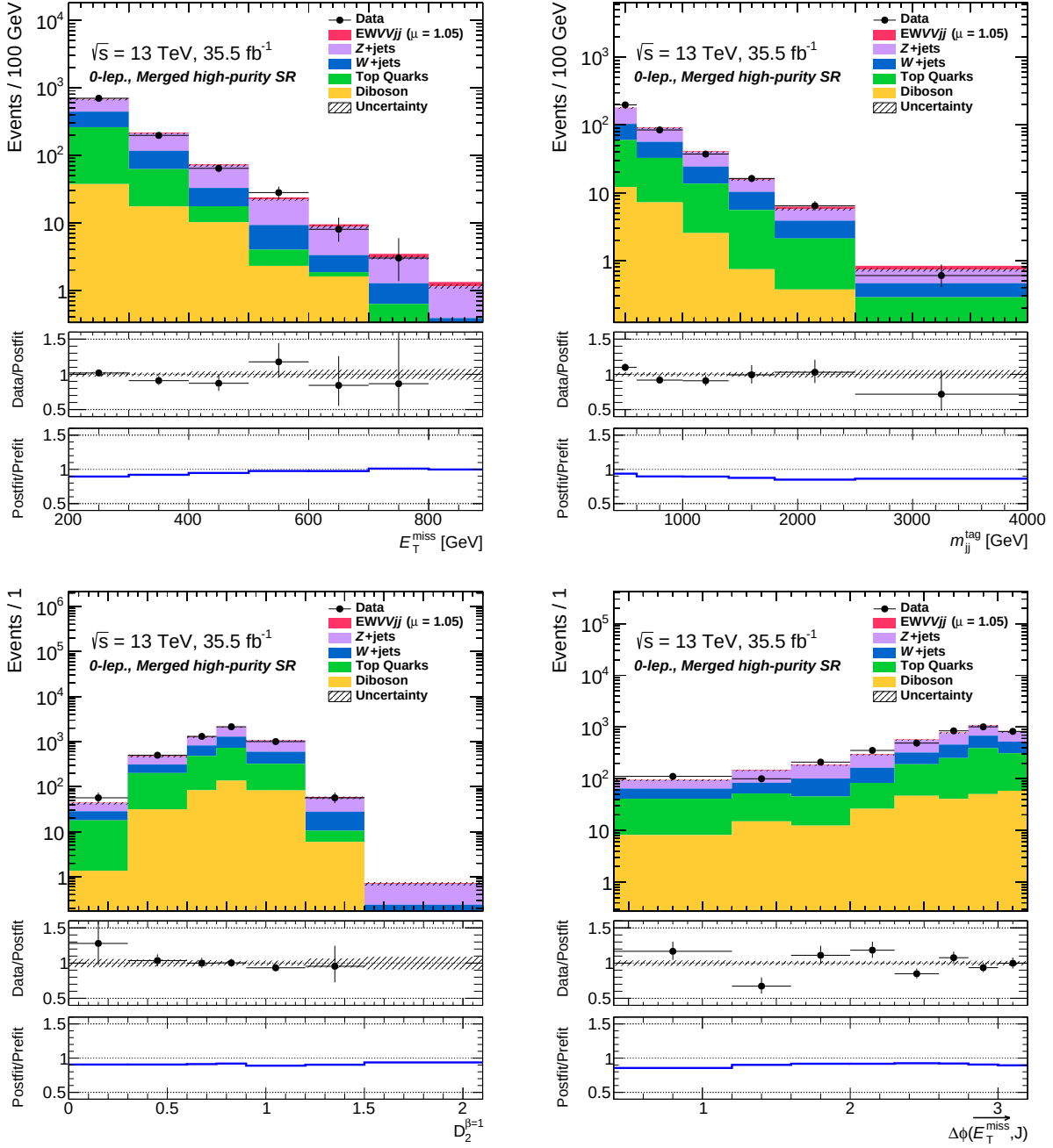
Fig. B.1: Distributions of variables used in the BDT training in the merged high-purity region for the 0-lepton channel applying post-fit uncertainties are shown.
