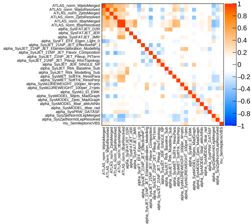
Fig. 6.32: A correlation matrix of nuisance parameters from the fit with the observed data is shown. Only nuisance parameters which are greater than 20% are shown.
