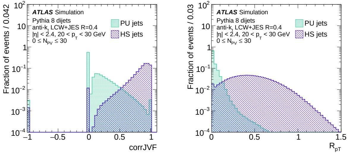
Fig. 4.16: Distributions for corrJVF (left) and R_{pT} (right) are shown [92]. The green filled and blue shaded histograms represent jets from pileup vertices and jets from the primary vertex, respectively.
