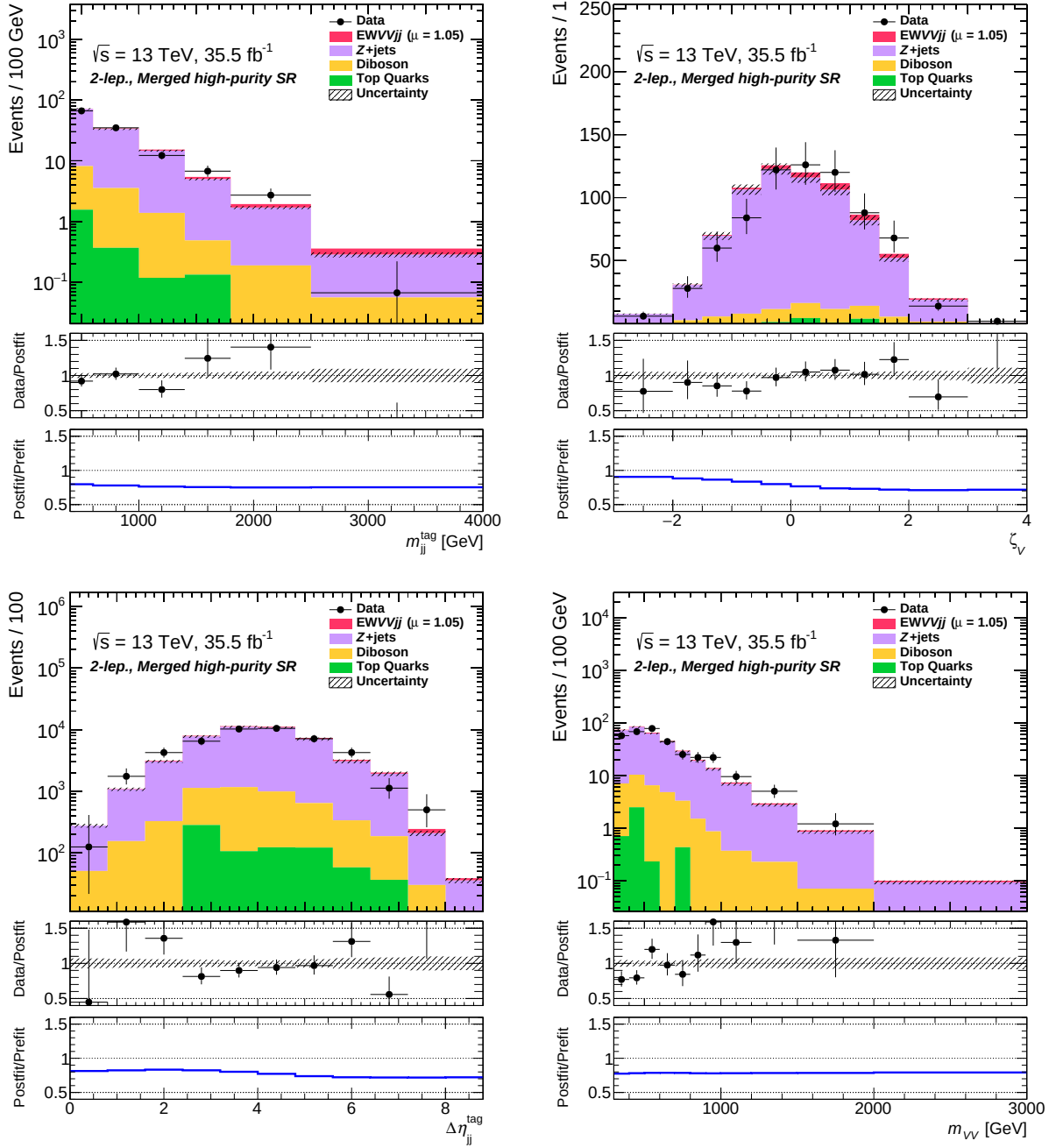
Fig. B.16: Distributions of variables used in the BDT training in the merged high-purity region for the 2-lepton channel applying post-fit uncertainties are shown.
