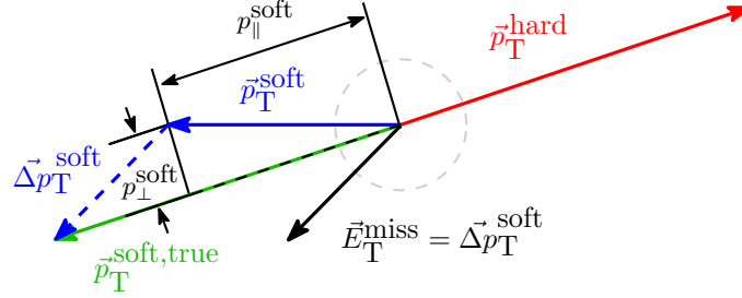
Fig. 4.18: A schematic graph of the TST projection for the calculation of the TST systematic uncertainties is shown [99].
