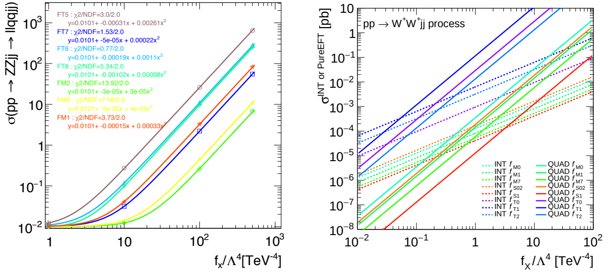
Fig. 7.1: Cross-sections as a function of couplings are shown in the left plot. Markers and liens stand for the calculated cross-sections and obtained parabolic functions, respectively. Cross-sections as a function of couplings for each INT (dashed line) and QUAD (solid line) component are shown in the right plot. Colors indicate sorts of operators.
