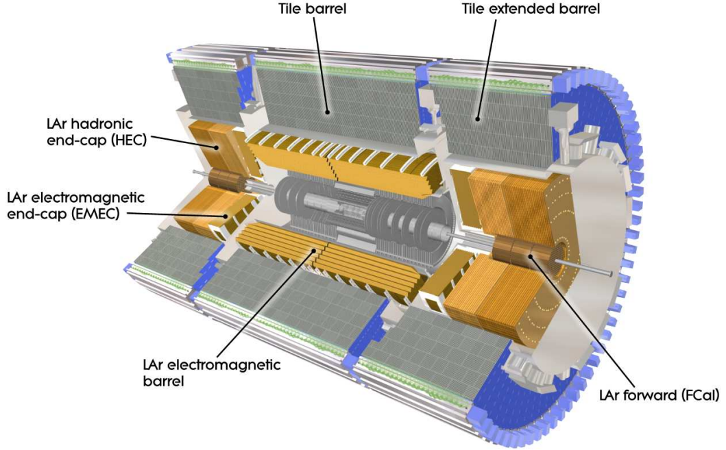
Fig. 3.5: A schematic graph of the calorimeter system taken from Reference [11] is shown. The calorimeter system consists of the LAr electromagnetic barrel, tile barrel, extended barrel, LAr electromagnetic end-cap, LAr hadronic end-cap, and LAr forward at the end-cap regions.
