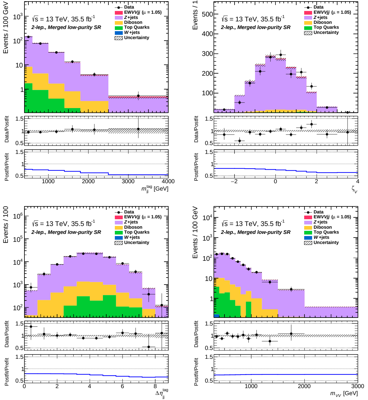
Fig. B.18: Distributions of variables used in the BDT training in the merged low-purity region for the 2-lepton channel applying post-fit uncertainties are shown.
