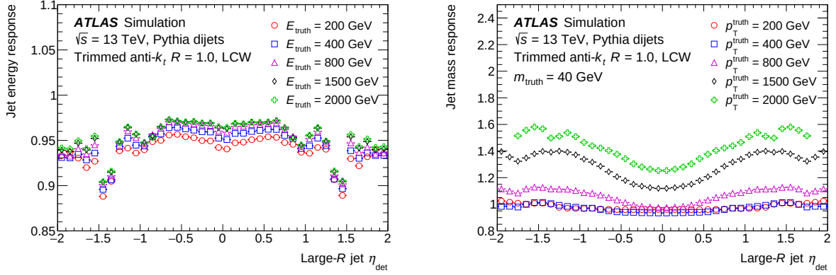
Fig. 5.3: The energy (left) and m (right) calibration factors for large-R jets with respect to \eta are shown [106]. The jet energy response is almost constant with respect to its energy, but explicit deficits observed around jet |\eta| \sim 1.4 because of the transition regions of the calorimeter. The mass response is almost unity at p_T = 200 GeV but it increases in \sim 1.6 at p_T = 2 TeV because gluon radiation increases at higher energy.
