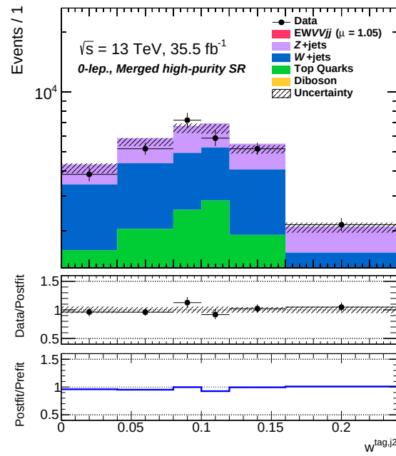
Fig. B.3: A distribution of variable used in the BDT training in the merged high-purity region for the 0-lepton channel applying post-fit uncertainties is shown.
