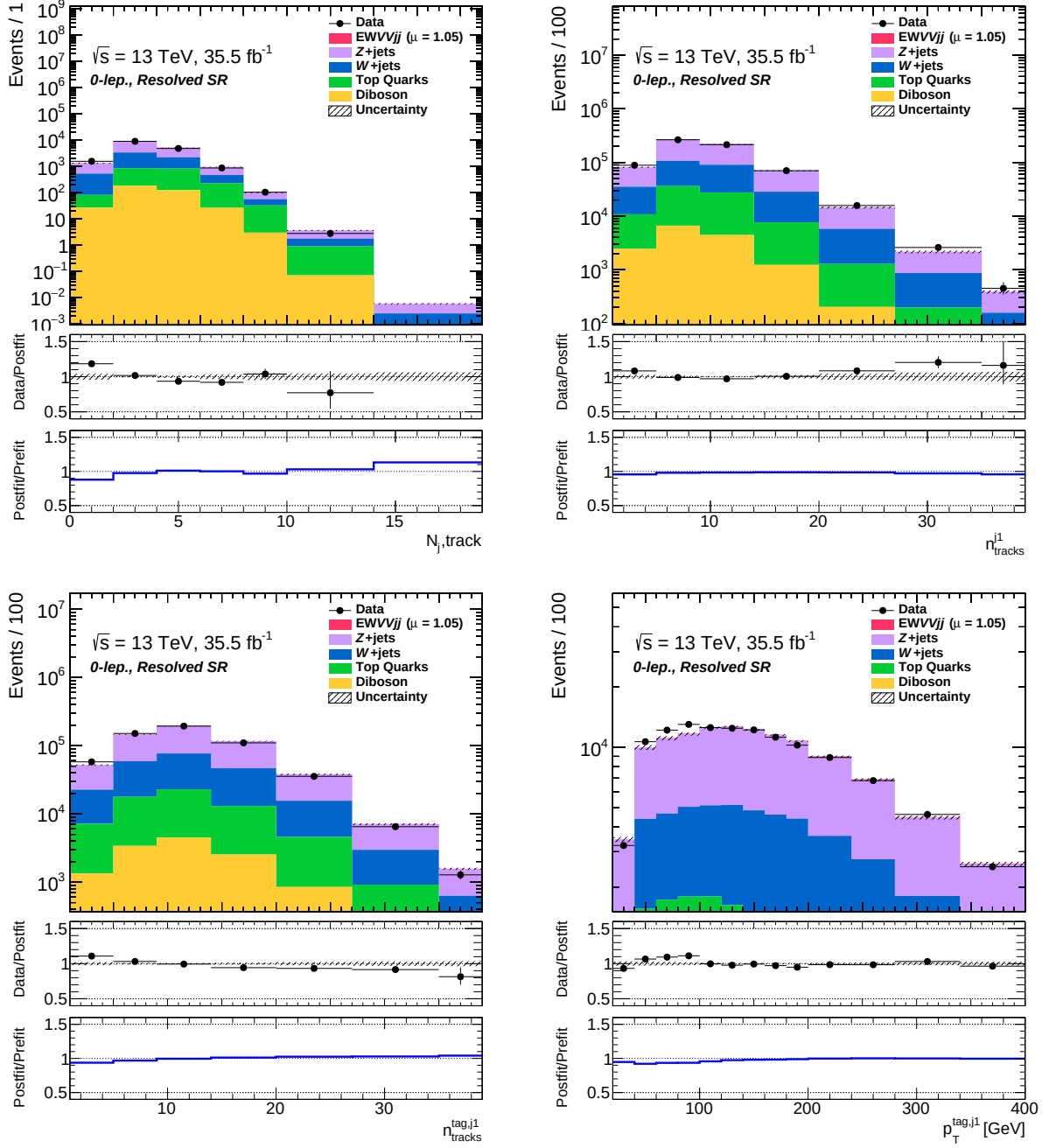
Fig. B.8: Distributions of variables used in the BDT training in the resolved region for the 0-lepton channel applying post-fit uncertainties are shown.
