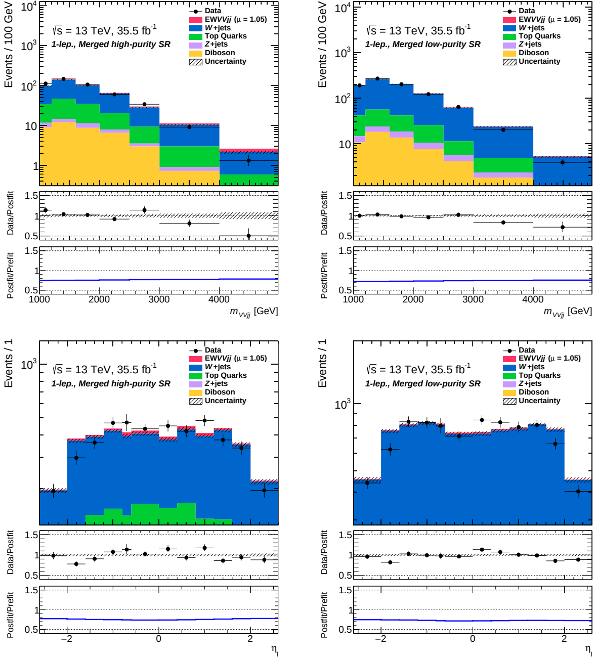
Fig. B.11: Distributions of variables used in the BDT training in the merged region for the 1-lepton channel applying post-fit uncertainties are shown.
