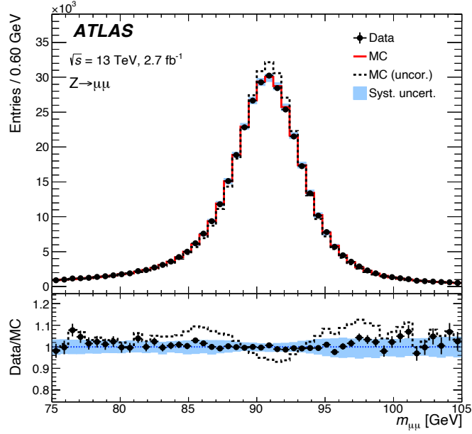
Fig. 4.11: A distribution for the invariant mass of the dimuon system ( m_{\mu\mu} ) with Z \rightarrow \mu^+\mu^- events is shown [86]. A corrected m_{\mu\mu} distribution (red line) describes distribution for the observed data (black dot) much better than an uncorrected m_{\mu\mu} distribution (dashed line).
