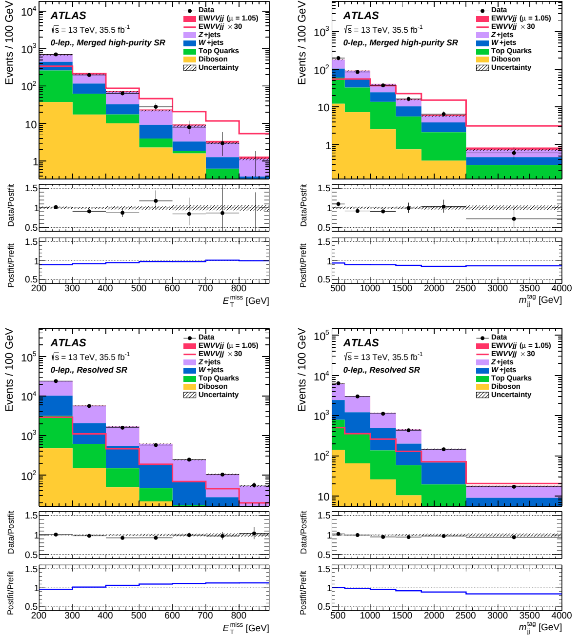
Fig. 6.28: The distributions for E_T^{\text{miss}} (left), m_{jj}^{\text{tag}} (right), in the 0-lepton merged HP (top) and 0-lepton resolved (bottom) signal regions. The background contributions after the likelihood fit are shown as filled histograms. The signal is shown as a filled histogram on top of the fitted backgrounds normalized to the signal yield extracted from the observed data ( \mu = 1.05 ), and unstacked as an unfilled histogram, scaled by the factor of 30. The size of the combined statistical and systematic uncertainty for the sum of the fitted signal and background is indicated by the hatched band. The middle pane shows the ratios of the observed data to the post-fit signal and background predictions. The bottom pane shows the ratios of the post-fit and pre-fit background predictions.
