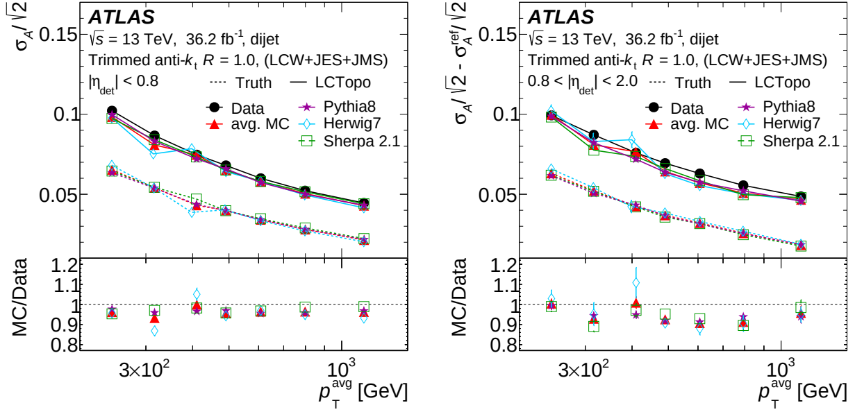
Fig. 5.8: The p_T dependence of \sigma(\mathcal{A}) at |\eta| < 0.8 (left) and |\eta| > 0.8 (right) regions are shown. The values of the observed data are shown in the black dots, the other colors indicate each MC simulation and an average of them. The dashed and solid lines stand for truth and reconstructed jets, respectively.
