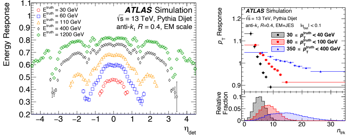
Fig. 4.14: The average energy response as a function of |\eta| for jets with several truth energies (left) and the p_T responses for a n_{\text{trk}} variable in several truth jet energies (right) are shown [90]. For the left plot, the energy responses are better at higher jet energies due to the sampling nature of the calorimeter and worse at the transition region |\eta| \sim 1.5 and |\eta| \sim 3.2 . For the right plot, jets with lower n_{\text{trk}} , i.e. jets contain many neutral particles have higher p_T responses because all of the constituents are calibrated to the EM-scale which is not stringently correct for the neutral hadrons.
