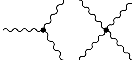
Fig. 2.6: Examples of 6- (left) and 8-dimensional (right) vertices. The wavy line denotes the vector boson field. The dot represents an anomalous gauge coupling.
