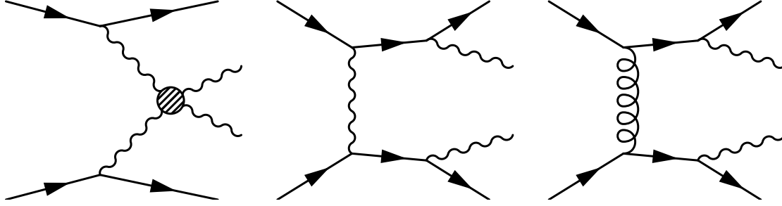
Fig. 6.2: Representative Feynman diagrams of the VBS processes (left), the electroweak productions of the non-VBS processes (center), and the strong productions of the non-VBS processes (right) are shown. The wavy, curled, and straight lines represent W/Z bosons, a gluon, and quarks, respectively. The dashed circle can be replaced with the VBS interactions as shown in Figure 2.1.
