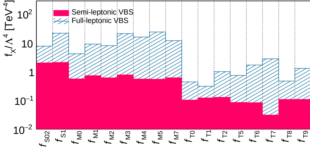
Fig. 7.7: 95% C.L. limits on the coefficient of EFT operators are summarized. The blue shaded histogram is the limits obtained by the full-leptonic VBS analyses [21, 24, 50, 51], the magenta filled histogram is the limits calculated by this study.
