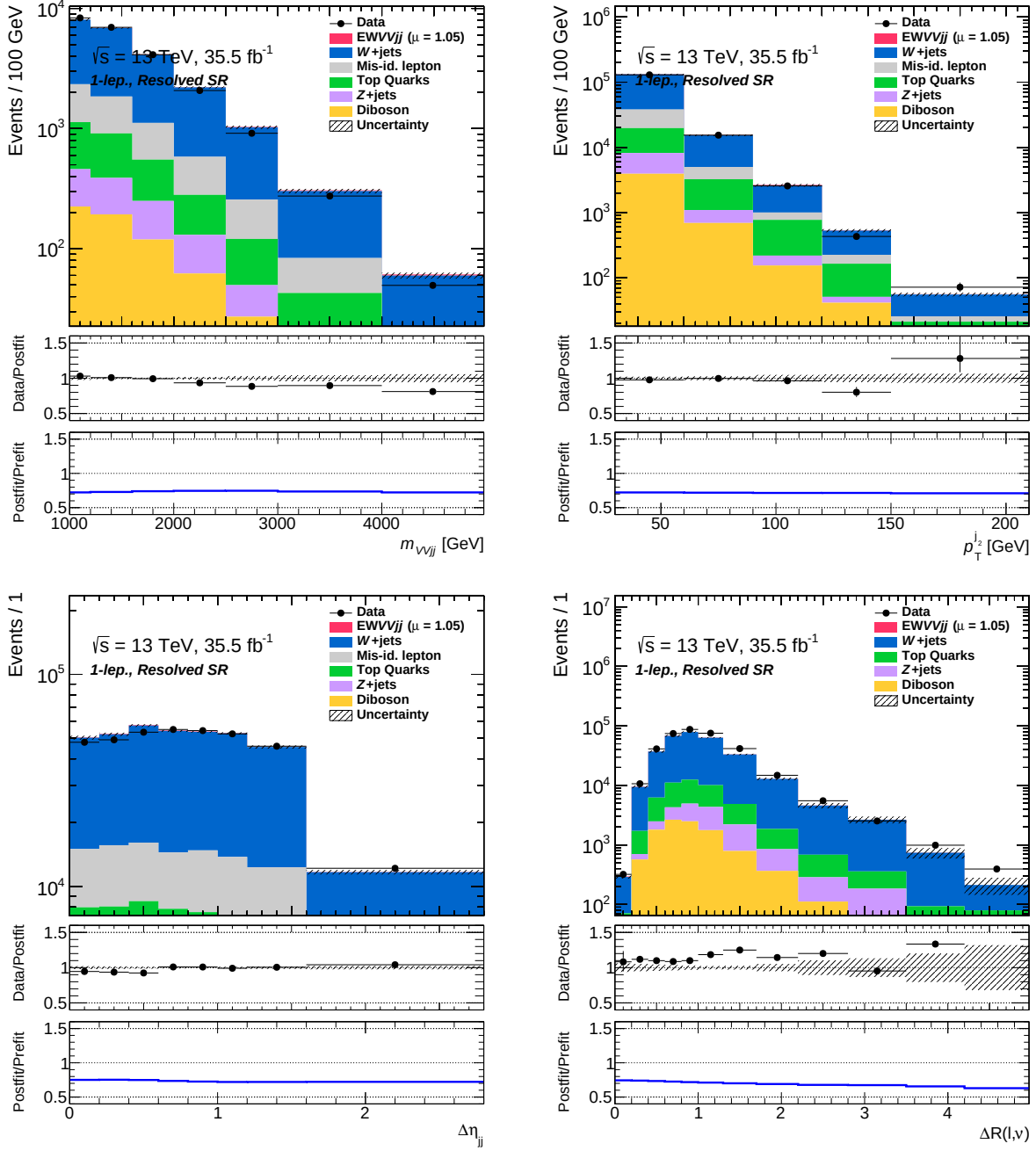
Fig. B.13: Distributions of variables used in the BDT training in the resolved region for the 1-lepton channel applying post-fit uncertainties are shown.
