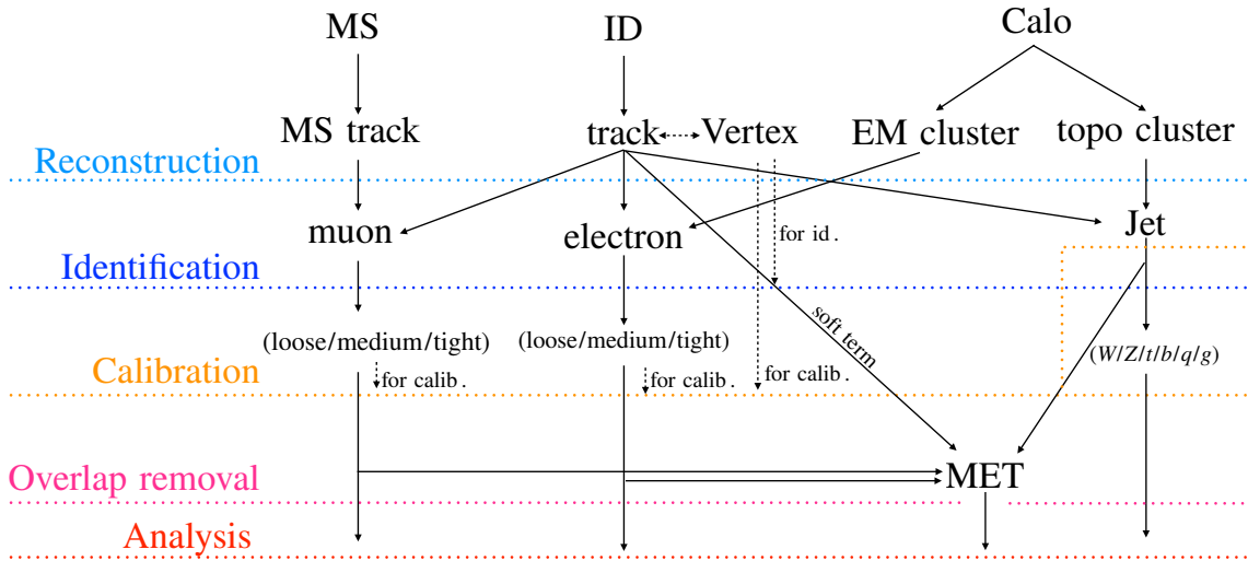
Fig. 4.1: A schematic graph of the workflow for the object reconstruction, identification, calibration, and overlap removal is shown. The ID, MS, and Calo stand for the inner detector, muon spectrometer, and calorimeters, respectively. The reconstruction and identification techniques are briefly introduced in the following sections. A dedicated schematic flow for large-R jets is described in Figure 5.1. The tau leptons and photons are not explicitly drawn in this schematic graph since those are not used in this study.
