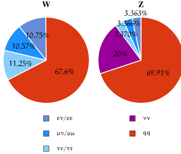
Fig. 2.3: Pie charts representing branching fractions for W (left) and Z (right) boson are shown. Antiparticles are not explicitly shown. q represents u, d, s, c, and b quarks. Values are taken from Reference [36].
