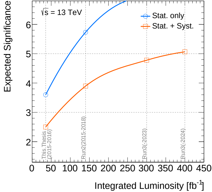
Fig. 9.1: Expected sensitivities with (orange) and without (blue) systematic uncertainties at integrated luminosities of 140,300, and 400 fb -1 are shown.
