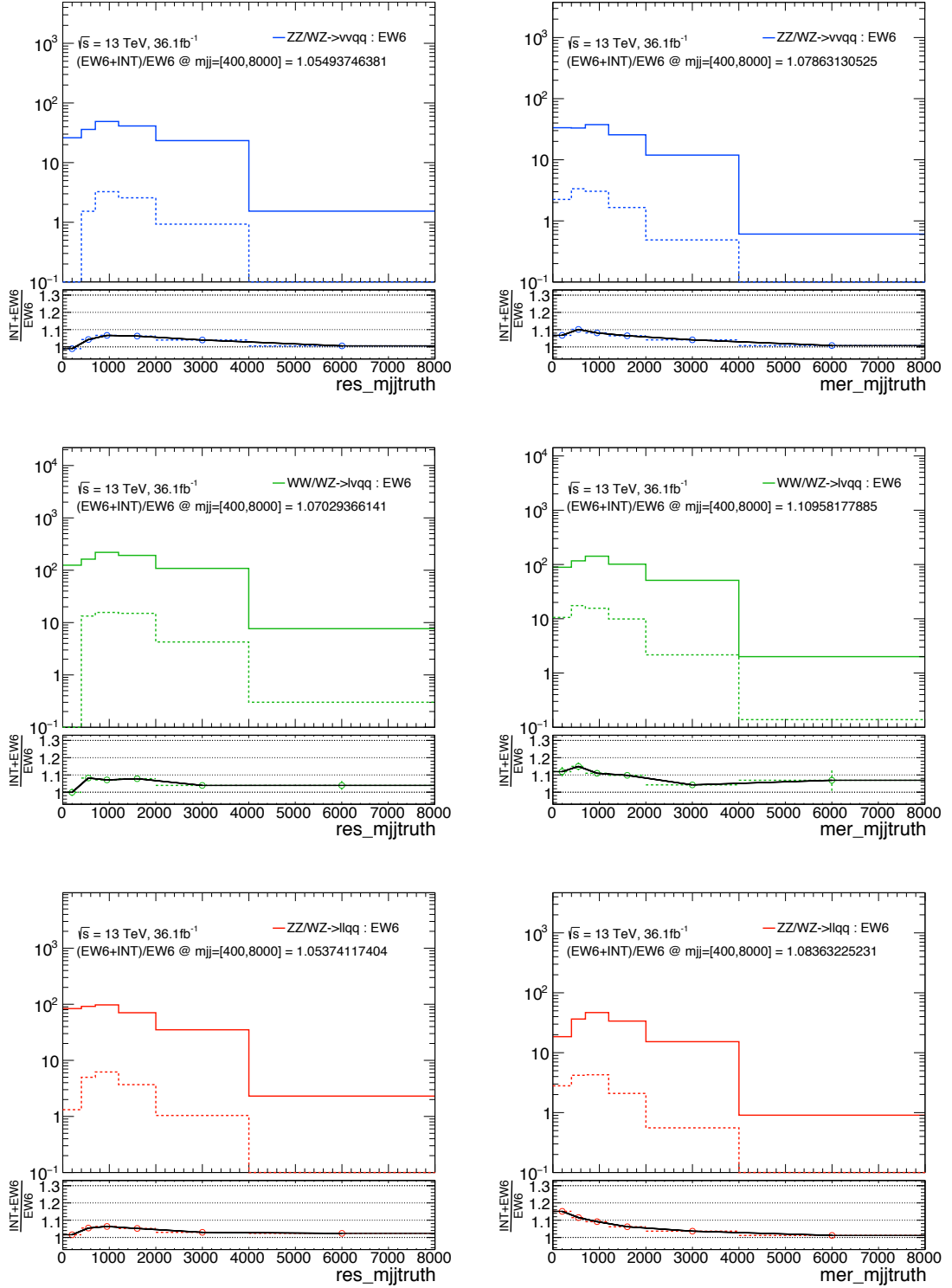
Fig. 6.20: m_{jj}^{\text{tag}} distributions for the EWK process (solid line) and the INT term (dashed line) for the resolved (left), and the merged (right) regions. The first row is for the \nu\nu qq final state, and the second row is for the \ell\nu qq final state, and the third row is for the \ell\ell qq final state. Fiducial event selections as described in Section 6.6 are applied. In the ratio plots beneath, the black line shows the interpolation of (N_{\text{INT}} + N_{\text{EWK}})/N_{\text{EWK}} as a function of m_{jj}^{\text{tag}} .
