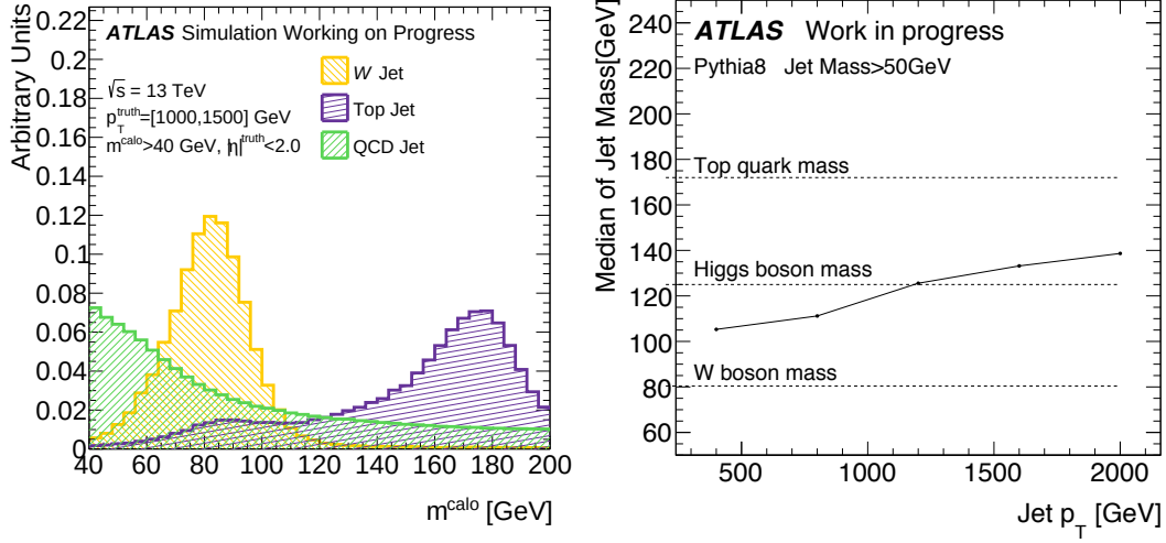
Fig. 2.8: Simulated W/top/q/g jets mass distributions (left) and median of the invariant mass for q/g jets with respect to the jet p_T (right) are shown. The jet masses originated from W bosons and top-quarks are peaked on those pole masses (80 and 170 GeV). The masses of q/g jets peak at low mass but extend to a few hundred GeV, therefore, those fake a massive elementary particle.
