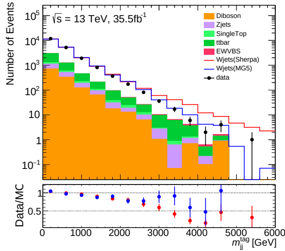
Fig. 6.12: Comparisons of m_{jj}^{\text{tag}} distributions between the observed data and SHERPA2.2.1 or MADGRAPH5_aMC@NLO v2.3.2 at merged WCR region except for the m_{jj}^{\text{tag}} cut. The prediction of MADGRAPH5_aMC@NLO performs better modeling than that of SHERPA2.2.1, however, it have been generated much fewer statistics in timescale of this analysis, SHERPA2.2.1 has been chosen as the nominal sample.
