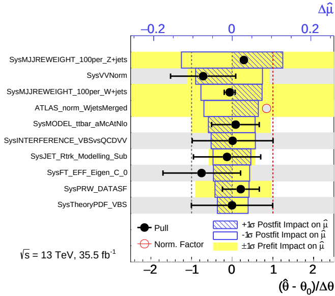
Fig. 6.33: Pre-fit (yellow) and post-fit (blue) nuisance parameter impacts on the signal-strengths are shown. The impacts are ranked by the order of \Delta\hat{\mu} = \hat{\mu}_X - \hat{\mu}_0 , where \hat{\mu}_0 is a signal-strength obtained by the nominal fit, and \hat{\mu}_X is a signal-strength obtained by a fit fixing the nuisance parameter X on plus or minus 1\sigma . The black and red dots denote pulls and normalization factors. The naming convention is summarized in Appendix D.
