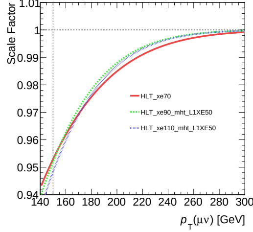
Fig. 6.5: The trigger scale factors for the E_T^{\text{miss}} triggers used in this analysis are shown. The E_T^{\text{miss}} trigger are used above p_T(\mu\nu) = 150 GeV (vertical dashed line).
