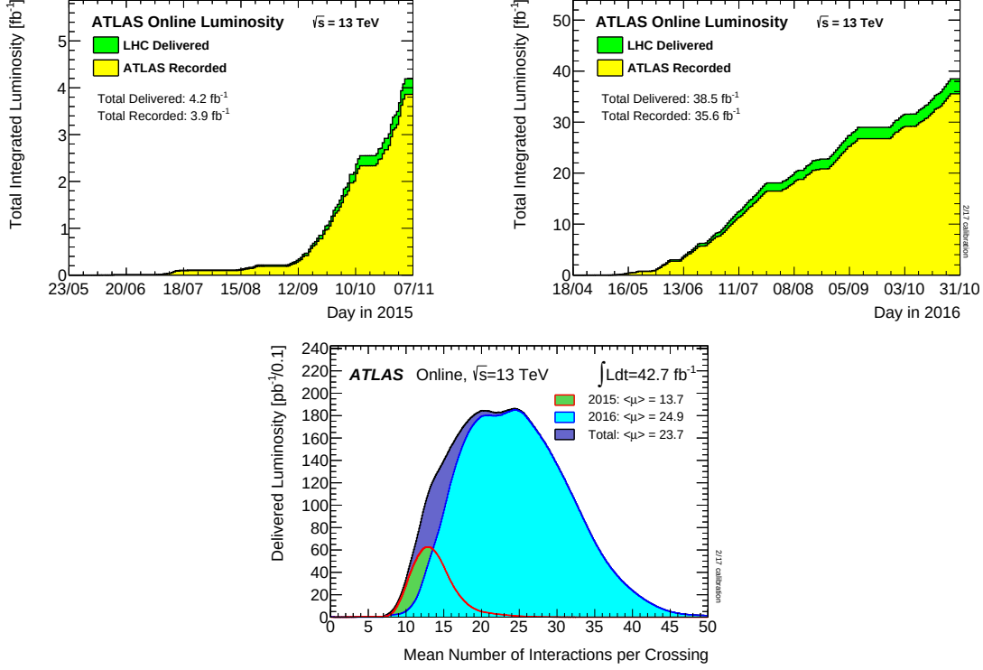
Fig. 6.4: Accumulated integrated luminosity plots for the years of 2015 (left) and 2016 (right) are shown. The green and yellow histograms are corresponding to the LHC delivered luminosity and ATLAS recorded luminosity. In the bottom plot, distributions for the number of interactions per crossing in runs for 2015 (green), 2016 (light blue), and its total (deep blue) are shown.
