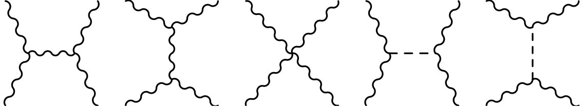
Fig. 2.1: The leading order Feynman diagrams of VBS are shown. From the left, those correspond to \mathcal{M}_1 , \mathcal{M}_2 , \mathcal{M}_3 , \mathcal{M}_4 , and \mathcal{M}_5 of Equation 2.8. The wavy and dashed lines represent the vector boson fields and Higgs fields, respectively.
