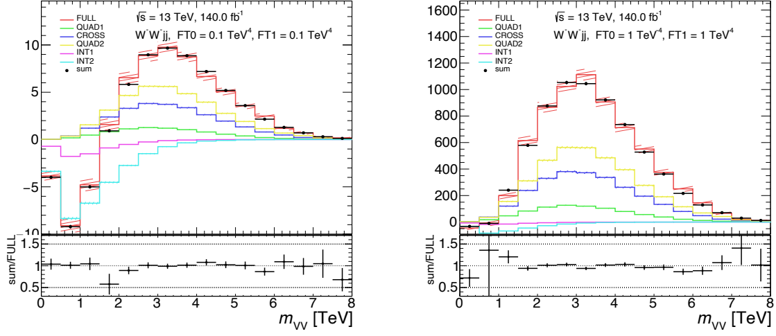
Fig. 7.2: m_{VV} distributions for L_{T0} quadratic term (QUAD1: green), L_{T1} quadratic term (QUAD2: yellow), L_{T0} interference term (INT1: magenta), L_{T1} interference term (INT2: cyan), those cross term (CROSS: blue), and simulating all of them at the same time (sum: black) with coefficient values of f_{T0}/\Lambda^4 = 0.1 TeV ^{-4} and f_{T1}/\Lambda^4 = 0.1 TeV ^{-4} (left) and coefficient values of f_{T0}/\Lambda^4 = 1 TeV ^{-4} and f_{T1}/\Lambda^4 = 1 TeV ^{-4} (right). To check whether the decomposition to five elements works well, generation with a full contribution (FULL: red) is compared to a sum of five elements (sum: black dot). the bottom plots show the ratios of the sum to FULL.
