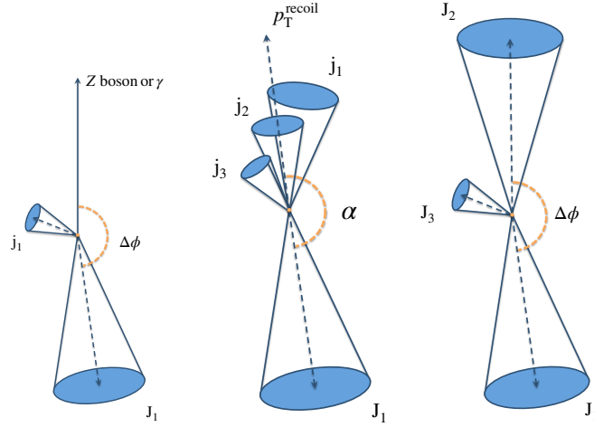
Fig. 5.4: Cartoons of topologies for Z/\gamma +jets (left), multijet (central), and dijet (right) are shown [106]. The capital j ( J ) and small j ( j ) denote a large- R jet and a small- R jet, respectively. The subscripts express the order of p_T . The \Delta\phi or \alpha is an angle between a large- R jet and recoil objects, Z , \gamma , the vector sum of small- R jets, or a large- R jet.
