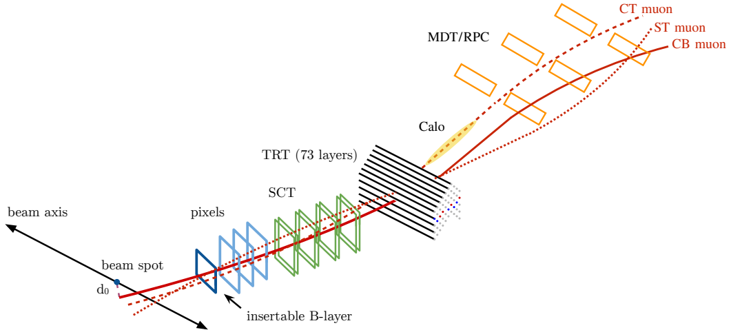
Fig. 4.9: A schematic illustration of muon paths (red lines) through detectors at the central region [77]. A muon goes through four pixel layers, four SCT layers, and several TRT drift tubes. A CB muon leaves hits on three MDT layers. A ST muon leaves hits on MDT layers. A CT muon goes through the crack region of the MS ( |\eta| < 0.1 ) but tagged by calorimeter energy deposits.
