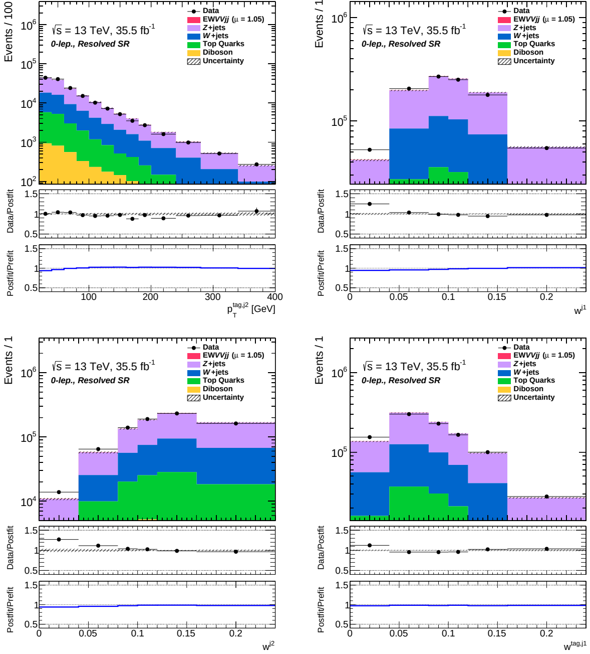
Fig. B.9: Distributions of variables used in the BDT training in the resolved region for the 0-lepton channel applying post-fit uncertainties are shown.
