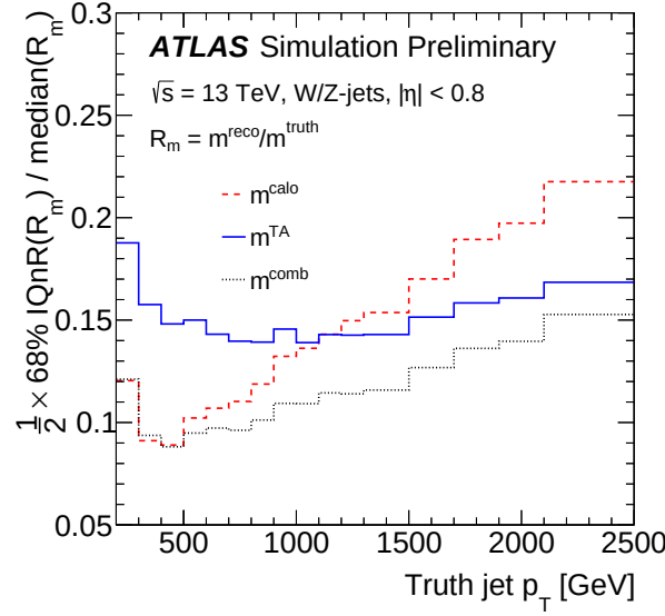
Fig. 5.14: The mass resolution for a calorimeter jet ( m^{\text{calo}} ), a track assisted mass ( m^{\text{TA}} ), and a combined mass ( m^{\text{comb}} ) are shown. The resolution (y-axis) is defined with the median of a mass response ( R_m = m^{\text{reco}}/m^{\text{truth}} ) and the 68% inter quantile range (IQnR). The m^{\text{calo}} has better mass resolution below p_T = 1 TeV, whereas m^{\text{TA}} has better resolution at above p_T = 1 TeV. The m^{\text{comb}} has the same or a better resolution than m^{\text{calo}} at the whole p_T range except a few bins at low p_T . This reverse feature is because R_m does not perfectly behave as Gaussian, and then the linear combination becomes a non-ideal combination.
