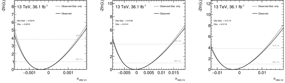
Fig. 7.5: Log-likelihood curves for L_{S0} (left), L_{M0} (center), and L_{T0} (right) are shown. The dashed curve only includes statistical uncertainty, the solid curve includes both the statistical and systematic uncertainties. Since no excess over the SM prediction is observed, curves have local minimum at \mu_{VBS\ VV} \sim 0 ( \mu_{VBS\ VV} stands for signal-strength for each operator). Horizontal dashed lines guide for the confidence limits based on the \chi^2 distribution with two degrees of freedom.
