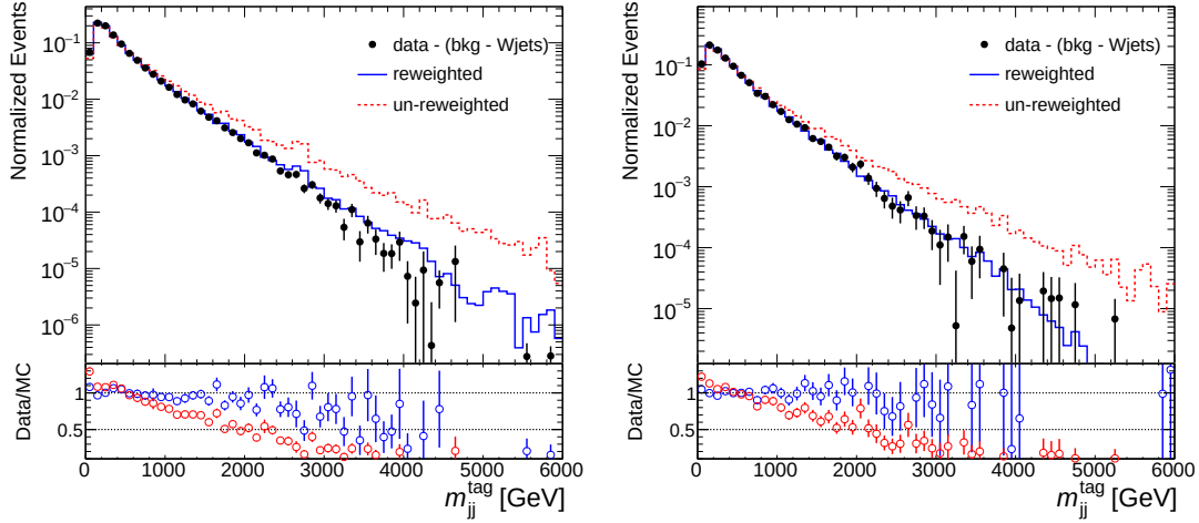
Fig. 6.15: The m_{jj}^{\text{tag}} distributions before and after m_{jj}^{\text{tag}} reweighting for the resolved WCR (left) and merged WCR (right) are shown. The histograms for the observed data are subtracted by distributions for the MC simulations other than the W +jets sample.
