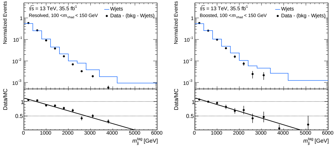
Fig. 6.13: Fits of m_{jj}^{\text{tag}} slope at a particular m_{\text{Vhad}} bin of the resolved (left) and merged (right) WCR are shown.
