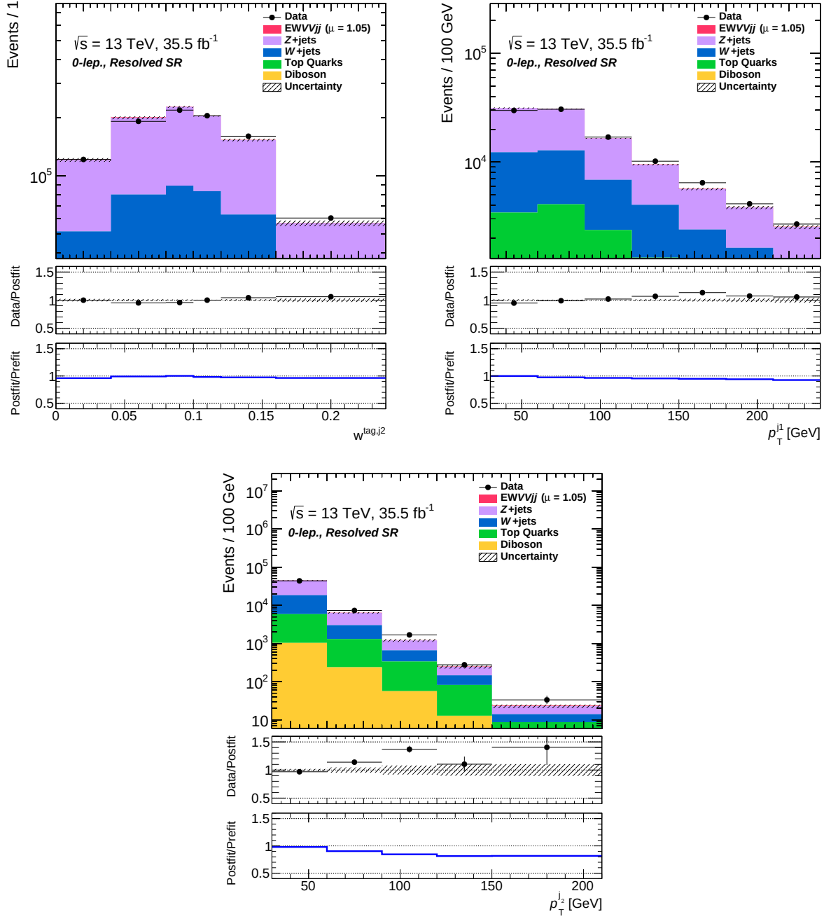
Fig. B.10: Distributions of variables used in the BDT training in the resolved region for the 0-lepton channel applying post-fit uncertainties are shown.)
