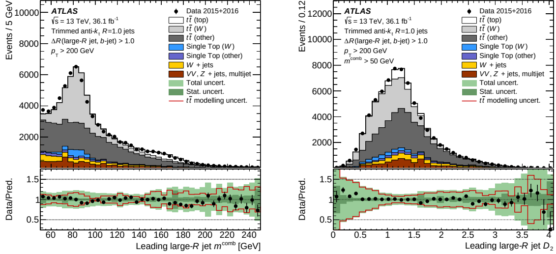
Fig. 5.15: Comparisons between the observed data and MC simulations for large-R jets mass (left) and D_2 (right) in t\bar{t} enhanced region are shown. The dominant systematic uncertainty is theoretical uncertainties for t\bar{t} shape [107].
