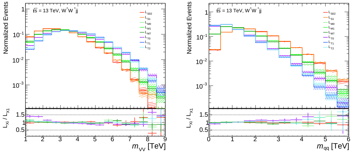
Fig. 7.3: Invariant masses of a diboson pair (left) and invariant mass of a spectator quark pair (right) shapes for different operators are shown. Red-ish, green-ish, and blue-ish colors represent L_S , L_M , and L_T operators, respectively. Histograms only include events for QUAD terms.
