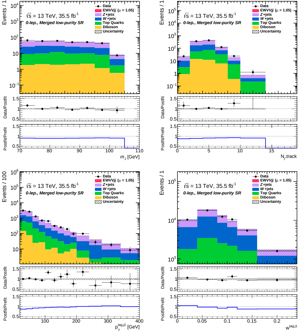
Fig. B.5: Distributions of variables used in the BDT training in the merged low-purity region for the 0-lepton channel applying post-fit uncertainties are shown.
