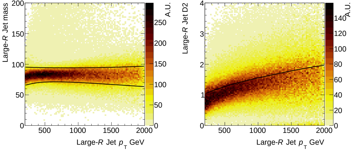
Fig. 5.16: A W jet population on the p_T and mass space (left) and the p_T and D_2 space (right) are shown. The black lines stand for 50% working point thresholds.
