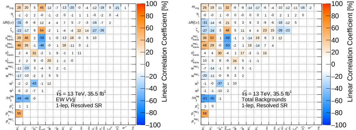
Fig. C.3: Linear correlation coefficients between input variables for signal EWVj events (left) and sum of background events (right) at the 1-lepton resolved SR. 100% (-100%) means completely correlated (anti-correlated).
