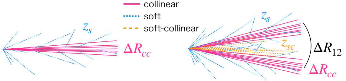
Fig. 2.9: Schematic graphs of 1-prong jet (left) and 2-prong jet (right) are shown. The 1-prong jet consists of collinear emissions (magenta) and soft radiations (cyan). The 2-prong jet consists of two subjets that having collinear emissions (magenta) and soft radiation (cyan), and soft-collinear emission from the dipole formed by two subjets (orange).
