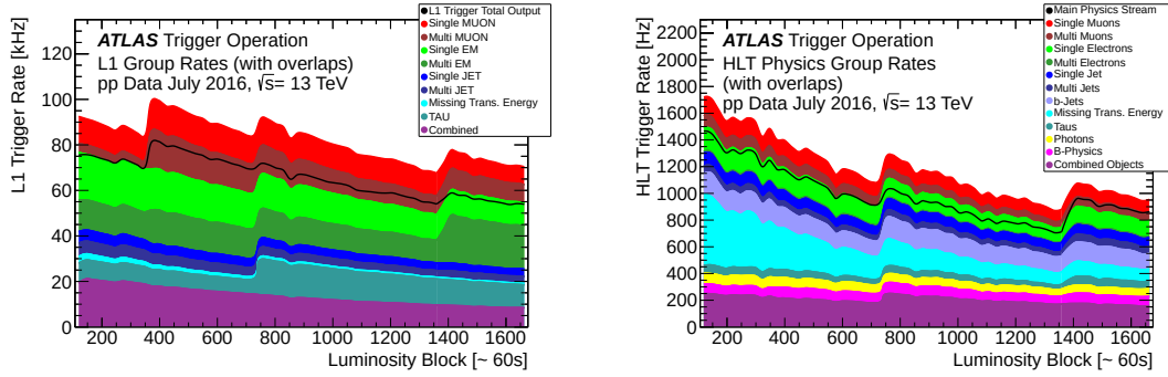
Fig. 3.10: A trigger rate decomposition for each the L1 (left) and HLT (right) in a data taking in July 2016 with a peak instantaneous luminosity of 1.2 \times 10^{34} \text{ cm}^{-2}\text{s}^{-1} are shown [70]. The x-axis corresponds to a running time since the collisions started. Due to the trigger multi-firing in an event, the total output rate (black) is less than the sum of the individual trigger rate. Generally, a trigger rate decreases with respect to a running time because of proton losses, but it increases several times in a run because of redefinitions of prescale factors.
