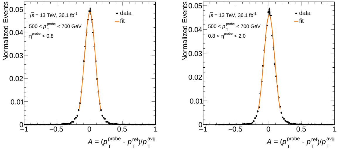
Fig. 5.7: The distribution of \mathcal{A} at |\eta| < 0.8 (left) and |\eta| > 0.8 (right) regions are shown. The results of fits (orange line) show good agreements with distributions for the observed data (black dots) avoiding non-Gaussian tails.
