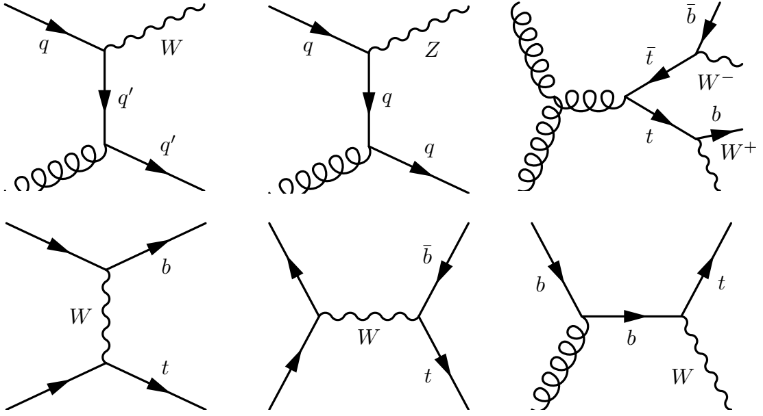
Fig. 6.3: Feynman diagrams of W +jets (top left), Z +jets (top center), t\bar{t} (top right), single top produced via t -channel (bottom left), s -channel (bottom center), and t -channel in association with a W boson (bottom right) are shown.
