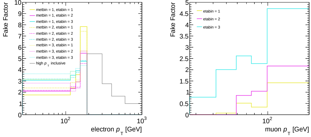
Fig. 6.18: Fake factors for the electron (left) and muon (right) channels. The bin numbers correspond to the binning defined in Table 6.14 by the ascending order.
