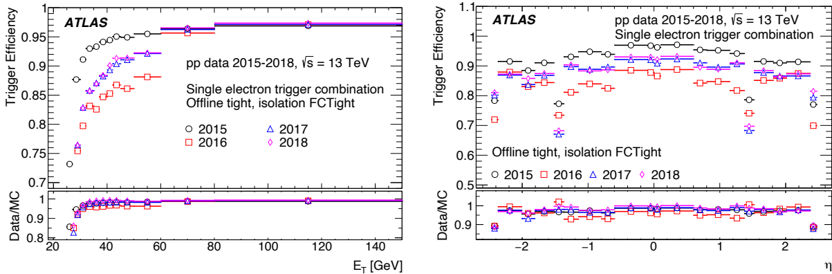
Fig. 4.8: Electron trigger efficiencies for each year as a function of p_T (left) and \eta are shown [84]. Three triggers shown in Table 4.2 for each year are combined by the logical “OR”. The efficiencies are given with respect to offline electrons required to be the tight identification and the “FixedCutTight” isolation. The bottom panel shows the ratio of the observed data to MC simulation efficiencies.
