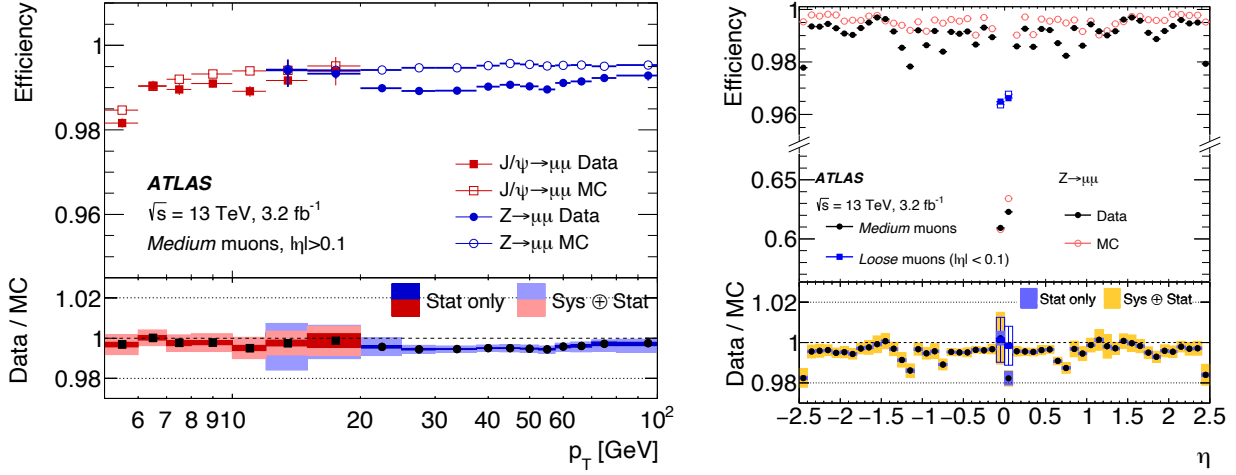
Fig. 4.10: Muon reconstruction efficiencies for p_{\text{T}} (left) and \eta (right) measured in Z \rightarrow \mu\mu and J/\Psi \rightarrow \mu\mu events are shown [86]. The efficiencies are shown as the product of a reconstruction efficiency and a “Medium” or “Loose” identification efficiency. The measured efficiencies from different sources, Z \rightarrow \mu\mu and J/\Psi \rightarrow \mu\mu events are consistent at overlap regions (10 – 20 GeV). The efficiencies are around 99% at most of the p_{\text{T}} ranges. The huge efficiency loss of “Medium” muons at the crack region ( |\eta| < 0.1 ) is recovered by CT (calorimeter tagged) muon shown as “Loose” muons.
