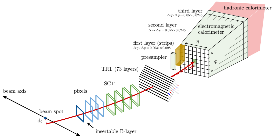
Fig. 4.2: A schematic graph of an electron path (red line) through detectors is shown [77]. An electron goes through four pixel layers, four SCT layers, and several TRT drift tubes. It makes then an electromagnetic shower in the electromagnetic calorimeter. The dashed red line denotes a radiated photon produced at TRT material.
