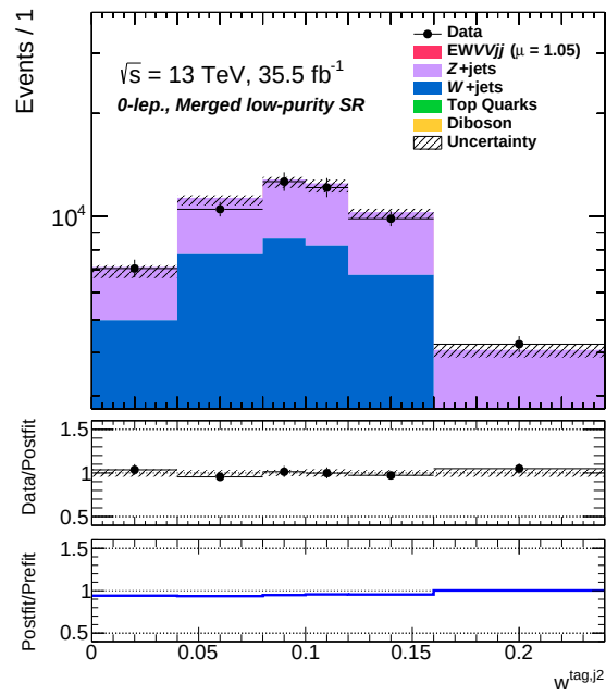
Fig. B.6: A distribution of variable used in the BDT training in the merged low-purity region for the 0-lepton channel applying post-fit uncertainties is shown.
