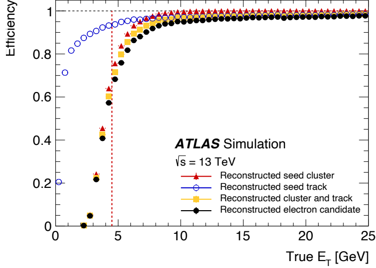
Fig. 4.3: The electron reconstruction efficiencies as a function of transverse energy ( E_T ) of a truth electron are shown [77]. The total reconstruction efficiency of electrons is less than 60% below 4.5 GeV (dashed line). Inefficiencies are coming from the seed-cluster reconstruction at low E_T regions and the track reconstruction at high E_T regions.
