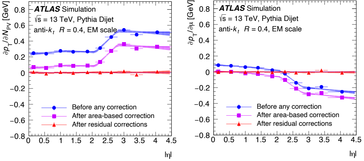
Fig. 4.13: Dependences of small-R jet p_T on N_{PV} (left) and \mu (right) with respect to small-R jet |\eta| are shown [90]. The flat distributions of the red points representing dependence after applying the correction indicate that the pileup dependencies are almost perfectly removed on average.
