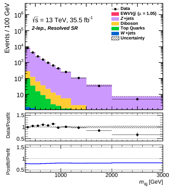
Fig. B.23: A distribution of variable used in the BDT training in the resolved region for the 2-lepton channel applying post-fit uncertainties are shown.
