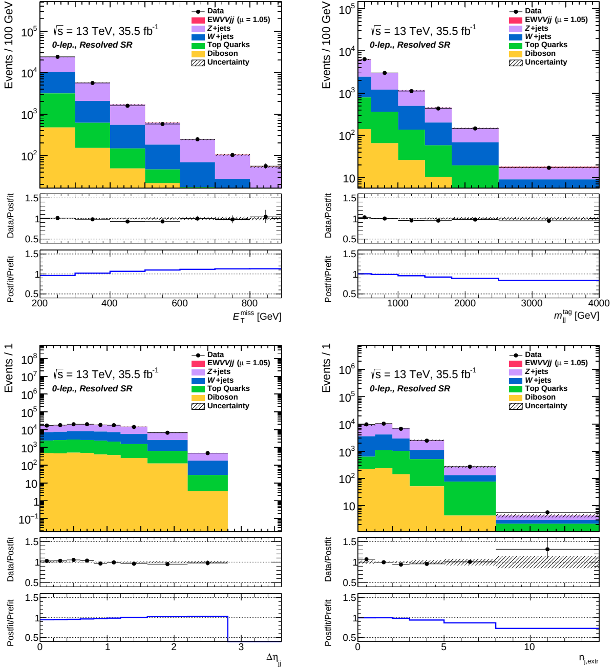
Fig. B.7: Distributions of variables used in the BDT training in the resolved region for the 0-lepton channel applying post-fit uncertainties are shown.
