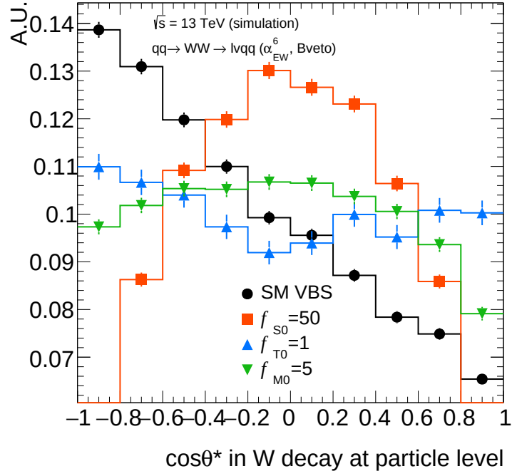
Fig. 7.4: Distributions for the angle between a decay product and original W momentum at the W rest frame ( \cos \theta^* ) for the WW \rightarrow lvqq processes. The red, blue, and green lines show f_{S0}/\Lambda^4 = 50 \text{ TeV}^{-4} , f_{T0}/\Lambda^4 = 1 \text{ TeV}^{-4} , and f_{M0}/\Lambda^4 = 5 \text{ TeV}^{-4} , respectively. In principle, \cos \theta^* for longitudinally polarized vector bosons follow 1 - \cos^2 \theta^* , whereas \cos \theta^* for transversely polarized vector bosons follow (1 \pm \cos \theta^*)^2 , so this plot indicates that the L_{S0} operator tends to generate longitudinally polarized vector bosons, the L_{T0} operator tends to generate transversely polarized vector bosons (equal contributions from left- and right-hand polarization), and the L_{M0} is in between those.
