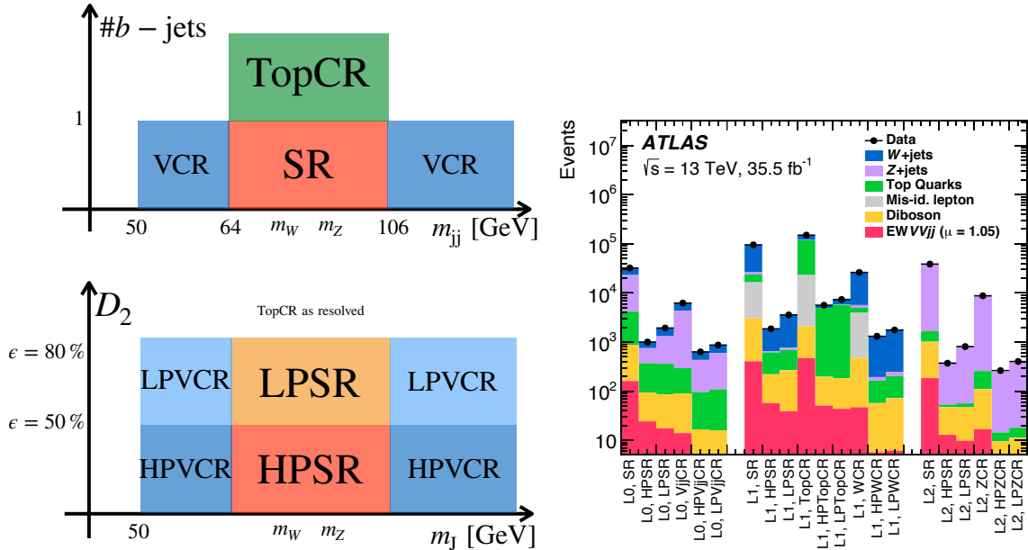
Fig. 6.8: A schematic diagram of SR/CR definitions for resolved (top left) and merged (bottom left) are shown. A plot for event yields in each signal and control region (right) is shown. The labels L0, L1, and L2 stand for the 0-, 1-, and 2-lepton channels, respectively. The labels ‘HP SR’, ‘LP SR’, and ‘SR’ stand for the high-purity merged, low-purity merged, and resolved signal regions, respectively.
