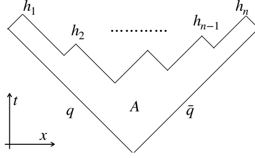
Fig. 2.7: A schematic graph of q\bar{q} string in space-time is shown. The h_n represents resultant hadrons by the hadronization. The swept out area is referred to as A .
