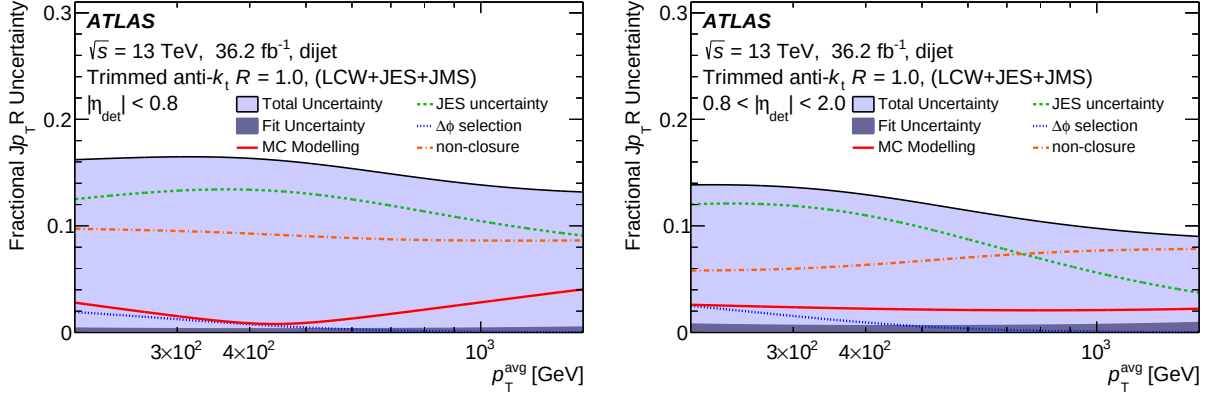
Fig. 5.10: The p_T dependence of uncertainty in jet p_T resolution at |\eta| < 0.8 (left) and |\eta| > 0.8 (right). An interpolation with a filter using a sliding Gaussian kernel is applied to all of the uncertainty dependencies with respect to large-R jets p_T .
