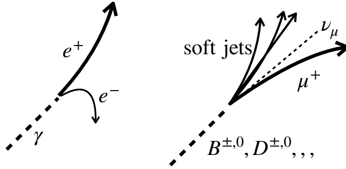
Fig. 6.17: . A schematic diagram of a representative electron fake is shown in the left. Asymmetric decay of \gamma cannot be reduced by the electron isolation cut, hence it can fake an electron. A schematic diagram of a representative muon fake is shown in the right. B and D mesons that produced from b- and c-quarks arising from the fragmentation can decay leptonically. This is the main source of \mu fakes.
