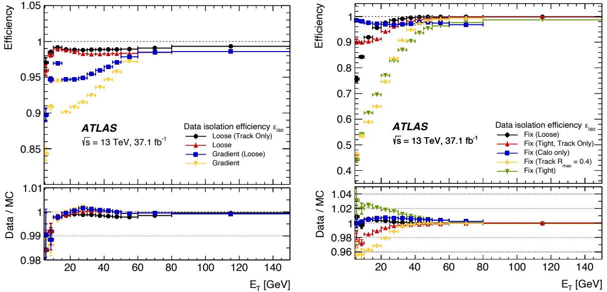
Fig. 4.6: Electron isolation efficiencies for E_T measured in the observed data with Z \rightarrow ee events [77]. The left and right plots show different working points. The Loose (Track Only) and Fix (Tight) isolation criteria are used in this analysis for the additional electron veto and the reconstructions of leptonically decaying W/Z boson, respectively.
