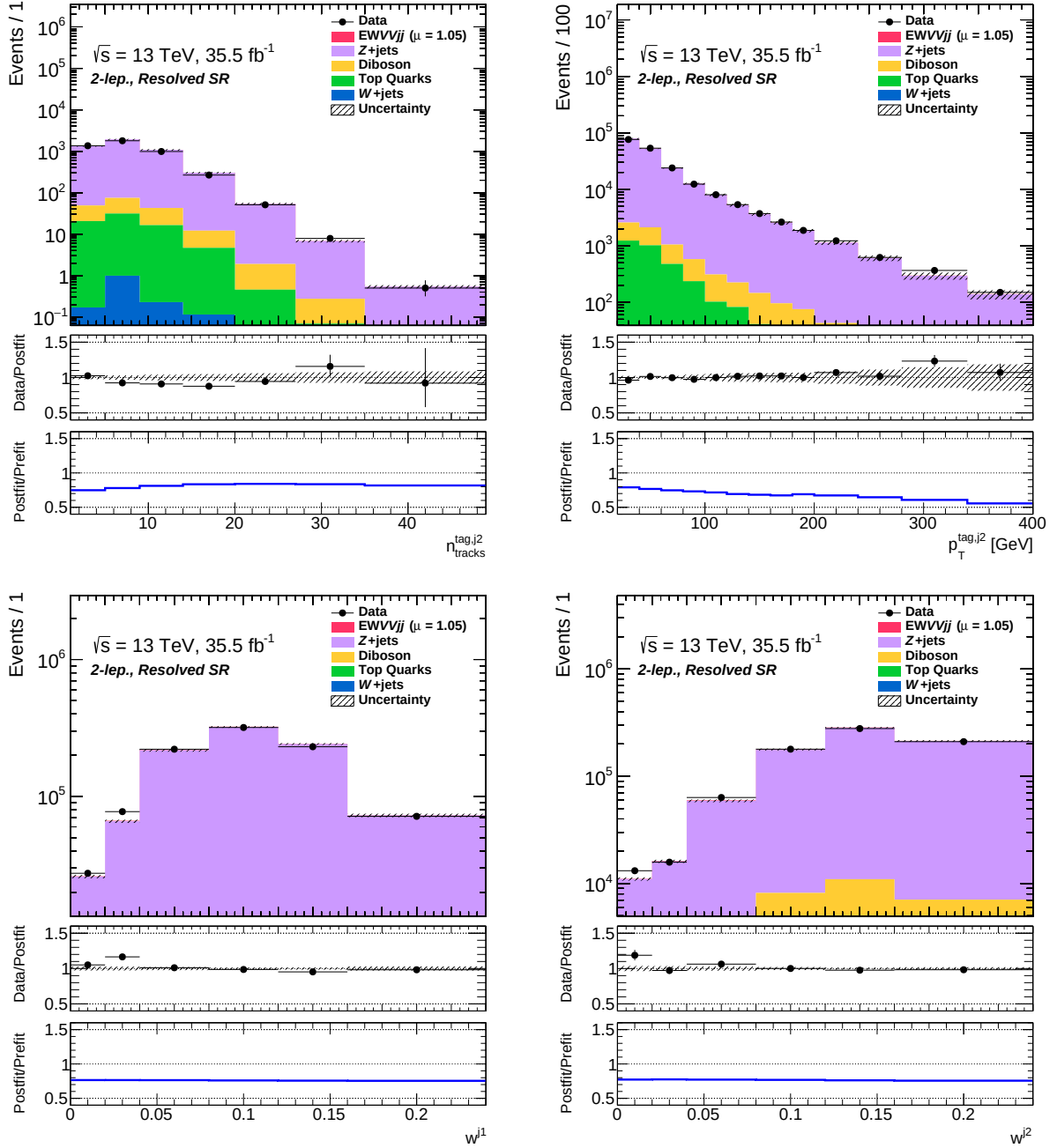
Fig. B.20: Distributions of variables used in the BDT training in the resolved region for the 2-lepton channel applying post-fit uncertainties are shown.
