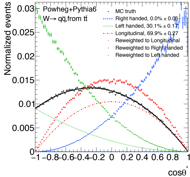
Fig. 9.2: \cos \theta^* distributions for tree-level quarks from W boson decay are shown. The black marker shows the SM prediction by the POWHEG event generator. The black line is the best fit function obtained by a 3-components( fr_0 , fr_R , and fr_L ) fit. The red, green, and blue makers represent \cos \theta^* distributions after reweighting to each pure polarization state.
