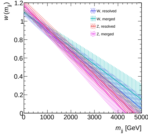
Fig. 6.16: m_{jj}^{\text{tag}} correction weights as a function of m_{jj}^{\text{tag}} for the W +jets and Z +jets processes in the merged and resolved regions are shown. The uncertainty band includes only the statistical uncertainty determined from the fit. For the illustration, the uncertainties in a pair of parameters are correlated 100% positively.
