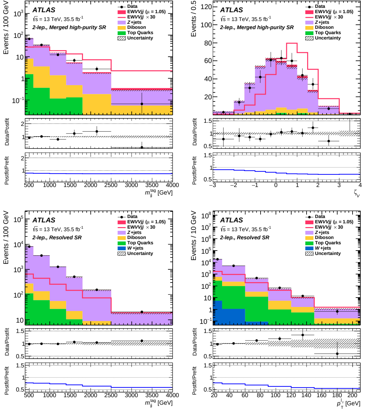
Fig. 6.30: The distributions for m_{jj}^{\text{tag}} (top left), \zeta_V (top right), and p_T^{j2} (bottom right), in the 2-lepton merged HP (top) and 2-lepton resolved (bottom) signal regions. The background contributions after the likelihood fit are shown as filled histograms. The signal is shown as a filled histogram on top of the fitted backgrounds normalized to the signal yield extracted from the observed data ( \mu = 1.05 ), and unstaked as an unfilled histogram, scaled by the factor of 30. The size of the combined statistical and systematic uncertainty for the sum of the fitted signal and background is indicated by the hatched band. The middle pane shows the ratios of the observed data to the post-fit signal and background predictions. The bottom pane shows the ratios of the post-fit and pre-fit background predictions.
