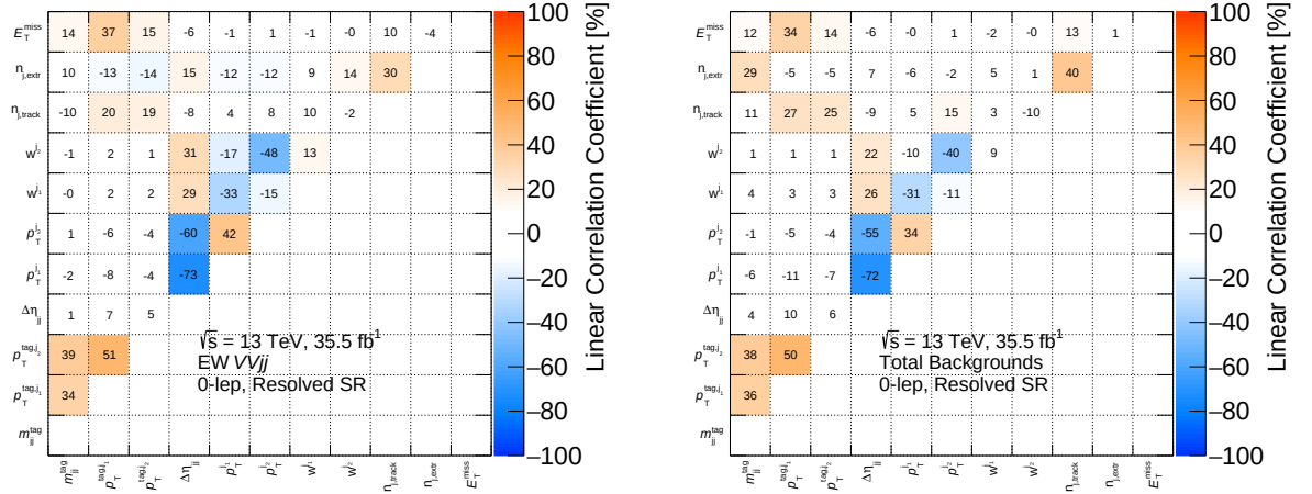
Fig. C.1: Linear correlation coefficients between input variables for signal EWVj events (left) and sum of background events (right) at the 0-lepton resolved SR. 100% (-100%) means completely correlated (anti-correlated).
