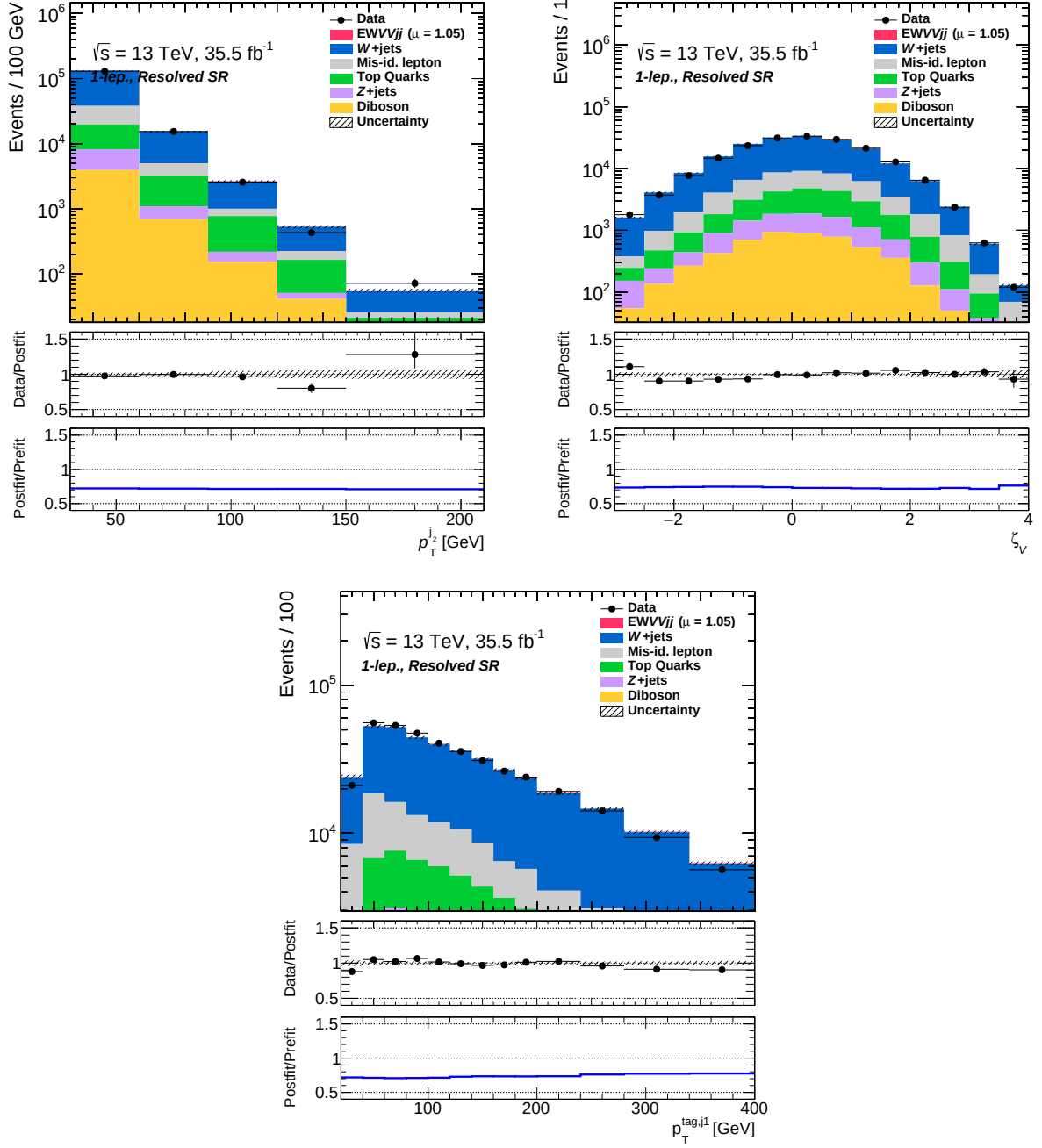
Fig. B.14: Distributions of variables used in the BDT training in the resolved region for the 1-lepton channel applying post-fit uncertainties are shown.
