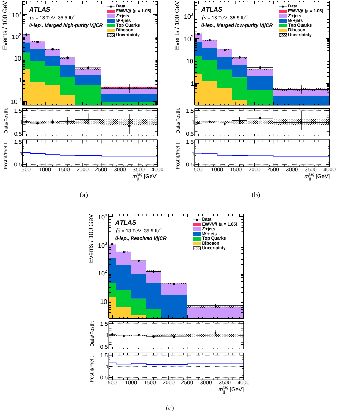
Fig. 6.22: Comparisons of the observed data and expected background distributions of m_{jj}^{\text{tag}} of the side-band control regions in the 0-lepton channel: (a) high-purity and (b) low-purity merged signal regions; (c) the resolved signal region. The background contributions after the global likelihood fit are shown as filled histograms. The signal is shown as a filled histogram on top of the fitted backgrounds normalized to the signal yield extracted from the observed data ( \mu = 1.05 ), but it is not visible due to its small contribution. The middle pane shows the ratios of the observed data to the post-fit signal and background predictions. The uncertainty in the total prediction, shown as bands, combines statistical and systematic contributions. The bottom pane shows the ratios of the post-fit and pre-fit background predictions.
