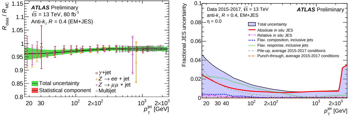
Fig. 4.15: A combination of jet energy responses measured in the observed data collected in 2015-2017 with \gamma +jets, Z \rightarrow ee +jets, Z \rightarrow \mu\mu +jets, and multijet (left) and its uncertainty breakdown (right) as a function of jet p_T are shown [91]. For the left plot, the measured energy responses with different events are consistent with each other at R_{\text{data}}/R_{\text{MC}} = 0.96 - 0.97 . As for the right plot, the flavor response and absolute in situ JES are dominant. The former is evaluated by comparing the average jet responses for each jet flavor using PYTHIA and HERWIG, the latter represents the propagated uncertainties from each measurement.
