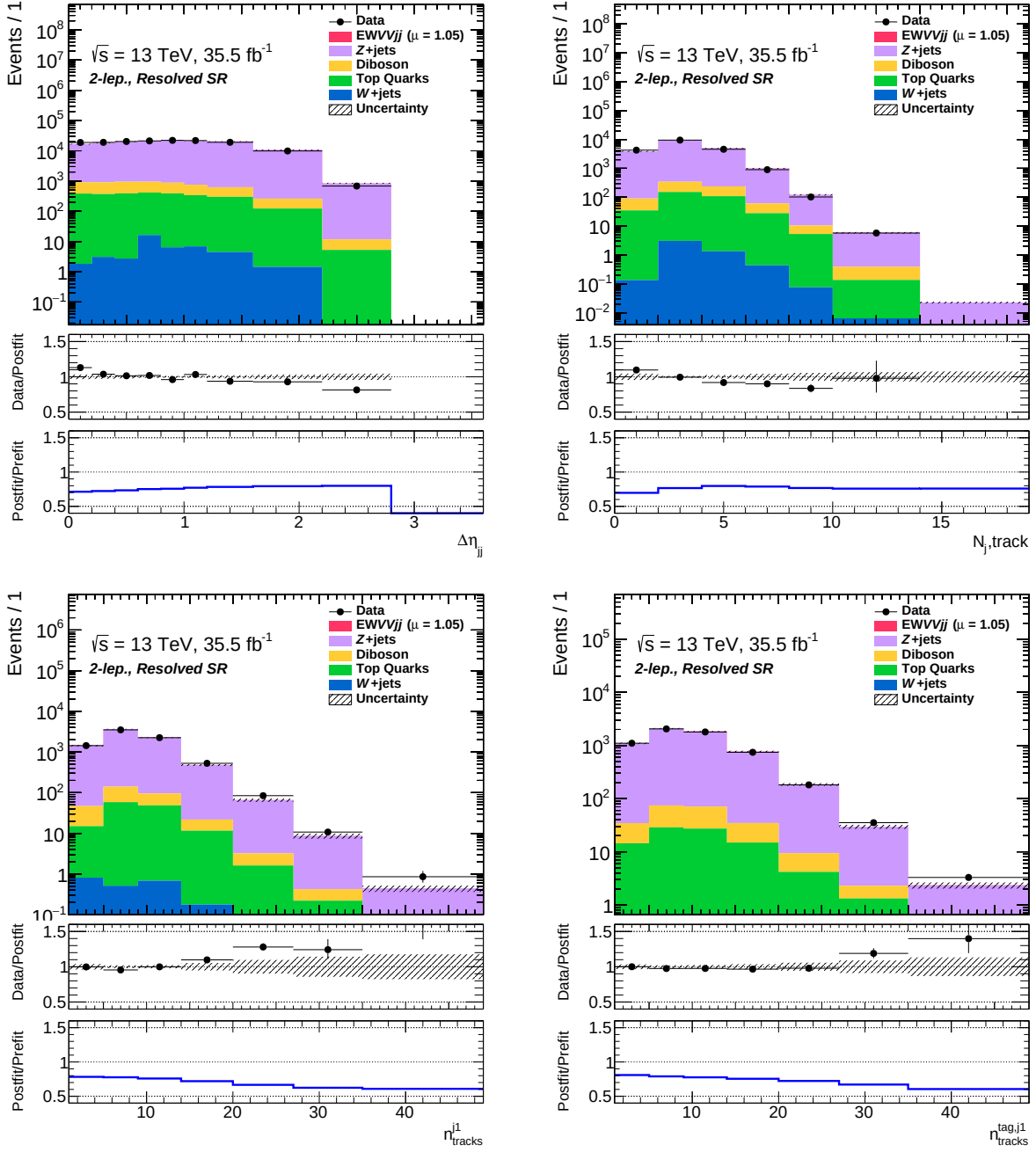
Fig. B.19: Distributions of variables used in the BDT training in the resolved region for the 2-lepton channel applying post-fit uncertainties are shown.
