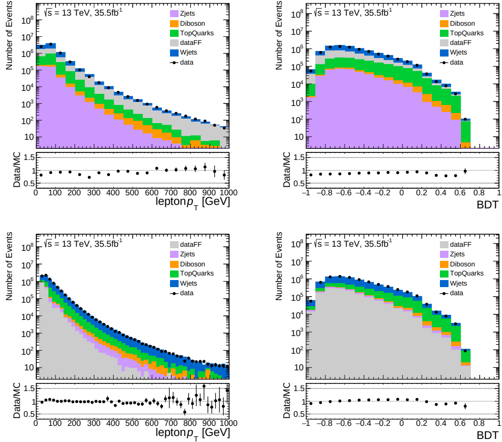
Fig. 6.19: Distributions of lepton p_T (top left) and BDT output (top right) for the electron channel, and lepton p_T (bottom left) and BDT output (bottom right) for the muon channel at the VR. The systematic uncertainties shown in Section 6.7.2 are not displayed in these plots. The gray histograms (labeled dataFF) represents the estimated multijet background by the fake factor method. The sum of predictions are approximately compatible with the observed data.
