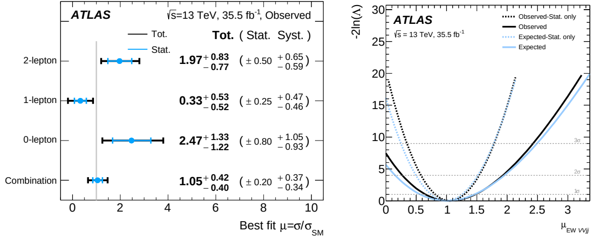
Fig. 6.34: The fitted values of the signal-strength parameter \mu_{EW VVjj}^{obs} for the 0-, 1-, and 2-lepton channels and their combination (left) and scan of the negative log-likelihood, -2 \ln \Lambda , for the signal-strength of the EW VVjj production (right) are shown. In the left plot, the individual \mu_{EW VVjj}^{obs} values for the lepton channels are obtained from a simultaneous fit with the signal-strength parameter for each of the lepton channels floating independently. The probability that the signal-strengths measured in the three lepton channels are compatible is 36%. In the right plot, the solid upper black (lower blue) line represents the observed (expected) value including all systematic uncertainties, whereas the dashed upper black (lower blue) line is for the observed (expected) value without systematic uncertainties (lower and upper refer here to the position of the lines in the legend).
