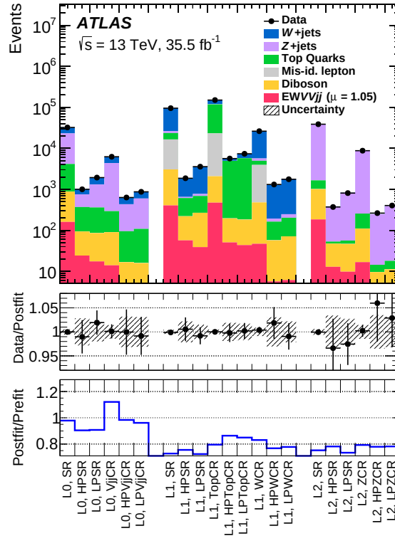
Fig. 6.21: Comparisons of the observed data and expected background event yields in each signal or control region. The labels L0, L1, and L2 stand for the 0-, 1- and, 2-lepton channels, respectively. The labels ‘HP SR’, ‘LP SR’, and ‘SR’ stand for the high-purity merged, low-purity merged and resolved signal regions, respectively. The middle pane shows the ratios of the observed data to the post-fit signal and background predictions. The bottom pane shows the ratios of the post-fit and pre-fit background predictions.
