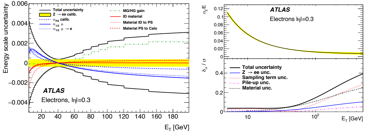
Fig. 4.7: Fractional uncertainties in the electron scale (left) and resolution (right) are shown [79]. For the left plot, the “ \alpha_X ” corresponds to the calibrations of calorimeter responses, the “MG/HG gain” denotes a relative calibration between high- and medium-gain readout, and the “material X” represents an uncertainty associated with calibrations for effects on material X. For the right plot, a stochastic term due to the sampling nature of the calorimeter (Sampling term unc.) and non-desired radiation from material in front of the calorimeter (Material unc.) are dominant.
