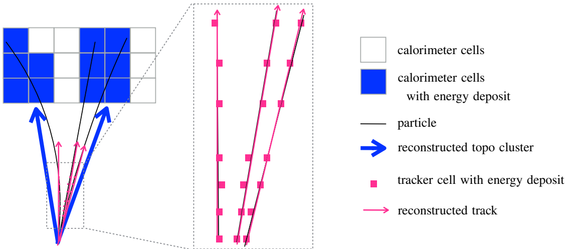
Fig. 5.12: A schematic graph for three charged particles into the calorimeter through the tracker. One of them is isolated, and the other ones are very close to each other. An isolated one is reconstructed as a single topo-cluster and a single track, whereas the other ones are reconstructed as a single topo-cluster and double tracks.
