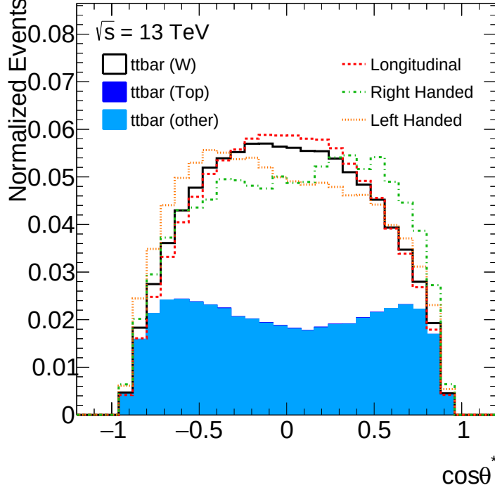
Fig. 9.3: The \cos \theta^* distribution at the reconstruction level. t\bar{t} events are shown in each case, a large-R jet matched to W \rightarrow q\bar{q} (white), a large-R jet matched to t \rightarrow W\bar{b} \rightarrow q\bar{q}\bar{b} (deep blue), and others (light blue).
