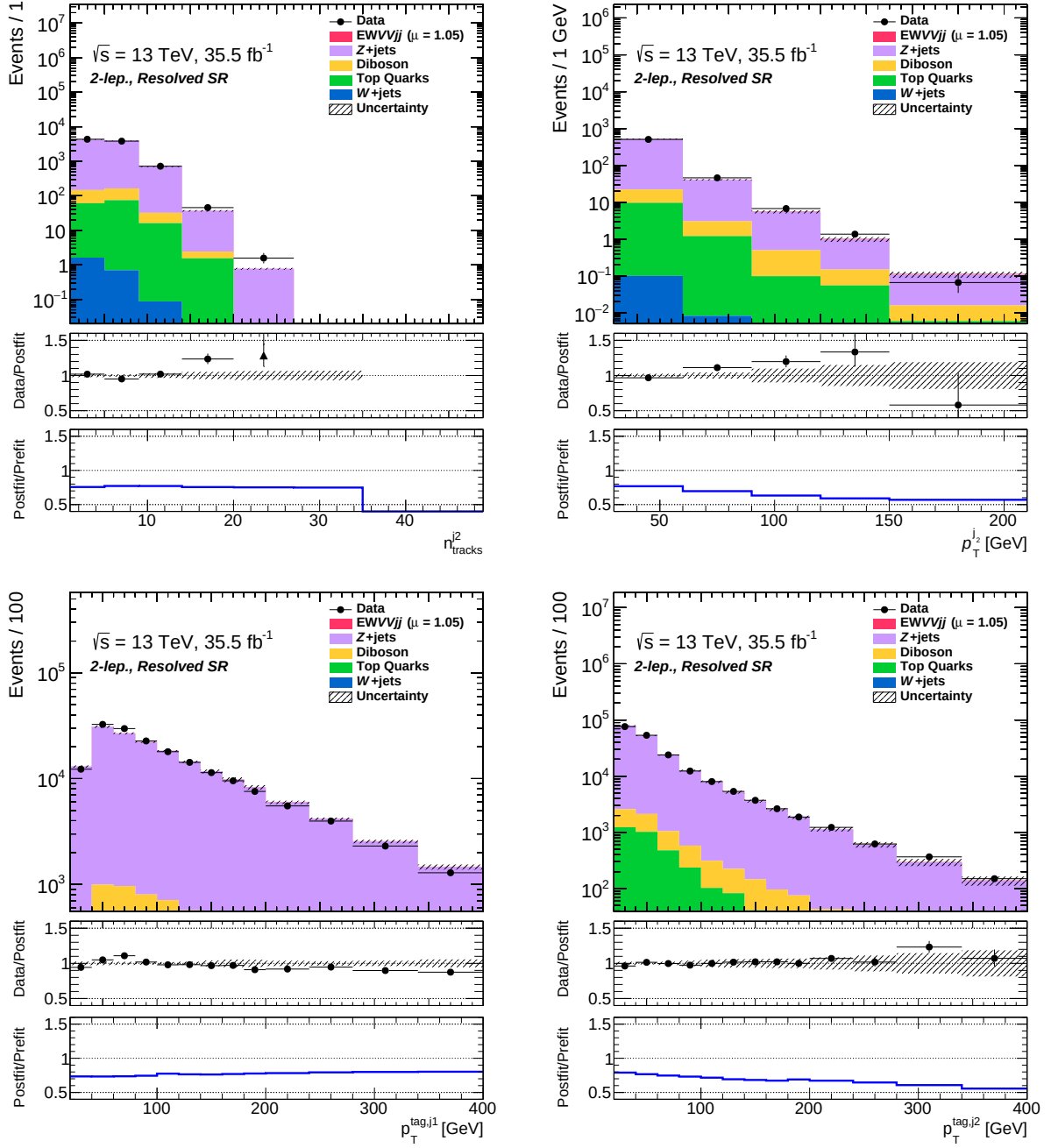
Fig. B.22: Distributions of variables used in the BDT training in the resolved region for the 2-lepton channel applying post-fit uncertainties are shown.
