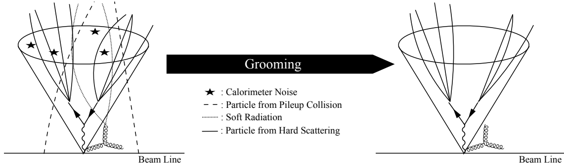
Fig. 5.2: An overview of a grooming technique is shown. The large area of a large-R jet significantly contains hits from undesired sources, pileup, soft radiation, and calorimeter noise. The trimming algorithm reclusters large-R jet with k_t R = 0.2 algorithm, and resultant jets satisfying p_T^{R=0.2}/p_T^{R=1.0} < 0.05 are trimmed.
