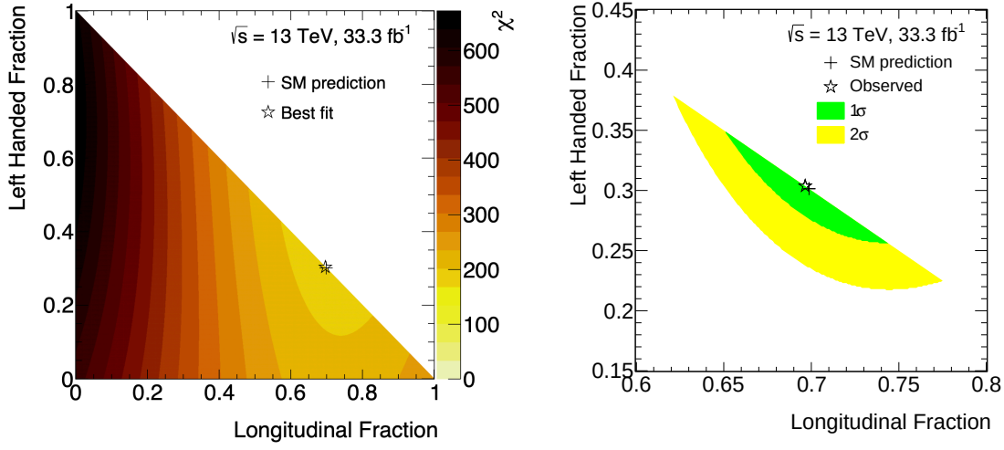
Fig. 9.6: The \chi^2 distribution with respect to each template fraction for \cos \theta^* distribution (left) and the confidence interval for the measurement (right) are shown. Only statistical uncertainty is considered.
