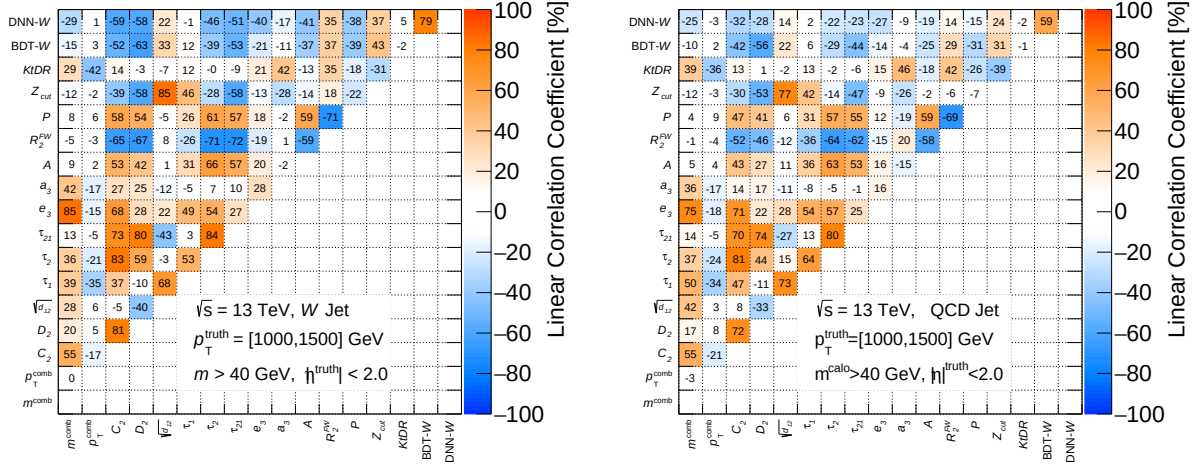
Fig. 5.18: Linear correlation coefficients between input variables for signal W boson jets (left) and background q/g jets (right) are shown. 100% (-100%) means completely correlated (anti-correlated).
