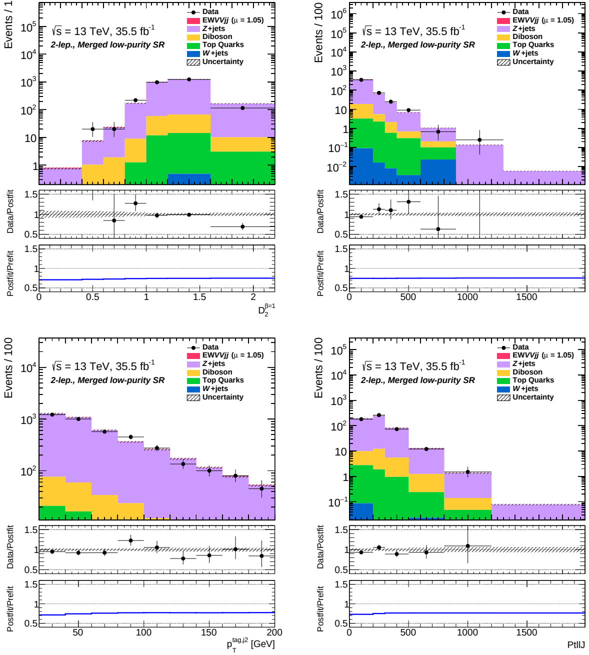
Fig. B.17: Distributions of variables used in the BDT training in the merged low-purity region for the 2-lepton channel applying post-fit uncertainties are shown.
