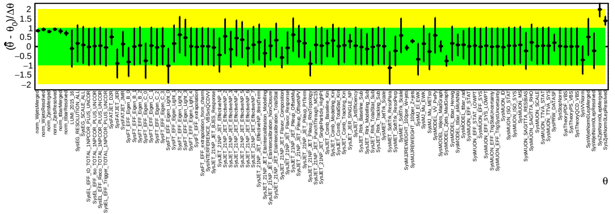
Fig. 6.31: Nuisance parameter pulls from the fit with the observed data are shown. Entries of normalization factors (begin with norm.) represent values of normalization factors and those errors as shown in Figure 6.22.
