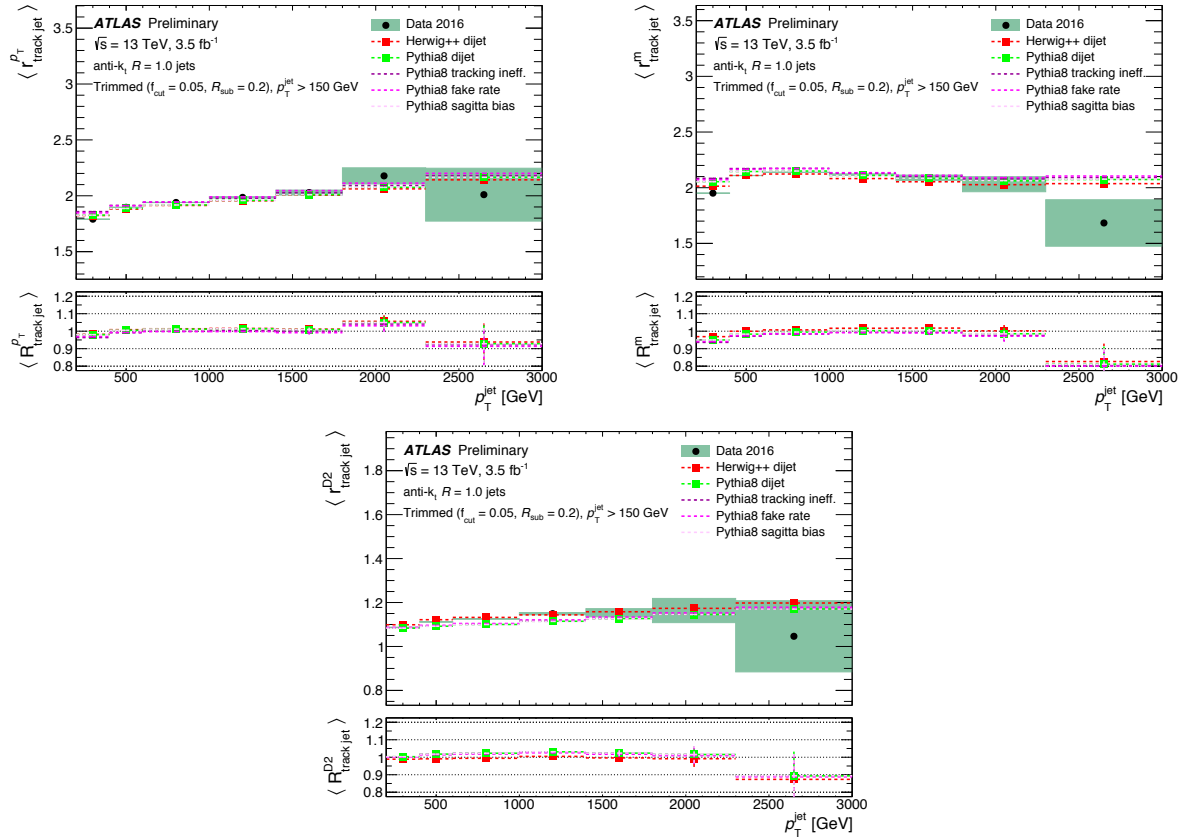
Fig. 5.11: The \langle r_{\text{trk}} \rangle and its double ratio for large-R jets p_T (left), m (right) and D_2 (bottom) with respect to large-R jets p_T are shown [112]. The observed data and nominal MC simulation (PYTHIA) are shown in black and green dots, respectively. The systematic variation of an MC simulator (HERWIG++) is shown in red dots. Three variations to evaluate tracking uncertainties are shown in dashed lines.
