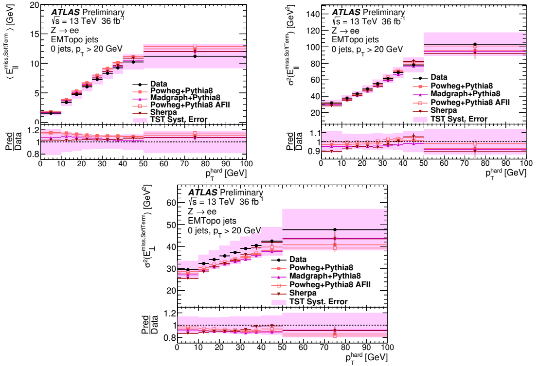
Fig. 4.19: Comparisons between the observed data and MC simulations for each the parallel scale (left), the parallel resolution (right), and the perpendicular resolution (bottom) as a function of p_T^{\text{hard}} are shown [99].
