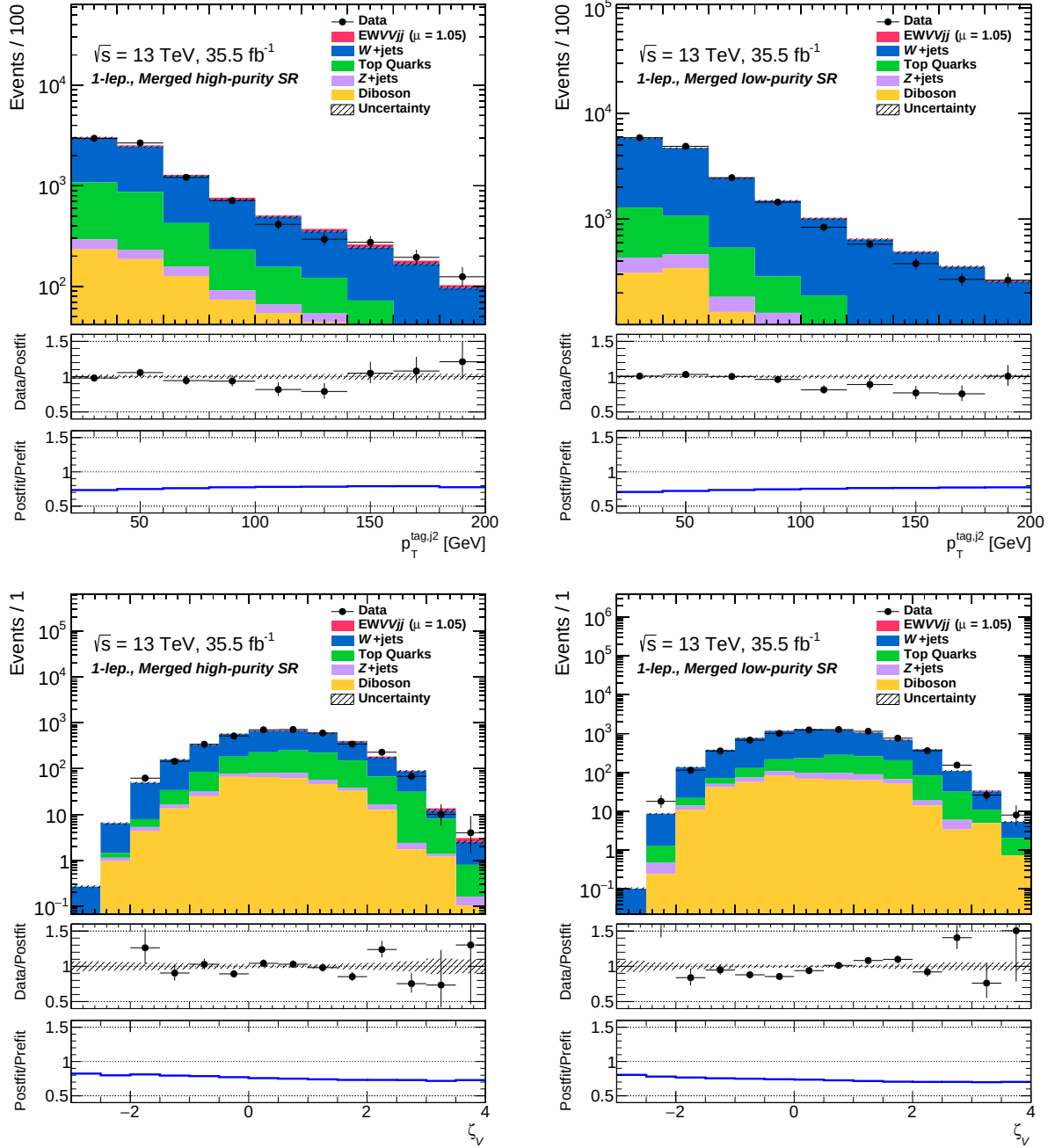
Fig. B.12: Distributions of variables used in the BDT training in the merged region for the 1-lepton channel applying post-fit uncertainties are shown.
