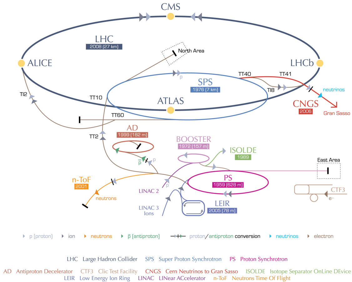
Fig. 3.1: A schematic graph of accelerators at CERN [63] is shown. The protons are accelerated by LINAC2, BOOSTER, PS, and SPS, and those are injected into LHC rings. The ATLAS detector is placed on one of the collision points of the LHC as well as the CMS, ALICE, and LHCb detectors.
