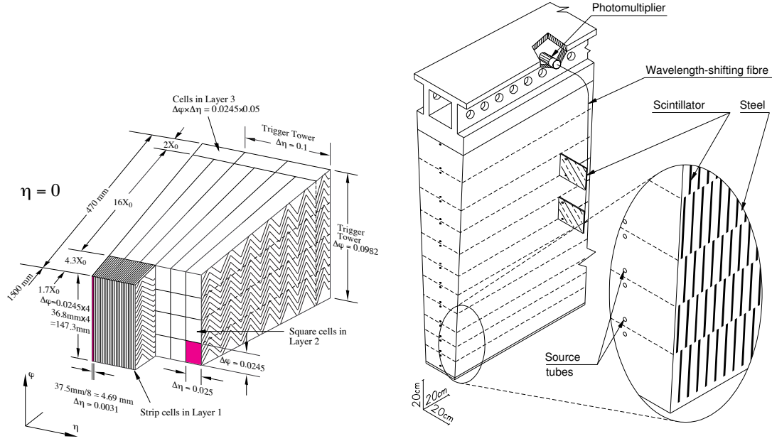
Fig. 3.6: A schematic graph of the electromagnetic calorimeter cells at pseudorapidity of 0 (left) and the barrel hadronic calorimeter cells (right) are shown. Those are taken from Reference [11]. The first layer of the electromagnetic calorimeter has a very thin width (4.69 mm) to separate \gamma and \pi_0 \rightarrow \gamma\gamma . The most of energy from electromagnetic shower deposits at the second layer having a 16 radiation length. The hadronic calorimeter cell consists of sandwiches of scintillator and steel, and the light produced by the scintillator is guided to the photomultiplier by wavelength-shifting fibers. Source tubes are made to calibrate photomultiplier gains.
