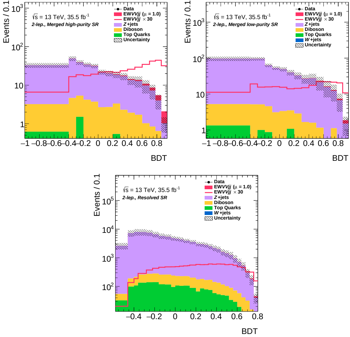
Fig. 6.11: BDT response distributions in the 2-lepton SRs, merged HP (top left), merged LP (top right) and resolved (bottom), are shown.
