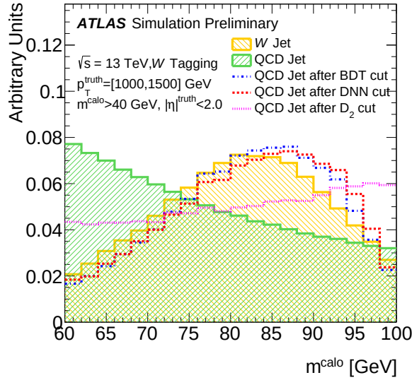
Fig. 5.22: Calorimeter mass distributions showing the signal before selection and the background both before selection, with a selection only on D_2 , with a selection on the BDT discriminant, and the DNN discriminant in the case of W boson tagging in 1000 < p_T < 1500 GeV are shown.
