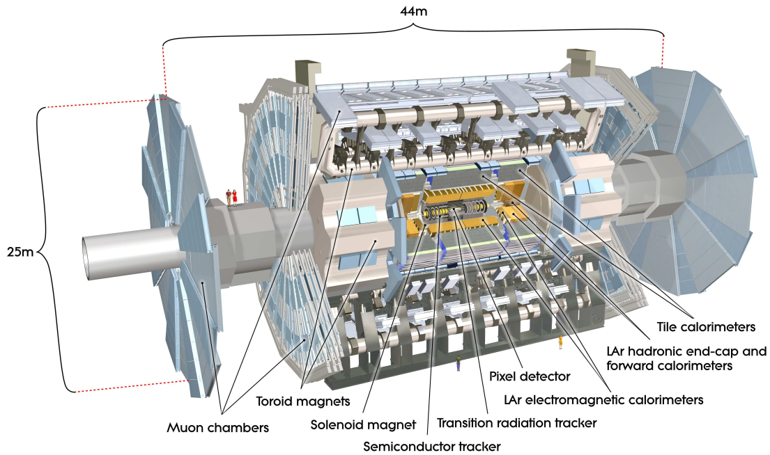
Fig. 3.2: A schematic overview of the ATLAS detector taken from Reference [11] is shown. The ATLAS has the dimensions of a 25 m diameter and a 44 m length, and its weight is 7000 tonnes. The several cylindrical detectors are explained in the main body.
