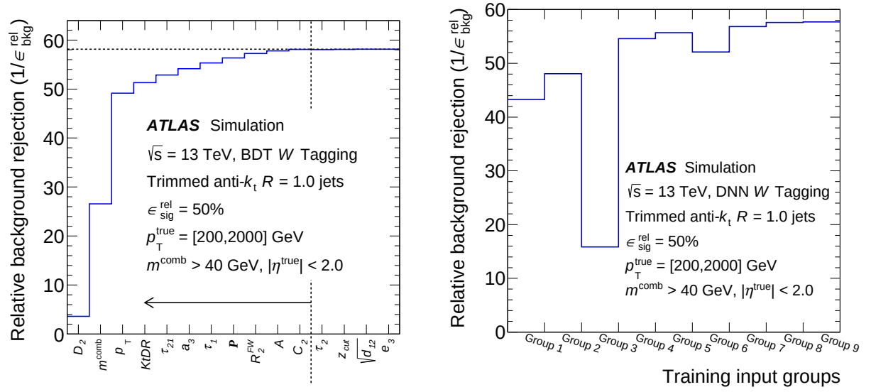
Fig. 5.19: Background rejections for the BDT (left) and DNN (right) taggers are shown. A variable set up to C_2 variable are chosen for the BDT. As for DNN, the Group 8 is chosen.
