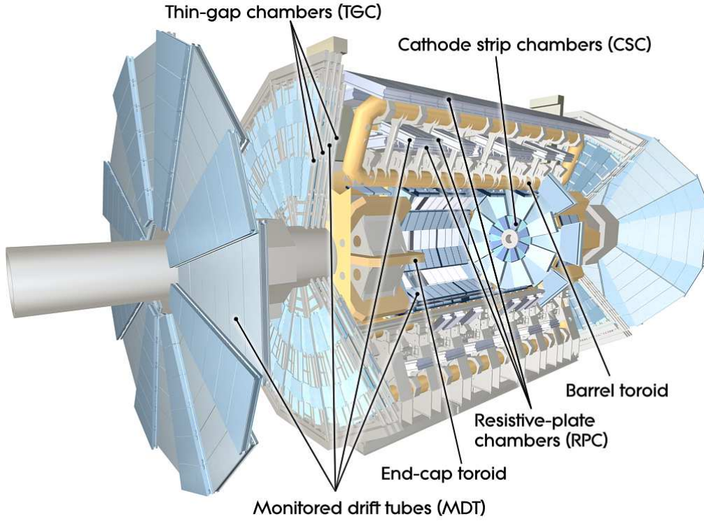
Fig. 3.8: A schematic graph of the muon spectrometer taken from Reference [11] is shown. The muon spectrometer consists of the MDT and RPC at the barrel region and the CSC and TGC at the end-cap regions. Muons are bent by the barrel toroid magnet to measure those charges and momenta.
