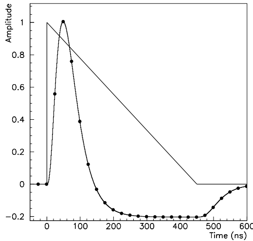
Fig. 3.7: A schematic graph of triangular pulse by the LAr calorimeter and a shaped amplitude are shown. The shaped amplitude is sampled every 25 ns. This plot is taken from [11].
