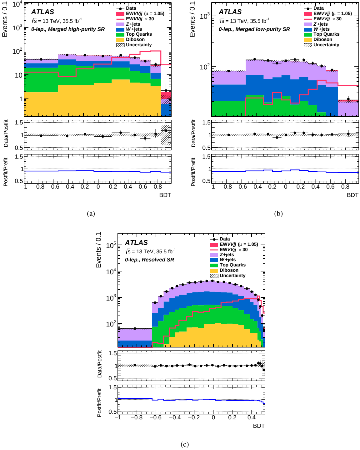
Fig. 6.25: Comparisons of the observed data and expected distributions of the BDT outputs of the 0-lepton channel signal regions: (a) high-purity and (b) low-purity merged signal regions; (c) the resolved signal region. The background contributions after the likelihood fit are shown as filled histograms. The signal is shown as a filled histogram on top of the fitted backgrounds normalized to the signal yield extracted from the observed data ( \mu = 1.05 ), and unstacked as an unfilled histogram, scaled by the factor of 30. The entries in overflow are included in the last bin. The middle pane shows the ratios of the observed data to the post-fit signal and background predictions. The uncertainty in the total prediction, shown as bands, combines statistical and systematic contributions. The bottom pane shows the ratios of the post-fit and pre-fit background predictions.
