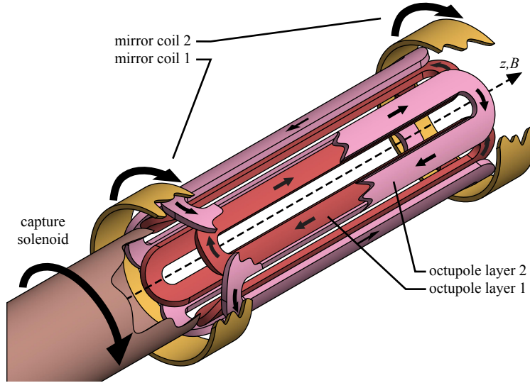
Figure 2.3: A schematic view of the cryostat magnet coils, showing the current directions in the four magnet coils. The octupole is made of layers of oppositely wound race-track coils such that the azimuthal currents on the two ends cancel out to the first order, and that the octupole would have no axial magnetic field contribution. Only two layers are shown in this schematic view, while the physical octupole contains eight counter-winding layers.
