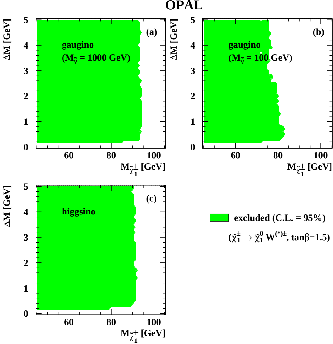
Figure 7: Lower mass limits at the 95% confidence level for various scenarios. These limits are valid for the case of a 100% branching ratio \tilde{\chi}_1^\pm \rightarrow \tilde{\chi}_1^0 W^{\pm(*)} . The limits shown for \Delta M < 0.5 GeV are only valid with the assumption of a zero chargino lifetime. For the gaugino-like scenario with a light sneutrino (b) the same signal efficiencies as in the case of a heavy sneutrino (a) were assumed.
