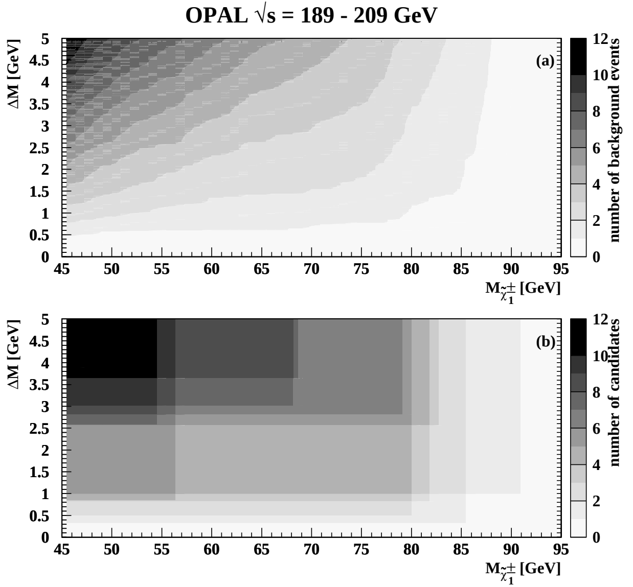
Figure 3: Number of expected background events (a) and number of candidates (b) passing the final selection cuts. The accumulated events for \sqrt{s} = 189 - 209 GeV are shown.
