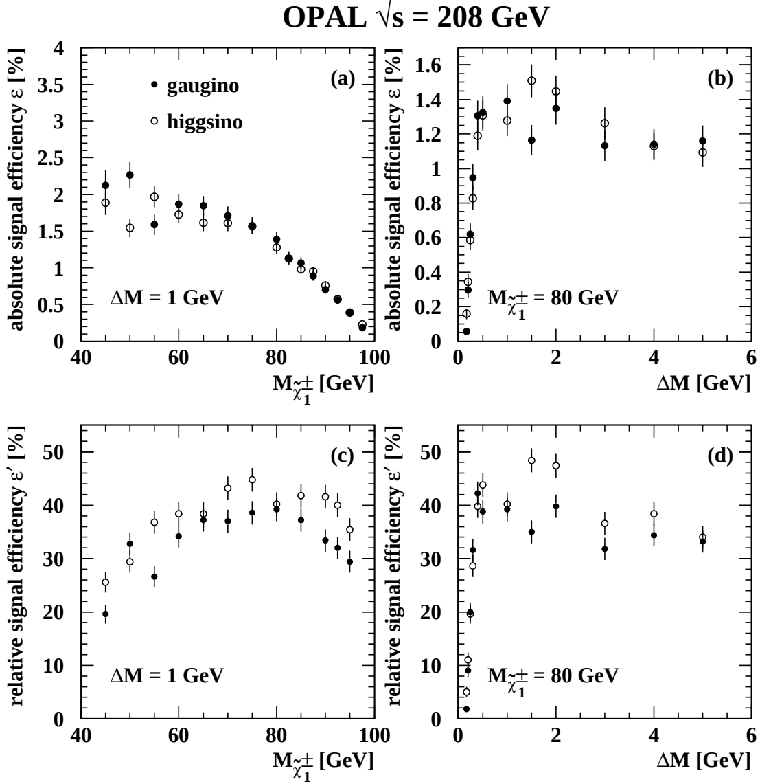
Figure 4: Absolute signal efficiency (number of selected signal events normalised to the number of generated events), \varepsilon , and relative efficiency (number of selected signal events normalised to a subset of generated events with E_T^\gamma > 0.025\sqrt{s} and |\cos\theta^\gamma| < 0.985 ), \varepsilon' , at \sqrt{s} = 208 GeV for a constant mass difference \Delta M = 1 GeV ((a)+(c)) and for a constant chargino mass M_{\tilde{\chi}_1^\pm} = 80 GeV ((b)+(d)). The efficiencies for the gaugino-like scenario are indicated by the points. The circles correspond to the efficiencies in the case of a higgsino-like chargino.
