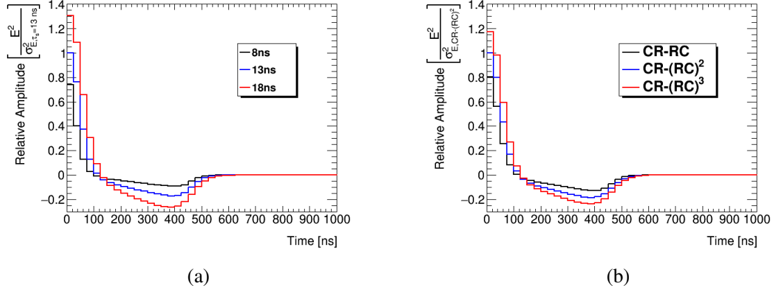
Fig. 5.8 Pileup autocorrelation function for (a) different shaper time constants with a CR - (RC)^2 shaper and (b) different shaper circuits with time constants CR = RC = 13 ns in the HEC channel located in layer HEC1 at \eta = 2.35 . Autocorrelation functions are normalized to the mean square of the pileup noise in the current HEC shaper (CR - (RC)^2) with \tau_s = RC = 13 ns).
