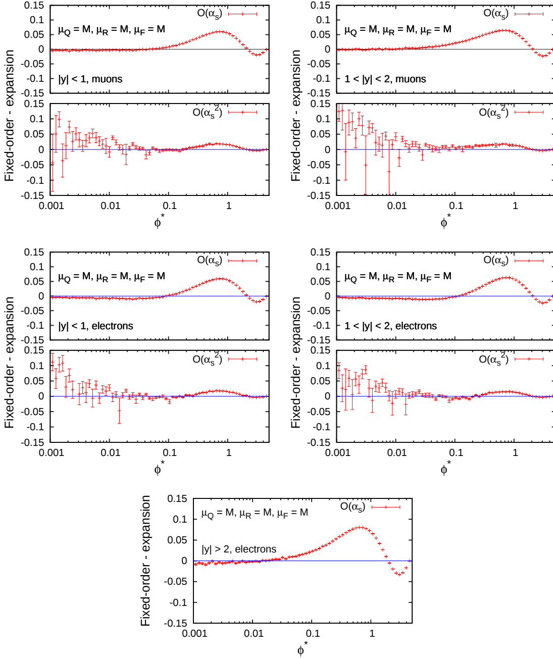
FIGURE 5.3. Remainder plots showing the cancellation of large logarithms between the fixed-order component and the expansion of the resummed component, order by order, for small values of \phi^* . The plots show the various rapidity ranges for the muon and electron channels in DØ data.
