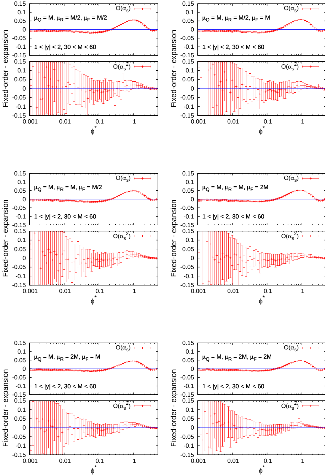
FIGURE C.20. Plots showing the cancellation of large logarithms between the fixed-order component and the expansion of the resummation, for D0 data at low invariant mass and the rapidity range 1 < |y| < 2 . The scale \mu_Q = M .
