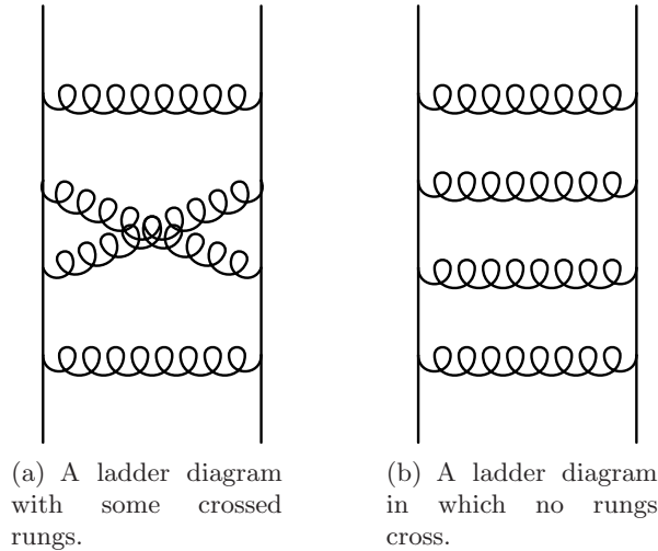
FIGURE 3.4. A ‘ladder’ diagram representation of |\mathcal{M}|^2 for an arbitrary number of gluon emissions. In the collinear limit, the leading terms come from the diagram in which no rungs cross, which gives rise to the concept of independent emission probabilities. Diagrams in which rungs cross give sub-leading contributions.
