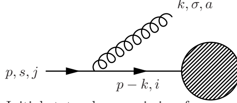
FIGURE A.6. Initial-state gluon emission for an arbitrary hard process \mathcal{M}_i^n , which may contain n additional gluons but which may not interfere with the gluon k . Momenta and quantum numbers have been labelled.
