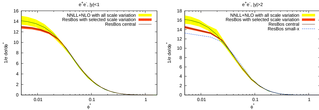
FIGURE 5.18. A comparison between our NNLL+NLO prediction and that of ResBos is shown, for the D\bar{O} electrons channel in the two rapidity bins |y| < 1 (central) and |y| > 2 (forward).
