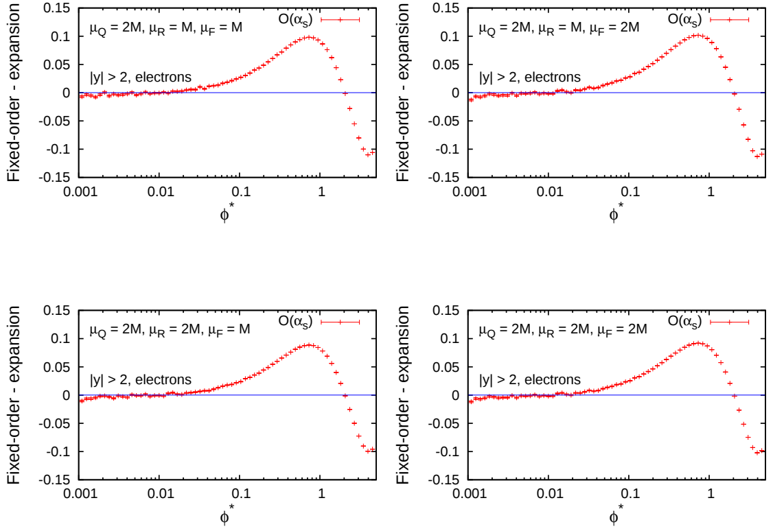
FIGURE C.9. Plots showing the cancellation of large logarithms between the fixed-order component and the expansion of the resummation, for DØ data in the Z \rightarrow ee channel around the resonance and the rapidity range |y| > 2 . The scale \mu_Q = 2M .
