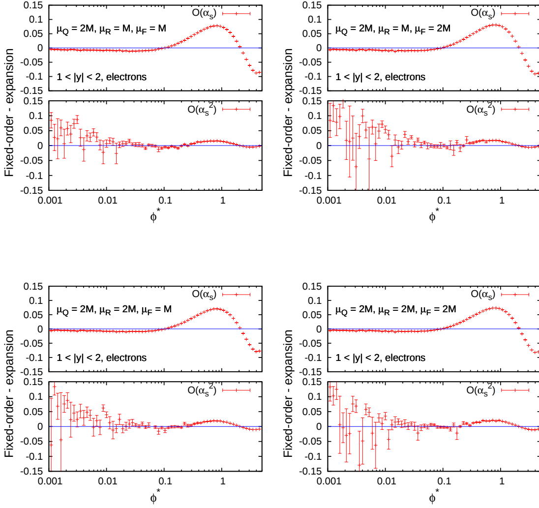
FIGURE C.6. Plots showing the cancellation of large logarithms between the fixed-order component and the expansion of the resummation, for DØ data in the Z \rightarrow ee channel around the resonance and the rapidity range 1 < |y| < 2 . The scale \mu_Q = 2M .
