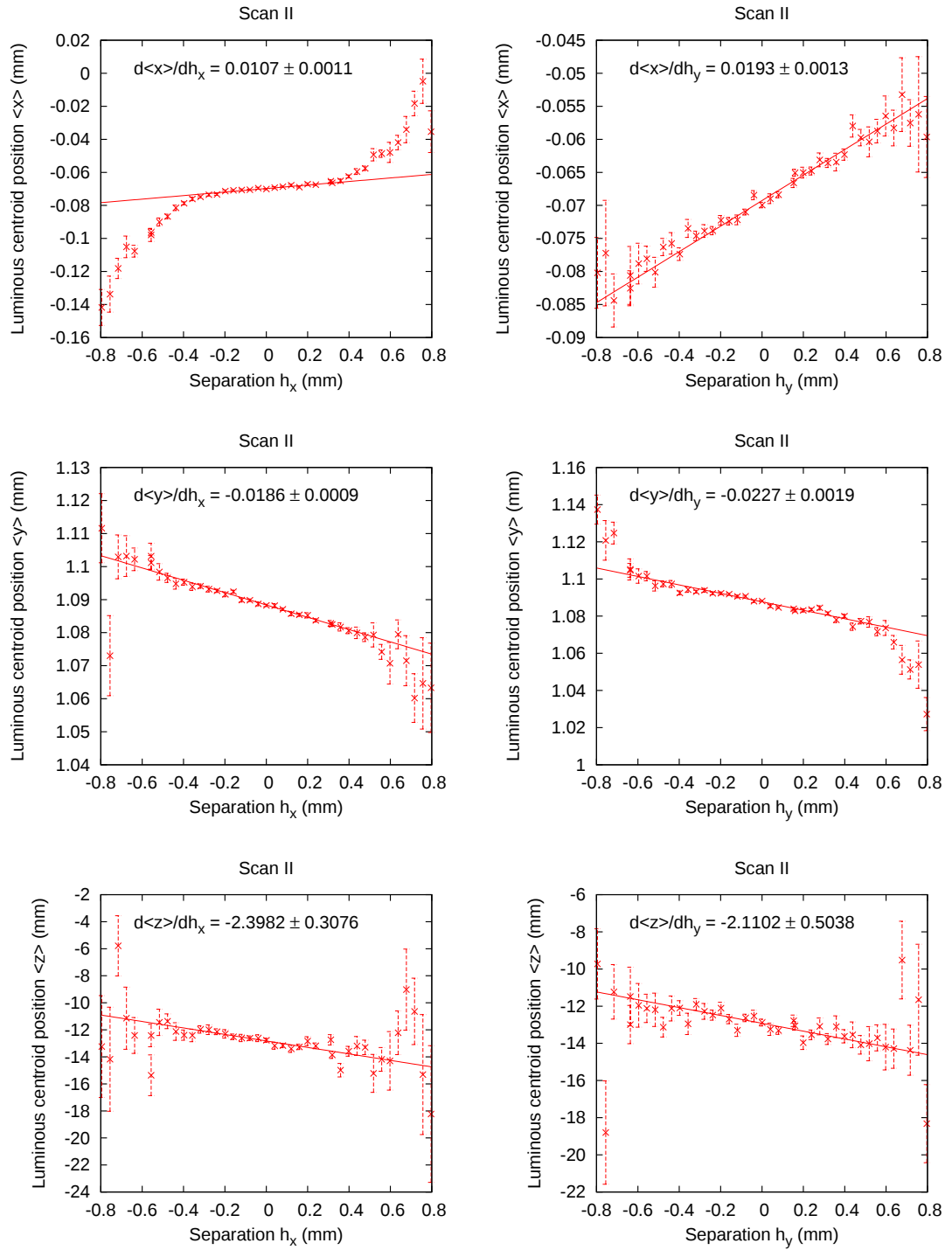
FIGURE 17.2. Luminous centroid movements during Scan II in (March) 2011. The continued presence of clearly non-linear tails again require that the fits are to central scan data only, in the range [-0.3, 0.3] mm. The errors on the luminous centroid positions are of statistical origin only.
