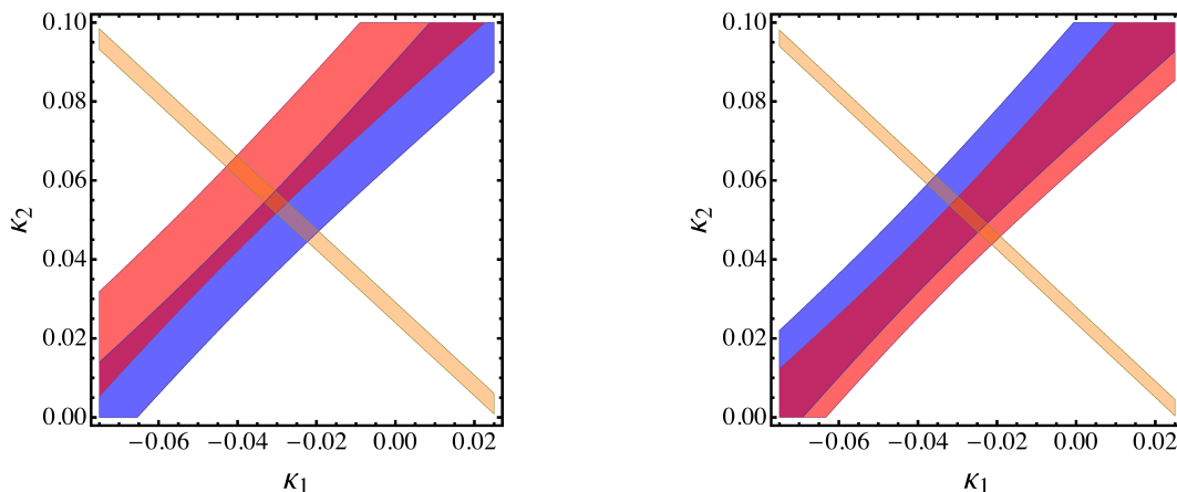
FIGURE 17.5. The constrained regions of (\kappa_1, \kappa_2) space, for scans I and II of March 2011. The constraints are generally very consistent, especially in scan II, and they are both strongly indicative of negligibly small correlation coefficients from the standpoint of the luminosity calibration error. The bands of negative slope come from a direct comparison of Eq. 16.15 with the values of \kappa^{\mathcal{L}} measured for the luminous region. The widths of the bands directly reflect the errors on these measurements. The bands of positive slope come from comparing the analytical expressions for d\langle x\rangle/dh_y (blue) and d\langle y\rangle/dh_x (red) with the corresponding fitted slopes of Figs. 17.1 and 17.2. The widths come from the fit errors and the propagated errors from the constrained individual beam widths.
