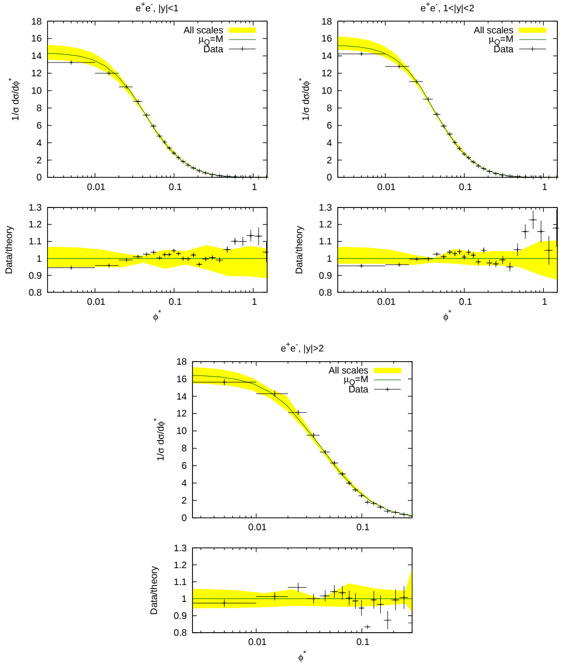
FIGURE 5.4. Our matched calculation for DØ data in the electrons channel, for the three boson rapidity regions |y| < 1 , 1 < |y| < 2 and |y| > 2 .
