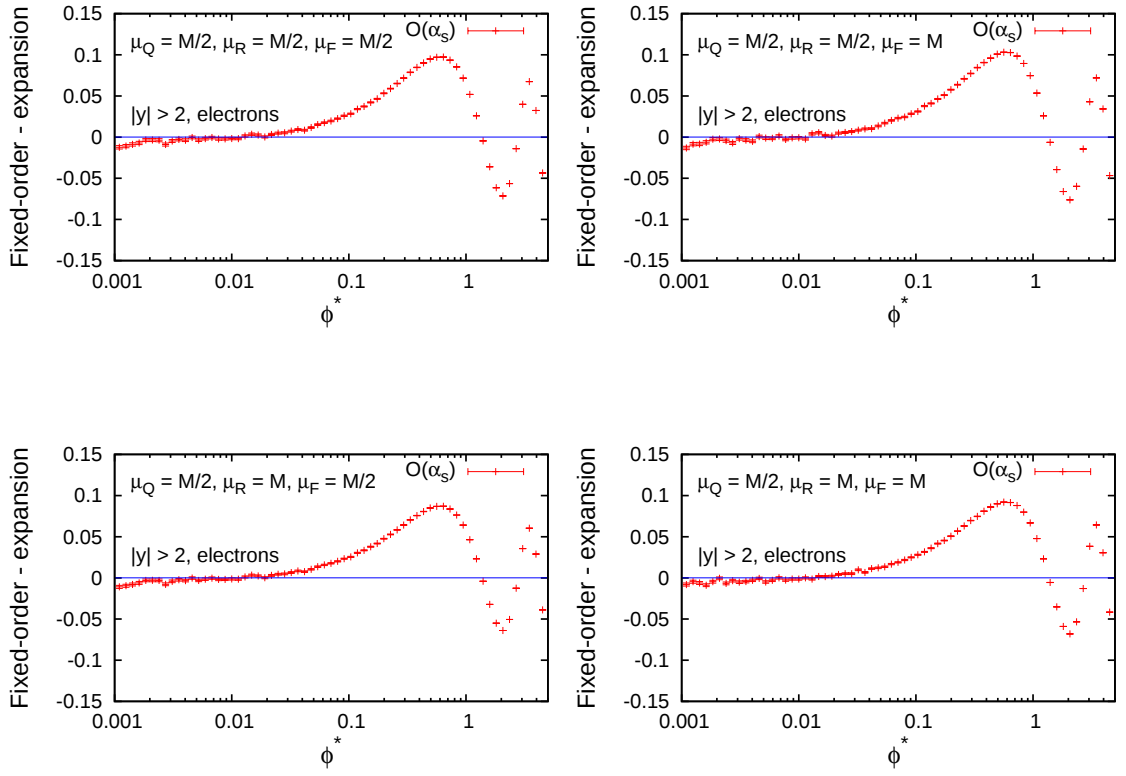
FIGURE C.7. Plots showing the cancellation of large logarithms between the fixed-order component and the expansion of the resummation, for DØ data in the Z \rightarrow ee channel around the resonance and the rapidity range |y| > 2 . The scale \mu_Q = M/2 .
