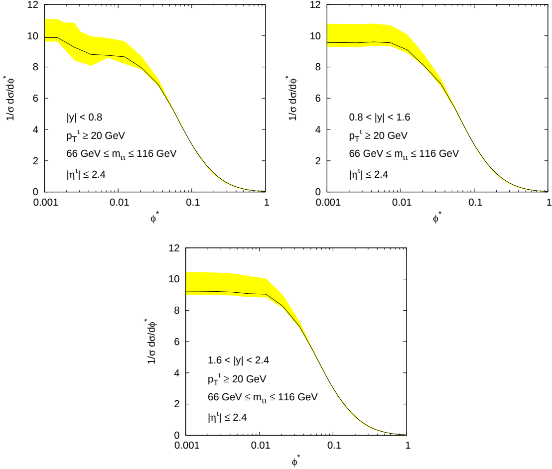
FIGURE 5.13. Our \phi^* predictions for ATLAS kinematics at \sqrt{s} = 7 TeV, in the three rapidity regions |y| < 0.8 , 0.8 < |y| < 1.6 and 1.6 < |y| < 2.4 , top left, top right and bottom centre, respectively.
