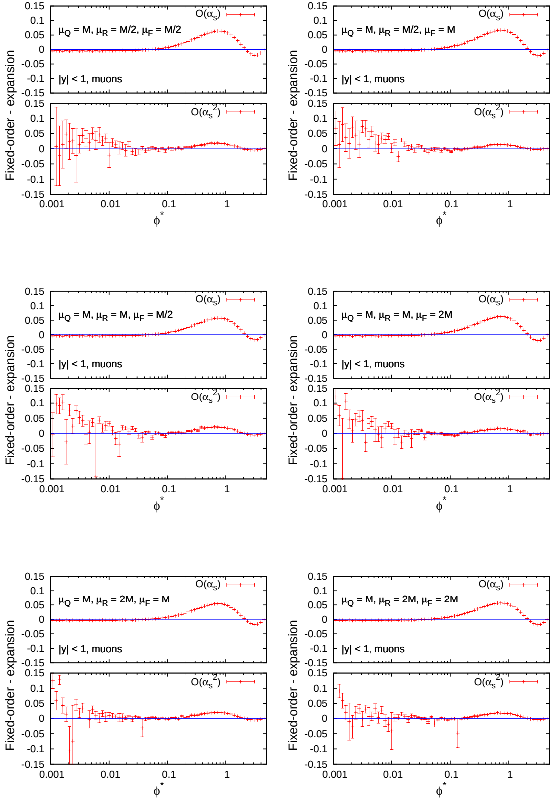
FIGURE C.11. Plots showing the cancellation of large logarithms between the fixed-order component and the expansion of the resummation, for D\bar{O} data in the Z \rightarrow \mu\mu channel around the resonance and the rapidity range |y| < 1 . The scale \mu_Q = M .
