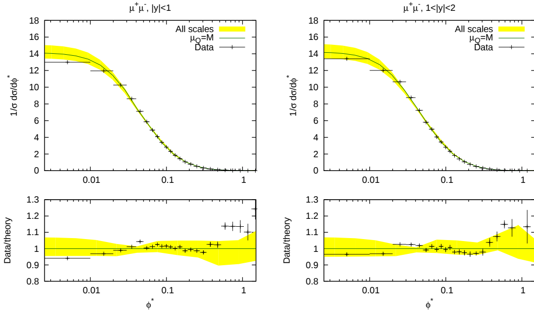
FIGURE 5.5. Our matched calculation for D\bar{O} data in the muons channel, for the two boson rapidity regions |y| < 1 and 1 < |y| < 2 .
