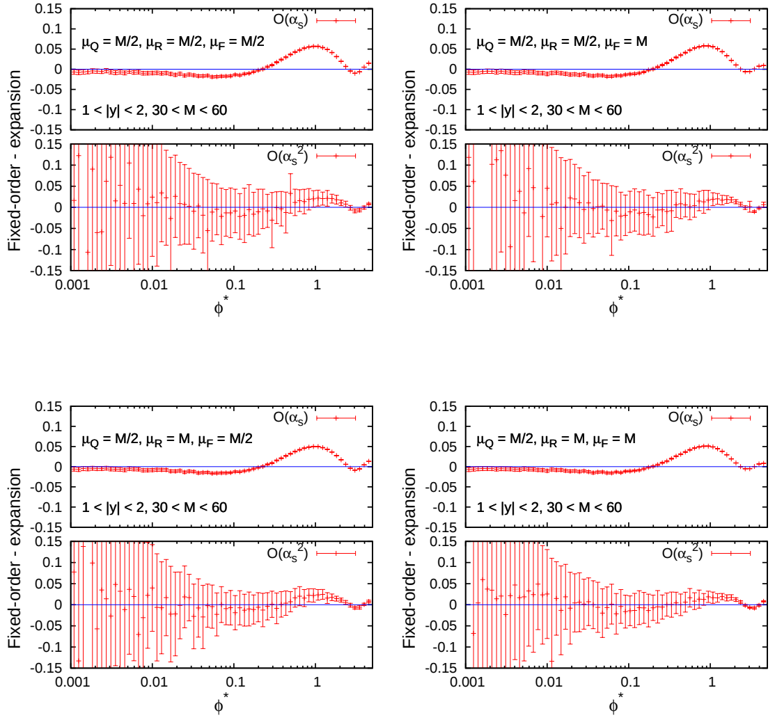
FIGURE C.19. Plots showing the cancellation of large logarithms between the fixed-order component and the expansion of the resummation, for D\bar{O} data at low invariant mass and the rapidity range 1 < |y| < 2 . The scale \mu_Q = M/2 .
