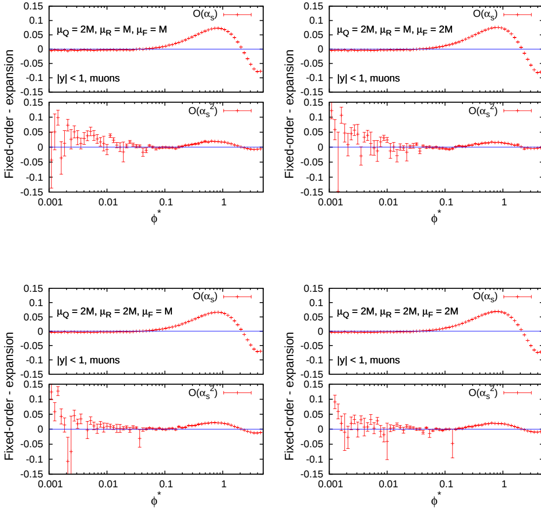
FIGURE C.12. Plots showing the cancellation of large logarithms between the fixed-order component and the expansion of the resummation, for DØ data in the Z \rightarrow \mu\mu channel around the resonance and the rapidity range |y| < 1 . The scale \mu_Q = 2M .
