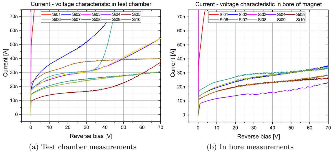
Figure 13: Current-voltage characteristics for the ten (eight) silicon detectors. Left: test in the small chamber with all ten detectors, right: test of eight detectors installed in the bore of the magnet.
