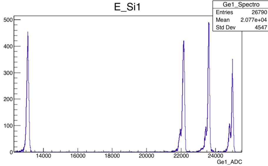
Figure 14: Energy spectrum of a mixed alpha source measured with one of the silicon detectors. The vertical axis shows counts in arb. units, the horizontal axis the not yet calibrated ADC channels. Plot from V. Araujo-Escalona.
