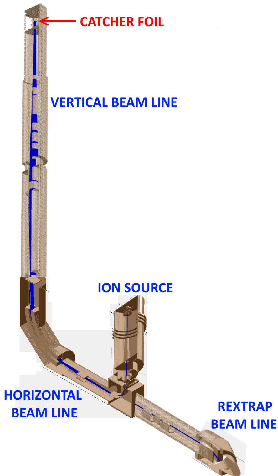
Figure 18: Visualization of the beam line simulation with SIMION. The four parts are the vertical beam line, the horizontal beam line, the REXTRAP beam line, and the ion source.
