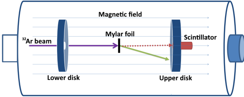
Figure 5: Schematic of the detector. The eight silicon detectors are located on the two disks above and below the Mylar foil. The scintillator sits in the hole of the upper disk. Gravity is pointing to the left. Graphic from V. Araujo-Escalona.
