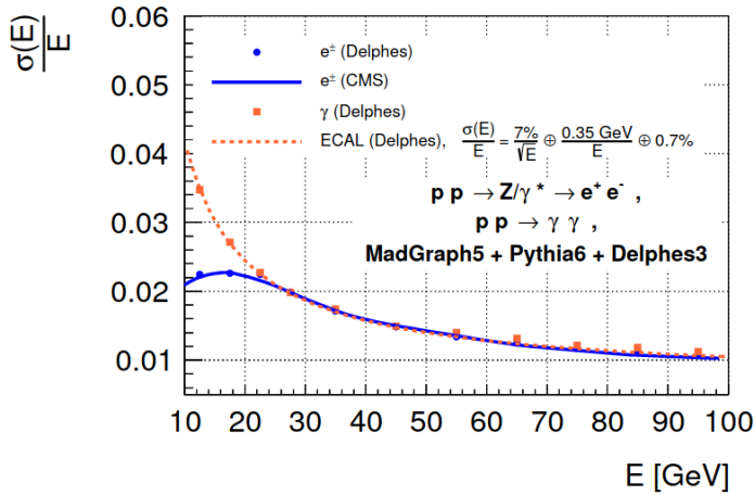
Figure 2.15. | Electron and photon energy resolution as a function of the energy for a CMS-like detector. The electron resolution agrees well between CMS and DELPHES. The electron and photon resolutions match perfectly the ECAL resolution at high energies. However, at low energies the electron resolution is driven by the tracking resolution. From [44].
