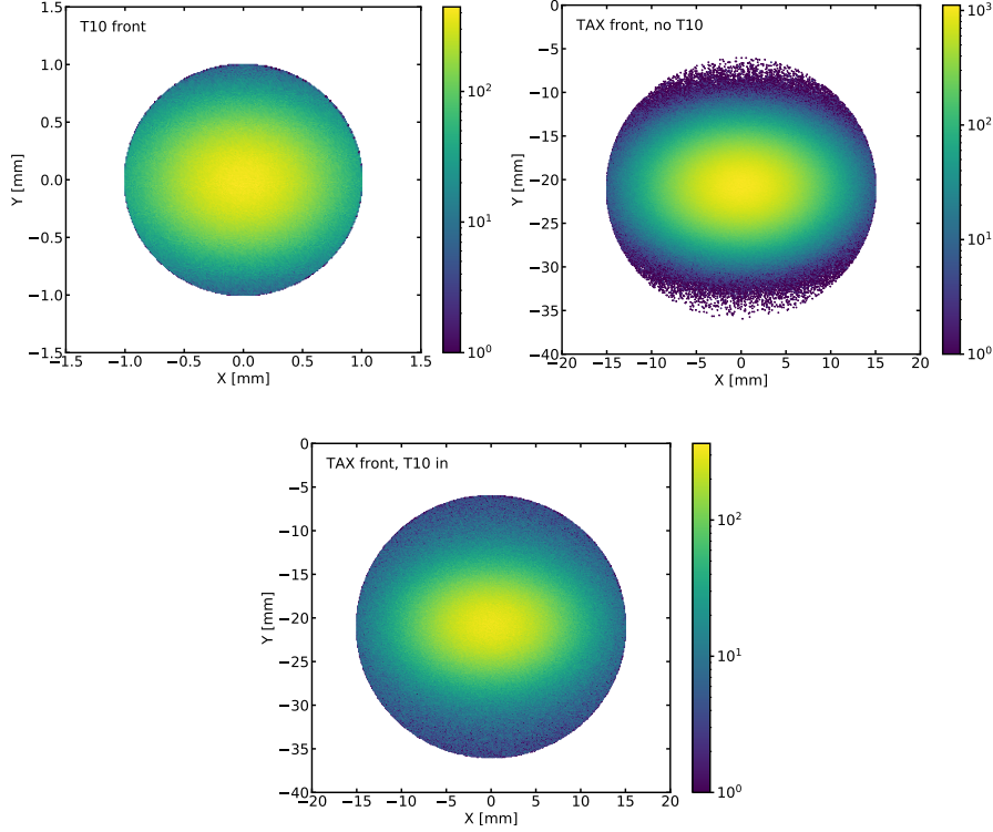
FIGURE 4.3: Proton distributions on the target and TAX front planes obtained with the help of the dedicated beamline simulation described in [168]. The distributions are used to sample the primary production position in the exotic Monte Carlo.
