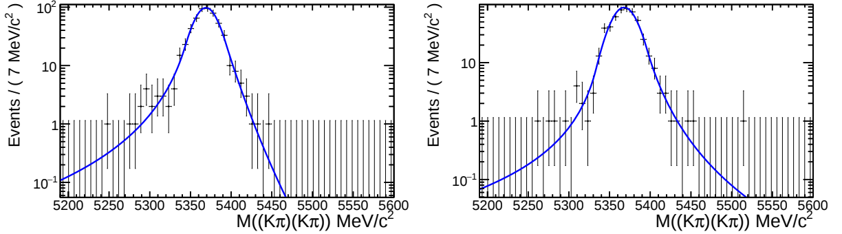
Figure 4.10: Hypatia fit to the B_s^0 \rightarrow K^*(892)^0 \bar{K}^*(892)^0 simulated samples, corresponding to 2011 and 2012 conditions, are shown in the left and right plots, respectively. The same set of parameters is used to describe the B_s^0 and the B^0 line shapes.
