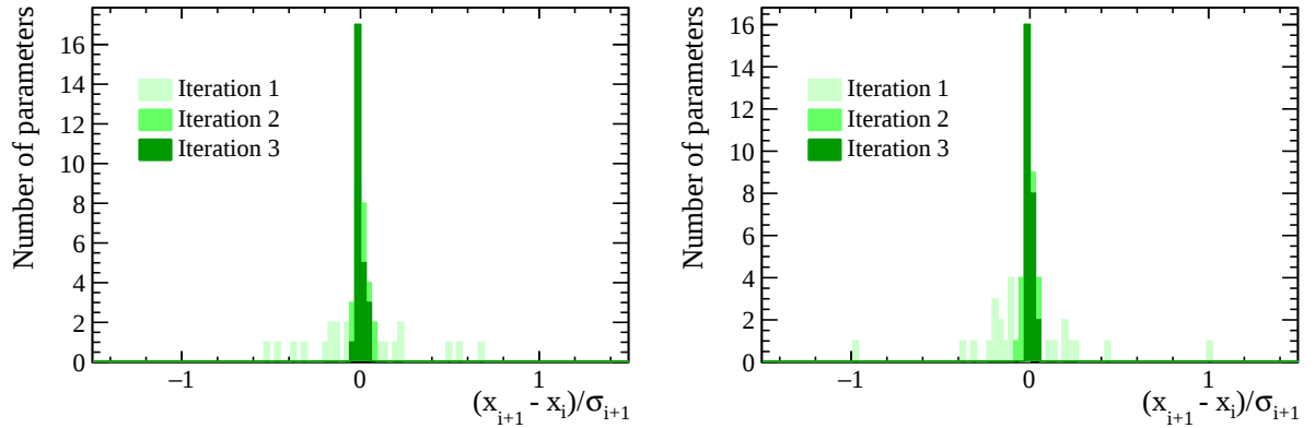
Figure 5.13: Evolution of the pull like distribution of the fit parameters with the number of iterations of the iterative reweight, for the B^0 sample on the right and the \bar{B}^0 sample on the left. The pull variable is built comparing the value of a given parameter ( x ) in the i^{\text{th}} and the (i + 1) iterations, divided by its statistical uncertainty ( \sigma ).
