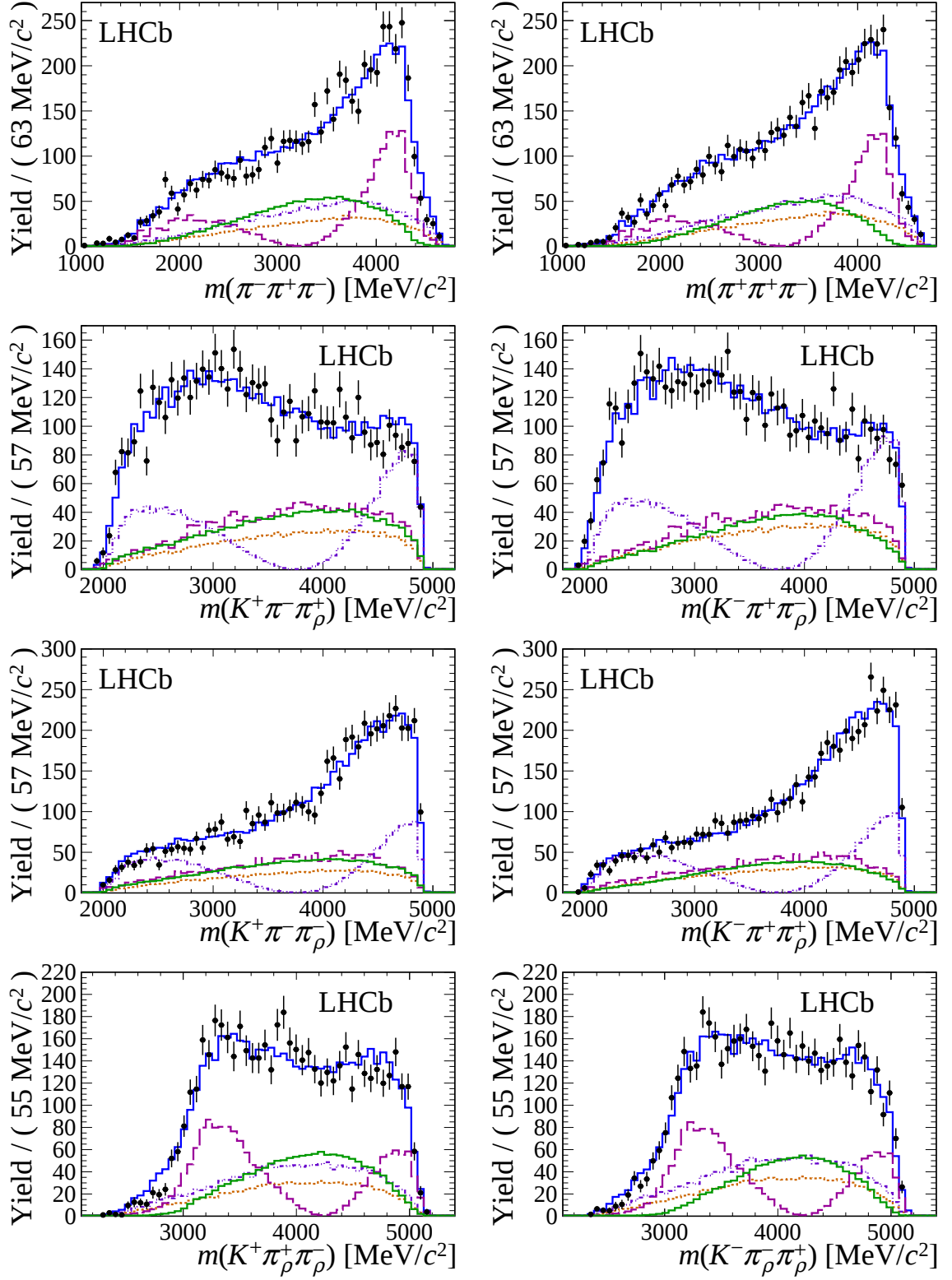
Figure 5.10: The four possible combinations of three-body invariant mass spectra for the fitted model, projected over weighted data in the B^0 (left) and \bar{B}^0 (right) samples.
