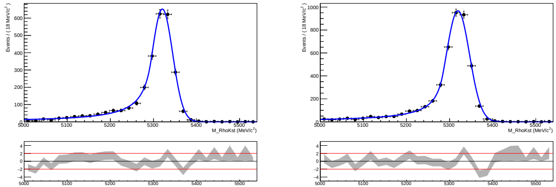
Figure 4.16: Fit to simulated B_s^0 \rightarrow K^*(892)^0 \bar{K}^*(892)^0 events per Year categories (2011MC on the left and 2012MC on the right). The fitted values are shown in Table 4.15.
