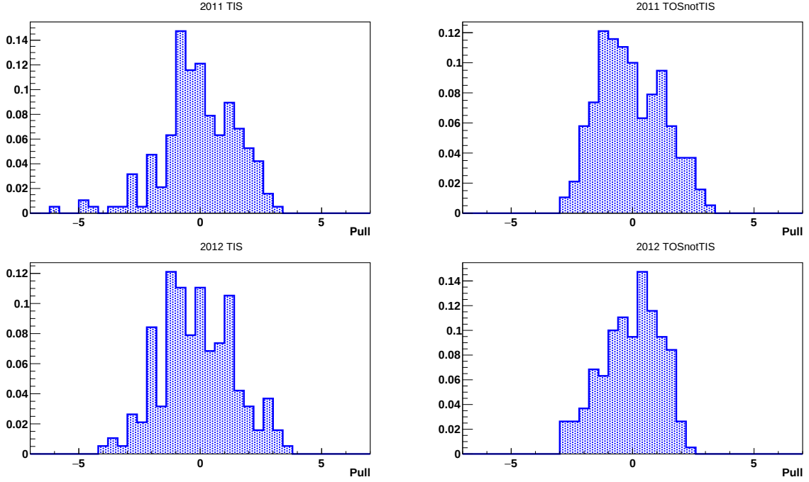
Figure 5.3: Pull distributions for the normalisation weights computed with the two simulated data sub-samples when compared with the nominal (combined) one.
