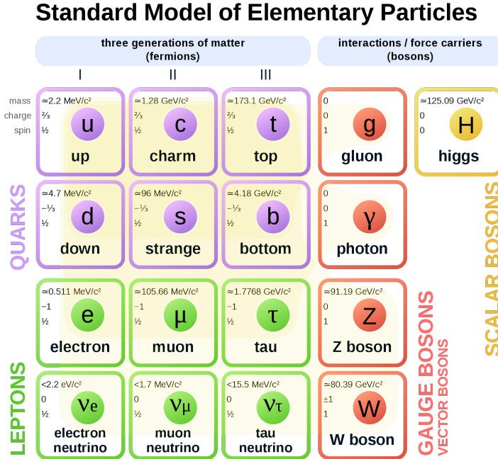
Figure 1.1: Fundamental particles in the Standard Model of Particle Physics. Leptons and quarks are the fermionic constituents of matter, organised in a 3-fold structure (first three columns) of families. The fourth column shows the gauge bosons, which are the force carriers associated to the strong, electromagnetic and weak interactions, respectively. The Higgs boson, arising from the spontaneous symmetry breaking of the electroweak sector, appears in the fifth column. Figure taken from [11].
