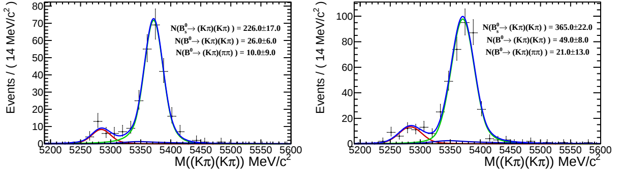
Figure 4.9: Fits to the (K^\pm\pi^\mp)(K^\mp\pi^\pm) invariant mass spectra, for 2011 (left) and 2012 (right) data, in Sample 2. The B_s^0 \rightarrow K^*(892)^0 \bar{K}^*(892)^0 is shown in light green, the B^0 \rightarrow K^*(892)^0 \bar{K}^*(892)^0 in red and the broad pollution below the peaks (dark blue) corresponds to the remaining B^0 \rightarrow \rho^0 K^{*0} events in these samples.
