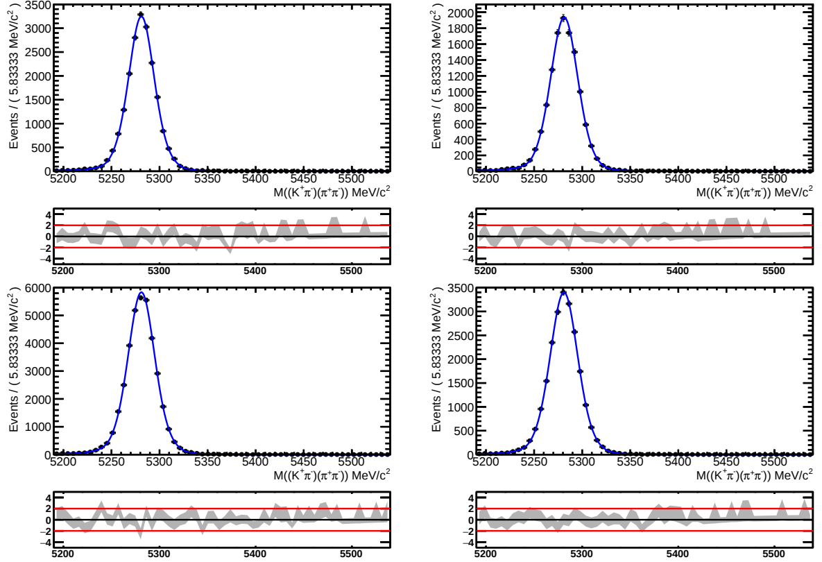
Figure 4.15: Fits to simulated B^0 \rightarrow \rho^0 K^{*0} events per Year | |Trigger categories. Results for 2011(12) are shown on the top (bottom) row, with the TIS(TO Snot TIS) on the left (right)side. The fitted values are shown in Table 4.14.
