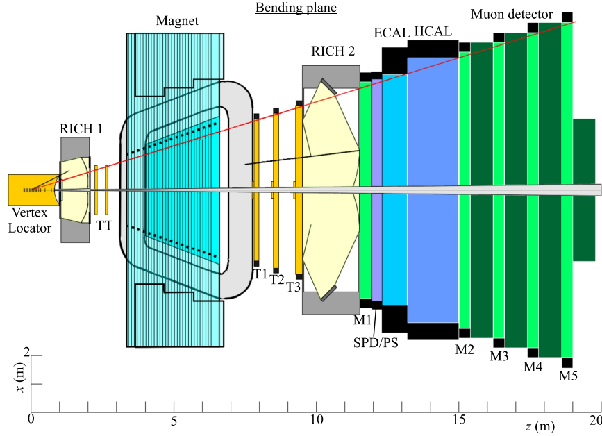
Figure 2.6: The LHCb setup [50] with the different subdetectors shown in the bending plane ( xz ) of the magnet.
