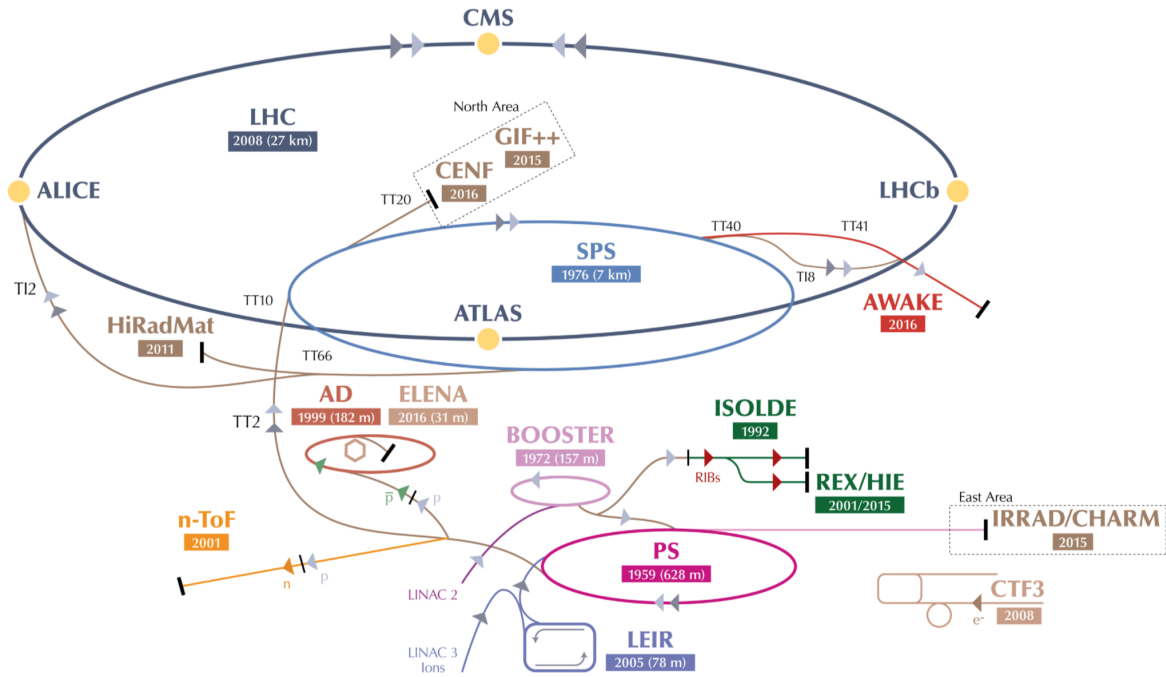
Figure 2.1: A schematic of the CERN accelerator complex, the LHC and the location of the main experiments. Figure taken from [44].
