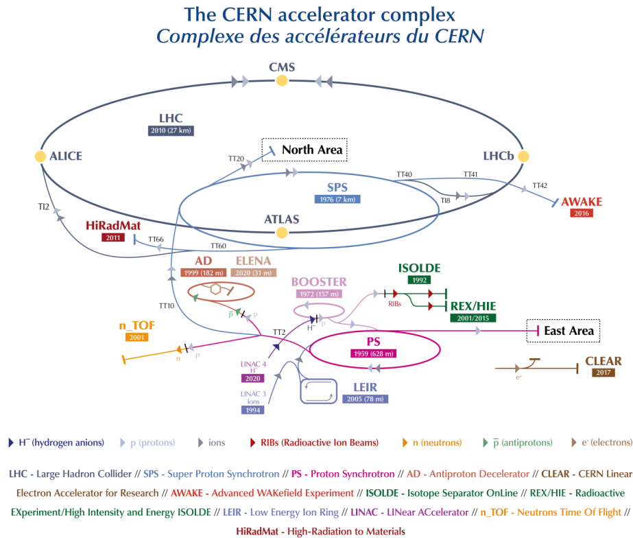
Figure 1.3: CERN Accelerator Complex, Source: [16]
