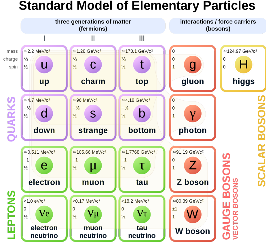
Figure 1.1: Particles of the Standard Model, Source: [4]
