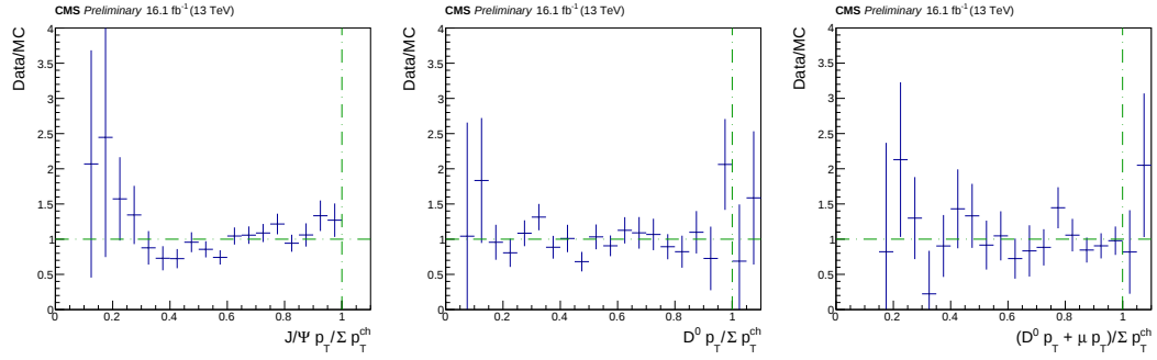
Figure 6.9: Ratio of J/\psi p_T divided by \sum p_T^{\text{ch}} (left), D^0 p_T divided by \sum p_T^{\text{ch}} (center), and ratio of (D^0 p_T + \mu p_T) divided by \sum p_T^{\text{ch}} (right) for data epochs GH
