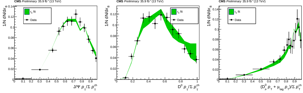
Figure 8.1: J/\psi p_T divided by \sum p_T^{\text{ch}} , D^0 p_T divided by \sum p_T^{\text{ch}} , and (D_\mu^0 p_T + \mu p_T) divided by \sum p_T^{\text{ch}} (bands are the total measurement uncertainties for each sample)
