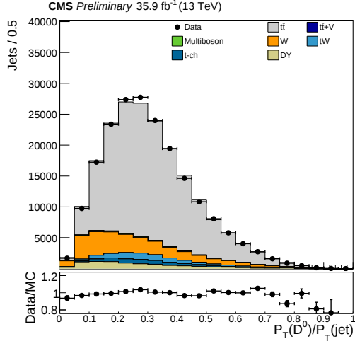
Figure B.1: D^0 p_T divided by full jet p_T
