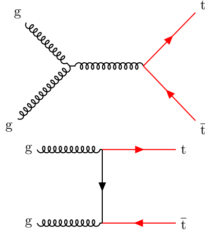
Figure 2.3: Gluon-gluon to t\bar{t} pair production
