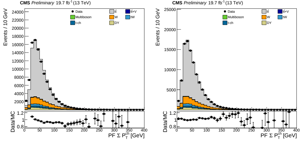
Figure A.3: Effects of the tracker corrections (uncorrected left and corrected right) on the \sum p_T^{ch} for the first half of the data
