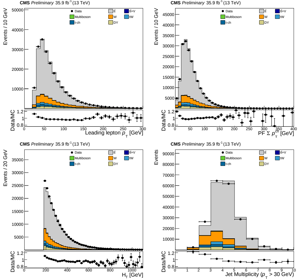
Figure 6.2: ( D^0 selection) All channels isolated lepton p_T (top left) all channels jet \Sigma p_T^{\text{ch}} (top right) all channels H_T (bottom left) and all channels jet multiplicity (bottom right)
