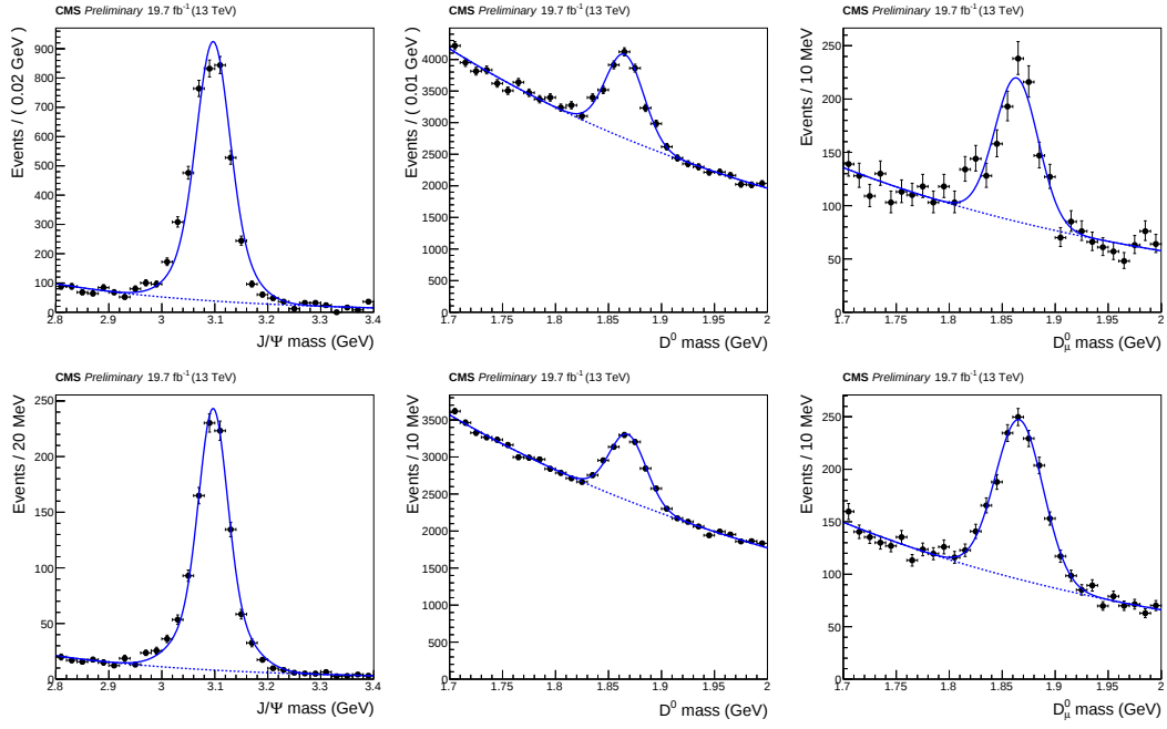
Figure 6.6: Mass fit for the J/\psi (left) D^0 (center) and D_\mu^0 samples (right) for epochs B–F in the Data (top) and MC (bottom)
