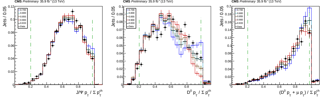
Figure 6.11: J/\psi , D^0 , and D_\mu^0 proxies for r_b = 0.700 , r_b = 0.800 , r_b = 0.855 , r_b = 0.900 , and the combined measurement value (dash-dotted line) compared with data
