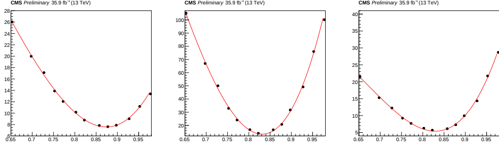
Figure 6.12: \chi^2 goodness-of-fit vs. r_b for J/\psi (left), D^0 (center), and D_\mu^0 (right). The number of degrees of freedom (n.d.f) are 12, 16, and 14 for the J/\psi , D^0 , and D_\mu^0 respectively.
