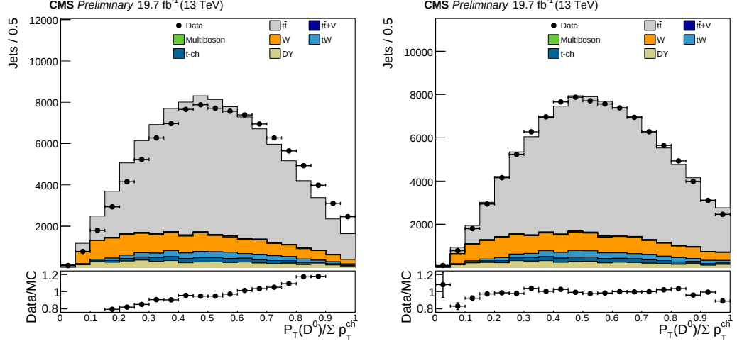
Figure A.1: Effects of the tracker corrections (uncorrected left and corrected right) on the fragmentation proxies D^0 p_T divided by \sum p_T^{\text{ch}} for the first half of the data
