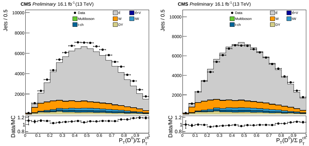
Figure A.2: Effects of the normalization correction (uncorrected left and corrected right) on the fragmentation proxies D^0 p_T divided by \sum p_T^{\text{ch}} for the second half of the data
