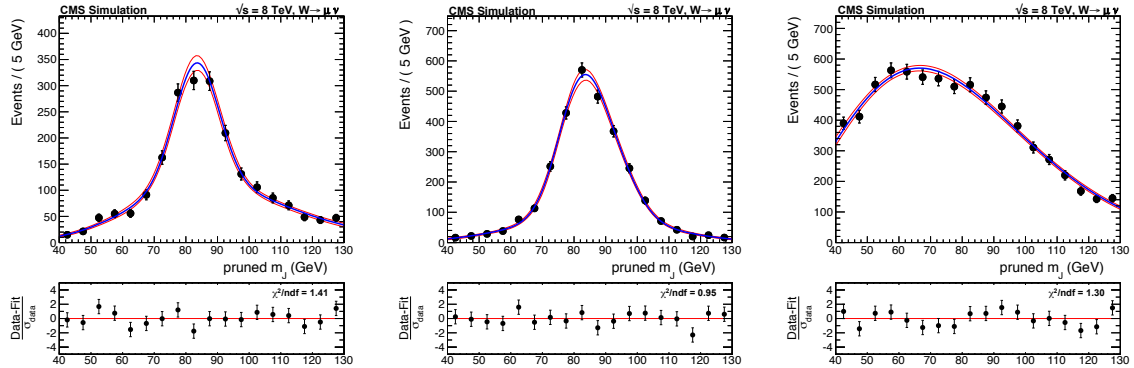
Figure 5.11: Fits to the pruned jet mass spectrum of simulated events with a reconstructed di-boson invariant mass ( m_{\text{WW}} ) in the range 0.55-1.5 TeV for the 0+1-jet \mu\nu +W-jet category. From left to right: t\bar{t} , di-boson (WW/WZ/ZZ) and W+jets ( F_{\text{ErfExp}} ) processes, which are re-weighted applying all the considered data-to-MC corrections, without normalizing them to the luminosity of data sample.
