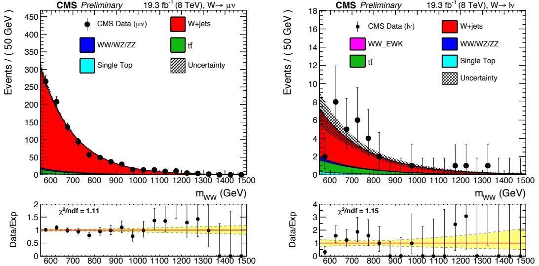
Figure 5.14: The fits for F_{\text{Data,SB}}^{\text{W+jets}}(m_{\text{WW}}) for 0+1-jet \mu\nu +W-jet (left) and 2-jet (right) categories. Minor backgrounds ( t\bar{t} , di-boson and single top) are estimated from simulation, while the W+jets shape is obtained from the fit to the data.
