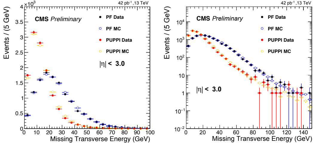
Figure 3.43: E_T^{\text{miss}} distributions as obtained in data and simulation through the PF and the PUPPI algorithms. On the left, distributions are reported in linear scale, while, on the right, in logarithmic one to better compare tail events.
