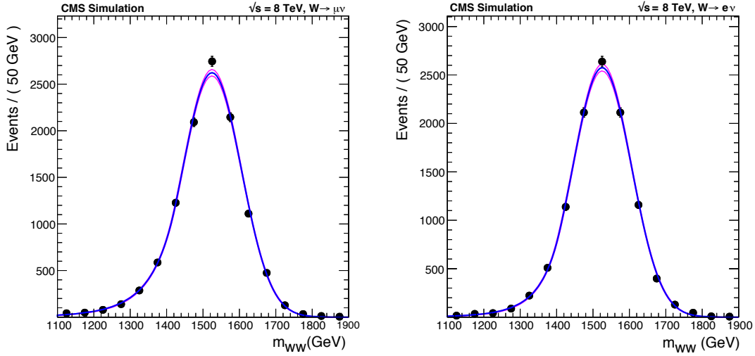
Figure 4.7: Modeling of the reconstructed signal shape with a double-sided Crystal Ball function for Bulk gravitons in the \ell\nu + V\text{-jet} analysis: HP muon category (left), HP electron one (right). In both cases, a Bulk graviton sample with a generated mass m_G = 1.5 TeV is considered.
