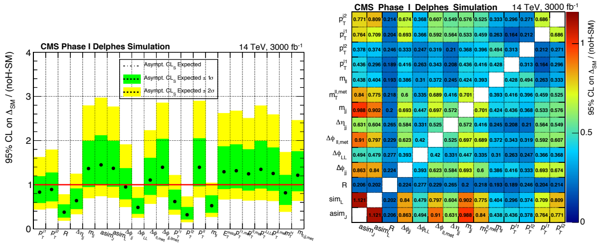
Figure 6.22: Determination of the best observables sensitive to the Higgs-less hypothesis considering the CMS Phase-I detector. Signal and backgrounds yields are normalized to 3 \text{ ab}^{-1} . (Left) Expected 95% CL exclusion limit obtained from single observables, (right) the exclusion limits evaluated for different pairwise combinations. The lowest limit is reached by a two-dimensional fit to R - m_{\ell\ell} .
