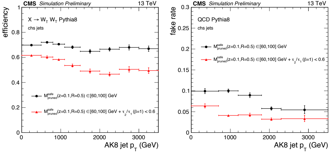
Figure 3.33: (Left) Efficiency of pruned jet mass 60 < m_{\text{pruned}} < 100 \text{ GeV} and N-subjettiness \tau_2/\tau_1 < 0.6 selection on W-jets as a function of p_T , with an average of 40 simulated pileup interactions. (Right) Fake rate for the pruned jet mass and \tau_2/\tau_1 selection on q/g-jets as a function of p_T .
