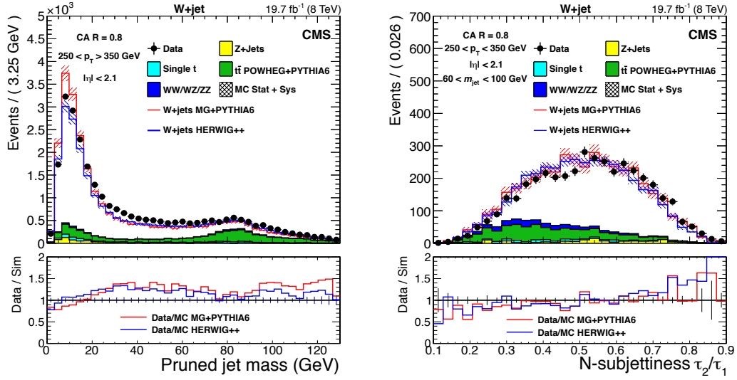
Figure 3.16: Pruned jet mass (left) and N-subjettiness \tau_2/\tau_1 (right) distributions in data and simulation for W+jet events. Below each figure the relative deviations, between data and MC, are reported.
