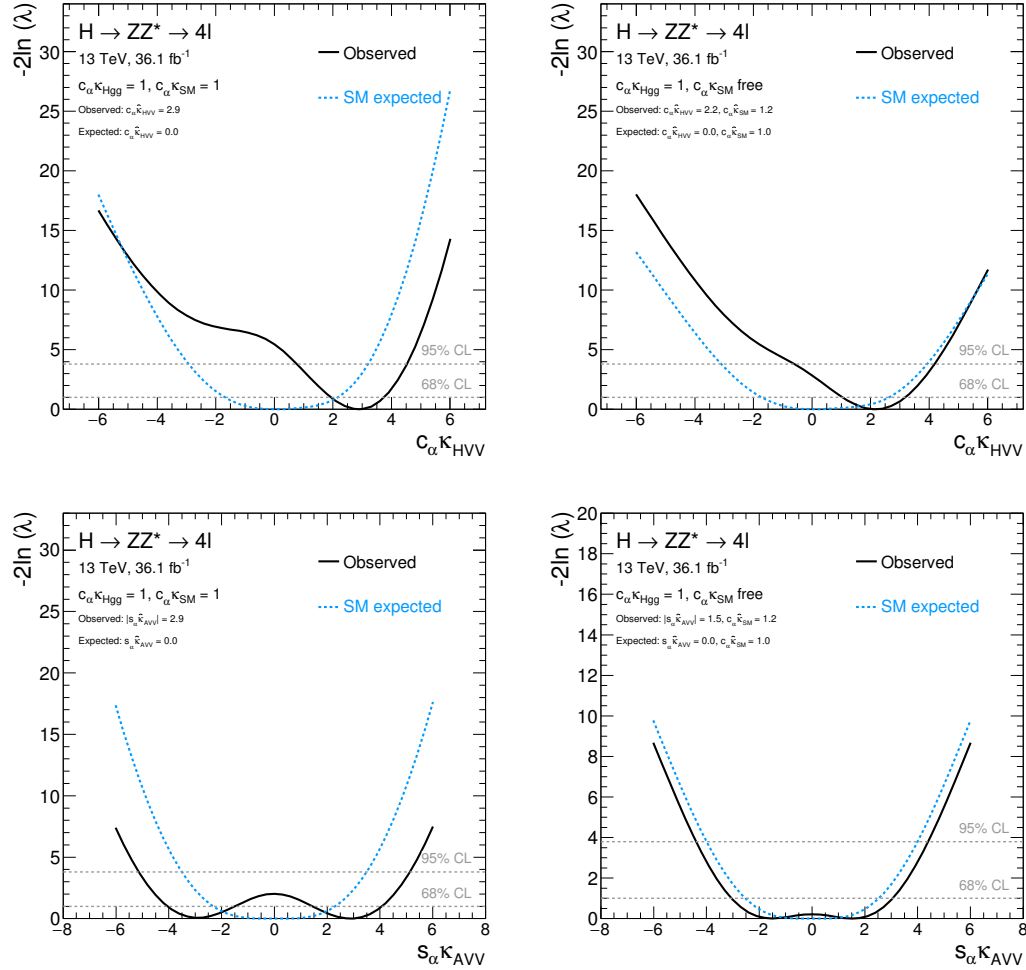
Figure 5.29: Observed (black) and SM expected (blue) dependence of the test statistic on c_\alpha\kappa_{HVV} (top) and s_\alpha\kappa_{AVV} (bottom) coupling parameters for the rate-based analysis of the Run-2 data set. The test statistic distribution is shown with SM coupling parameters fixed to the SM expectation (left) and free (right) in the fit. The horizontal lines indicate the 68 % and 95 % confidence levels assuming a \chi^2 distribution of the profiled likelihood ratio.
