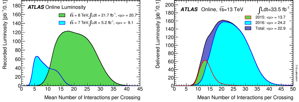
Figure 2.13: Distributions of the mean numbers \mu of inelastic interactions per proton-proton bunch crossing for data taking in 2011 and 2012 (left), and for the runs in 2015 and 2016 (right).
