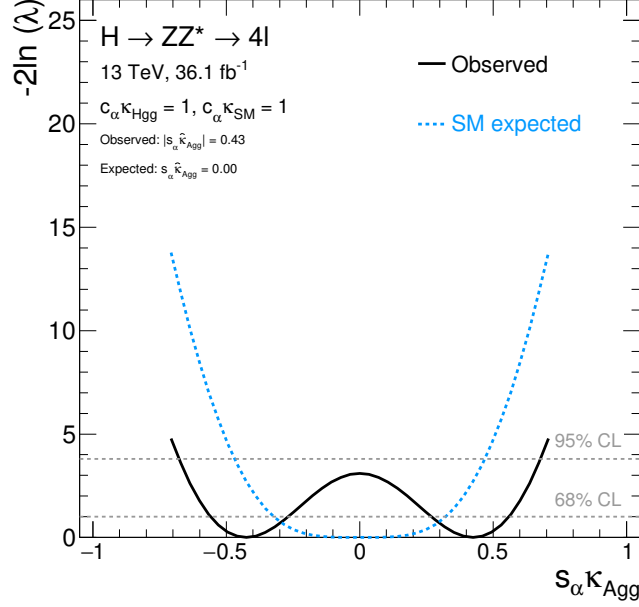
Figure 5.28: Observed (black) and SM expected (blue) dependence of the test statistic on the s_\alpha\kappa_{\text{Agg}} coupling parameter for the rate-based analysis of the Run-2 data set. The horizontal lines indicate the 68 % and 95 % confidence levels assuming a \chi^2 distribution of the profiled likelihood ratio.
