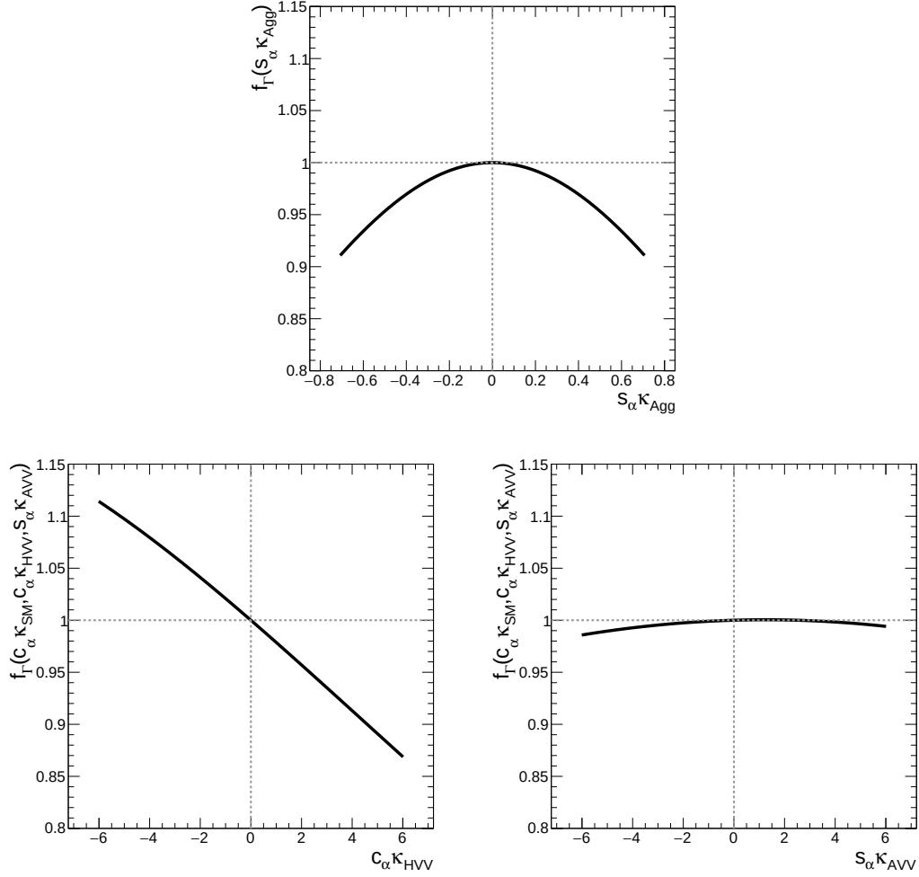
Figure 5.25: The correction factor f_T to the inverse of the width of the Higgs boson as a function of s_\alpha \kappa_{\text{Agg}} (top), c_\alpha \kappa_{\text{HVV}} (bottom left) and s_\alpha \kappa_{\text{AVV}} (bottom right).
