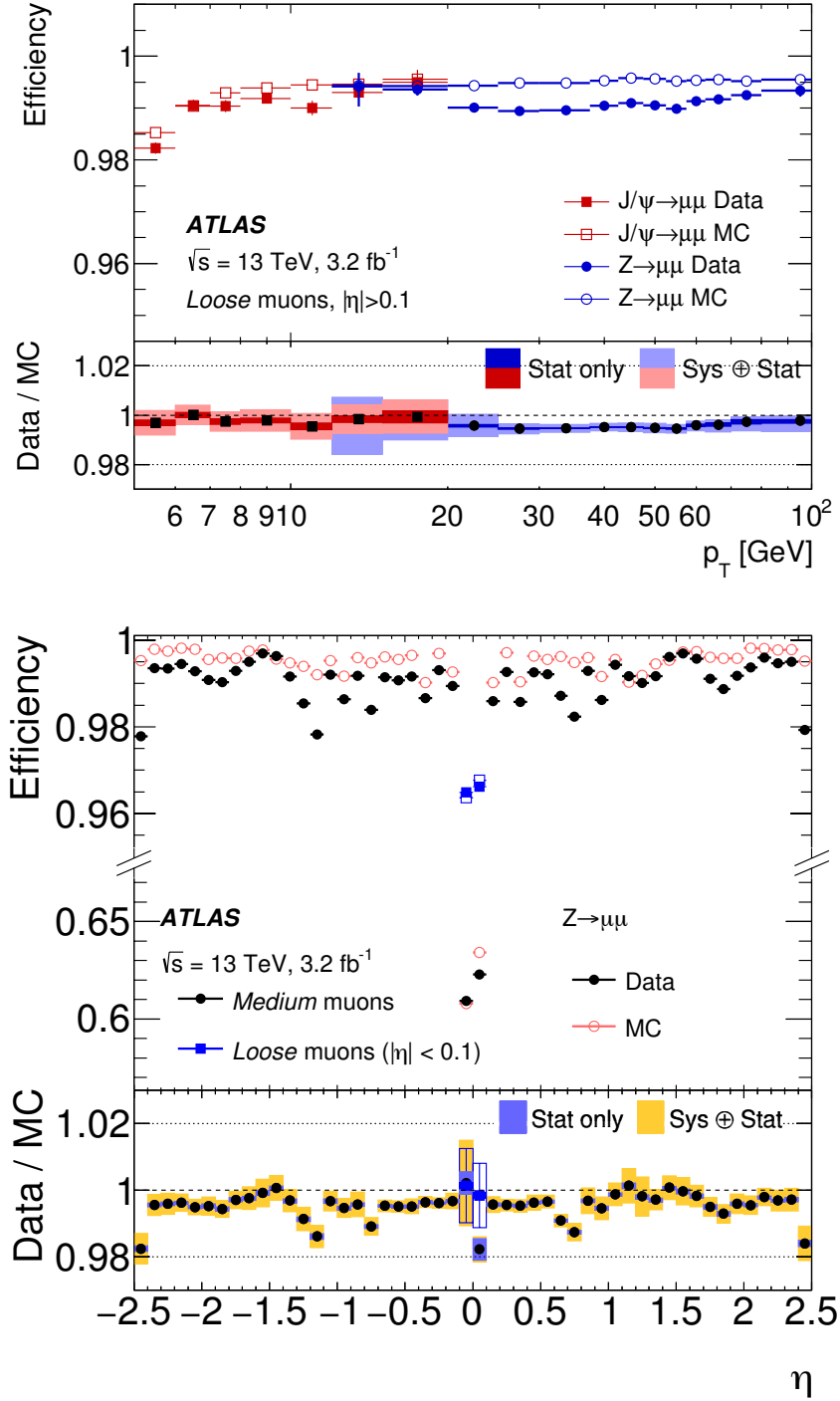
Figure 3.2: Loose and medium muon identification efficiencies as a function of p_T (top) and \eta (bottom) measured with 3.2 \text{ fb}^{-1} of data collected at \sqrt{s} = 13 TeV in 2015 [135]. The lower panels show the ratio of the observed and simulated data.
