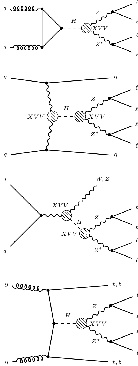
Figure 5.14: From top to bottom: Feynman diagrams of Higgs boson production via ggF , VBF , VH and t\bar{t}H/b\bar{b}H with effective XVV interaction vertices with potential BSM contributions. At the XVV production vertices both W and Z -bosons contribute.
