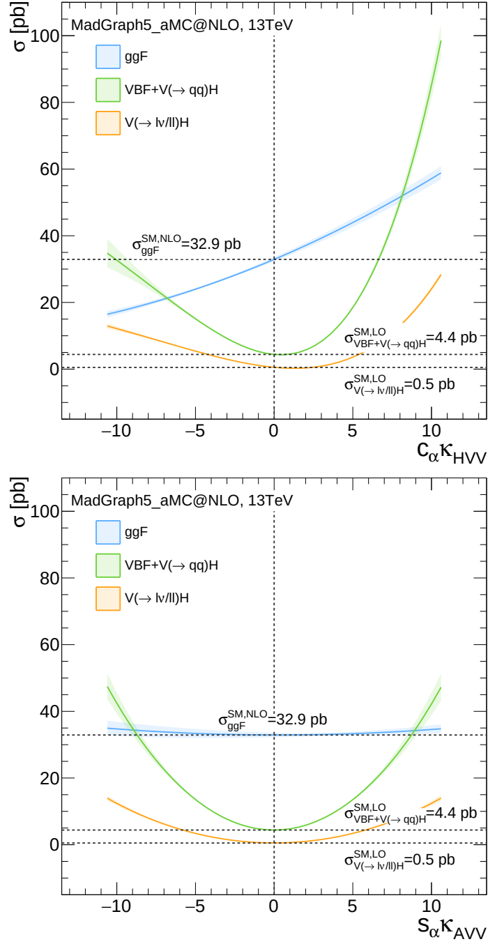
Figure 5.16: The ggF (blue), VBF + V(\rightarrow qq)H (green) and V(\rightarrow \ell\nu/\ell\ell)H Higgs boson production cross sections at \sqrt{s} = 13 TeV calculated at next-to-leading-order (ggF) and leading-order (VBF + V(\rightarrow qq)H and V(\rightarrow \ell\nu/\ell\ell)H ) with MADGRAPH5_AMC@NLO as a function of the CP-even and CP-odd non-SM coupling parameters c_\alpha \kappa_{HVV} (top) and s_\alpha \kappa_{AVV} (bottom), respectively.
