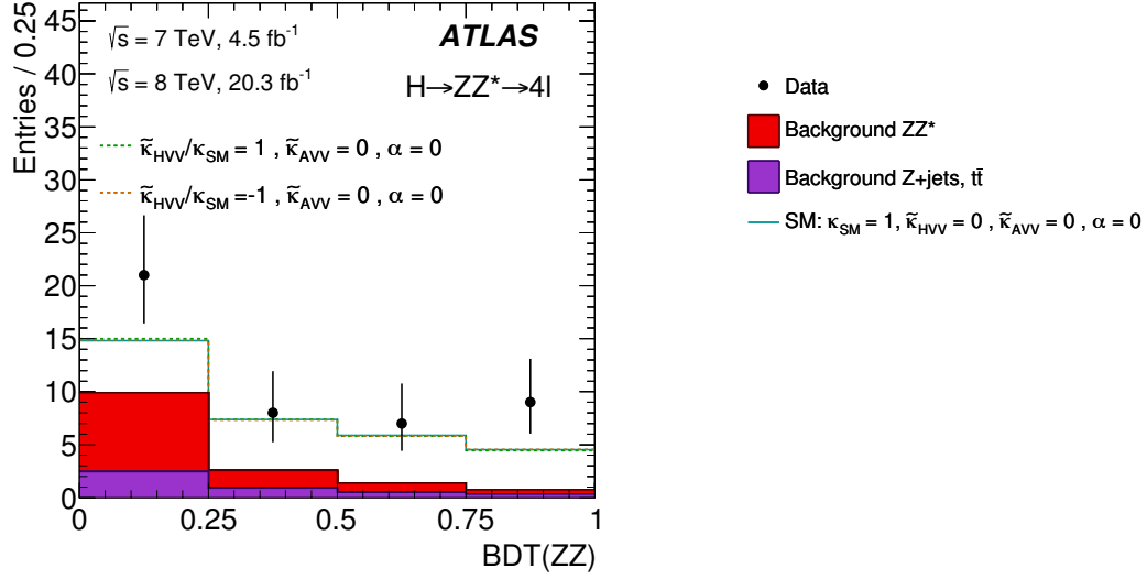
Figure 5.9: The observed and the expected distributions of the BDT(ZZ) discriminant for the Higgs signal and backgrounds in Run-1. The BSM expectations for positive (dotted green) and negative (dotted orange) couplings are shown in addition to the SM expectation (solid green) [14].
