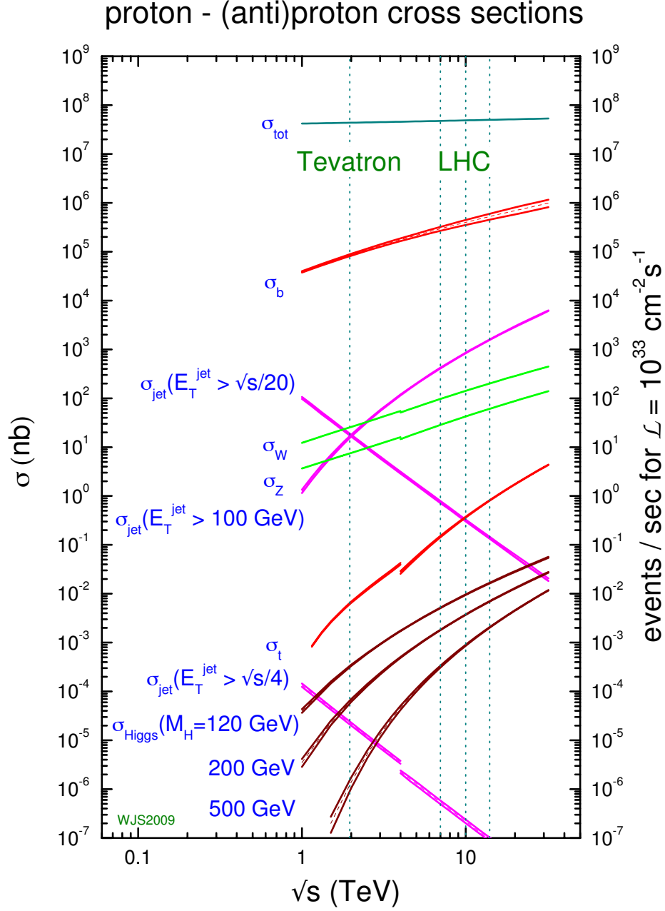
Figure 2.3: Cross sections of selected processes (left y-axis) and corresponding event rates at an instantaneous luminosity of L_{\text{inst}} = 10^{33} \text{ cm}^{-2} \text{ s}^{-1} (right y-axis) as a function of the centre-of-mass energy at hadron colliders [109]. The break in the cross section curves is at the transition from proton-antiproton (at the Tevatron) to proton-proton collisions (at the LHC).
