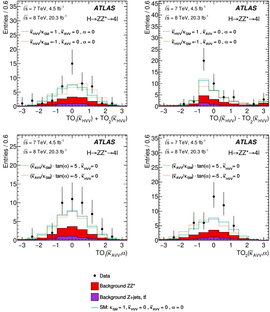
Figure 5.8: Observed and expected distributions of the CP-sensitive observables TO_1(\tilde{\kappa}_{HVV}) + TO_2(\tilde{\kappa}_{HVV}) , TO_1(\tilde{\kappa}_{HVV}) - TO_2(\tilde{\kappa}_{HVV}) , TO_1(\tilde{\kappa}_{AVV}, \alpha) and TO_2(\tilde{\kappa}_{AVV}, \alpha) for the Higgs signal and background in Run-1. The BSM contributions with positive (dotted green) and negative (dotted orange) BSM couplings are shown in addition to the SM signal expectation (solid green) [14].
