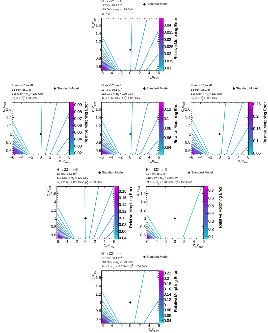
Figure J.6: Contour of the morphing error in the c_\alpha \kappa_{HVV} and c_\alpha \kappa_{SM} plane for the ggF 2D XVV signal model in Run-2 .
