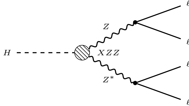
Figure 5.2: Tree-level Feynman diagram of the H \rightarrow ZZ^* \rightarrow 4\ell decay with effective Higgs to Z -boson coupling.
