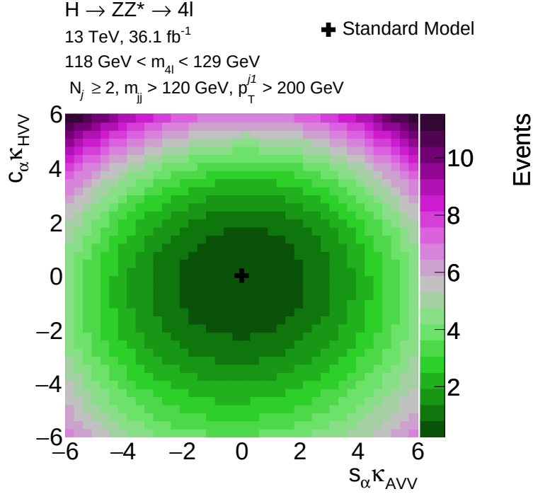
Figure 5.24: The predicted H \rightarrow ZZ^* \rightarrow 4\ell event yield for m_H = 125 GeV in VBF and VH production as a function of the BSM couplings c_\alpha \kappa_{HVV} and s_\alpha \kappa_{AVV} coupling parameters corresponding to the luminosity of the analysed Run-2 data set.
