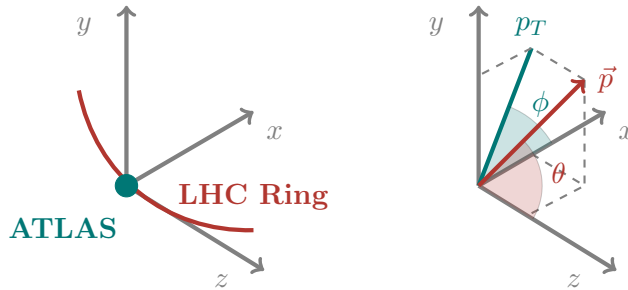
Figure 2.4: Illustration of the ATLAS coordinate system in Cartesian (left) and polar coordinates (right) [110].
