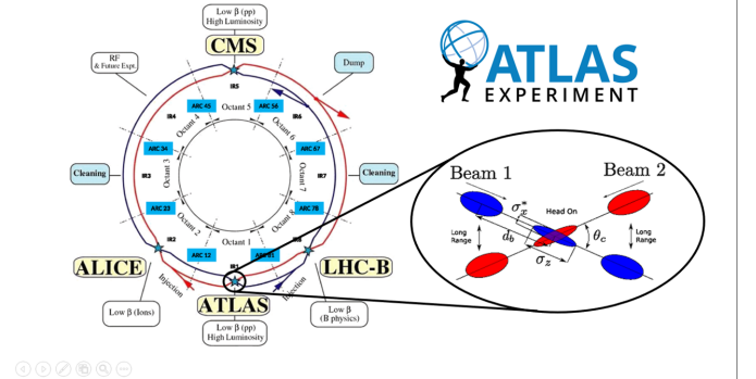
FIG. 2. Schematic layout of the LHC showing the eight insertions of which four house experiments (ATLAS among them), the two counterrotating beams (194 mm separated) and their crossing on these four insertion points. Each beam consists of 10^{11} proton bunches 25 ns separated and focused by strong magnetic fields.
