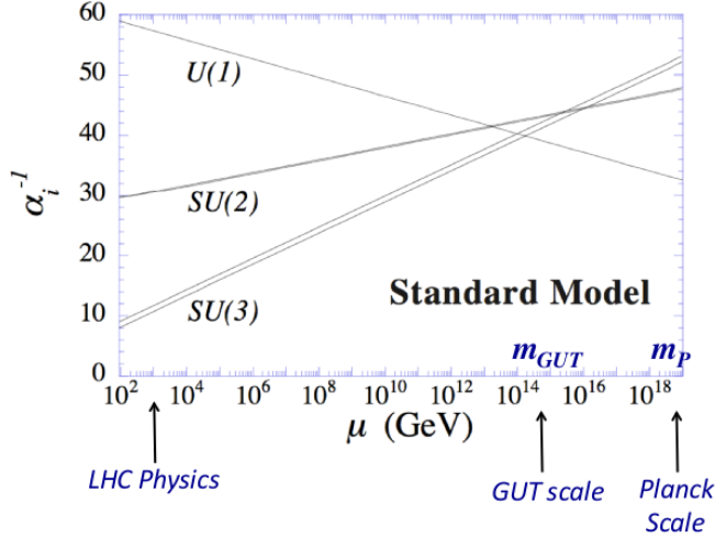
Figure 1: Evolution of the inverse of the coupling constants with the energy
