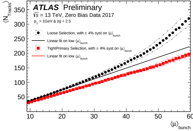
Figure 70: Average number of charged particle tracks that pass a preselection of p_T > 1 GeV and |\eta| < 2.5 reconstructed per event in the ATLAS Inner Detector as a function of \langle\mu\rangle_{\text{bunch}} , for the Loose and TightPrimary track selections. The solid lines show a linear fit to the data in the region 9 < \langle\mu\rangle_{\text{bunch}} < 16 , and extended to higher \langle\mu\rangle_{\text{bunch}} . From ref. [140].
