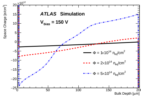
Figure 57: Simulation of the space charge density profile for ATLAS planar pixel modules along the z axis. From ref. [98].
