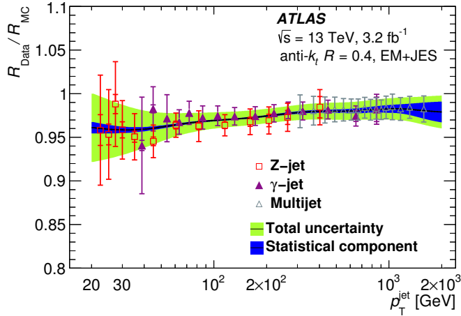
Figure 76: Ratio of the EM+JES jet response in data to that in the nominal MC event generator as a function of jet p_{\text{T}} for Z -jet, \gamma -jet, and multijet in situ calibrations. The final derived correction (black line) and its statistical (dark blue) and total (light green) uncertainty bands are also shown. From ref [149]
