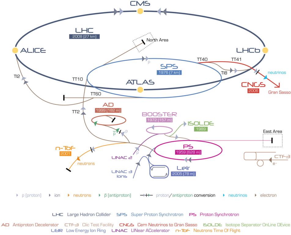
Figure 21: Chain of accelerating facilities at CERN and most important ant experiments
