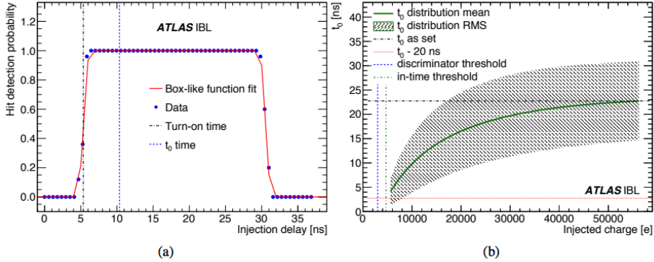
Figure 38: (a) Single pixel hit detection probability for one pixel during t_0 scan with injected charge of 10\text{ ke}^- . (b) distribution of the measured t_0 as a function of the injected charge for an entire chip. Solid line is the average of all measurement and shaded area is the RMS of the t_0 obtained. From ref. [94].
