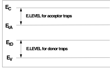
Figure 55: Energy band and trapping levels for acceptor and donor.
