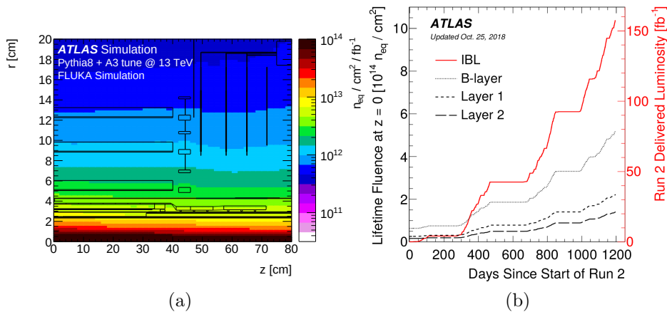
Figure 50: (a) Simulated 1 MeV n_{eq} fluence prediction in the Pixel detector as a function of r and z position using FLUKA for 1 fb -1 . The position of the detector elements are overlaid on the figure. (b) Predictions for the lifetime fluence experienced by the four layers of the current ATLAS pixel detector as a function of time since the start of Run 2 (June 3, 2015) at z \sim 0 up to the end of 2017. For the IBL, the lifetime fluence is only due to Run 2 and for the other layers, the fluence includes all of Run 1. The IBL curve represents both the fluence on the IBL (left axis) as well as the delivered integrated luminosity in Run 2 (right axis). (a) from ref. [116], (b) from ref. [117].
