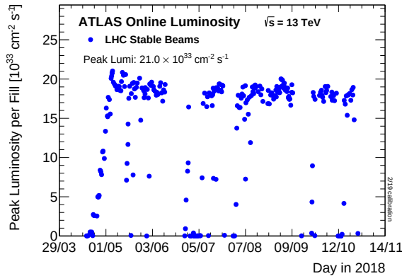
Figure 20: Peak Luminosity measured by ATLAS detector as a function of time.
