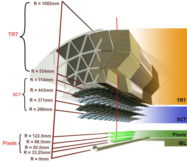
Figure 23: Cut-away view of Inner Detector
