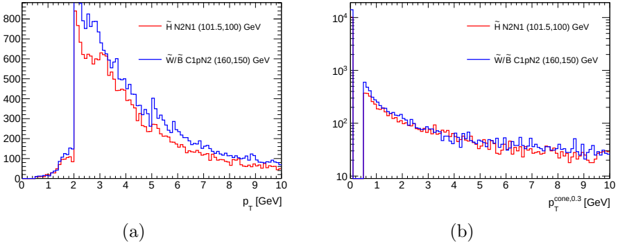
Figure 137: (a) p_T and (b) p_T^{cone=0.3} distribution for two signal points for baseline objects of events in the container.
