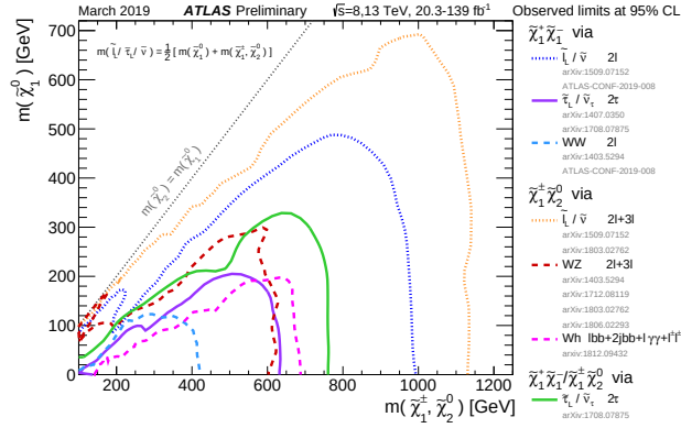
Figure 15: Exclusion limits at 95% CL are shown in the \tilde{\chi}_1^0 - (\tilde{\chi}_1^\pm, \tilde{\chi}_2^0) mass plane for \tilde{\chi}_1^+ \tilde{\chi}_1^- and \tilde{\chi}_1^\pm \tilde{\chi}_2^0 production with either SM-boson-mediated or \tilde{\ell} -mediated decays. The production cross-section is for pure wino \tilde{\chi}_1^+ \tilde{\chi}_1^- and \tilde{\chi}_1^\pm \tilde{\chi}_2^0 . Each individual exclusion contour represents a union of the excluded regions of one or more analyses. From ref [52]
