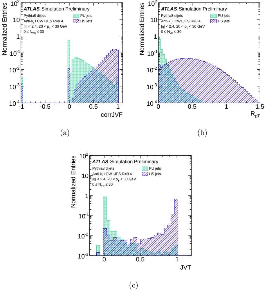
Figure 79: Distribution of (a) \text{corrJVF} , (b) R_{pT} , and (c) \text{JVT} for pileup and hard-scatter jets with 20 < p_T < 30 GeV. From [157].
