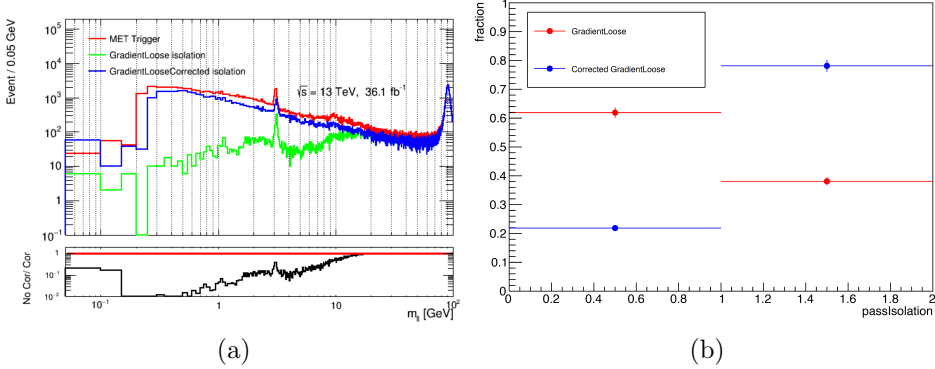
Figure 98: (a) m_{\ell\ell} spectrum for data passing the inclusive E_T^{\text{miss}} trigger and with |\Delta\phi(j_1, \mathbf{p}_T^{\text{miss}})| < 1.5 (to avoid signal contamination). The red line shows events with two baseline leptons without any requirement on isolation, the green line shows events with two baseline leptons passing the GradientLoose isolation WP, and the blue line instead shows events with two baseline events passing GradientLoose isolation WP corrected with the NearbyLepIsoCorrection tool. (b) shows the fraction of events with two baseline leptons passing the GradientLoose isolation WP, while blue dots for the corrected GradientLoose isolation WP, for a signal samples with \Delta m(\tilde{\chi}_2^0, \tilde{\chi}_1^0) = 3 GeV.
