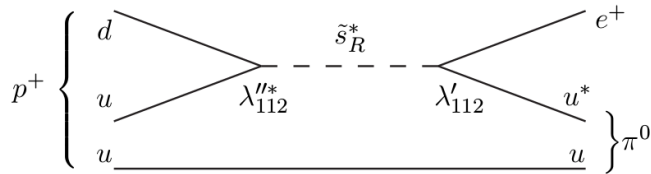
Figure 5: Squark mediated proton decay p \rightarrow e^+ + \pi^0
