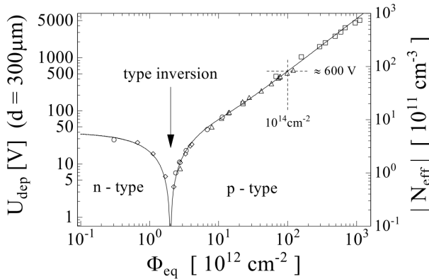
Figure 48: Evolution of the depletion voltage for a 300 \mu\text{m} thick silicon sensor as a function of the fluence. From [104].
