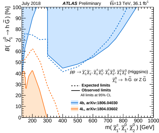
Figure 16: The 95% CL exclusion limits on a general gauge mediation model from \sqrt{s} = 13 TeV data. The model assumes a pure Higgsino NLSP that promptly decays to either Z gravitino or Higgs gravitino. The limits are displayed as a function of the mass of the nearly mass-degenerate Higgsino triplet and the branching fraction of lightest Higgsino to Higgs gravitino. From ref. [52].
