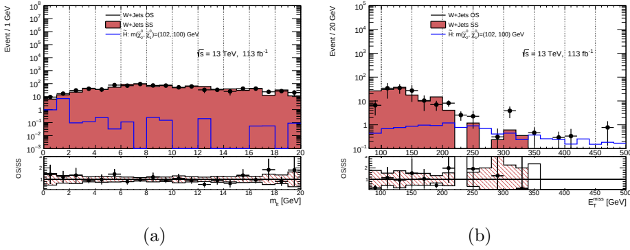
Figure 168: OS/SS ratio as a function of m_{\ell\ell} (left, E_T^{\text{miss}} > 180 \text{ GeV} ) and E_T^{\text{miss}} (right, for m_{\ell\ell} < 2 \text{ GeV} )
