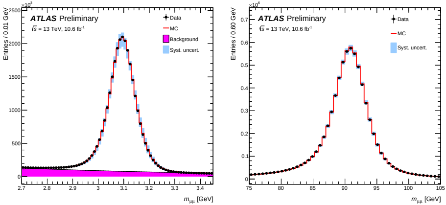
Figure 88: Invariant mass of the \mu^+\mu^- couple for the J/\psi and the Z . From ref. [170].
