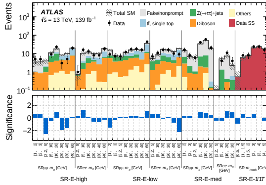
Figure 172: Expected and observed yields in all the 2\ell channels and in the one lepton + one track selection
