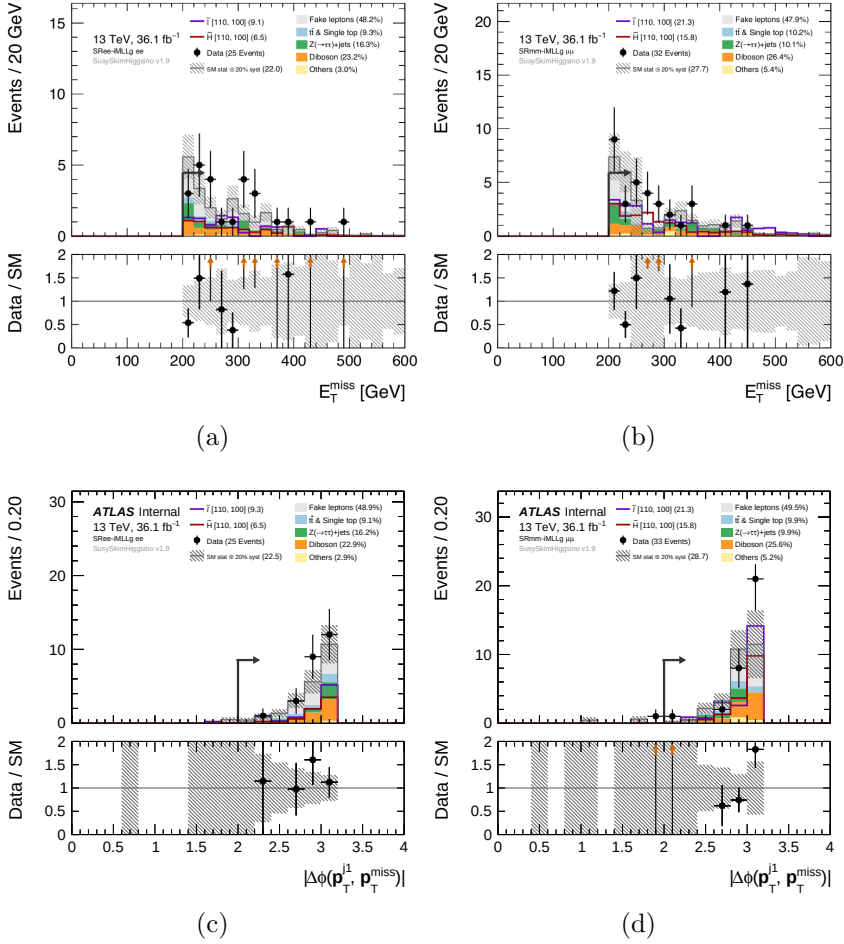
Figure 103: N-1 plot in SR-iMLLg ( ee and \mu\mu ) for (a) E_T^{\text{miss}} ( ee ), (b) E_T^{\text{miss}} ( \mu\mu ), (c) |\Delta\phi(j_1, \mathbf{p}_T^{\text{miss}})| ( ee ), and (d) |\Delta\phi(j_1, \mathbf{p}_T^{\text{miss}})| ( \mu\mu ).
