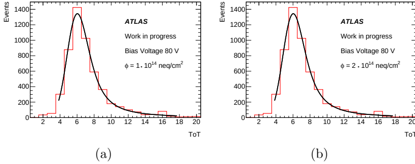
Figure 64: Distribution of the IBL pixels cluster ToT for (a) fluence of 1 \times 10^{14} n_{eq}/\text{cm}^2 and (b) 2 \times 10^{14} n_{eq}/\text{cm}^2 , both with a bias voltage of 80 V. Distribution are fitted with a Landau curve.
