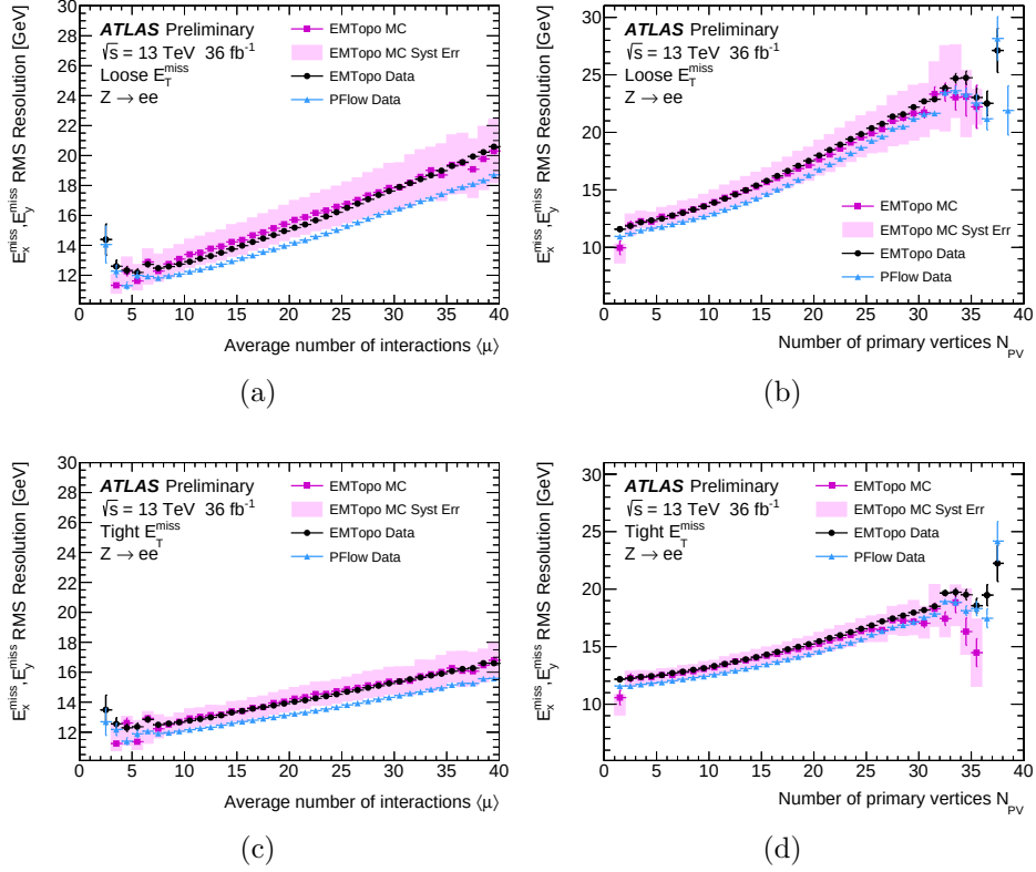
Figure 92: The RMS obtained from the combined distributions of EMTopo E_x^{\text{miss}} and E_y^{\text{miss}} using the Loose E_T^{\text{miss}} (top) and Tight E_T^{\text{miss}} (bottom) operating point for data and MC simulation in Z \rightarrow ee events as a function of (a)/(c) \langle\mu\rangle and (b)/(d) N_{PV} . From ref. [172].
