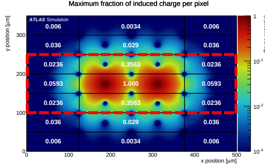
Figure 62: Ramo potential maps of a ATLAS IBL 3D module. Numbers indicate the maximum induced charge (normalized to one). Blue holes are the p^+ columns. The red dashed lines illustrate which pixel are put in the simulations. From ref. [98].
