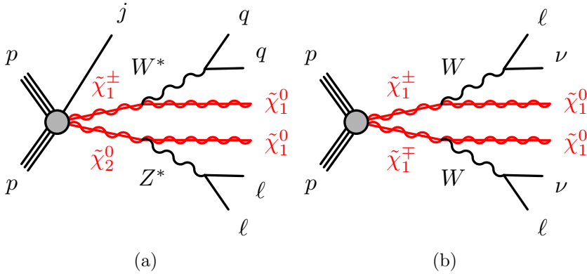
Figure 94: Diagram of the production of (a) pp \rightarrow \tilde{\chi}_2^0 \tilde{\chi}_1^\pm decaying in llj\tilde{\chi}^0\tilde{\chi}^0q\bar{q} and (b) pp \rightarrow \tilde{\chi}_1^+ \tilde{\chi}_1^- decaying in l\nu l\nu j\tilde{\chi}^0\tilde{\chi}^0 .
