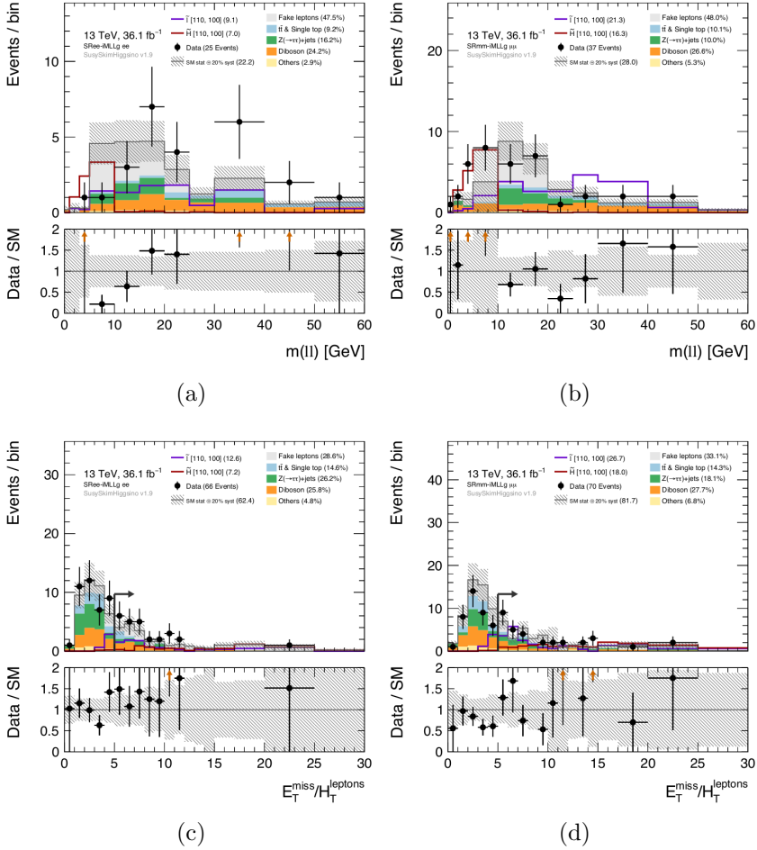
Figure 102: N - 1 plot in SR-iMLLg ( ee and \mu\mu ) for (a) m_{\ell\ell} ( ee ), (b) m_{\ell\ell} ( \mu\mu ), (c) E_T^{\text{miss}}/H_T^{\text{leptons}} ( ee ), and (d) E_T^{\text{miss}}/H_T^{\text{leptons}} ( \mu\mu ).
