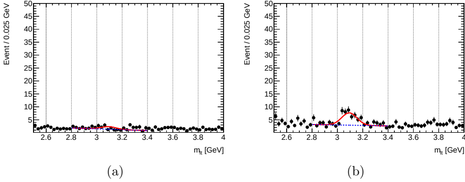
Figure 147: m_{\ell t} distributions for t\bar{t} MC events passing 1 lepton trigger and with 1 lepton and 1 track with a match to an (a) electron or (b) muon container.
