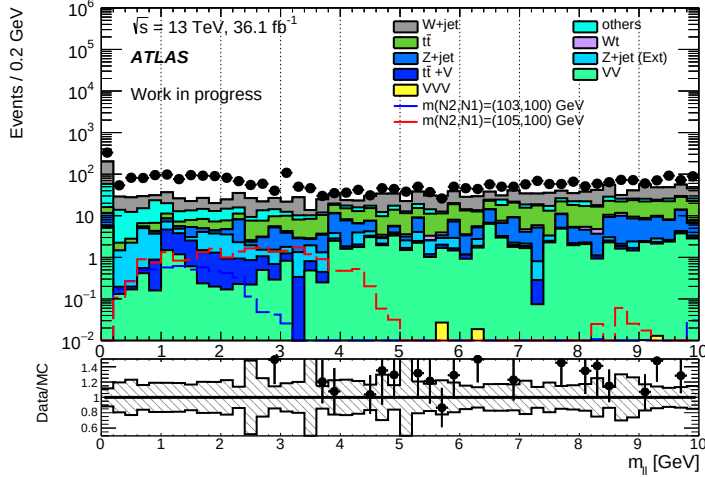
Figure 114: m_{\ell\ell} distribution in CR_{l_{Emiss}} , with no isolation applied. This figure shows that there is an excess of data with respect of MC outside of the Drell-Yan, and this difference is exactly what is measured by this ABCD method.
