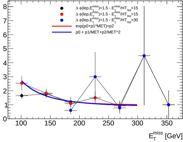
Figure 167: OS/SS ratio as a function of E_T^{\text{miss}} for m_{\ell t} < 2 GeV, with the following selections: |\Delta\phi(\ell\ell, \mathbf{p}_T^{\text{miss}})| < 1.5 , E_T^{\text{miss}}/H_T^{\text{lep+trk}} > 15 , E_T^{\text{miss}} < 180 GeV (black), |\Delta\phi(\ell\ell, \mathbf{p}_T^{\text{miss}})| > 1.5 and E_T^{\text{miss}}/H_T^{\text{lep+trk}} > 15 (red), and |\Delta\phi(\ell\ell, \mathbf{p}_T^{\text{miss}})| > 1.5 and E_T^{\text{miss}}/H_T^{\text{lep+trk}} > 30 (blue). The red and blue lines are, respectively, an exponential and a polynomial fit of the red data points.
