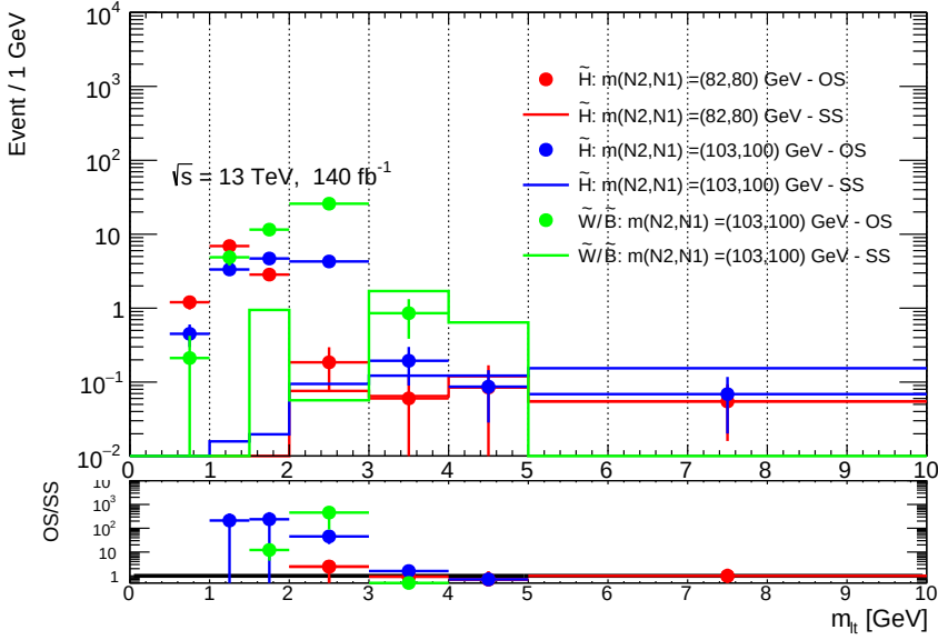
Figure 161: OS and SS events m_{\ell\ell} distribution for signal samples in the SR. The bottom box shows the OS/SS ratio.
