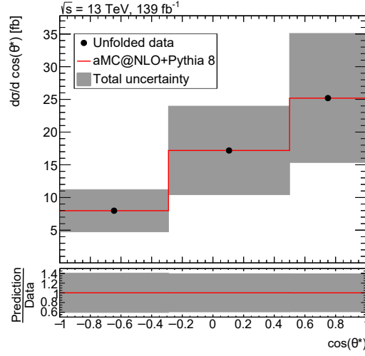
Figure 7.10: Unfolded reco-distribution as data points compared to truth-distribution in red. A regularisation of strength \tau = 2.5 is applied. The ratio between the shown distributions is exactly one as without the regularisation.
