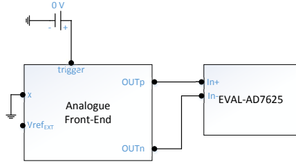
Figure 10.1 – Test Setup for Noise Measurement
