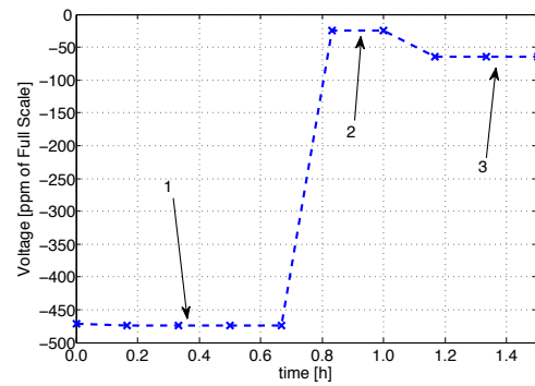
Figure 9.11 – Power-up
