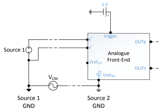
Figure 10.13 – Ground Loop Between Two Far Grounds
