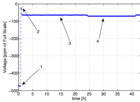
Figure 9.10 – Overall Measurement
