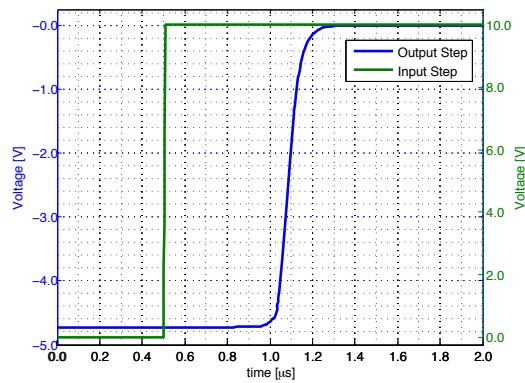
Figure 5.4 – Response to 10 V – 10 ns step (Input Step in Green, Output Step in Blue)
