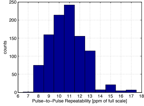
Figure 10.18 – Pulse-to-Pulse Repeatability in nominal working conditions
