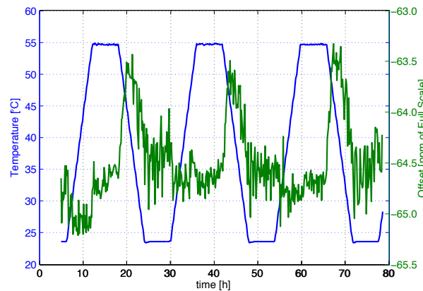
Figure 9.14 – Offset Variations (right-hand scale in green) Due to a 5 °C/h Temperature Profile (left-hand scale in blue)
