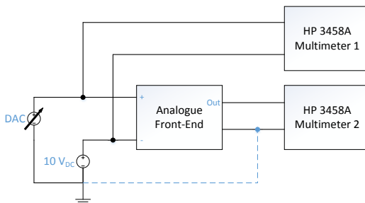
Figure 8.5 – Linearity Setup
