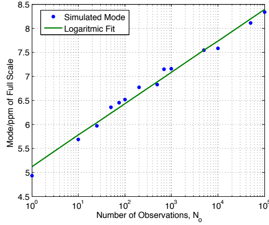
Figure 4.4 – Mode of WCR versus N_o , \sigma = 1 ppm of Full Scale
