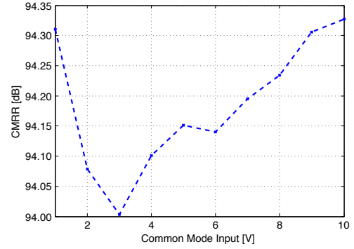
Figure 10.12 – CMRR vs Common-Mode Input Voltage ( 1 - \sigma Uncertainty)
