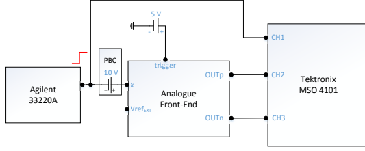
Figure 10.7 – Test Setup for Delay Measurement
