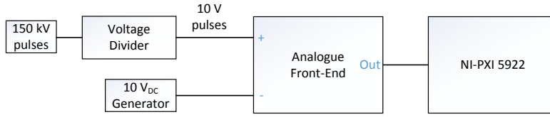
Figure 4.1 – Reference Acquisition System Block Diagram.
