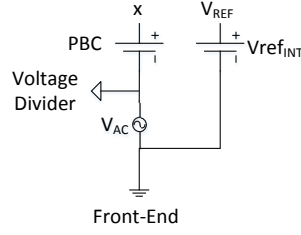
Figure 10.15 – V_{CM} Definition
