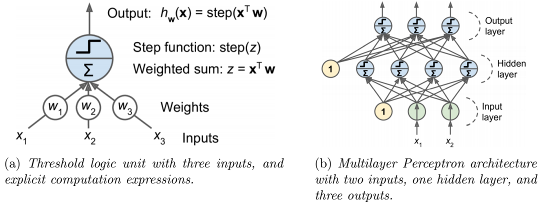
Figure 3.2: Schematic representation of Perceptron and Multilayer Perceptron, reproduced from Ref. [35].
