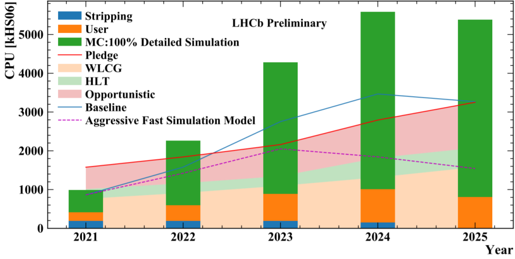
Figure 2.1: Estimated CPU usage for the LHCb experiment from 2021 through 2025. The bars give the total CPU usage expected, composed of stripping jobs (blue), all estimated user jobs (orange) and simulation production (green). The green bars here assume only fully detailed simulation to be run. CPU usage is also considered under different scenarios: the baseline scenario (light blue line) uses a 40%/40%/20% split between full, fast and ultra-fast simulations, while the aggressive scenario (dashed purple line) increases to 30%/50%/20% the fast simulation usage. These two trends are compared to the computing resources available, represented by the pledge (red line). Reproduced from LHCb-FIGURE-2019-01.
