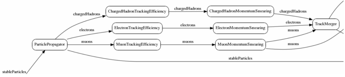
Figure 2.4: Scheme of the DELPHES data flow through the tracking system modules.
