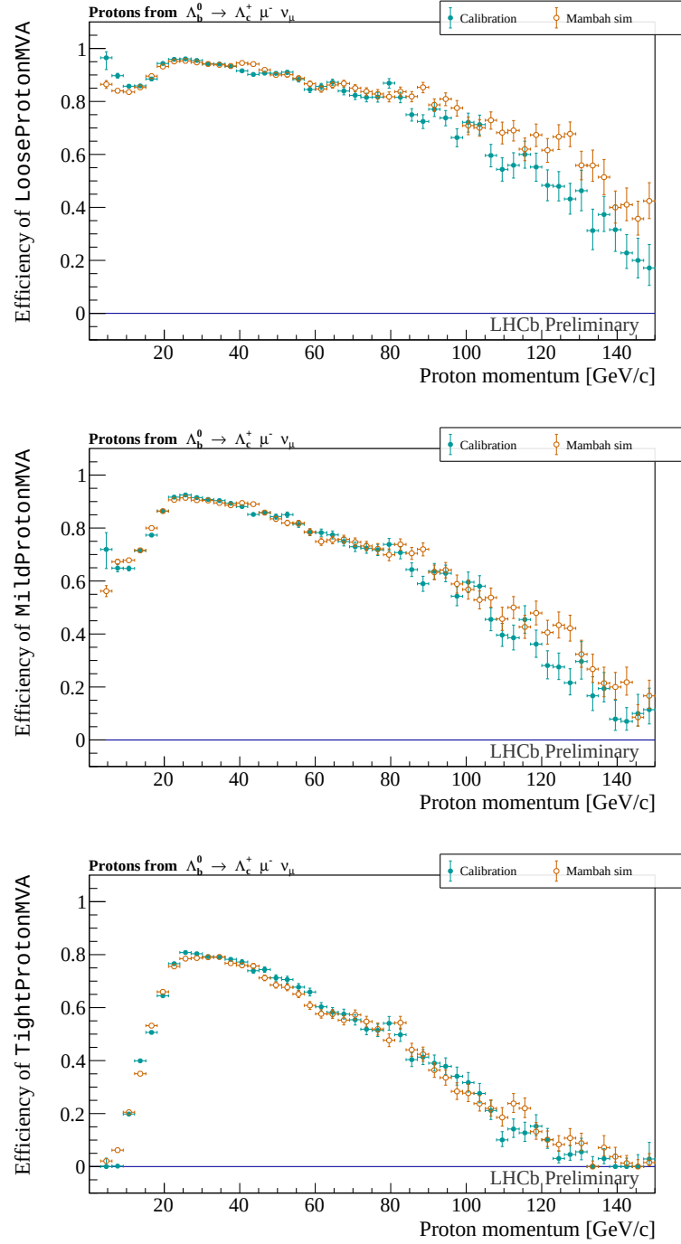
Figure 5.15: Performance plots of the mambah.sim Prototype reporting the efficiency of three different requirements on the output of a FNN trained to identify protons (namely ProbNNp ) as evaluated on protons tagged through the decay \Lambda_b^0 \rightarrow \Lambda_c^+ \mu^- \bar{\nu}_\mu with \Lambda_c^+ \rightarrow p K^- \pi^+ . The efficiency is compared, in bins of the proton momentum, for a dataset selected without introducing bias on the particle identification of the proton (cyan shaded area), and an ultra-fast simulation sample where the PID variables are modeled through a Generative Adversarial Network trained using protons from \Lambda^0 \rightarrow p \pi^- decays, only (orange markers).
