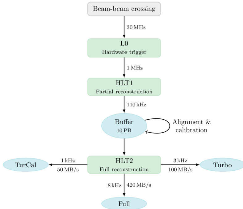
Figure 1.7: An overview of the LHCb trigger scheme in Run 2. The green boxes represent trigger stages, the blue ellipses represent storage units, and arrows between elements represent data flow, labelled with approximate flow rates. Reproduced from Ref. [14].
