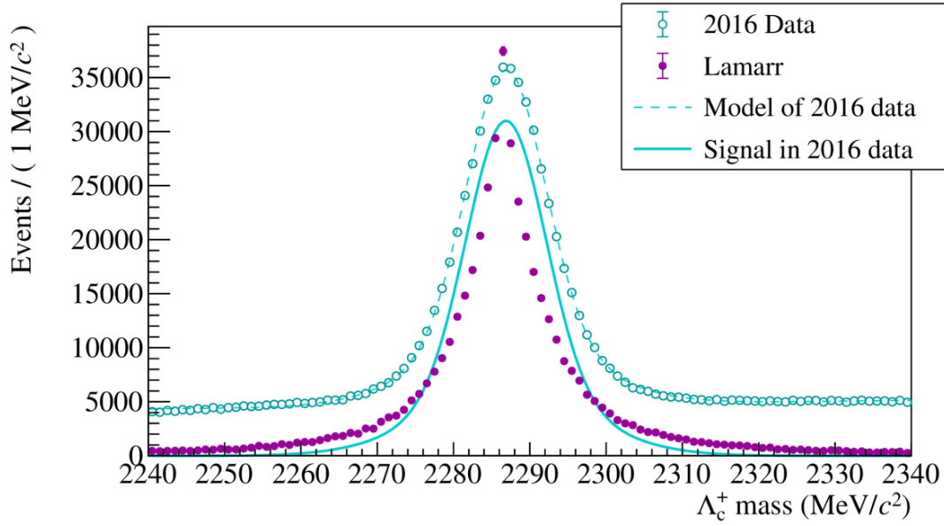
Figure 5.1: Performance plots of the Lamarr Prototype reporting the invariant mass distribution of reconstructed and simulated \Lambda_c^+ baryons produced in the decay \Lambda_b^0 \rightarrow \Lambda_c^+ \mu^- \bar{\nu}_\mu and decays as \Lambda_c^+ \rightarrow p K^- \pi^+ . The data is fitted with a model composed of a double Gaussian function for the signal and a second-order polynomial for the combinatorial background. The shape of the signal peak is compared to the distribution obtained from simulation. Reproduced from LHCb-FIGURE-2019-017.
