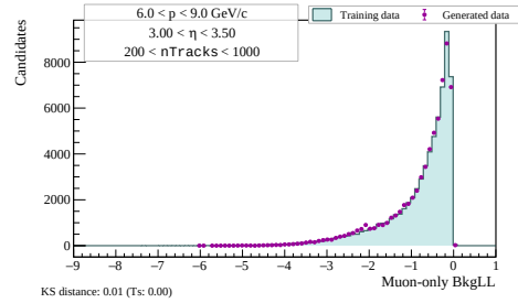
(h) Proton track candidates.
