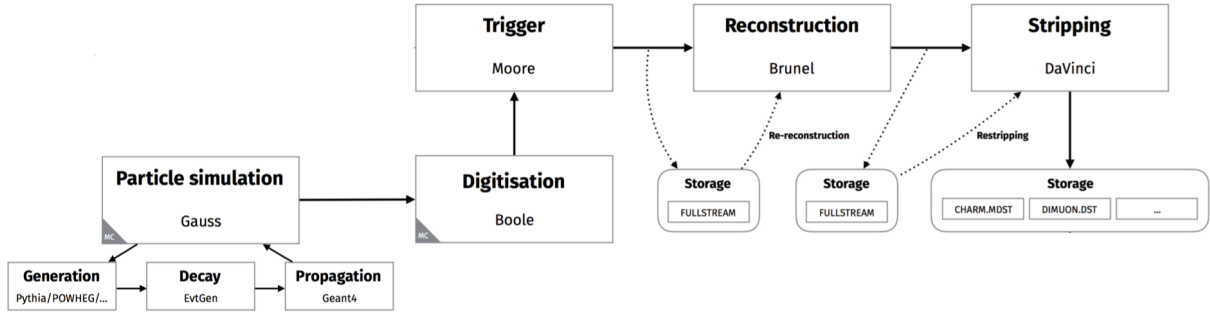
Figure 2.3: The LHCb event simulation flow [16].
