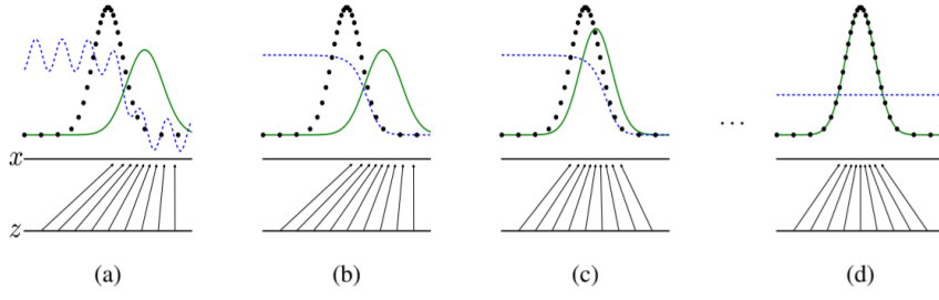
Figure 3.4: GANs are trained by simultaneously updating both of the discriminator D (dashed line in blue) and of the generator G . The goal of D is to distinguish between the data sample (dotted line in black) from the generator one (solid line in green). The lower horizontal lines and the upward arrows represent the latent space \mathcal{Z} and the generator map G : \mathbf{z} \rightarrow \mathbf{x} . In (a) an adversarial pair near convergence is shown, where p_g is similar to p_r , and D is a partially accurate classifier. In the inner loop of the algorithm ( k steps), D is trained to discriminate samples from data, converging to D^* (b). After an update to G , gradient of D has guided the map G to flow to regions that are more likely to be classified as data (c). After a sufficient number of iterations (d), if G and D have enough capacity, they will reach a point at which both cannot improve because p_g = p_r . Here the discriminator is unable to differentiate between the two distributions, and D(\mathbf{x}) = 1/2 . Pedagogical example reproduced from Ref. [43].
