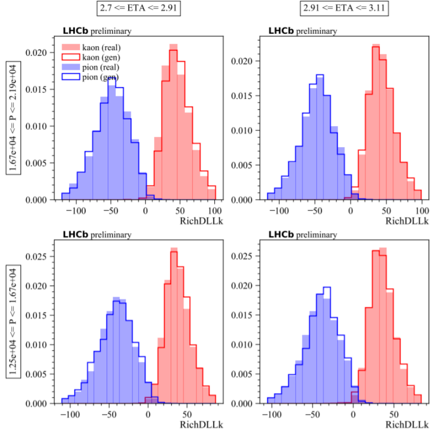
Figure 4.1: Weighted real data and generated distributions of RichDLLk for kaon and pion track candidates in bins of pseudorapidity ( \eta ) and momentum ( P ) in a well-populated phase space region. Histograms reproduced from Ref. [59].
