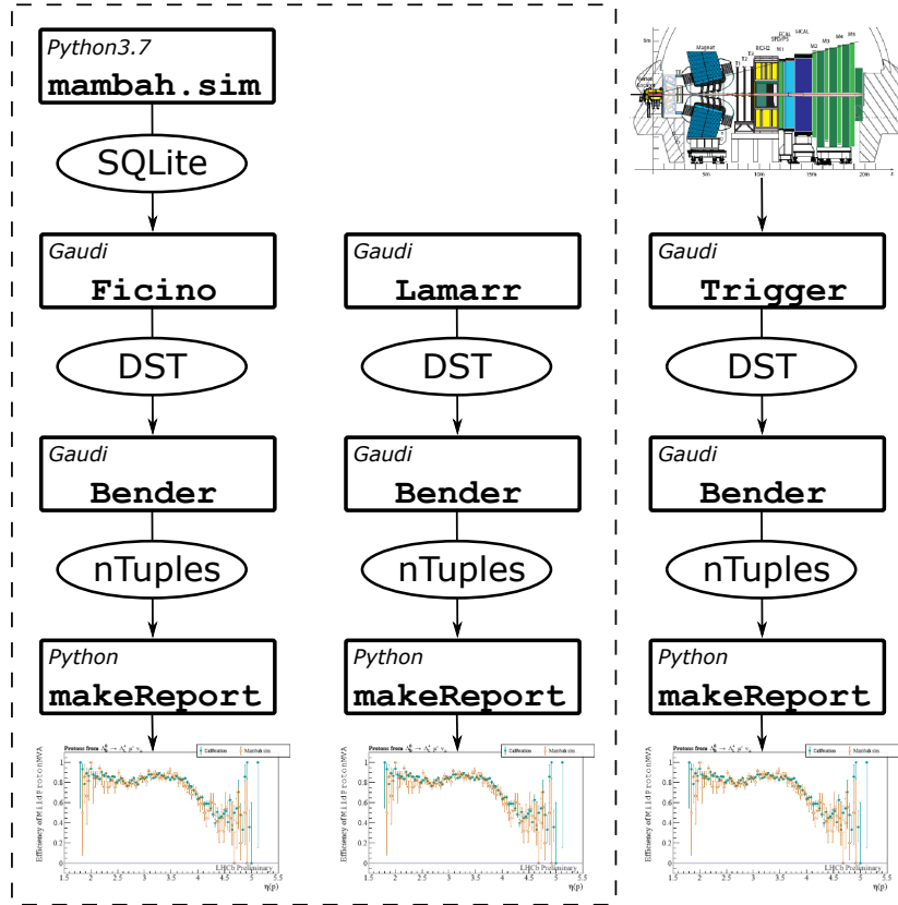
Figure 5.7: Schematic and simplified representation of the dataflows used to obtain the datasets compared in the validation. The left and middle flows represent simulation systems, the right one instead describes the data flow of real physics events.
