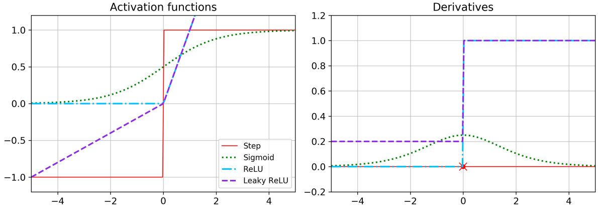
Figure 3.3: Activation functions and their derivatives. The step function shown is \text{sign}(z) , and the Leaky ReLU reported has \alpha = 0.2 .
