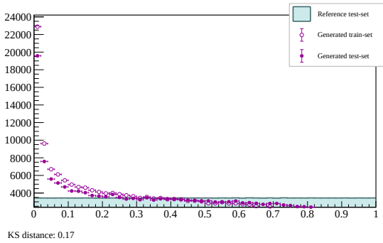
(b) Typical outcome of our Generative Models.
