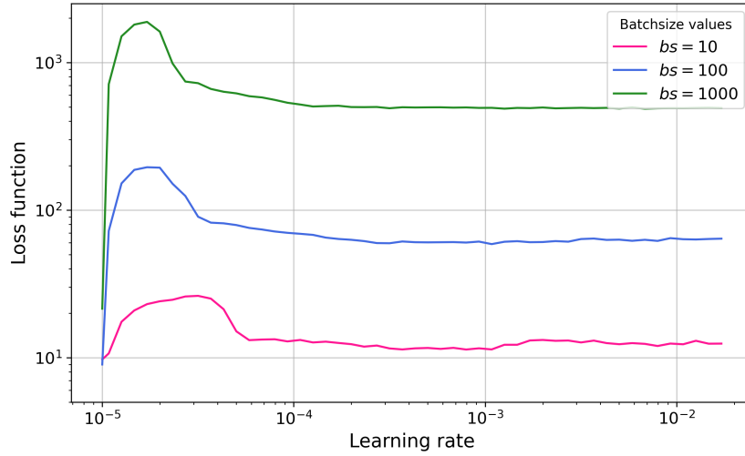
Figure 4.7: Learning rate preliminary study.
