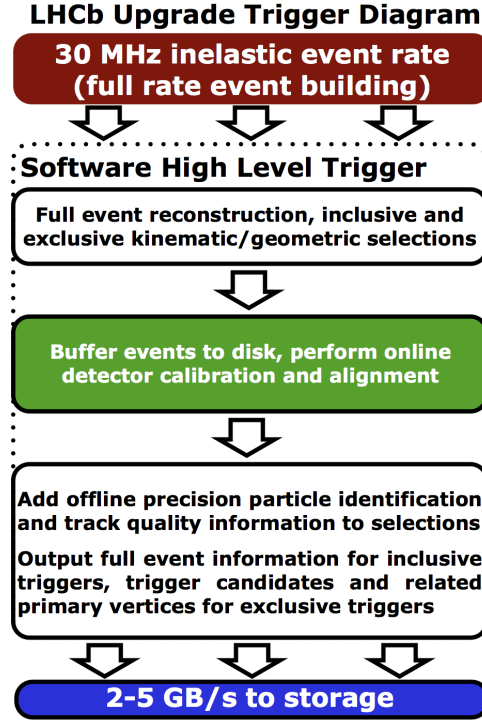
Figure 1.8: Representation of the Run 3 trigger scheme.
