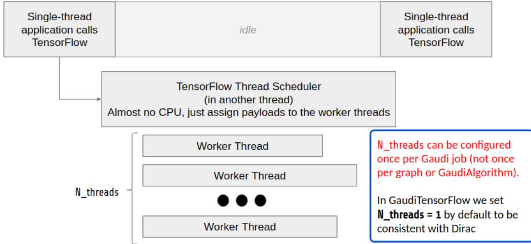
Figure 5.3: Simplified and schematic representation of the interplay between the GAUDI and TensorFlow scheduler when using GaudiTensorFlow.
