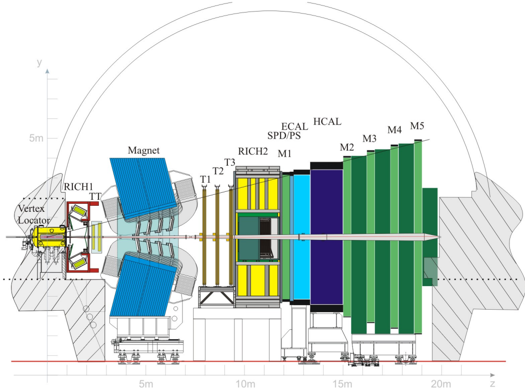
Figure 1.4: View of the LHCb detector.
