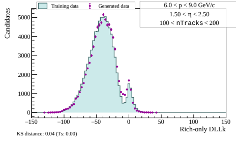
(a) Pion track candidates.
