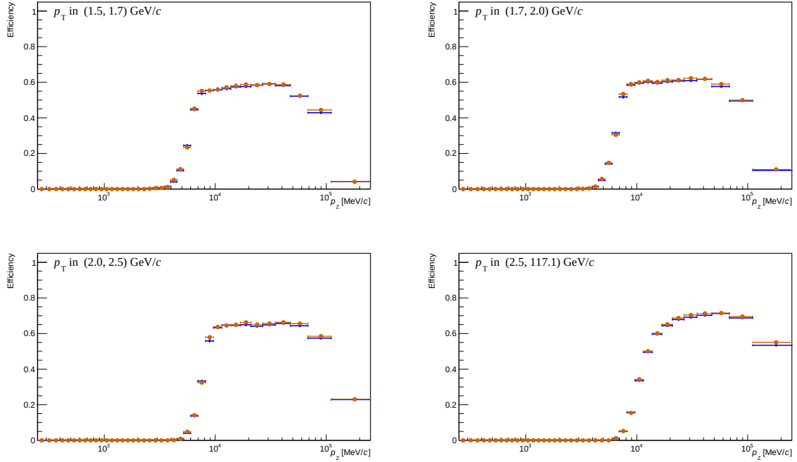
Figure 5.6: Comparison of the efficiency modeled with a deep neural network (represented with orange markers) superposed to the efficiency obtained from full simulation (represented with blue markers). The efficiency is defined here as the ratio between the number of fully reconstructed tracks (from the VELO to the calorimeter) to the number of charged particles generated. The agreement of the projection is exceptionally good.
