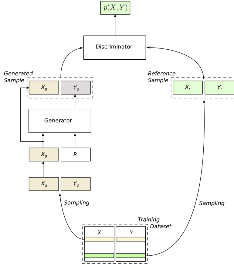
Figure 4.2: Conditional GAN scheme. Here, the discriminator outputs a probability like in the original Goodfellow’s proposal. Anyway, the representation remains valid also in case of conditional Cramér GAN, substituting p(X, Y) with the map h(X, Y) . Finally, notice that latent space elements are denoted with R instead of Z .
