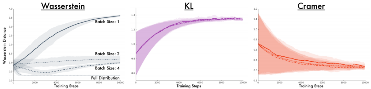
Figure 3.6: Learning curves of three different adversarial models: using Wasserstein distance, Kullback–Leibler divergence and Cramér distance respectively. For the last two, having unbiased sample gradients, the batch size does not prevent from reaching the minimum. Instead, the convergence of Wasserstein distance is heavily conditioned by hyperparameter setting. Plots reported from Ref. [49].
