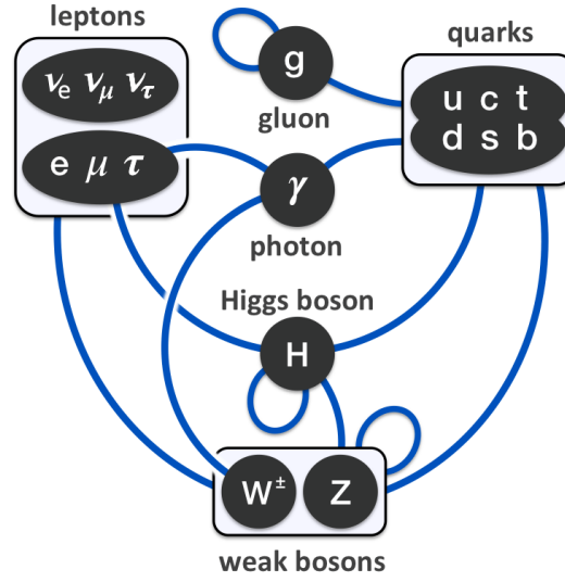
Figure 1.1: Summary of interactions between particles described by the Standard Model. Reproduced from https://en.wikipedia.org/wiki/Standard_Model .
