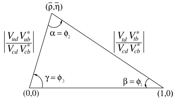
Figure 1.2: Sketch of the unitarity triangle [1].
