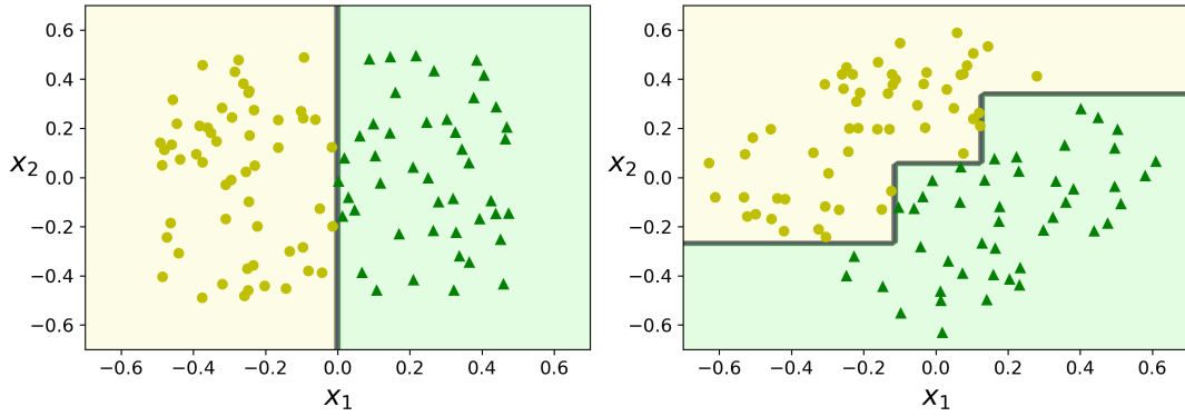
Figure 4.3: Representation of a classification problem faced with Decision Tree algorithm. The feature space is 2-dimensional and composed by x_1 and x_2 . While in the left plot the split is easy, on the right the decision boundary looks unnecessarily convoluted, although the dataset is simply rotated by 45^\circ . Reproduced from Ref. [35].
