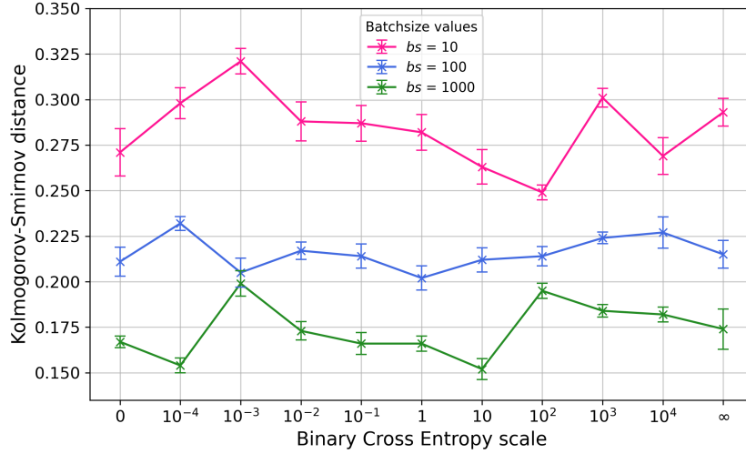
Figure 4.10: Comparison between models trained with a combination of the energy distance and the binary cross-entropy, weighted by the hyperparameter \xi , the binary cross-entropy scale. The results are reported for three different batch-size values ( bs = 10, 100, 1000 ). It should be noticed that the x -axis is not in scale and include the special symbol \infty . The latter denote simply a GAN system based only on a cross-entropy loss.
