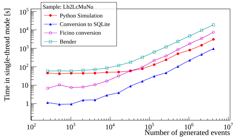
Figure 5.8: CPU time requested by each step of the data-flow when producing the sample of simulated \Lambda_b^0 decays described in text. The number of events on the x -axis is the number of generated events, before any acceptance or efficiency requirement.
