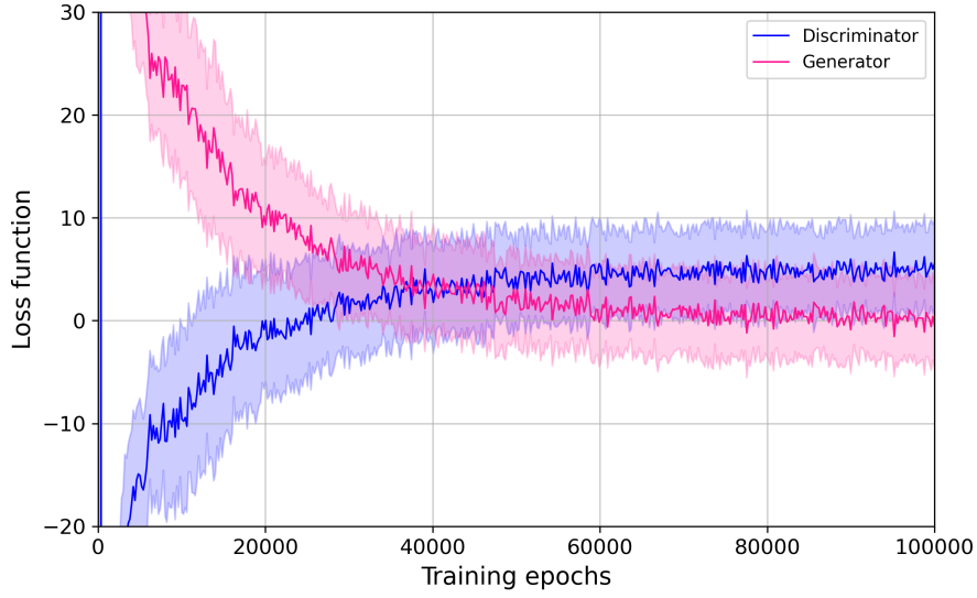
Figure 4.6: Discriminator and generator learning curves.
