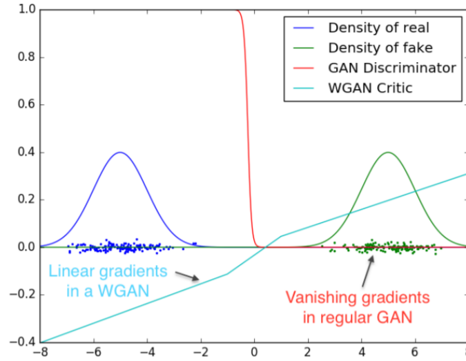
Figure 3.5: Optimal discriminator and critic when learning to distinguish two Gaussians. Here it's clearly shown that the discriminator of original GAN saturates and results in vanishing gradients. On the other hand, WGAN critic is able to provide very clean gradients on all parts of the space. Reproduced from Ref. [47].
