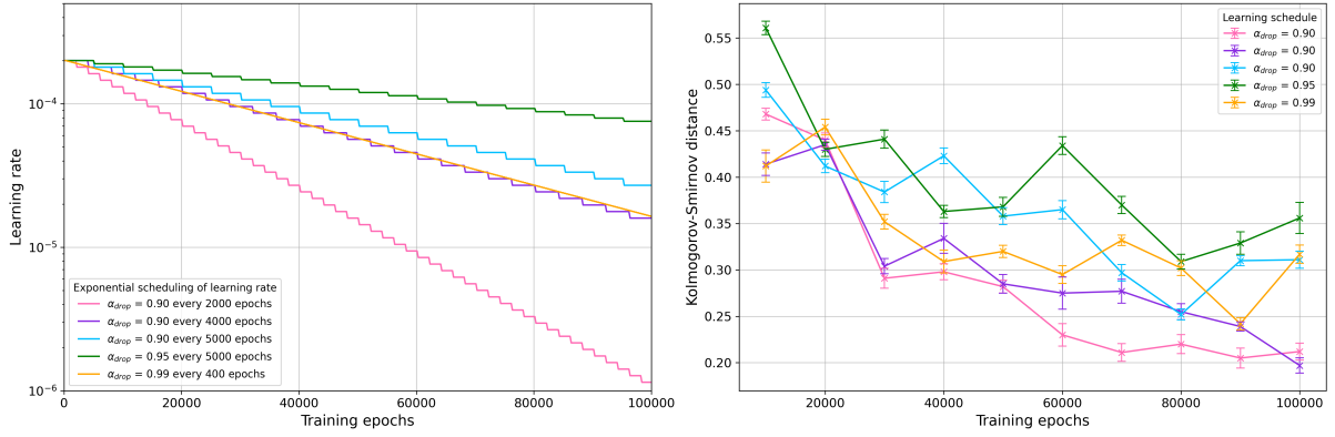
Figure 4.8: Studying the effects of exponential scheduling over a model with bs = 100 and \eta_0 = 2 \times 10^{-4} . On the left, the learning rate trends are reported for different values of \alpha_{drop} and for various updates frequency. On the right, the corresponding KS distances are shown as a function of the training epochs.
