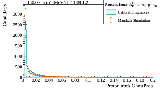
Figure 5.10: Ghost probability of the proton track as obtained from a sample of \Lambda_b^0 decays simulated with mambah.sim and from calibration data.
