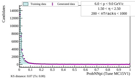
(f) Kaon track candidates.
