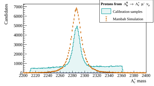
Figure 5.11: Invariant mass of the \Lambda_c^+ \rightarrow pK^-\pi^+ decay as obtained from ultra-fast simulation and with the calibration samples. The agreement of the resolution is astonishing, while the simulated sample does not include combinatorial background events.
