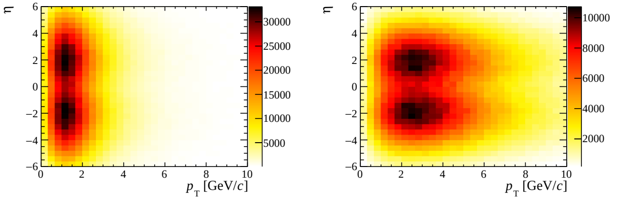
Figure 5.5: Distribution in pseudorapidity and transverse momentum of a generic charm (left) or beauty (right) hadron. Plots reproduced from Ref. [30].
