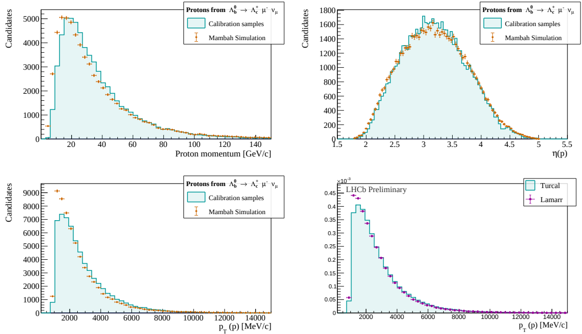
Figure 5.9: Kinematic variables of the proton produced in \Lambda_b^0 \rightarrow \Lambda_c^+ \mu^- \bar{\nu} decays followed by \Lambda_c^+ \rightarrow p K^- \pi^+ . The momentum and the pseudorapidity distributions are shown on the first row, while the transverse momentum is reported in the second row, where the comparison between Lamarr and calibration data is also reported.
