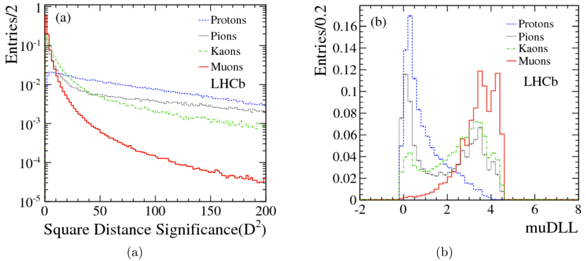
Figure 1.6: In (a) it is shown the average square distance significance distributions for muons, protons, pions and kaons as obtained from data, while in (b) it is represented their corresponding muDLL distributions. Plots reported from Ref. [10].
