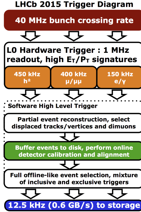
Figure 1.5: Representation of the Run 2 trigger scheme.
