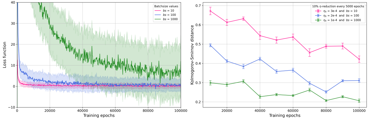
Figure 4.9: Study of the different outcomes for three combinations of learning rate and batch-size. On left plot, the loss function values are reported with the corresponding variance. On the right, the KS distances are shown for ten different points of the training process.
