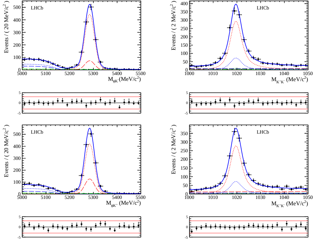
Figure 7.11 K^+K^-K^\pm (left) and K^+K^- (right) mass distributions of K -like B^- \rightarrow \phi K^- (top) and B^+ \rightarrow \phi K^+ (bottom) data candidates in the subsample selected by the L0Hadron TOS trigger line. The curves represent the results of the simultaneous two-dimensional fit described in the text. The following components are present: B^\pm \rightarrow \phi K^\pm signal (dotted red), non-resonant B^\pm \rightarrow K^+K^-K^\pm background (dashed red), partially reconstructed b -hadron background with (dotted blue) or without (dashed blue) a true \phi meson, and combinatorial background with (dotted green) or without (dashed green) true \phi meson. The total fit function is shown as the solid blue curves. The fit pulls are displayed in the small plots at the bottom.
