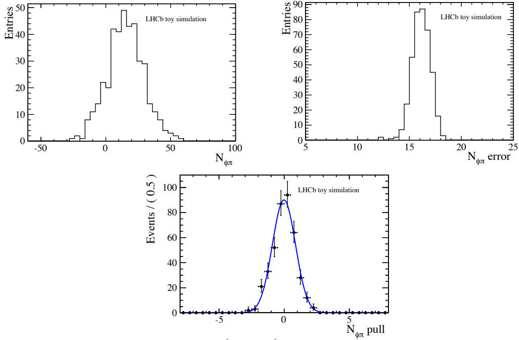
Figure 7.7 Distributions of the fitted B^\pm \rightarrow \phi\pi^\pm signal yield (top left), its estimated error (top right) and the corresponding pull (bottom), obtained from 400 embedded toy samples generated with 15 signal events each. The conditional variable \delta m is used in the fits and the \pi -like sample is divided in four \delta m bins. The mean value and the RMS of the signal yield distribution are 15.2 \pm 0.7 and 14.2 \pm 0.5 , respectively. The mean value and width obtained from a Gaussian fit to the pull distribution are -0.02 \pm 0.04 and 0.89 \pm 0.03 , respectively. The width is smaller than 1 because the number of events in each sample is fixed in the generation.
