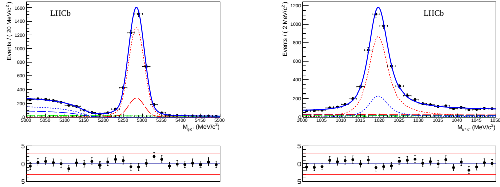
Figure 7.5 K^+K^-K^\pm (left) and K^+K^- (right) mass distributions of K-like B^\pm \rightarrow \phi K^\pm data candidates. The curves represent the results of the two-dimensional fit described in the text, with the following components: B^\pm \rightarrow \phi K^\pm signal (dotted red), non-resonant B^\pm \rightarrow K^+K^-K^\pm background (dashed red), partially reconstructed b-hadron background with (dotted blue) or without (dashed blue) a true \phi meson, and combinatorial background with (dotted green) or without (dashed green) true \phi meson. The total fit function is shown as the solid blue curves. The fit pulls are displayed in the small plots at the bottom.
