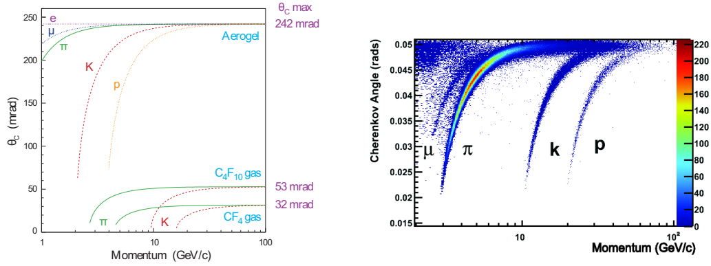
Figure 4.10 Cherenkov angle of different radiators (left) and of C_4F_{10} (right) as a function of the particle momentum.
