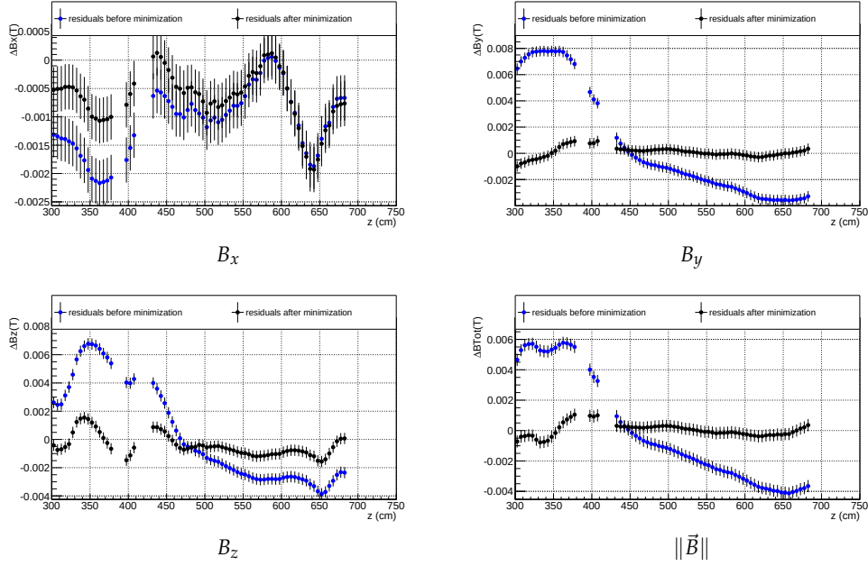
Figure 5.18 Difference between the new measurements and the old map without (blue points) or with (black points) the corrections obtained from the global fit. The magnetic field is plotted as a function of z , at y = 33.1 cm.
