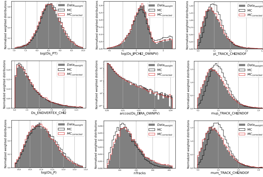
FIGURE 6.2: Distributions of the kinematic and track quality variables used as input features to the GBReweighter in data and simulation, before (black) and after (red) applying the w_{\text{Data/MC}} corrections. The plots are generated for 2017 data.
