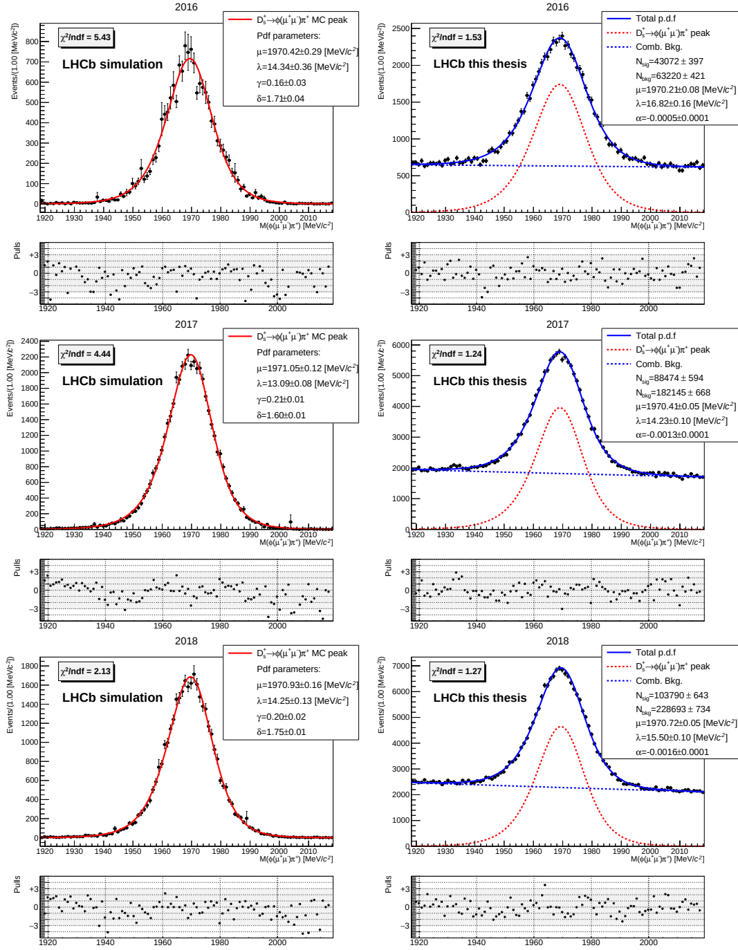
FIGURE 6.8: Fit to the D_s^+ \rightarrow \phi(\mu^+ \mu^-) \pi^+ invariant mass distribution obtained for simulated events (left) and recorded data (right). Simulated events are weighted with w_{\text{fraction}} , w_{\text{fracCorr}} and w_{\text{Data/MC}} . The mass shape is modelled using a Johnson's S_U function to describe the signal peak and an exponential distribution to describe the combinatorial background in data. The fit parameters \gamma and \delta describing the signal peak in data are fixed from the fit to simulated events. The plots are shown for the three data-taking years.
