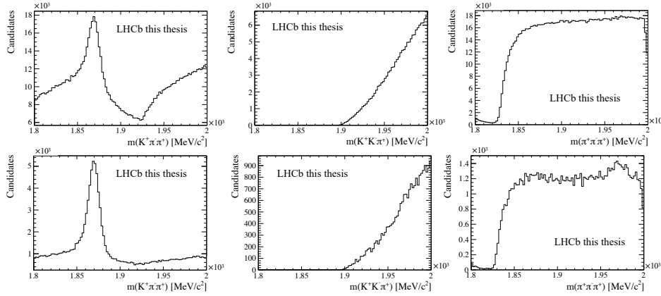
FIGURE 8.4: Distribution of the three muons invariant mass in the 2018 data sample under the K^-\pi^+\pi^+ (left), K^-K^+\pi^+ (middle) and \pi^-\pi^+\pi^+ (right) mass hypotheses. The distributions in the first row are obtained by applying the preselection cuts reported in Chapter 5 while in the second row an additional requirement on XGB ( > 0.5 ) is applied in order to reduce the contamination of the combinatorial background.
