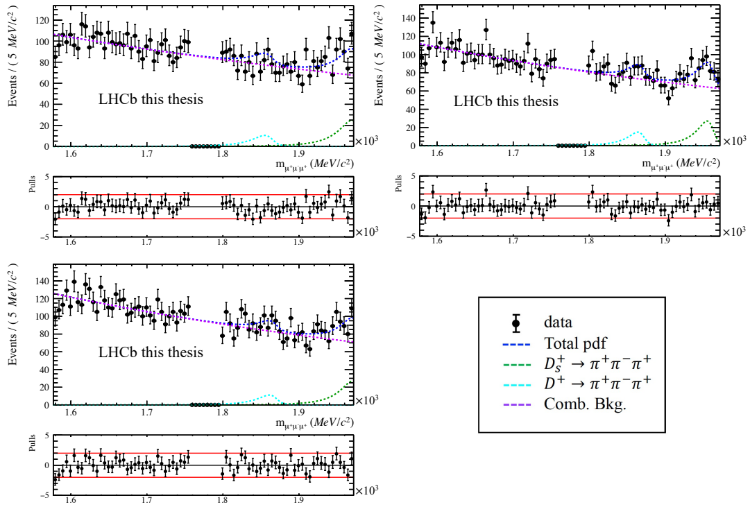
FIGURE 8.12: Fit to the data sidebands invariant mass distribution in the 3\mu sample after the minimum requirements on XGB and SuperPNN and the veto on ProbNNk assuming the contribution of the combinatorial background and of the D^+ \rightarrow \pi^- \pi^+ \pi^+ and D_s^+ \rightarrow \pi^- \pi^+ \pi^+ modes. Plots are shown for the three data-taking years: 2016 (top-left), 2017 (top-right), 2018 (bottom).
