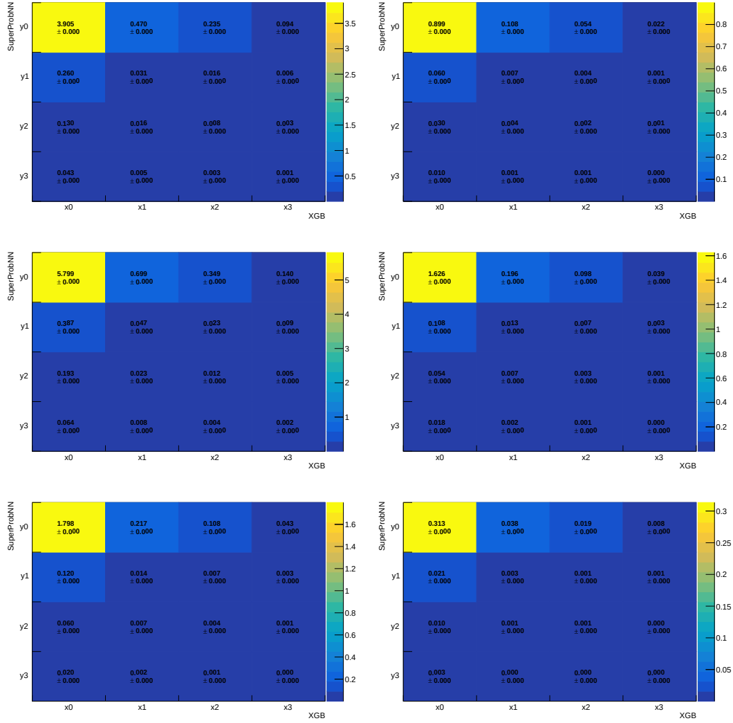
FIGURE 8.13: Number of D^+ \rightarrow \pi^- \pi^+ \pi^+ (left) and D_s^+ \rightarrow \pi^- \pi^+ \pi^+ (right) candidates expected in the signal region in the 3\mu sample in bins of XGB and SuperPNN. The maps are reported for the three data-taking periods: 2016 (top), 2017 (middle) and 2018 (bottom).
