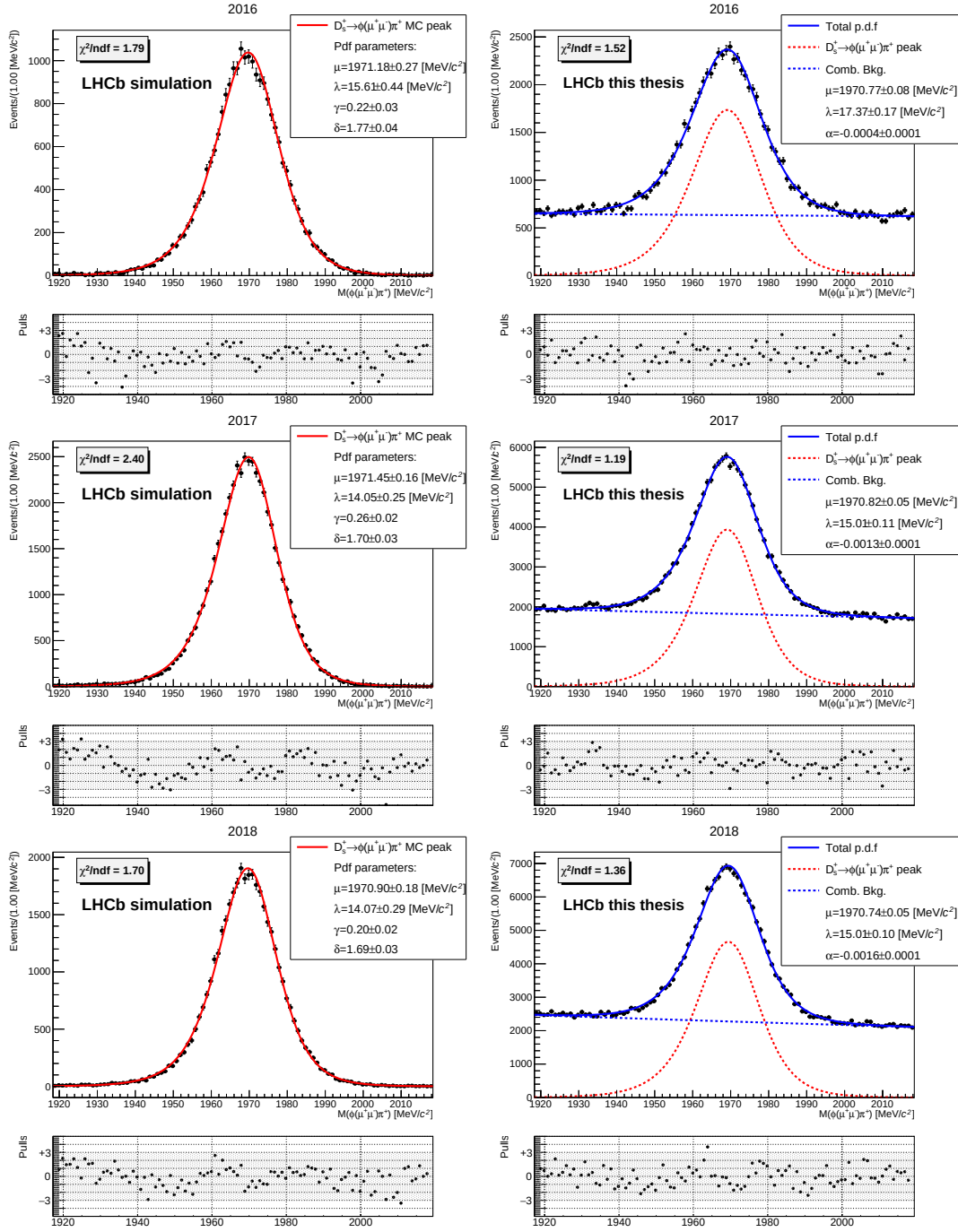
FIGURE 6.1: Fit to the D_s^+ \rightarrow \phi(\mu^+ \mu^-) \pi^+ invariant mass distribution obtained for simulated events (left) and recorded data (right). Simulated events are weighted with w_{\text{fraction}} . The mass shape is modelled using a Johnson's SU function to describe the signal peak and an exponential distribution to describe the combinatorial background in data. The fit parameters \gamma and \delta describing the signal peak in data are fixed from the fit to simulated events. The plots are shown for the three data-taking years.
