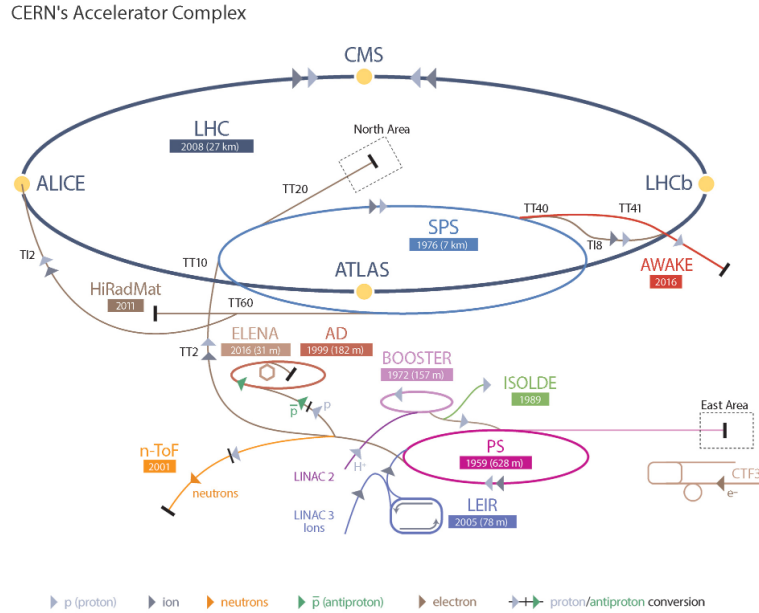
Figure 5: The LHC accelerator complex.
