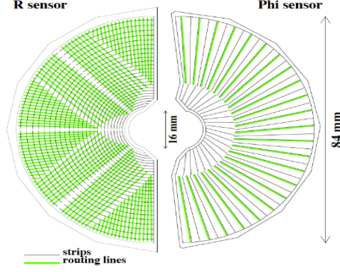
Figure 10: Representation of an R and \phi sensor.
