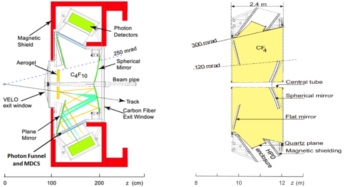
Figure 18: Left: RICH1, Right: RICH2.
