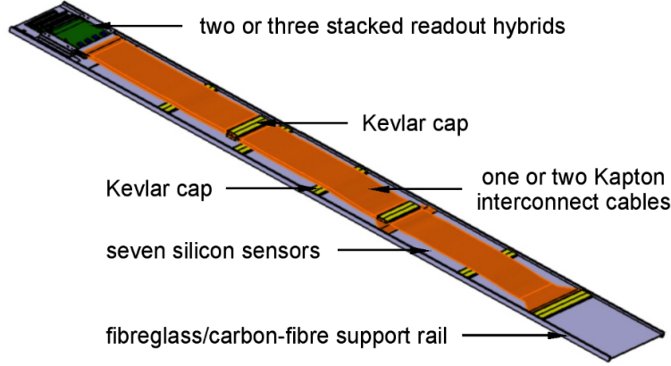
Figure 13: The TT half module.
