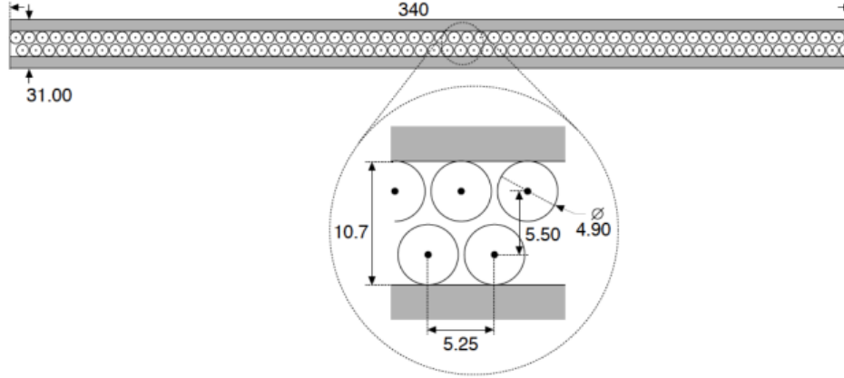
Figure 17: The Outer Tracker cross section.
