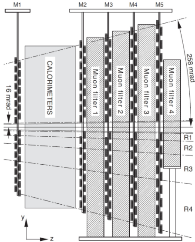
Figure 27: Overview of the LHCb muon stations.
