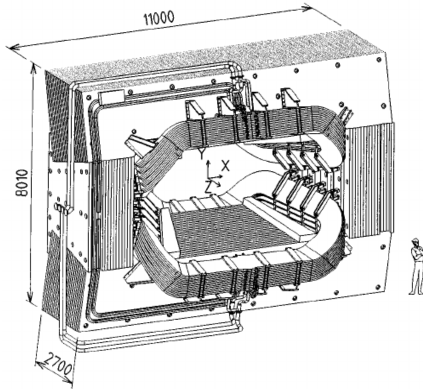
Figure 11: The LHCb magnet.
