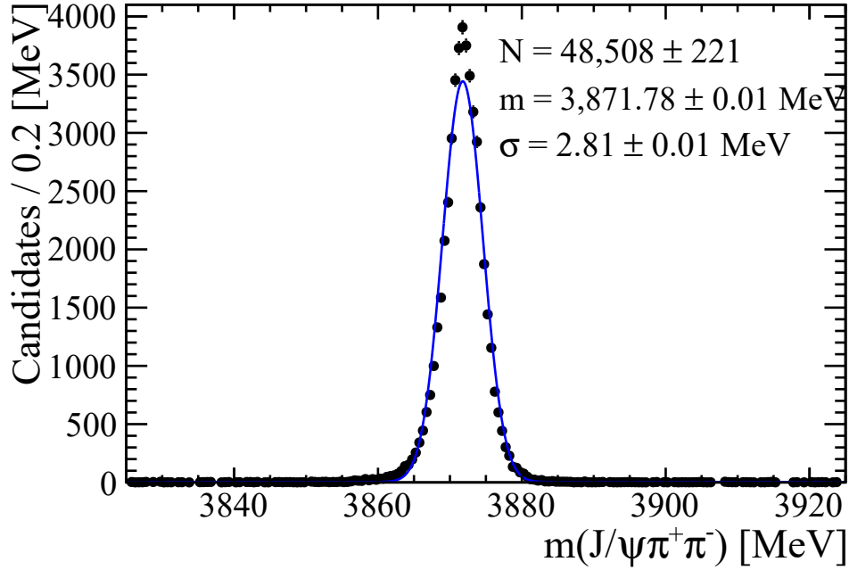
Figure 85: Fit to the J/\psi\pi^+\pi^- distribution in the signal simulations, after the 2\sigma B^+ mass cut, and with the PV, J/\psi and B^+ mass constraints. We used Gaussian function for the signal peak and flat background. The blue line represents the total fit. Compare to fit with the double-sided Crystal Ball lineshape shown in Fig. 42.
