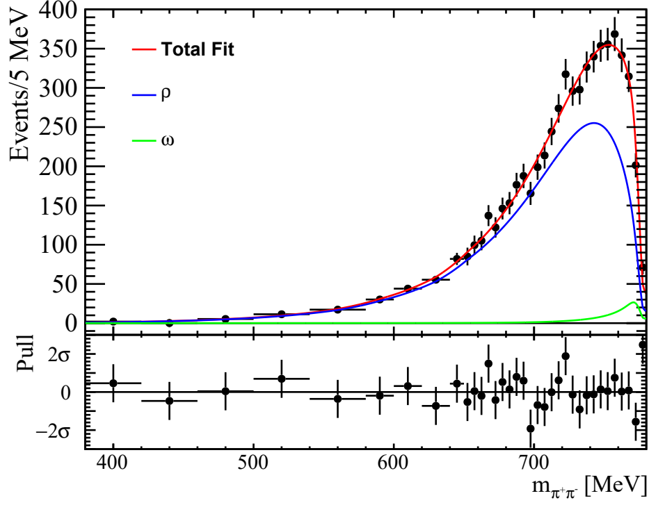
Figure 62: Fits of the coupled-channel model with \rho^0 and \omega contributions and linear dependence of \alpha_{2\pi} on m_{\pi\pi}^2 . Fit result when g_{\omega \rightarrow 2\pi}^2 . \chi^2/\text{NDoF} = 24.7/32 , pV = 0.82 and P_1 = 0.23 \pm 0.05 .
