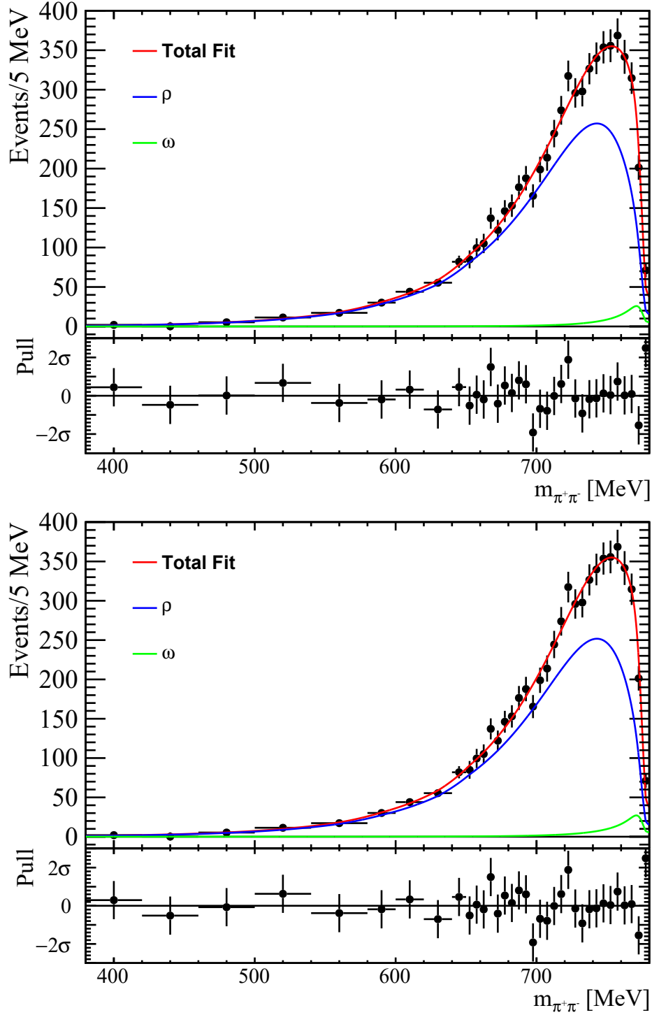
Figure 59: Fit of the coupled-channel model with the \rho^0 and \omega contributions and linear dependence of \alpha_{2\pi} on m_{\pi\pi}^2 . The top (bottom) figures are obtained with R_{\text{prod}} = 0 (30) \text{GeV}^{-1} (see the text). The P_1 coefficients are 0.17 \pm 0.04 ( 0.56 \pm 0.05 ), respectively.
