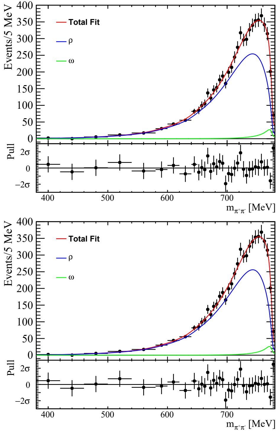
Figure 58: Fits of the coupled-channel model with \rho^0 and \omega contributions and linear dependence of \alpha_{2\pi} on m_{\pi\pi}^2 . In these fits, R = 1.3 ( 1.6 ) \text{GeV}^{-1} at the top (bottom) displays. The P_1 coefficients are 0.21 \pm 0.05 ( 0.24 \pm 0.05 ), respectively.
