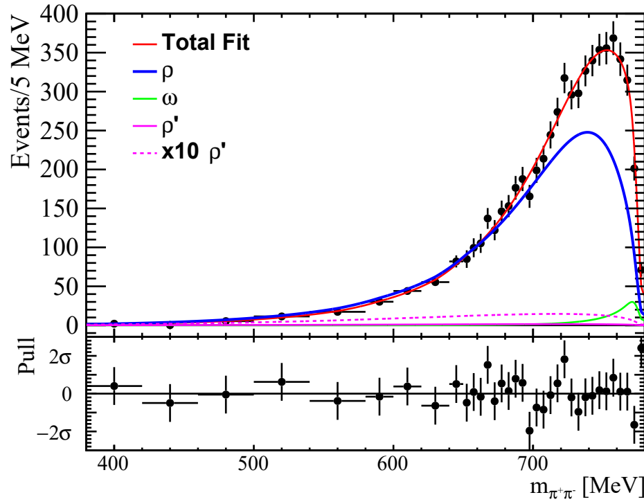
Figure 94: Fit of Gounaris-Sakurai (GS) model of \rho^0 coupled with \omega via Eq. 50, and \rho'^0 in the GS representation added to the fit. The relative phase of \omega was set to zero. The relative phase of \rho'^0 was set to 3.76 rad [4]. The fit qualities are \chi^2/\text{NDoF} = 24.8/32 and pV = 0.81 .
