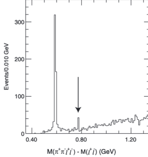
Figure 3: The distribution of mass difference between \pi^+\pi^-J/\psi and J/\psi in B^\pm \rightarrow \pi^+\pi^-J/\psi K^\pm decays. The peak at 0.59 GeV is due to the \psi(2S) charmonium state. The peak corresponding to the X(3872) discovery is indicated with an arrow.
