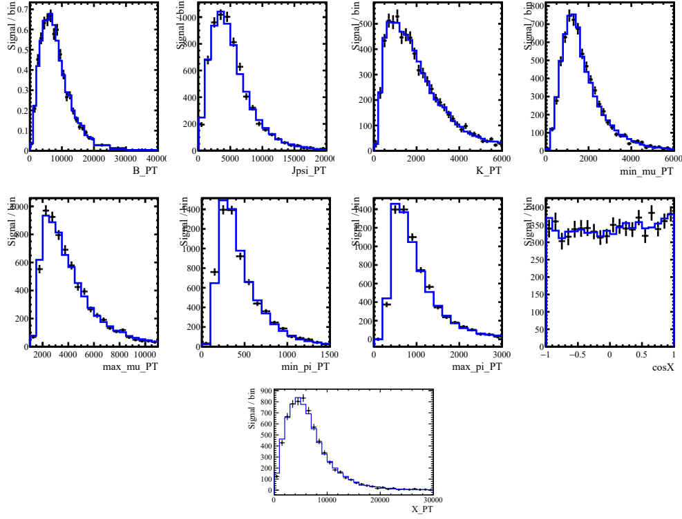
Figure 79: The distributions of p_T of various reconstructed particles, and of X(3872) helicity angle, for the data (points with error bars) and for the MC (histogram) with use of PIDcalib package. The distributions were corrected for the varying bin width. The data points were obtained by fitting the X(3872) peak in the J/\psi\pi^+\pi^- mass distributions for various bins. The MC events were weighted by the run-dependent, dipion-mass-dependent and p_T(B^+) -dependent weights. The MC distributions were normalized to the same number of entries as the data.
