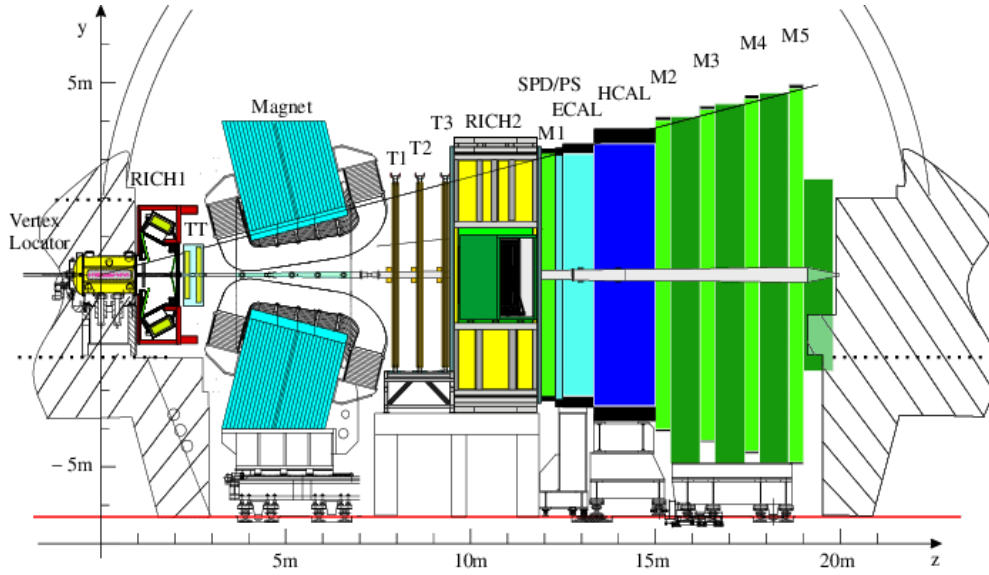
Figure 6: LHCb Detector .
