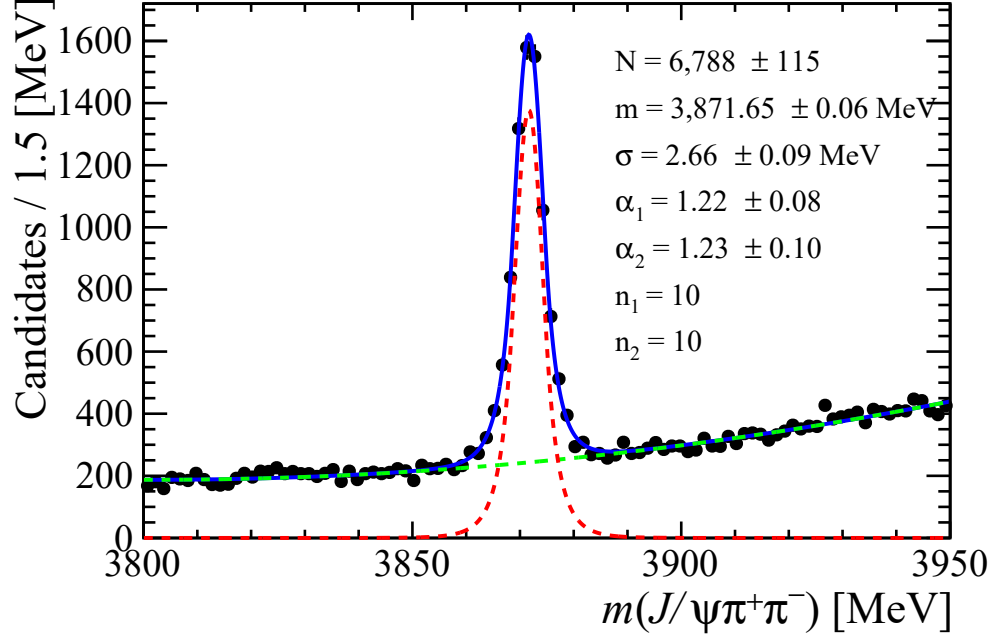
Figure 30: M(J/\psi\pi^+\pi^-) mass fit with the 2\sigma B^+ mass signal cut, with the PV , J/\psi and B^+ mass constraints. We used DSCB for the signal peak and quadratic polynomial for the background. The blue line represents the total fit, red is the signal component, and the dashed-green is the background.
