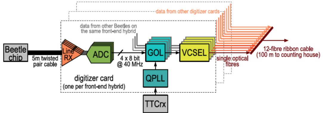
Figure 15: Signal processing from Beetle chip.
