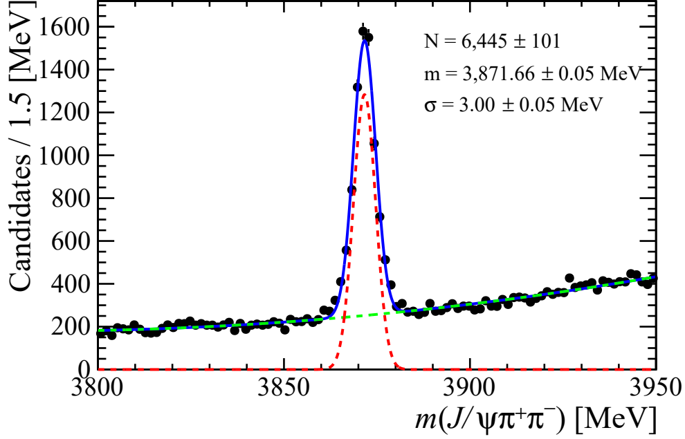
Figure 86: The distribution of m_{J/\psi\pi^+\pi^-} with the 2\sigma B^+ mass signal cut, with the PV, J/\psi and B^+ mass constraints, fit with a Gaussian for the signal, and quadratic polynomial for the background. The blue line represents the total fit, red is the signal component, and the dashed-green is the background. Compare to the fit with the double-sided Crystal Ball lineshape in Fig. 30.
