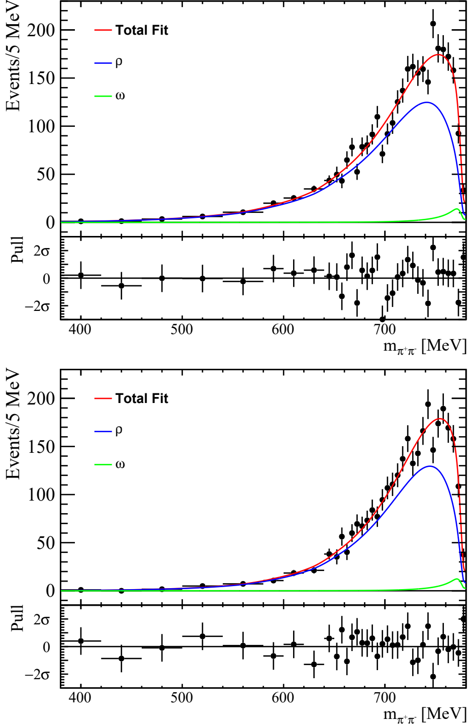
Figure 66: Fit of the coupled-channel model with the \rho^0 and \omega contributions and linear dependence of \alpha_{2\pi} of m_{\pi\pi}^2 . The top: fit sample is in the \cos\theta_X > 0 region, \chi^2/\text{NDoF} = 42.2/32 , pV = 0.11 . The bottom: fit sample is in the \cos\theta_X < 0 region, \chi^2/\text{NDoF} = 26.9/32 and pV = 0.72 . \theta_X is the helicity angle of X(3872) . The P_1 coefficients are 0.16 \pm 0.05 and 0.31 \pm 0.08 , respectively.
