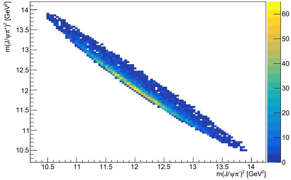
Figure 99: Dalitz plot for X(3872) \rightarrow J/\psi \pi^+ \pi^- decay. The pion candidate which has the same sign as B in the selected B \rightarrow X(3872)K decay is labeled as \pi^+ .
