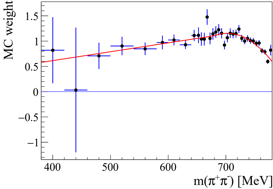
Figure 96: The ratio of the dipion mass distribution reconstructed in the data and in the simulations (points with error bars), with the smoothing weight function superimposed. p -value of the fit is 47%.
