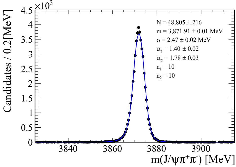
Figure 42: Fit to the J/\psi\pi^+\pi^- distribution in the signal simulations, after the 2\sigma B^+ mass cut, and with the PV, J/\psi and B^+ mass constraints. We used DSCB for the signal peak and flat background. The blue line represents the total fit. The fitted background level is only 2.8 \pm 0.5 events per bin. The signal shape parameters are: 48,805 \pm 216 signal events, m = 3,871.91 \pm 0.01 MeV, \sigma = 2.47 \pm 0.02 MeV, n_1 = n_2 = 10 (fixed), \alpha_1 = 1.40 \pm 0.02 , and \alpha_2 = 1.78 \pm 0.03 .
