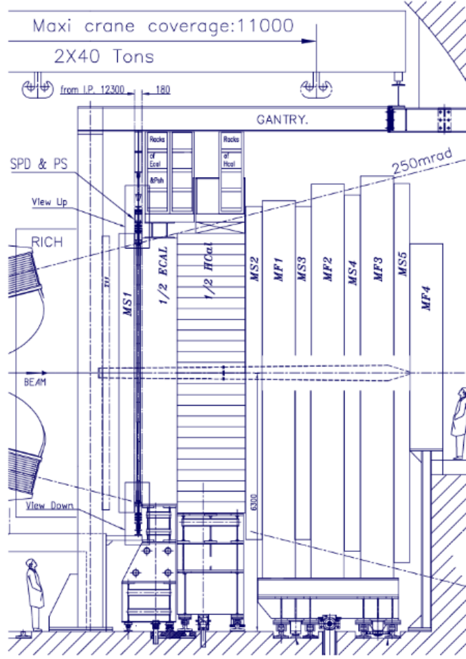
Figure 24: View of the SPD/PS detectors.
