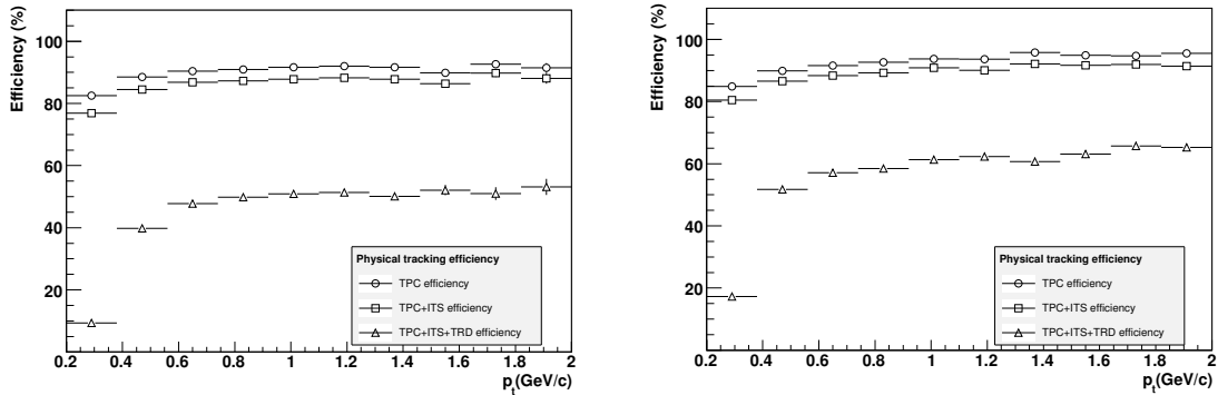
Figure 3.7: Physical track finding efficiency for different combinations of tracking detectors as a function of particle transverse momentum. Left: central Pb–Pb collisions ( dN_{\text{ch}}/d\eta = 6000 ). Right: pp collisions.
