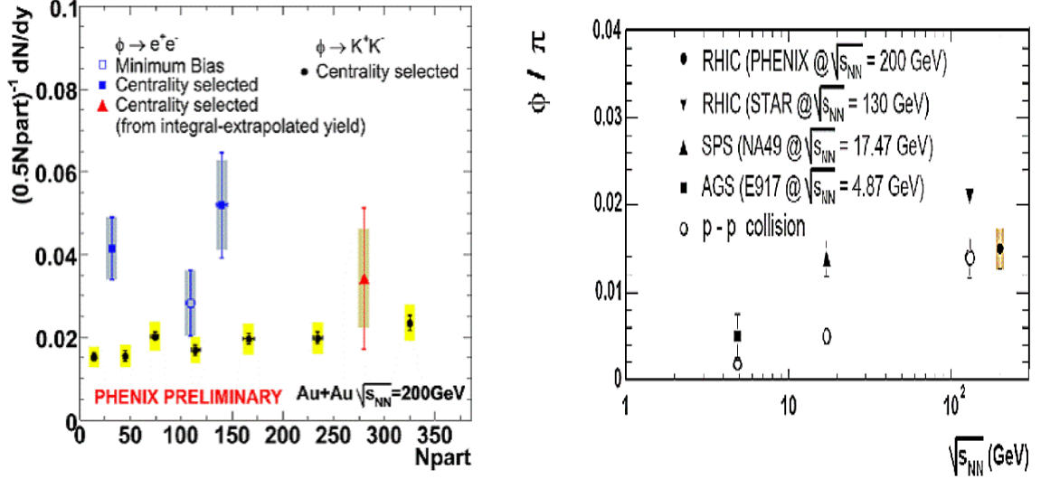
Figure 1.4: Left: Multiplicity dependence of the \phi yield for e^+e^- and K^+K^- decay channels [126]. Right: \phi/\pi ratios as a function of collision energy. The data points are from the \phi \rightarrow K^+K^- channel [123].
