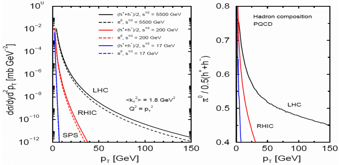
Figure 1.10: The predicted leading order (LO) differential cross section for neutral pion and charged hadron production for pp collisions at \sqrt{s} = 17, 200, \text{ and } 5500 \text{ GeV} . The predicted hadron composition in pp is plotted in the right panel.
