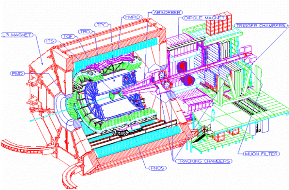
Figure 2.1: The ALICE setup in its final layout. For the sake of visibility the HMPID detector is shown in the 12 o'clock position instead of the 2 o'clock position at which is actually located.
