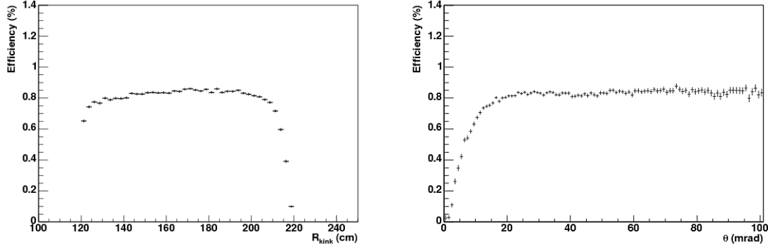
Figure 5.4: pp collisions: Left: Reconstruction efficiency for as a function of the decay vertex. Right: Reconstruction efficiency as a function of the decay angle.
