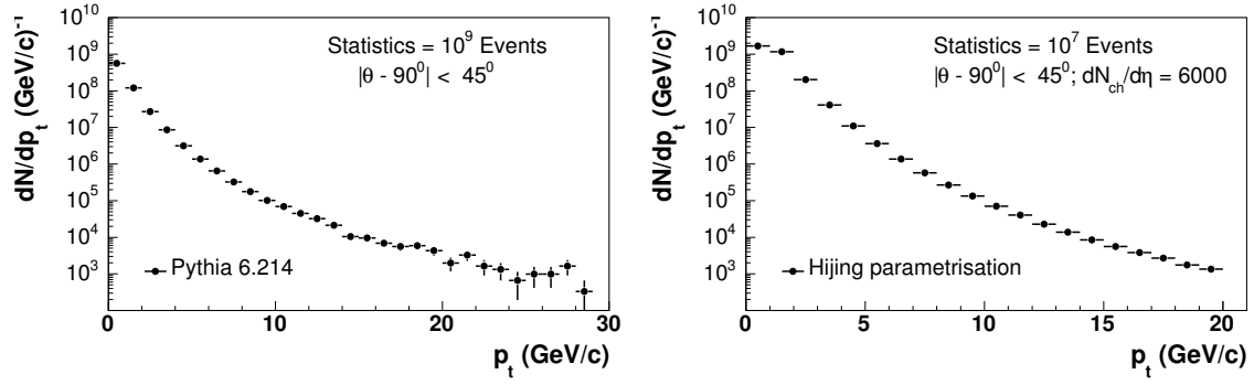
Figure 5.6: Left: PYTHIA 6.214 prediction for p_T distribution of charged kaons in 10^9 pp collisions at \sqrt{s} = 14\text{TeV} in the central barrel. An overall event trigger efficiency of about 82% was taken into account. Right: HIJING parametrisation prediction for 10^7 central Pb–Pb collisions with dN_{ch}/d\eta = 6000 at \sqrt{s} = 5.5\text{TeV} .
