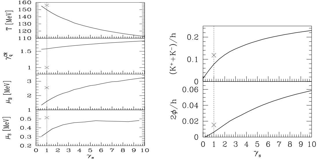
Figure 1.11: Left: The values of hadronization temperature, T , maximum quark phase space occupancy, \gamma_q^{CR} , and baryon, \mu_B , and strange, \mu_S , chemical potentials, as a function of \gamma_s as obtained in the hadronization model [190]. Right: Particle ratios of K^+ + K^-/h and 2\phi/h as a function of \gamma_s . The crosses indicates chemical equilibrium model predictions. From [190].
