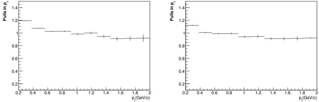
Figure 3.3: Pulls in track momentum as a function of particle transverse momentum. Left: central Pb-Pb collisions ( dN_{ch}/d\eta = 6000 ). Right: pp collisions.
