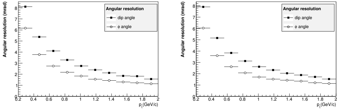
Figure 3.9: Angular resolution for combined track finding as a function of particle transverse momentum. Left: central Pb-Pb collisions ( dN_{\text{ch}}/d\eta = 6000 ). Right: pp collisions.
