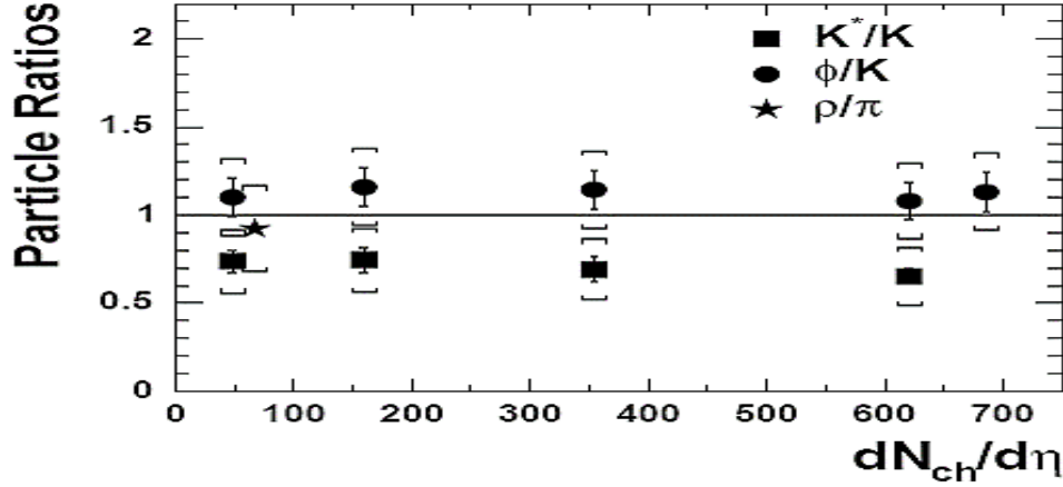
Figure 1.5: The K^*/K^- , \phi/K^- , and \rho^0/\pi^- yield normalized to the pp ratios as function of centrality for Au–Au collisions at \sqrt{s} = 200 GeV [141].
