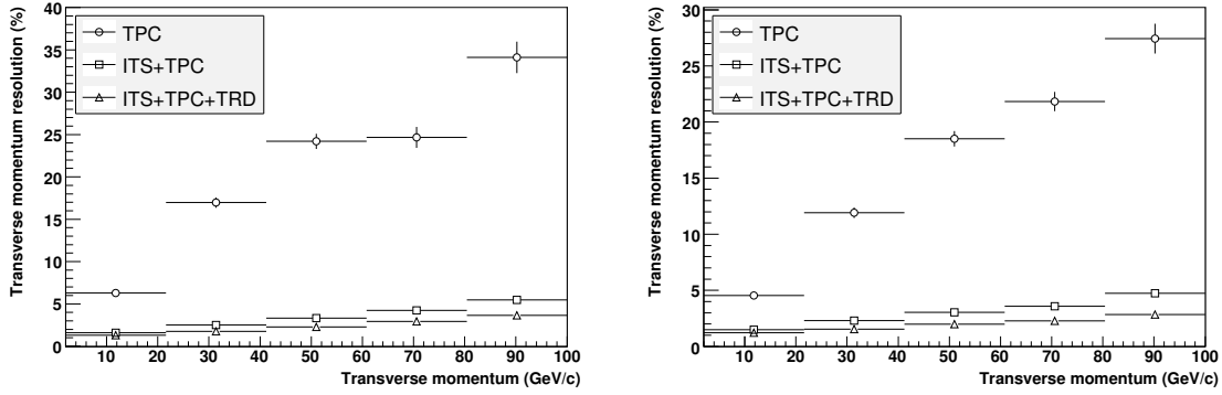
Figure 3.8: Transverse momentum resolution for combined track finding as a function of particle transverse momentum. Left: central Pb-Pb collisions ( dN_{\text{ch}}/d\eta = 6000 ). Right: pp collisions.
