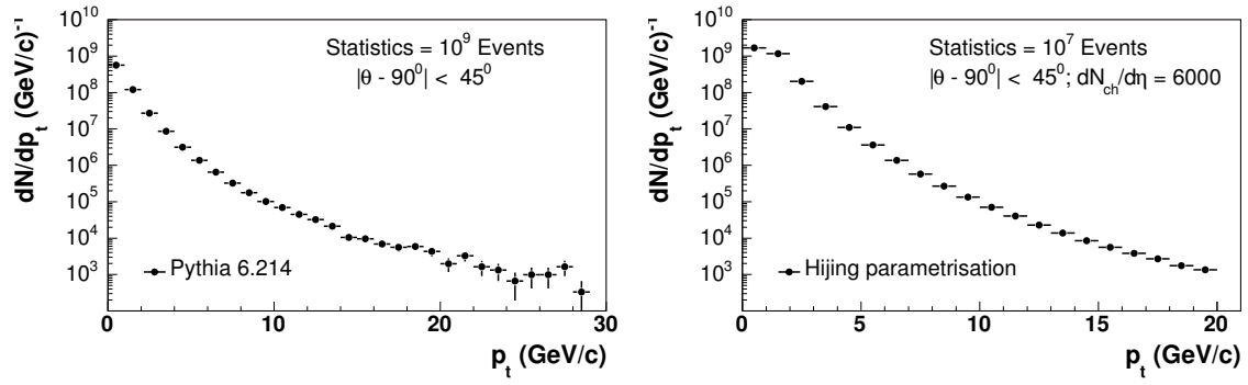
Figure 5.6: Left: PYTHIA 6.214 prediction for p_T distribution of charged kaons in 10^9 pp collisions at \sqrt{s} = 14\text{TeV} in the central barrel. An overall event trigger efficiency of about 82% was taken into account. Right: HIJING parametrisation prediction for 10^7 central Pb–Pb collisions with dN_{ch}/d\eta = 6000 at \sqrt{s} = 5.5\text{TeV} .
