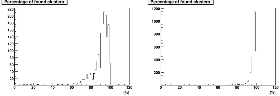
Figure 3.2: Ratio of the number of clusters associated to a track to the number of pad-rows crossed by this track. Left: central Pb-Pb collisions ( dN_{ch}/d\eta = 6000 ). Right: pp collisions.
