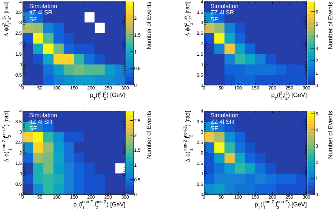
Figure 3.5.: The distributions of the number of events as a function of \Delta\phi and p_T of the Z leptons in the upper plots and the non-Z leptons in the lower plots for ZZ and ttZ . For ZZ the distributions look similar, because the leptons labelled as “non-Z leptons” actually originate from a Z boson, too. This way these observables can help to distinguish ZZ from the signal ttZ .
