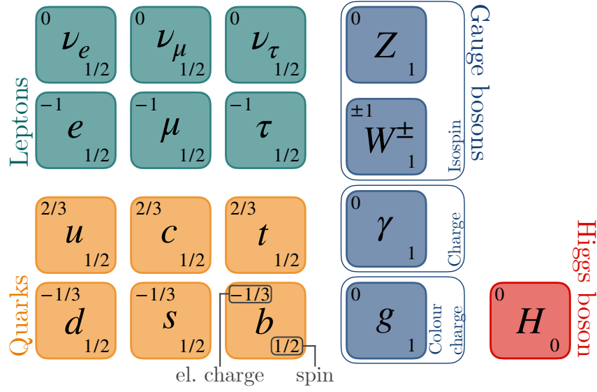
Figure 1.1.: The elementary particles of the Standard Model. The upper left part shows the leptons ordered by generations. The quarks are shown in the lower left and are ordered the same way. The bosons are split into the gauge bosons in blue with spin 1 and the Higgs boson in red with spin 0. The electric charge and spin are listed for all elementary particles. In addition, the quantum numbers the gauge bosons couple to are given.
