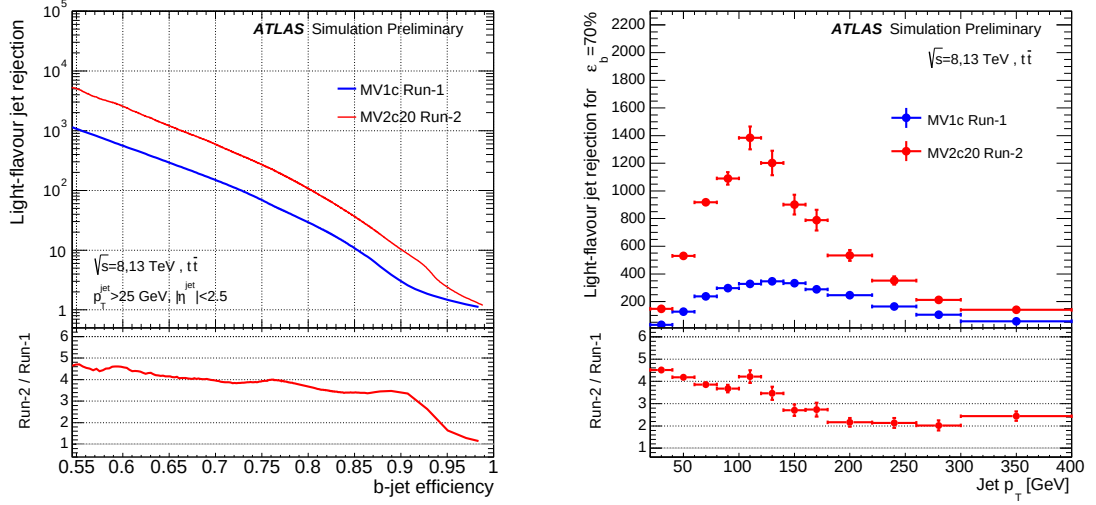
(a) Light-jet rejection versus b-tagging efficiency \varepsilon_b . (b) Light-jet rejection for a fixed \varepsilon_b = 70\% versus jet p_T .
