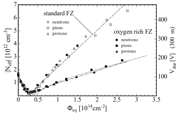
Figure 3.9.: Absolute effective doping concentration ( |N_{\text{eff}}| ) versus fluence ( \Phi ) [70].
