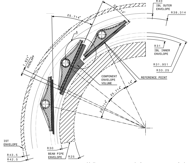
Figure 3.10.: Drawing of the Insertable B-Layer.
