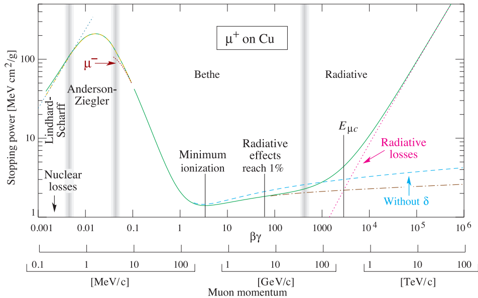
Figure 4.1.: Stopping power for anti-muons in copper normalised by density. Particle Data Group © 2018.
