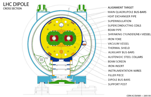
Figure 3.1.: Cross-section of an LHC dipole used to bend the charged beam. Copyright and image credit: CERN.
