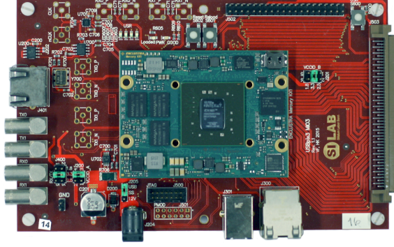
(b) MultiIO3 board.
