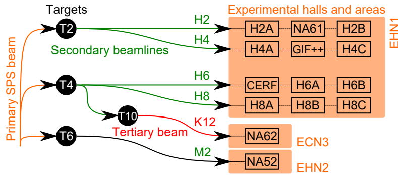
Figure 5.3.: Beam generation and beamlines at CERN's North Area experimental site.
