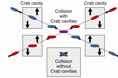
Figure 3.3.: Crab cavities. Copyright and image credit: CERN.
