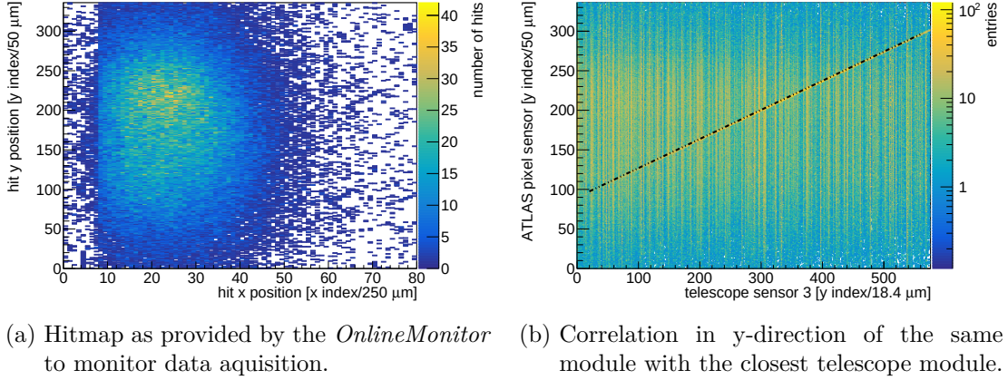
Figure 5.7.: Two monitoring plots produced by EUDAQ during data taking. The line in the right plot has been added by hand to correlate the different pixel pitches of the Mimosa26 sensor and FE-I4 module.
