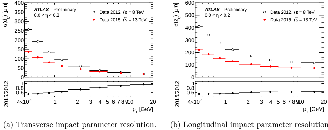
Figure 2.6.: Comparison of the tracking resolution prior to the upgrade (Data 2012) and after (Data 2015). Shown is the transverse ( d_0 ) and longitudinal ( z_0 ) impact parameter resolution \sigma , binned in transverse momentum p_T .
