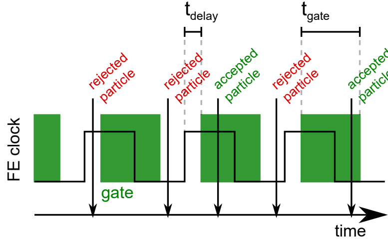
Figure 9.1.: Principle of an acceptance window to only select particles which arrive within the gate. The vertical arrows indicate incident particles.
