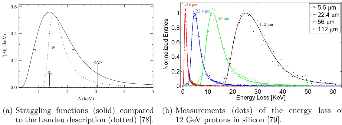
Figure 4.2.: The Landau distribution and straggling functions for the energy loss of individual particles.
