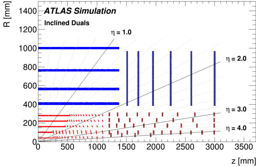
Figure 3.19.: The approximate layout for the ITk upgrade. The pixel detector in red and the strip layers in blue [74].
