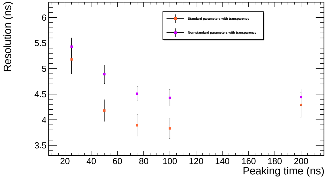
FIGURE 4.35: Time resolution computed with the CFD methods for the FastSim with transparency as a function of the VFAT n3 peaking time for a gas mixture of Ar/CO 2 /CF 4 (45:15:40) for the ‘non-standard’ parameters and the ‘standard’ parameters.
