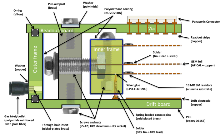
FIGURE 3.24: Cross section through inner and outer chamber frames and GEM foils of the GE1/1-V showing the stretching apparatus [17].
