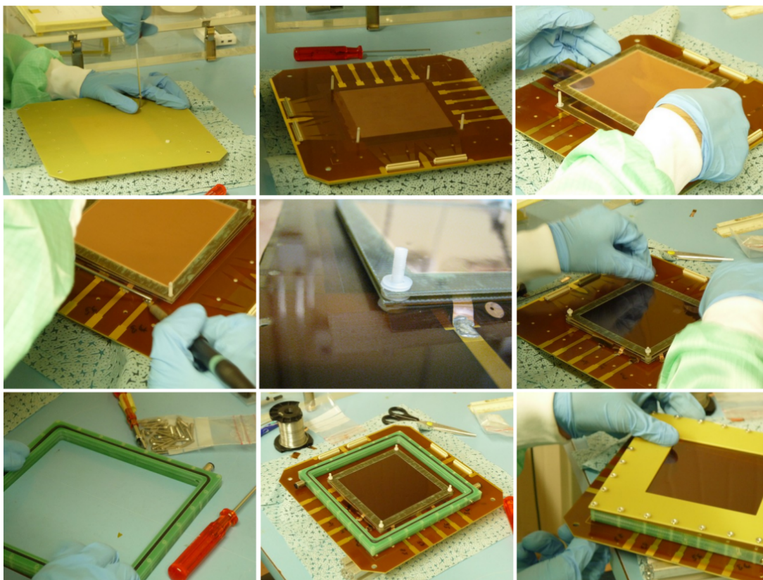
FIGURE 5.1: Assembly of one of the ULB 10x10 cm 2 Triple-GEM prototypes.
