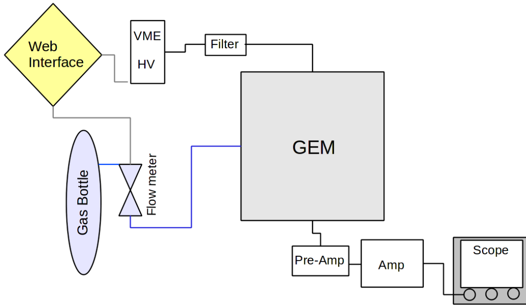
FIGURE 5.9: Schematic view of the experimental setup.
