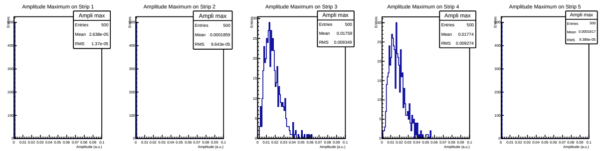
FIGURE 4.40: Distributions of the maximum amplitude of 500 shaped signals on the five strips for perpendicular muon track passing between strip 3 and 4 in the Ar/CO 2 /CF 4 (45:15:40) gas mixture.
