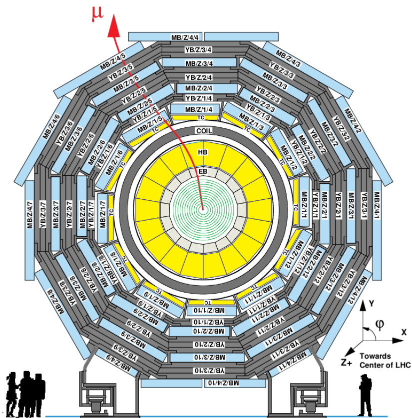
FIGURE 2.10: Transversal view of one of the five wheels of CMS [13].
