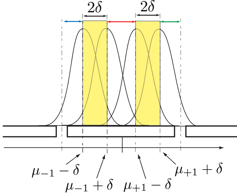
FIGURE 6.11: Transition region around \mu_{\pm 1} with its width of 2\delta in the two parameter model.
