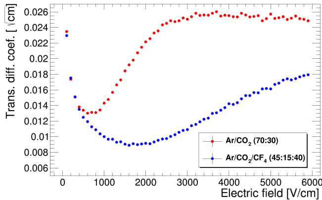
FIGURE 4.23: Evolution of the transverse diffusion coefficient as a function of the electric field for the Ar/CO 2 (70:30) and Ar/CO 2 /CF 4 (45:15:40) gas mixtures simulated by GARFIELD and Magboltz.
