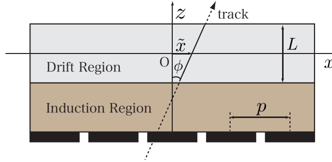
FIGURE 6.1: Detector Model.
