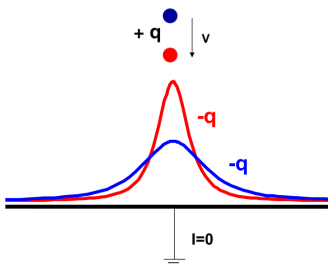
FIGURE 3.10: Diagram of the distribution of charge on a non-segmented electrode.
