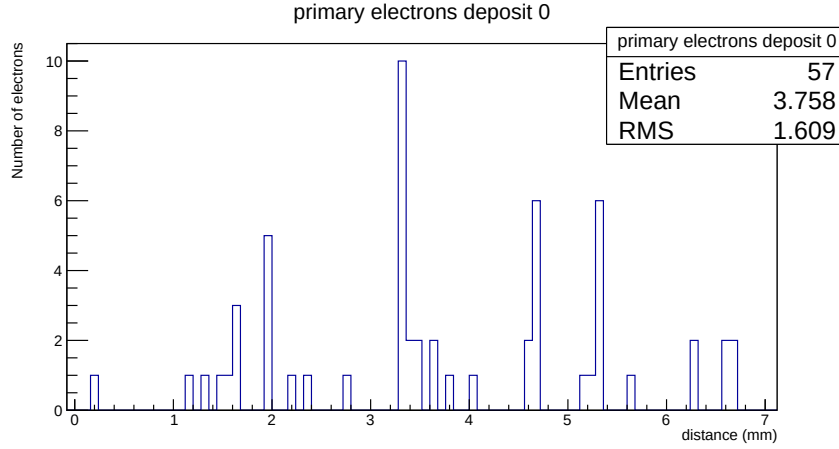
FIGURE 4.28: Cluster sizes along a perpendicular muon track of 15 GeV in Ar/CO 2 (70:30) gas mixture.
