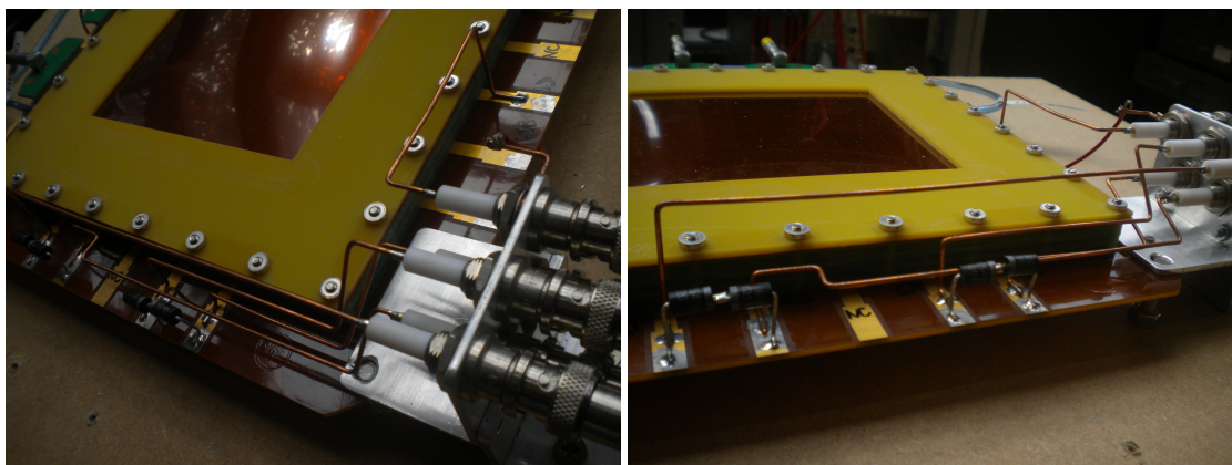
FIGURE 5.7: The five HV connector and the four Zener diodes of the Double-GEM prototype.
