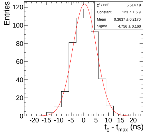
FIGURE 4.12: Time resolution distribution computed with the CFD method for a peaking time of 100 ns for the VFAT 3 .
