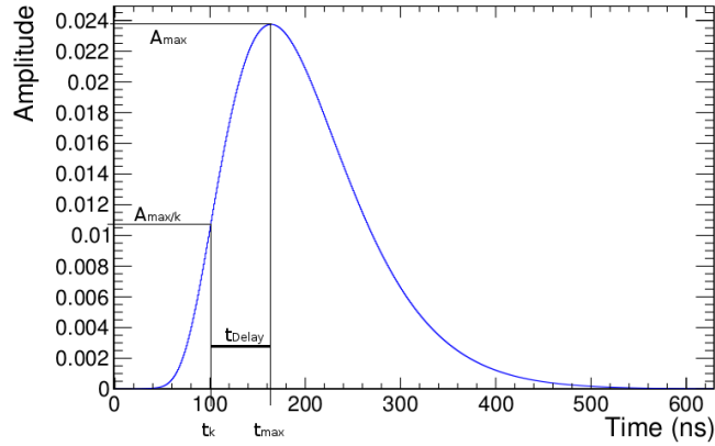
FIGURE 4.9: A Triple-GEM signal after the convolution with the VFAT3 transfer function. The delay time t_{\text{delay}} applied in the CFD construction is the difference between the time t_{\text{max}} when the signal amplitude is the maximum ( A_{\text{max}} ) and the time t_k when the signal amplitude is at maximum divided by the constant k ( A_{\text{max}}/k ).
