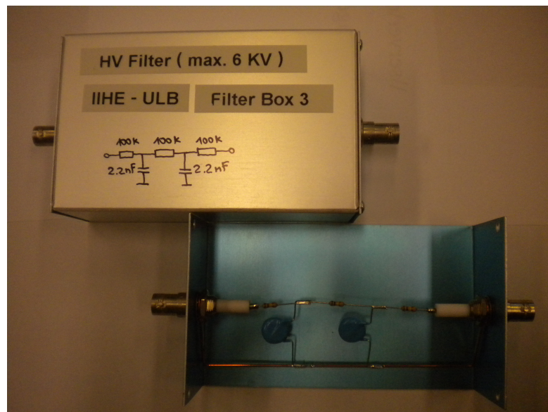
FIGURE 5.11: HV filter.
