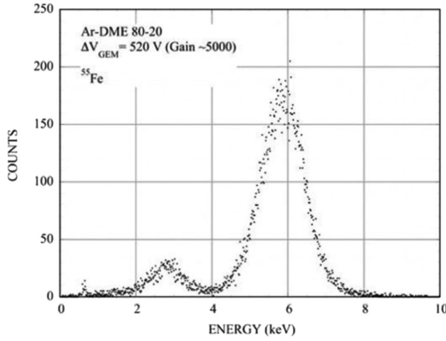
FIGURE 5.14: Energy spectrum of the ^{55}\text{Fe} source for a single GEM [64].
