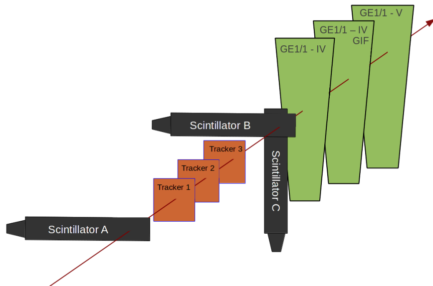
FIGURE 5.28: Schematic view of the test beam setup.
