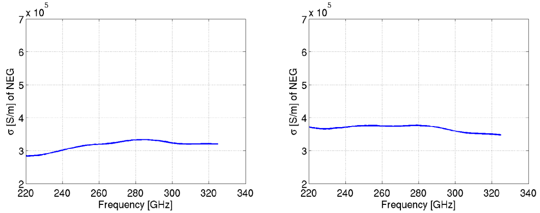
Figure 4.44: NEG effective conductivity between 220 and 330 GHz for a non-uniform profile. For the wider part of the groove, coating of 5 and 10 \mu\text{m} was considered, while 1.5 \mu\text{m} was assumed for the side walls (left plot) and 1.8 \mu\text{m} (right plot).
