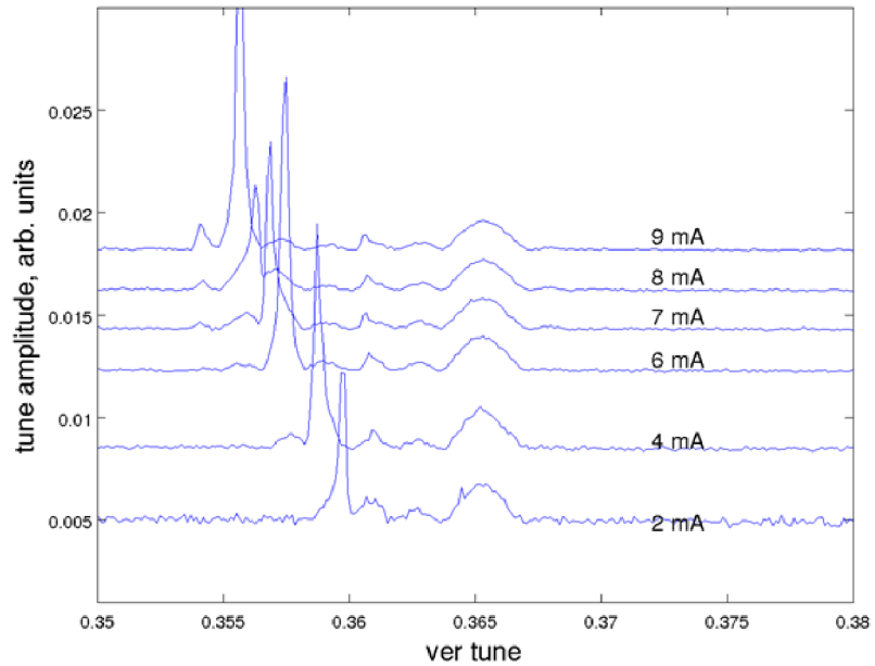
Figure 5.3: Tune monitor for open IVUs [75]. Mode 0 shifts down as current increases and mode -1 appears before the instability onset (9.8 mA).
