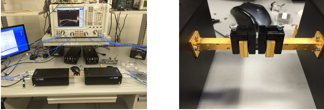
Figure 4.31: Measurement setup at VDI. A WR1.5 is connected with flanges to the VNA extenders of 500-750 GHz.
