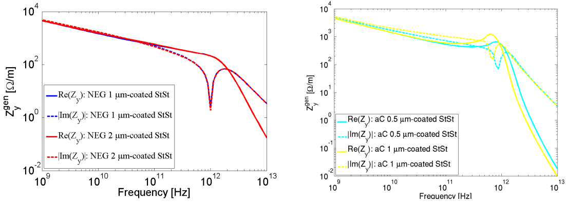
Figure 3.16: Generalized vertical impedance of the wigglers for NEG (left) or aC (right) on StSt chamber of various thicknesses.
