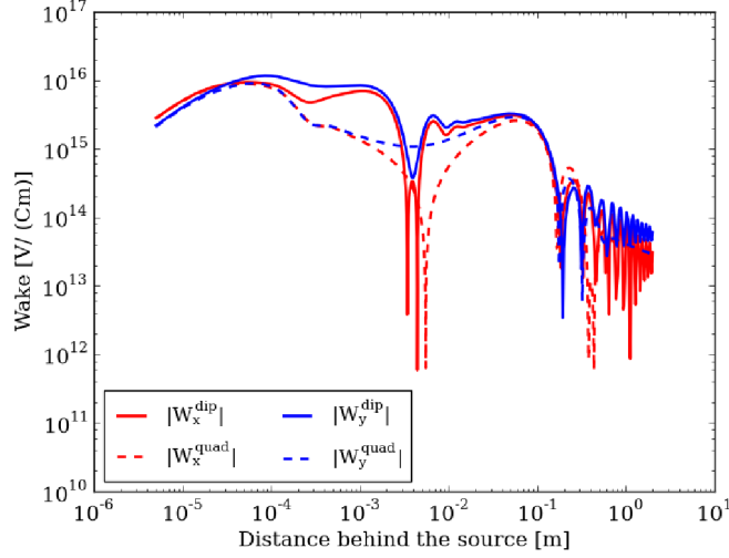
Figure 5.6: Transverse wake function model in HEADTAIL.
