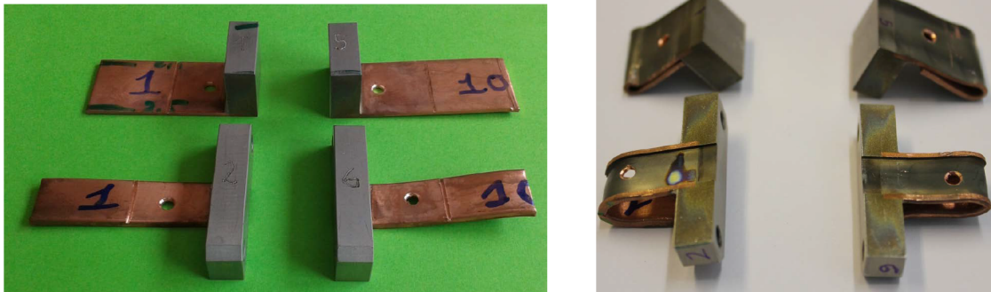
Figure 4.20: Samples for the SEM profile measurements.
