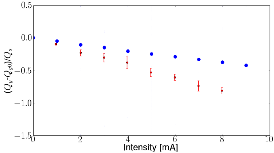
Figure 5.7: Normalized tune shift as predicted with HEADTAIL simulation (blue) based on the current impedance model and as measured (red) when the IVUs were closed.
