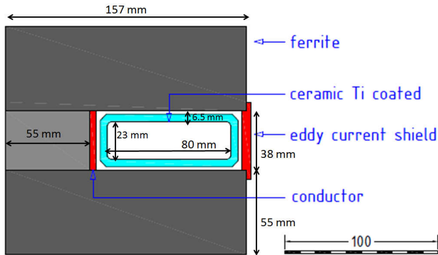
Figure 5.9: Cross section of the injection kicker.
