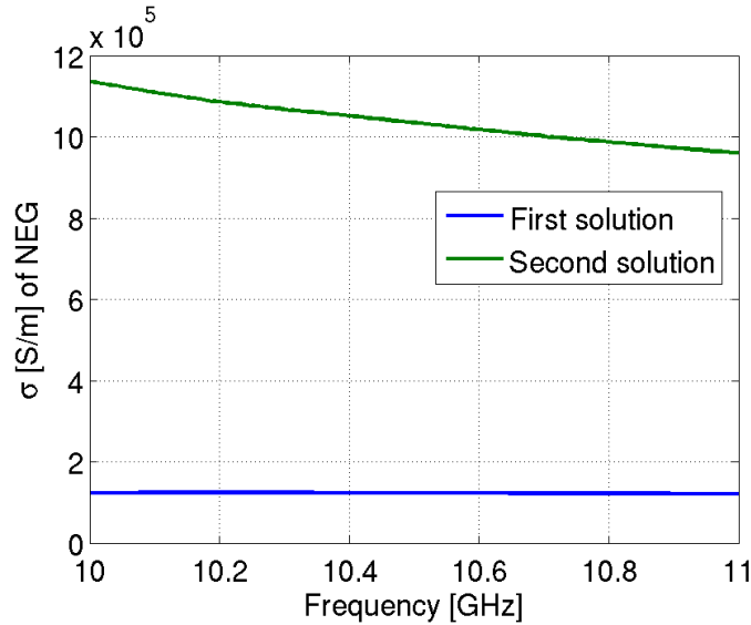
Figure 4.16: Effective conductivity of NEG.
