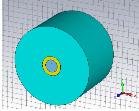
Figure 5.11: CST 3D model of a round multilayer structure with 11.5 mm radius. The inner layer is ceramic of 6.5 mm thickness (yellow) and the outer layer is Fe of 55 mm thickness (blue).
