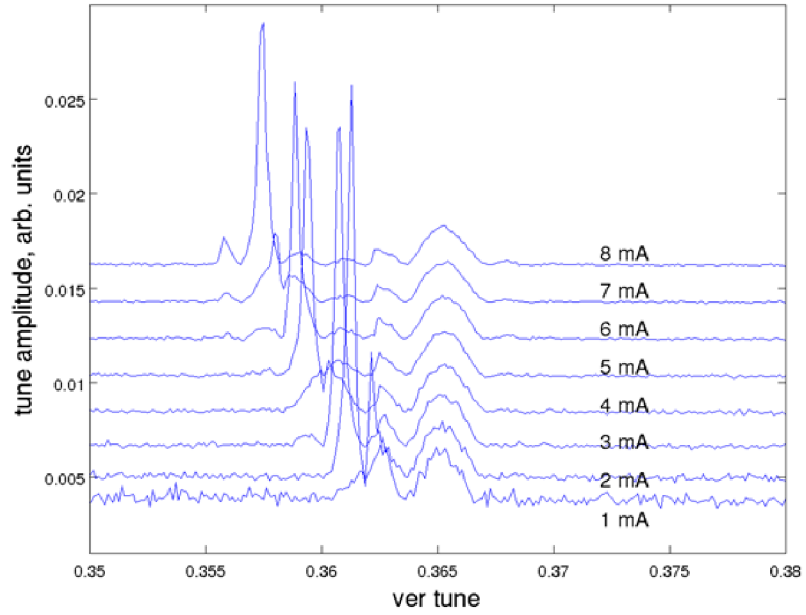
Figure 5.2: Tune monitor for closed IVUs [75]. Mode 0 shifts down as current increases and mode -1 appears before the instability onset (8.8 mA).
