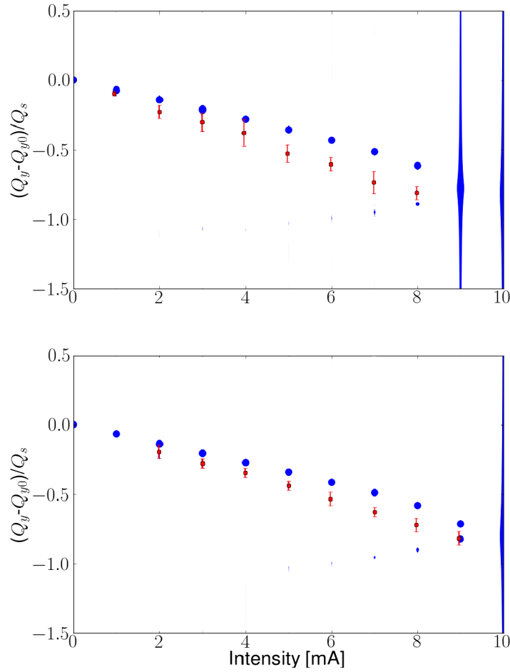
Figure 5.8: Normalized tune shift with HEADTAIL (blue) when a 5 th BBR with f_r=1 GHz, Q=1 and R_s=1.6 \text{ M}\Omega/\text{m} is added in the model. The comparison with measurements (red) is shown. The top plot is for IVUs closed (TMCI from simulation at 9 mA) and the bottom for open (TMCI from simulation at 10 mA).
