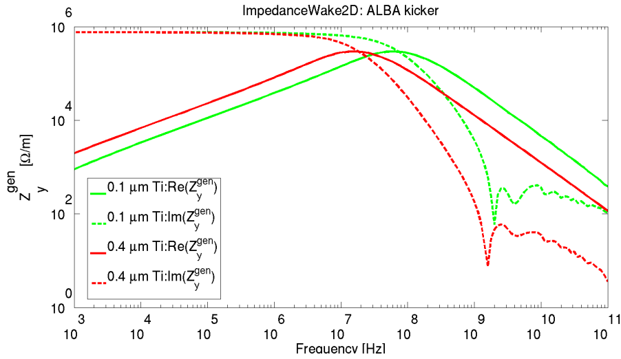
Figure 5.18: Vertical generalized impedance of the ALBA kicker with ImpedanceWake2D. In red, Ti thickness is 0.4 \mu m . In green, a thinner coating is considered of 0.1 \mu m . The absolute value of the imaginary impedance is displayed.
