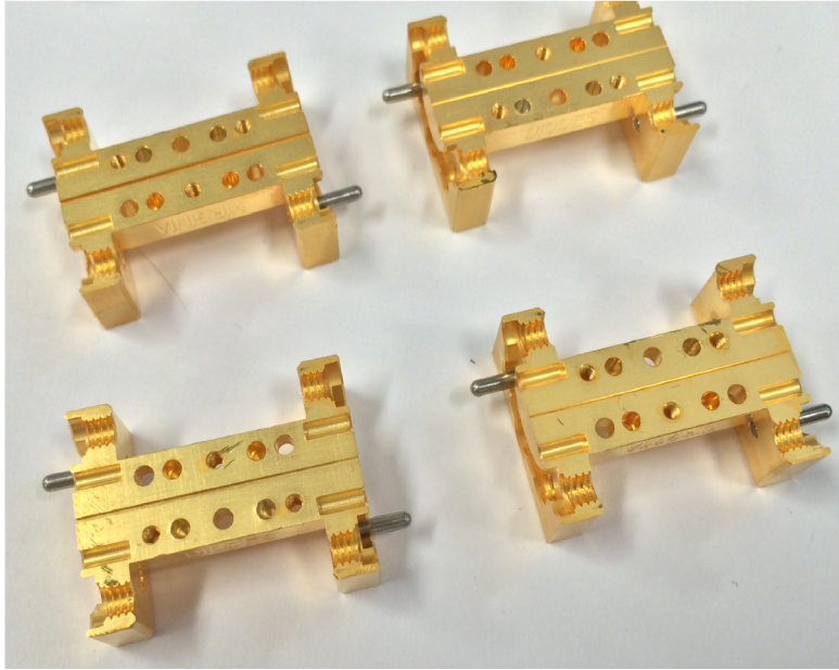
Figure 4.28: WR3.4 (left) and WR1.5 (right) waveguides from VDI made of Aluminum with a thin gold plating.
