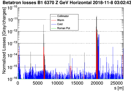
(a) Standard system, full loss map
