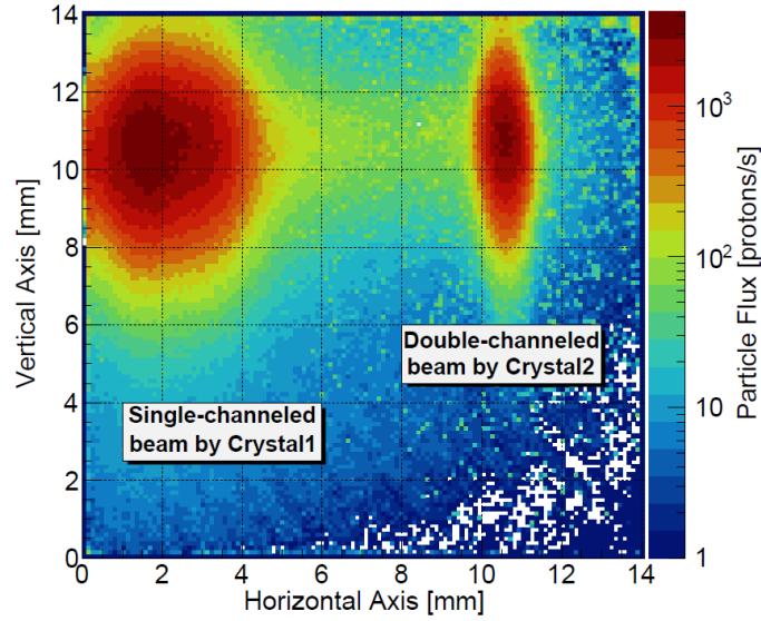
Figure 7.8: Timepix integrated image of the single- and double-channelled beam [120].
