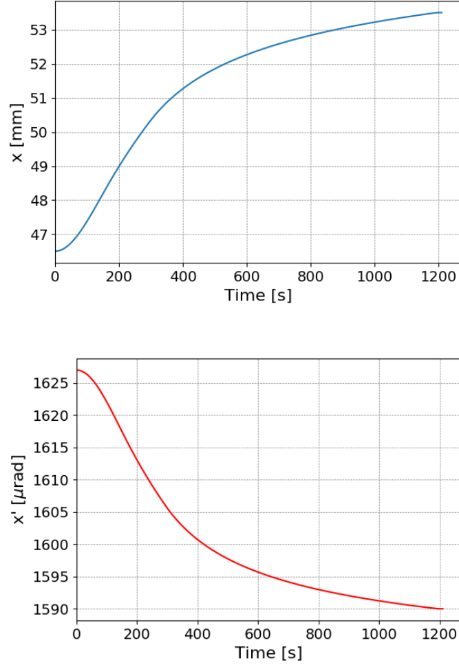
Figure 4.9: Linear (top) and rotational (bottom) ramp functions generated for the horizontal crystal on Beam 1.
