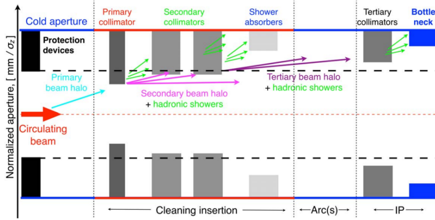
Figure 2.9: Schematic representation of the LHC multistage collimation system [9].
