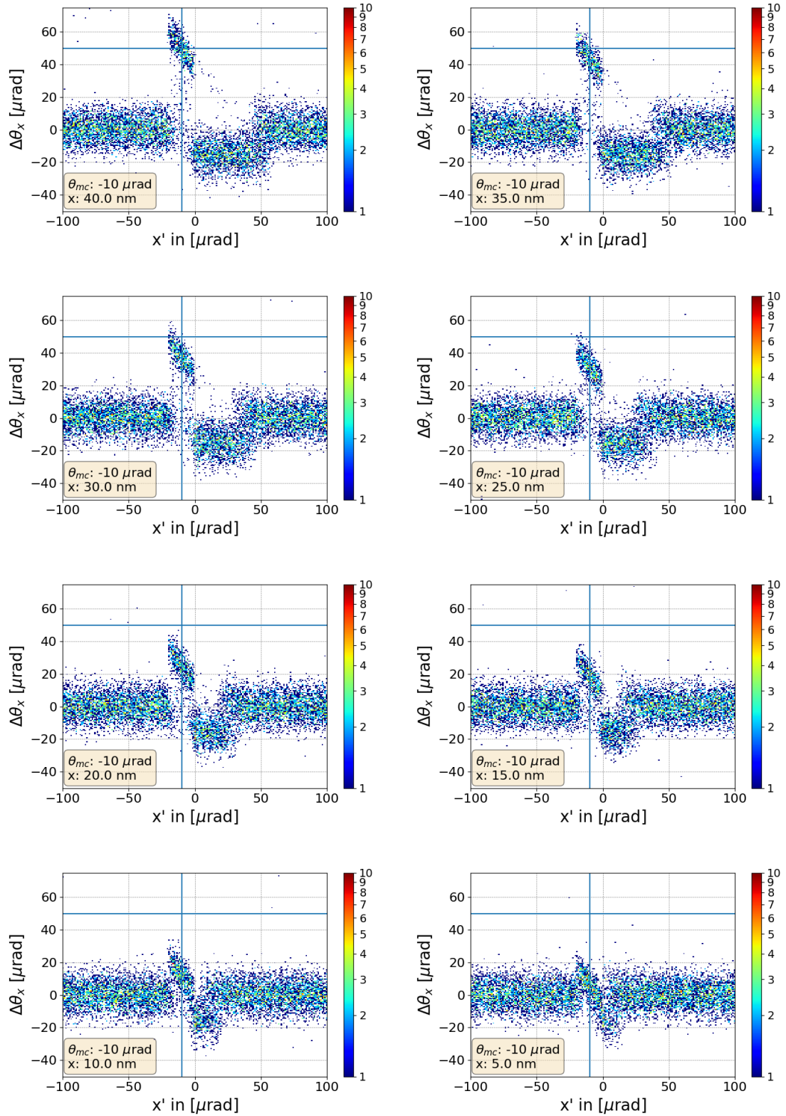
Figure 6.15: Simulated deflection as a function of the impact angle for single-pass interaction of a 400 GeV proton beam. The crystal bending angle is 50 μrad and the entrance face is 3 mm wide along the x direction. The impact parameter of the simulated beam is progressively reduced. The horizontal and vertical lines in each plot indicate the miscut angle and the bending angle of the crystal, i.e. the area where the channeling isle is located if the particles see the full crystal length.
