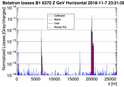
(c) Crystal system, full loss map
