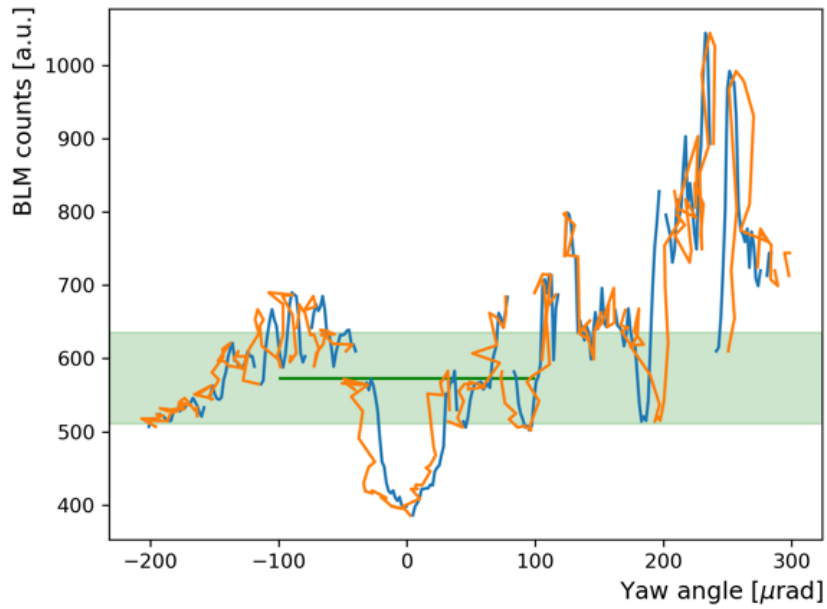
Figure 7.10: Angular scan performed with Crystall1 [78]. The BLM signal is shown as a function of the angular settings given as input to the hardware (orange) and effective angular position measured by the goniometer (blue). A green line indicates the average losses recorded in steady configuration, with the light green band being the standard deviation.
