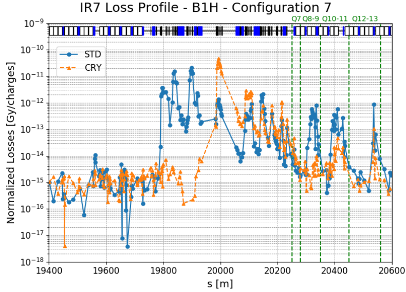
Figure 5.8: Comparison of the BLM signal recorded during loss maps on the horizontal plane of Beam 1 with Pb ion beams at 6.37Z TeV during MD tests, for the standard and crystal system in configuration 7 (see Tab. 5.3 and 5.4 respectively). The signal is normalized to the flux of particles lost during the loss map.
