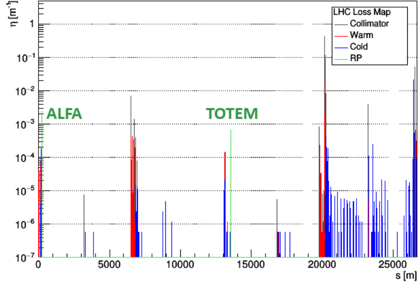
(a) Standard collimation scheme.
