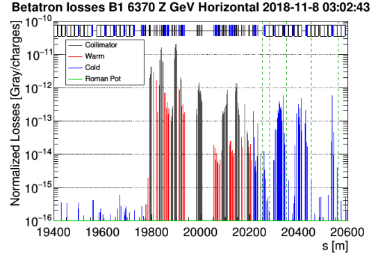
(b) Standard system, zoom in IR7
