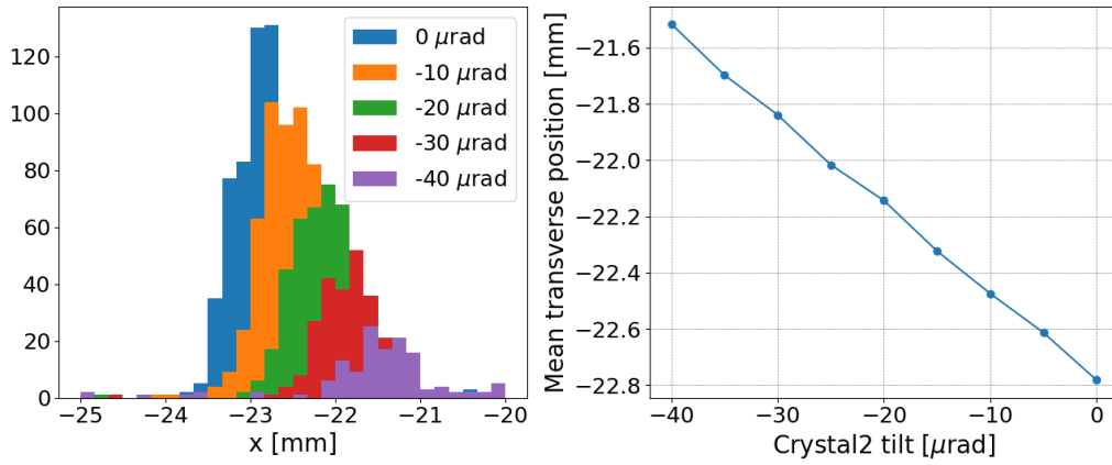
Figure 7.12: Left frame: simulated transverse distribution of the double-channeled beam for different values of angular tilt applied to Crystal2 with respect to the optimal channeling orientation. Right frame: mean transverse position of the simulated double-channeled beam as a function of the tilt applied to Crystal2.
