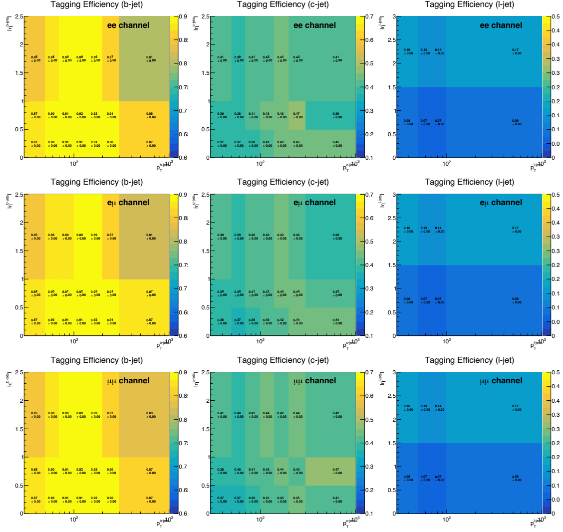
Figure F.3: The b-tagging efficiency and mistag rates are computed in bins of jet p_T and \eta and are shown for 2018 in the e^\pm e^\mp (top row), e^\pm \mu^\mp (middle row) and \mu^\pm \mu^\mp (third row) channels. The b-tagging efficiency is shown in the first column while the mistag rates for c- and light-jets are shown in the second and third column, respectively.
