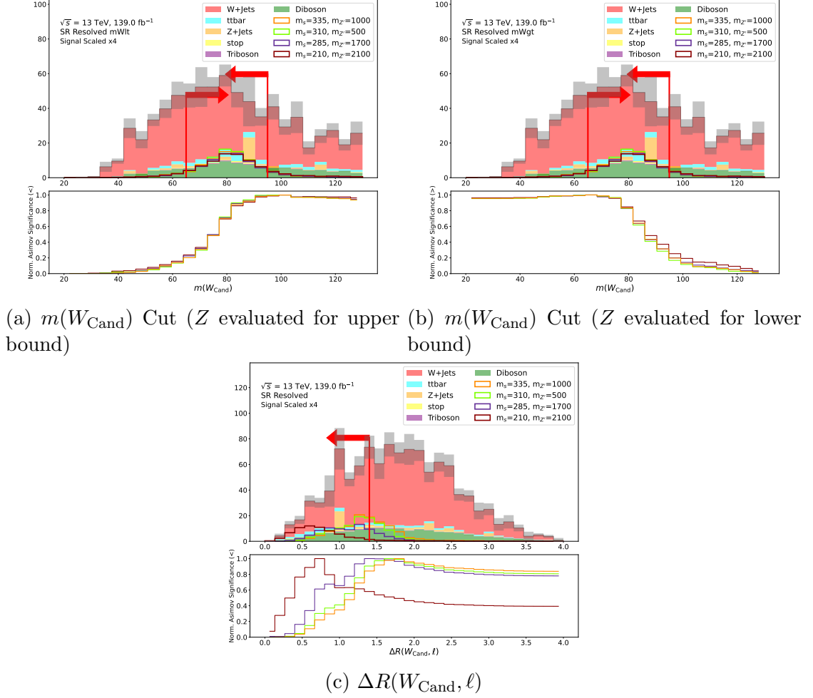
Figure 5.11: N-1 Distributions for the m(W_{\text{Cand}}) and \Delta R(W_{\text{Cand}}, \ell) variables used in the resolved signal region definition. Grey bands show statistical uncertainty on the background estimate. The lower panel shows the cumulative Asimov significance normalized to unit peak, where the direction ( > or < ) specified in the y label indicates whether the significance is being summed from above ( > ) or from below ( < ). Red vertical line and arrow show placement and direction of selection on the given variable in this region.
