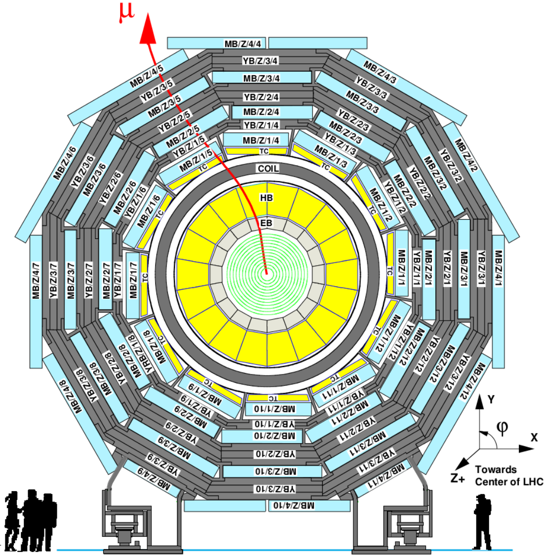
Figure 3.14: Transverse view of one of the five wheels with Drift Tube chambers in the barrel region of the CMS.
