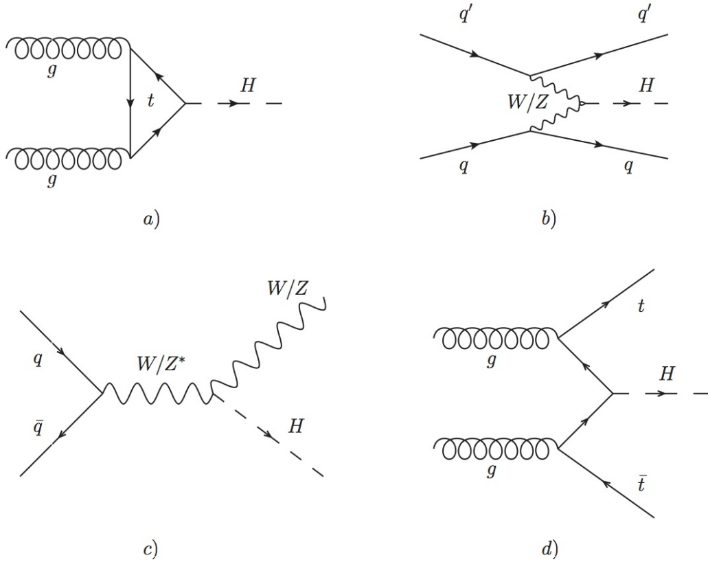
Figure 2.2: Main production modes of the Higgs boson using proton-proton collisions at LHC: gluon-gluon fusion (top left), vector boson fusion (top right), production with associated production of a vector boson (bottom left) or t\bar{t} (bottom right) (from [35]).
