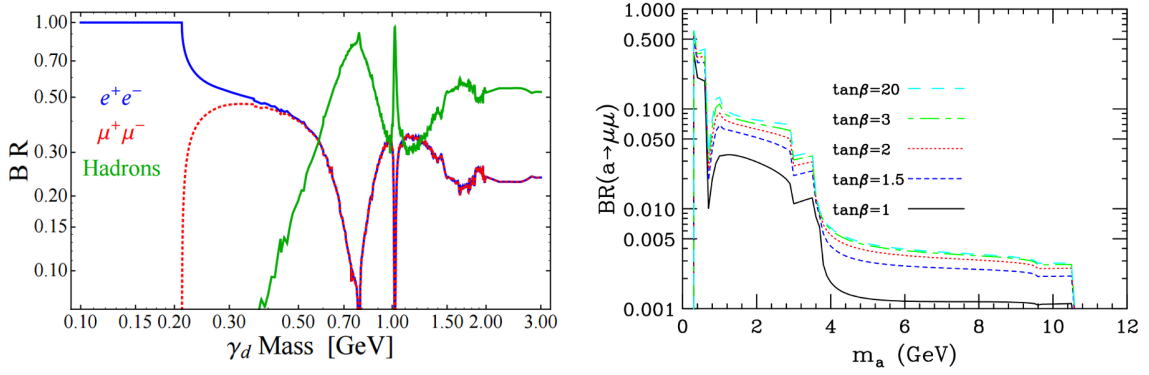
Figure 2.5: Branching ratios of decays into pairs of muons of new light vector (left, red dotted line) and scalar (right) bosons, \gamma_d and a , respectively (from [108, 109]).
