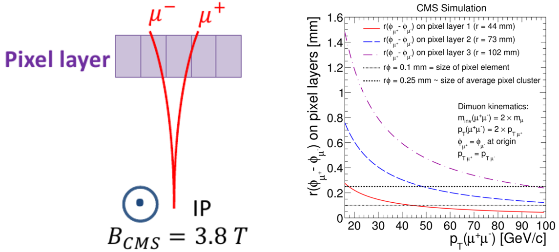
Figure 5.4: Left: sketch of the two close muon tracks of opposite sign crossing pixel layer in adjacent elements forming single shared cluster. Right: distance between two muon tracks in r - \phi plane on three barrel layers of pixel tracker vs. transverse momentum of the dimuon ( p_T(di-\mu) = p_T(a_1) ) in the threshold case with m(di-\mu) = 2 \times m(\mu) . Size of pixel element and typical cluster size are also shown as dashed horizontal lines.
