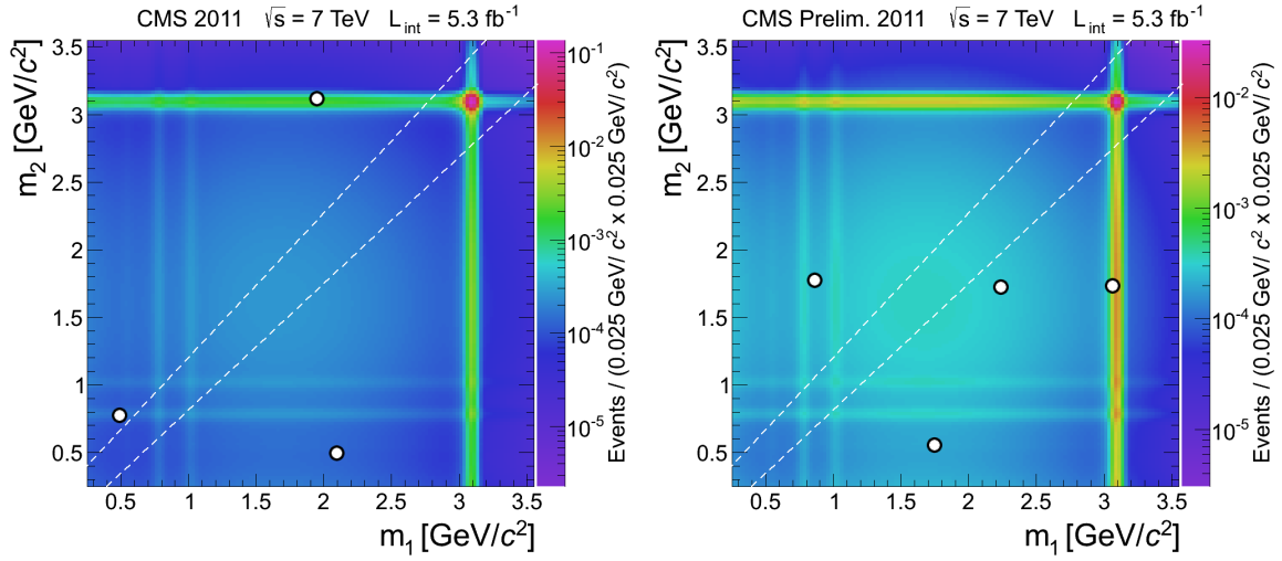
Figure 5.25: The distribution m_1 versus m_2 of masses of the dimuons for data events (shown as empty circles) surviving all selections except the requirement that these two masses fall into the diagonal signal region m_1 \approx m_2 (outlined with dashed lines). The background expectation (shown in color) is a sum of the b\bar{b} (2D template normalized to number of events in the off-diagonal region) and the direct J/\psi J/\psi production contributions. Left: the analysis tight isolation requirement for dimuons applied ( Iso_{di-\mu_{1,2}} < 3 GeV). Right: loose isolation requirement for dimuons applied ( 3 < Iso_{di-\mu_{1,2}} < 8 GeV).
