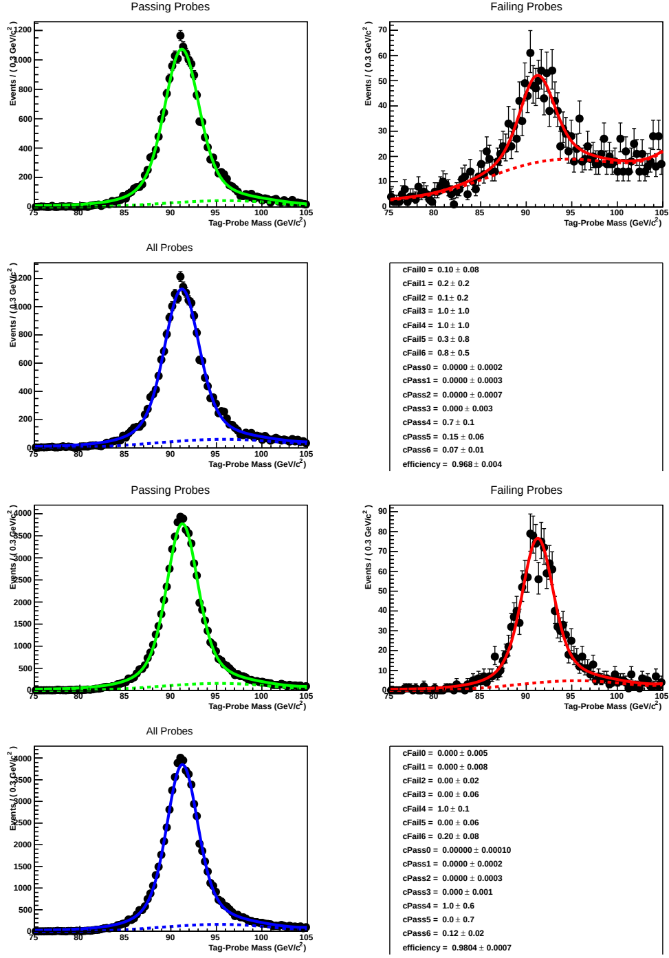
Figure 5.21: Distributions of dimuon masses consistent with Z mass (from 75 to 105 GeV) containing passing, failing, and all probe muons with p_T from 40 to 60 GeV in tag and probe study of the analysis muon identification efficiency. Top four: data; bottom four: MC.
