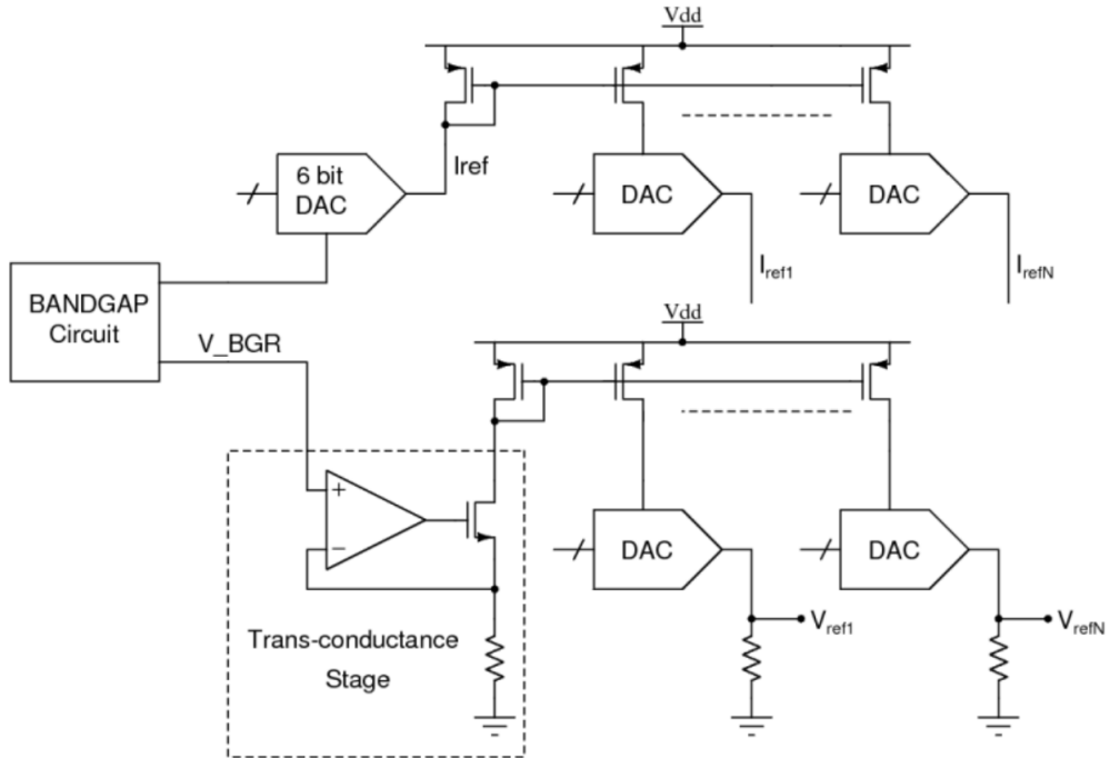
Figure 3.8: The architecture of the VFAT3 bias block.
