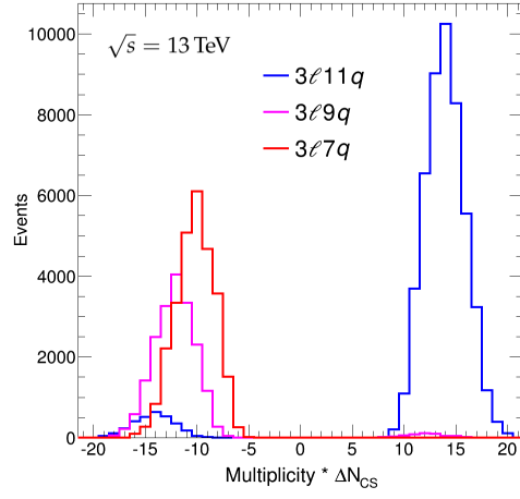
Figure 4.13: The distributions of multiplicities of energetic ( p_T > 20 \text{ GeV} ) jets and leptons within a nominal fiducial detector acceptance of |\eta| < 2.5 , after processing with PYTHIA, including top quark and W decays, as well as jet fragmentation and hadronization. The multiplicities are plotted separately for N_{CS} = \pm 1 by multiplying them by N_{CS} , and are shown separately for each of the possibilities for number of quark-antiquark cancellations (0, 1, and 2).
