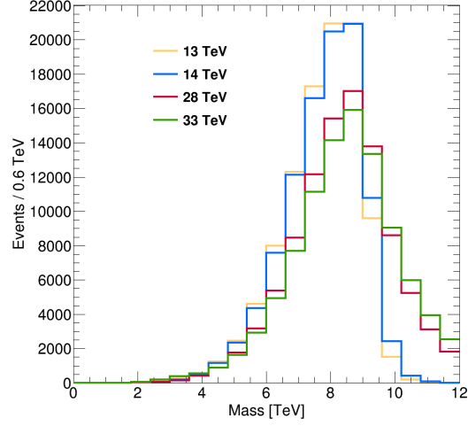
Figure 4.11: Invariant-mass distributions of observable final-state particles in simulated LHC collisions at 13, 14, 28, and 33 TeV. These simulations are made with the nominal E_{Sph} = 9 TeV.
