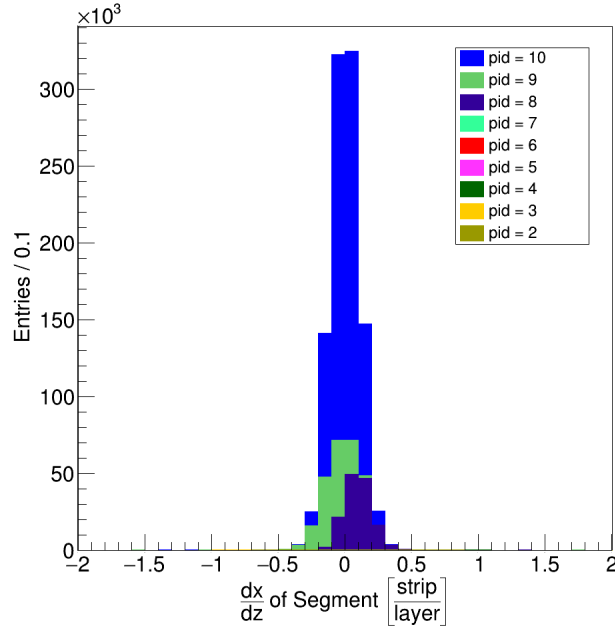
Figure 2.13: The segment slope distribution in ME1/2 broken up by associated CLCT PID.
