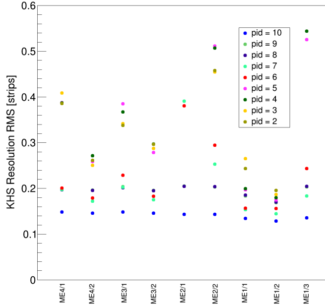
Figure 2.20: The RMS of the LCT position resolution distributions for each CLCT PID separated by chamber type.
