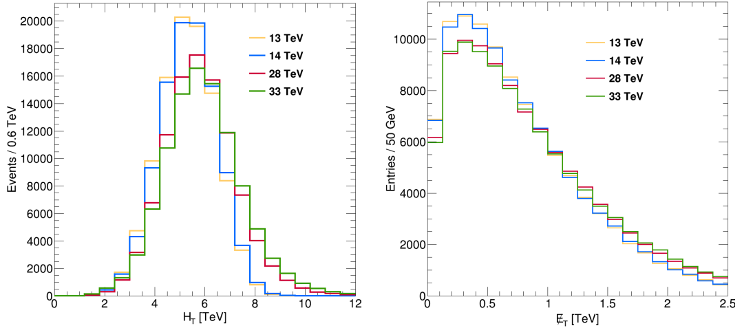
Figure 4.12: Left Panel: Distributions of the scalar sum of p_T^{jet} of events in simulated LHC collisions at 13, 14, 28, and 33 TeV. Right Panel: Distributions of E_T in simulated LHC collisions at all four energies. These simulations are made with the nominal E_{Sph} = 9 TeV.
