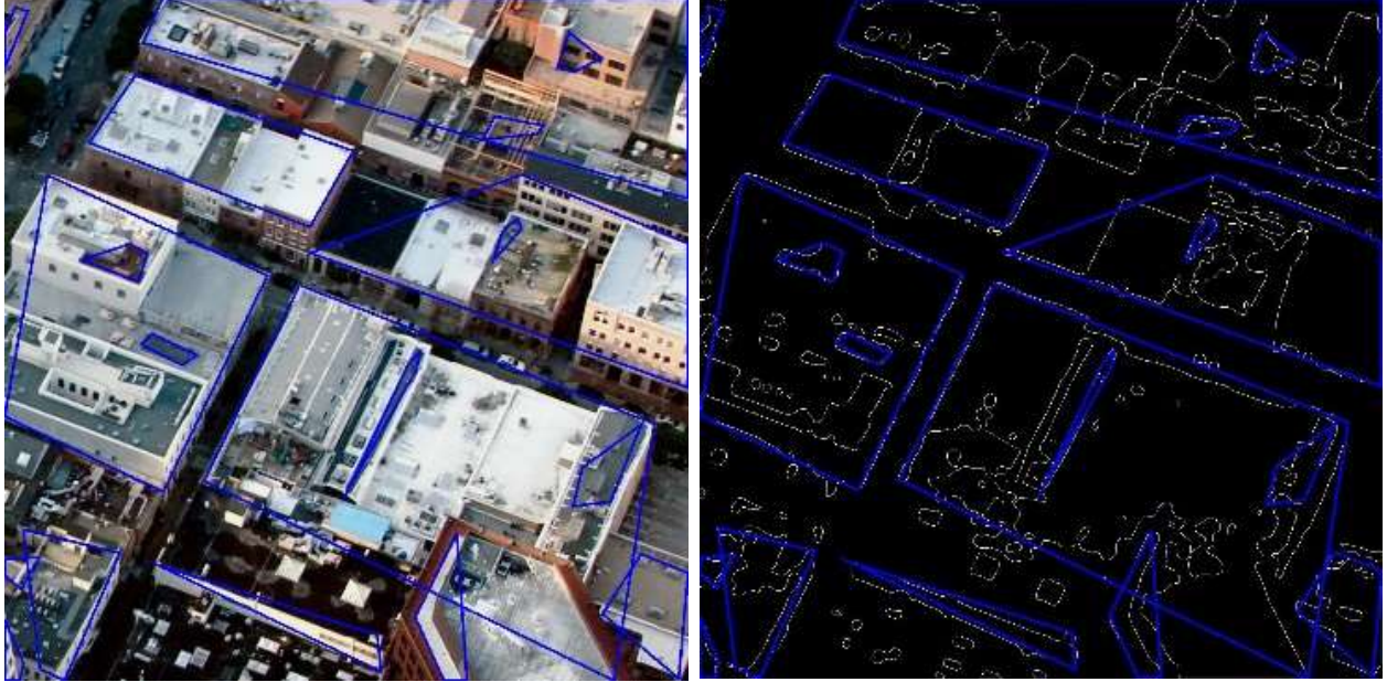
Figure 33 represents the images introduced in Figure 13 after Figure 14's steps 1, 2, 3, 4, 5 and 6.b, Shape hulling using Graham scan algorithm. The right image presents shape contouring directly applied on the original image for comparison.
