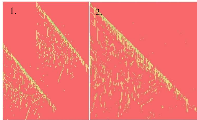
Figure 15 Results of brightness correction and matching between a pair of images. The closer the color is to green; the more points were found with a combination of brightness correction. 1) a pair of images before histogram normalization, 2) the same pair after histogram normalization.
