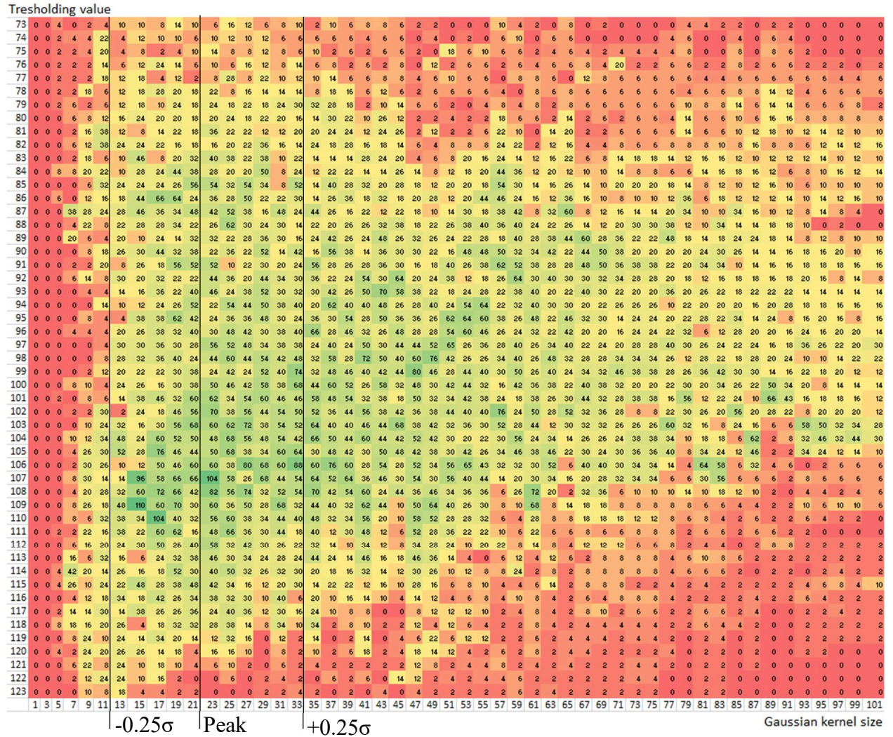
Figure 23 Partial blob match count between two pairs of images depending on Gaussian Kernel size (X) and Thresholding value (Y). Overlaid, the statistical peak of point found on a dataset, as described later in the document.
