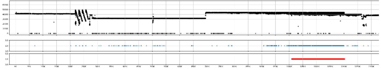
Figure 72 Illustration of the labelling obtained from a sample of LINAC 4's data with in black, the signal, in blue the labelling obtain from label-related clustering and in in red labelling estimation by domain expert
