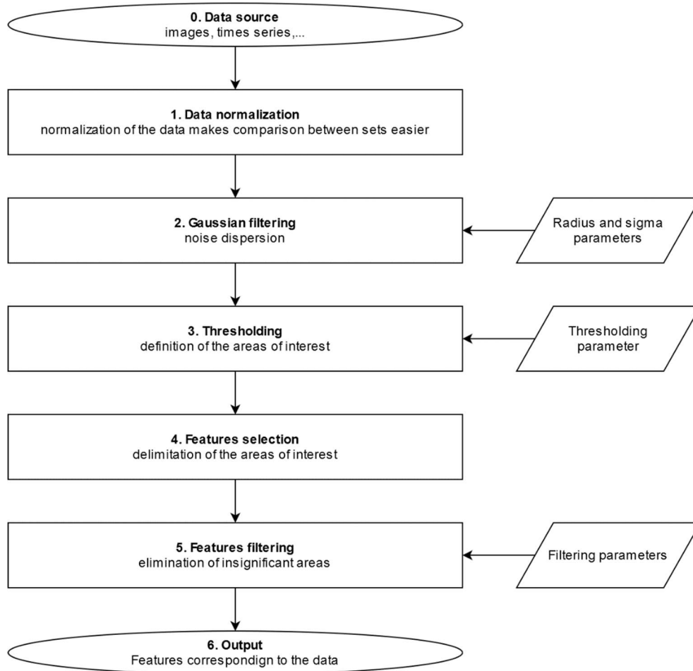
Figure 3 Representation of the algorithm presented in this thesis independently from the type of data that is to be treated.
