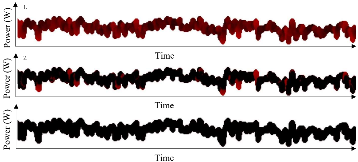
Figure 82 shows a data sample containing no jittering periods but rich in noise with 1. A data sample after blurring, red shades indicate likelihood. 2. A data sample after thresholding and 3. a data sample after filtering. After the third stage, no false positive area remains. The image colorimetry has been altered from the original content in order to highlight color differences.
