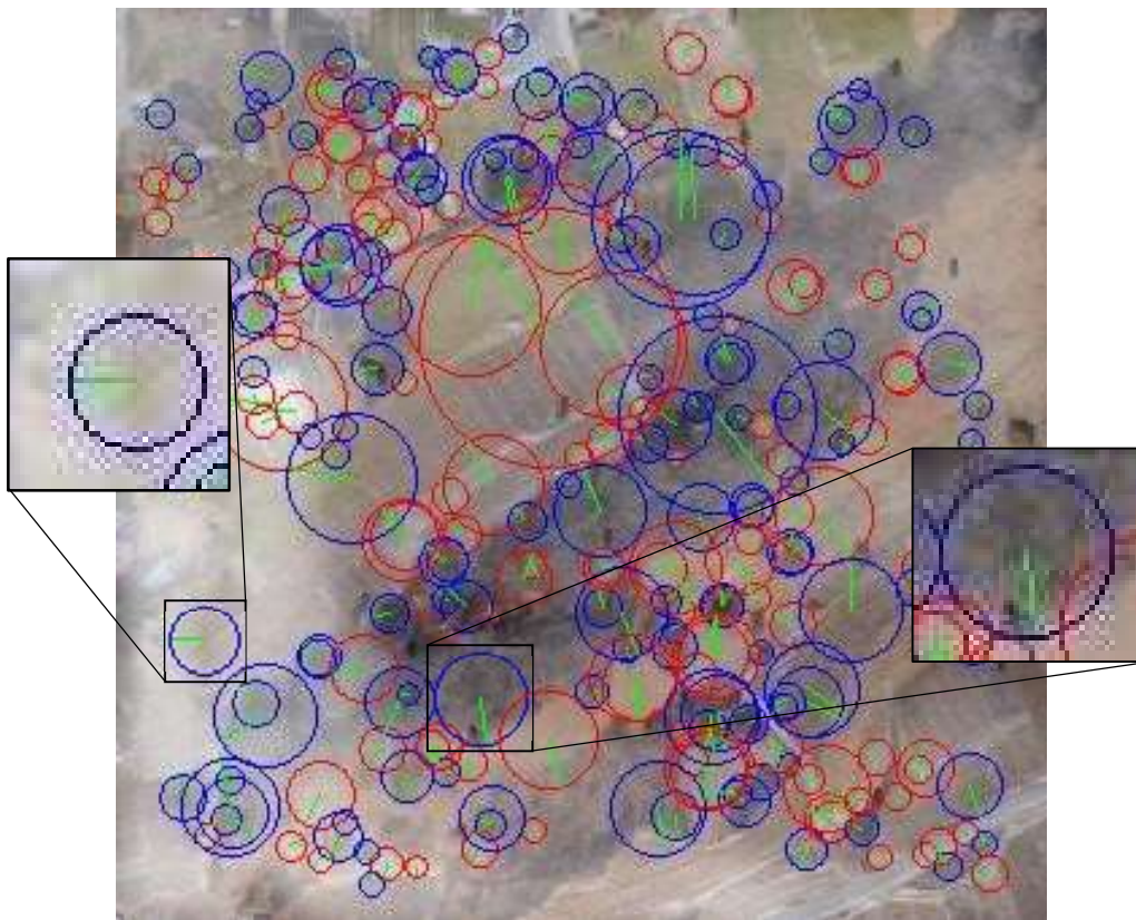
Figure 8 Shows a SURF implementation for features detection, using the Accord.net framework. The image shows how the technique is influenced by noise.
