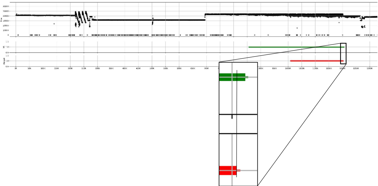
Figure 86 Illustration of the labelling obtained from a sample of LINAC 4’s data with in black, the signal, in green the labelling obtain from SNiF and in in red labelling estimation by domain expert.
