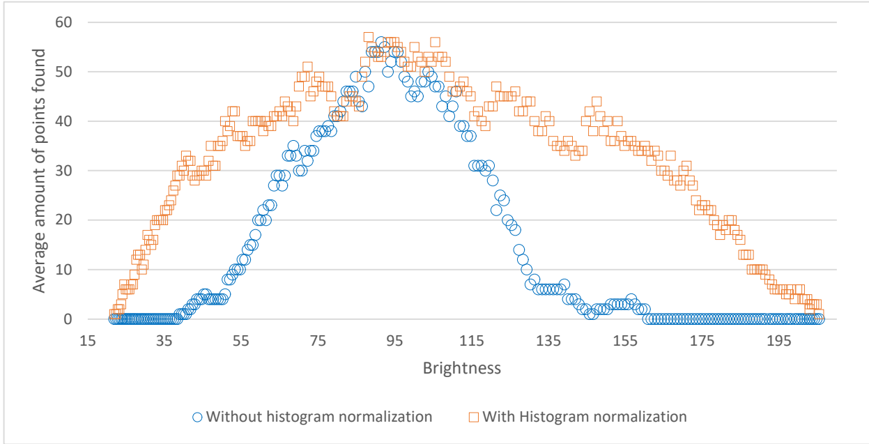
Figure 19 Represents the distribution of points found with and without brightness normalization. The curb using brightness normalization has a significantly higher variance. (Yann Donon R.).
