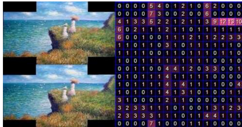
Figure 37 Comparison between two successfully matched pictures, with a Bhattacharyya difference index of 1.5%. Between the original mage (top) and stitched image (bottom), no difference appears to the human eye.
