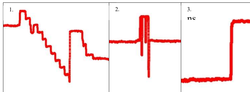
Figure 66 Examples of power modifications resulting from human operations on the source (Yann Donon A., 2019).
