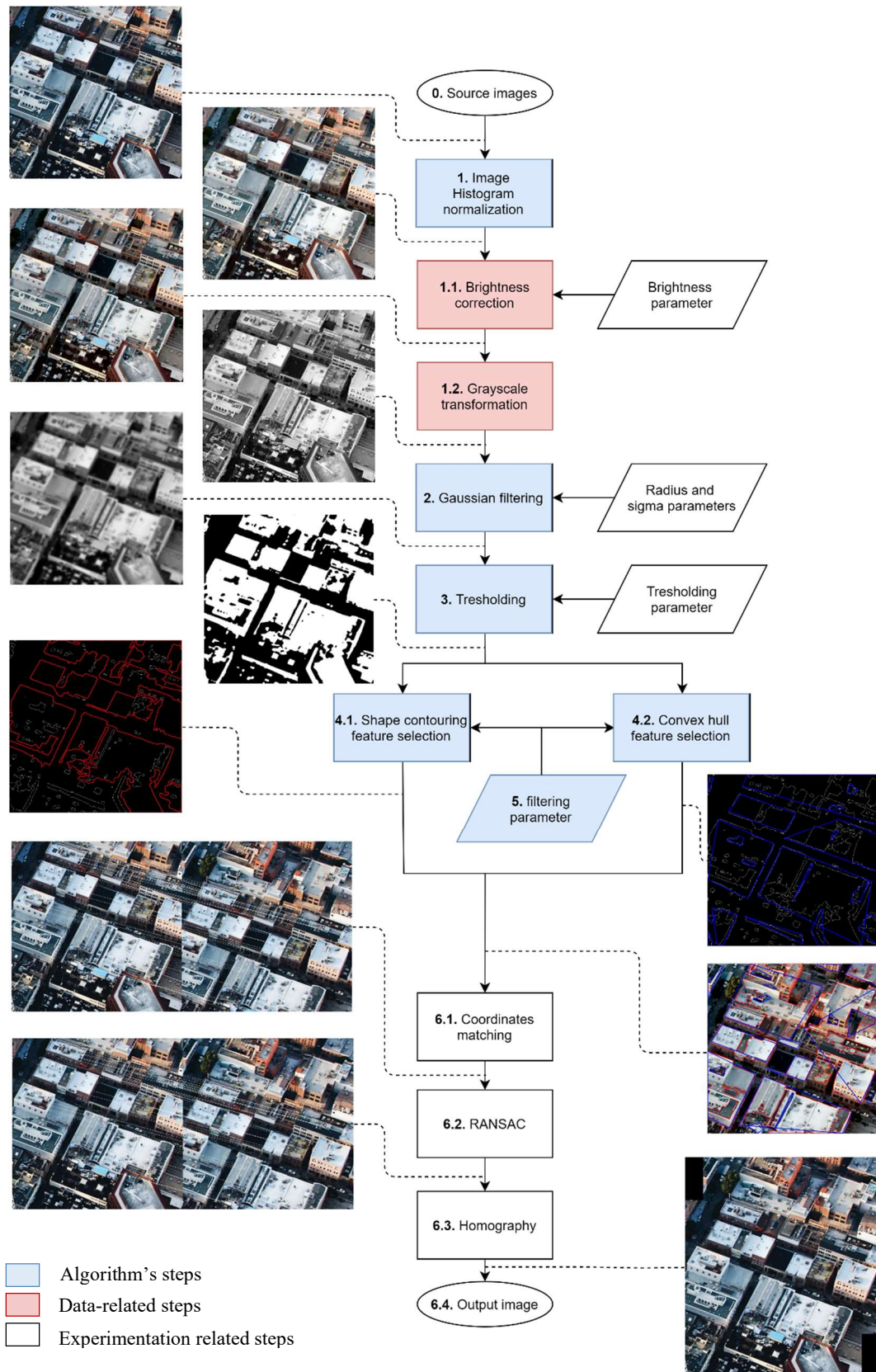
Figure 14 Illustrated BIM process used for image stitching.
