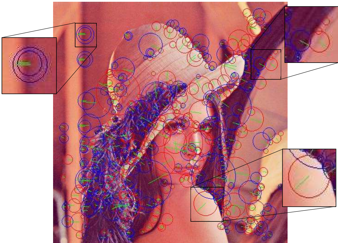
Figure 7 Shows an image on which SURF feature detection has been applied. Circles' center represents points selected by SURF as significant for a comparison. Enlarged fragments of the images shows three points locations characteristic of the technique.
