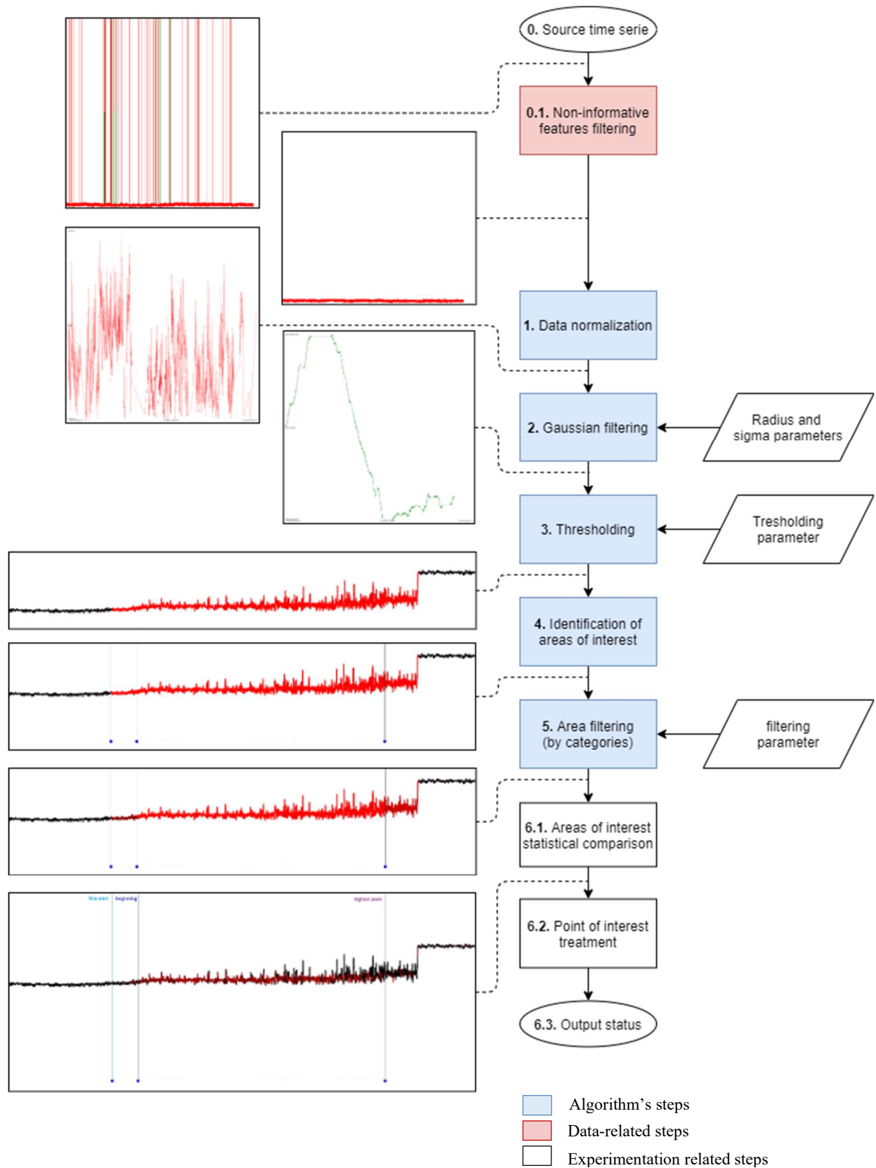
Figure 79 Illustrated SNiF process used for time series analysis
