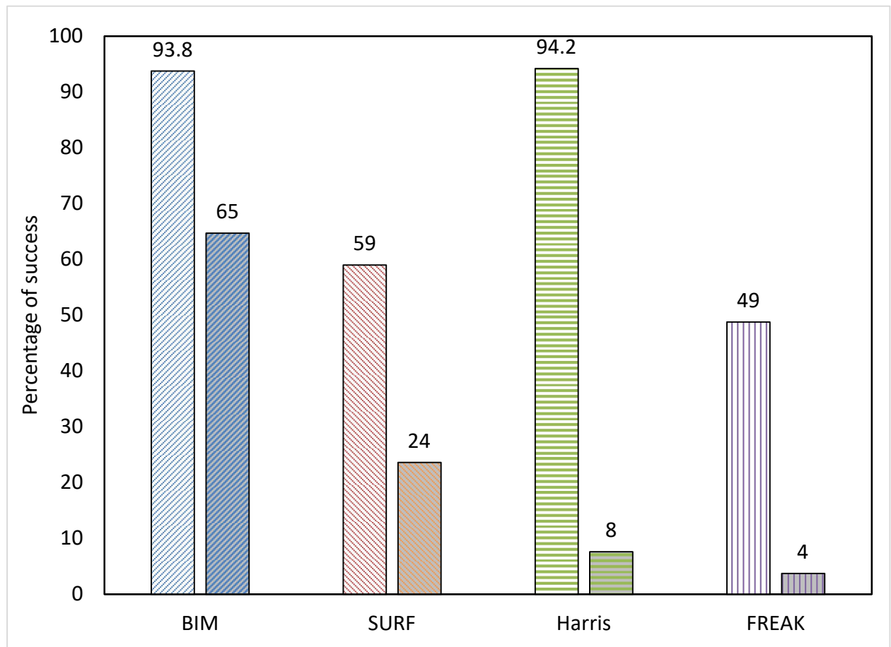
Figure 42 Techniques' success rate comparison in percent, on both sets. In this figure BIM presents the second highest performance on the regular set and the highest on the blurred set.
