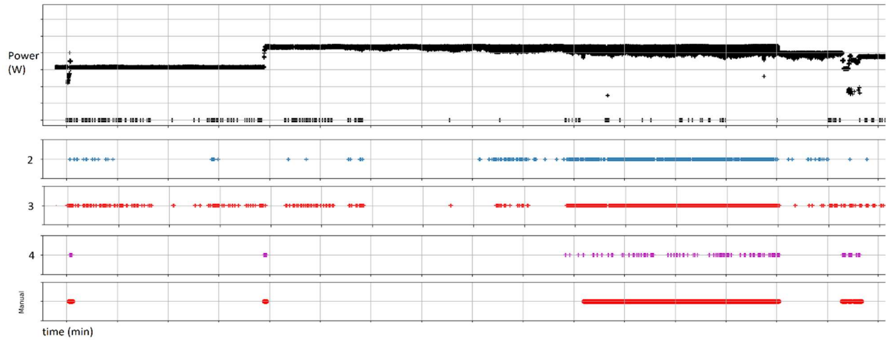
Figure 2 LINAC 4's data anomaly detection using existing techniques (Labelled 2, 3, 4), compared to the original labelling. All techniques show significant imprecisions when compared to the original labelling.
