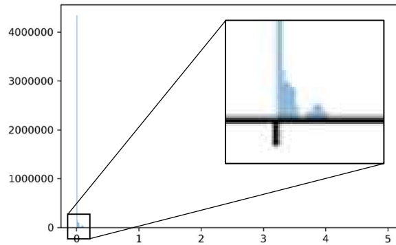
Figure 73 Coefficient of variation distribution graph.
