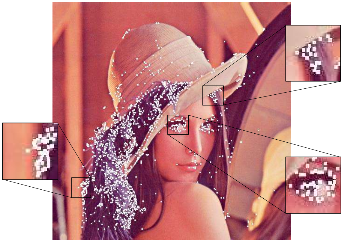
Figure 9 Shows an image on which FREAK feature detection has been applied. Circles' center represents points selected by FREAK as significant for a comparison. Enlarged fragments of the images shows three points locations characteristic of the technique.
