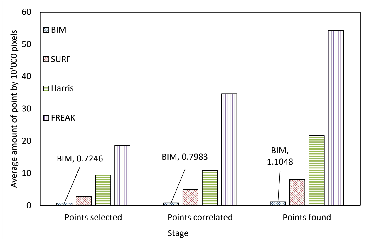
Figure 40 Average points found by technique on 10k pixels images. This figure highlights how fewer points are selected by BIM compared to other techniques.
