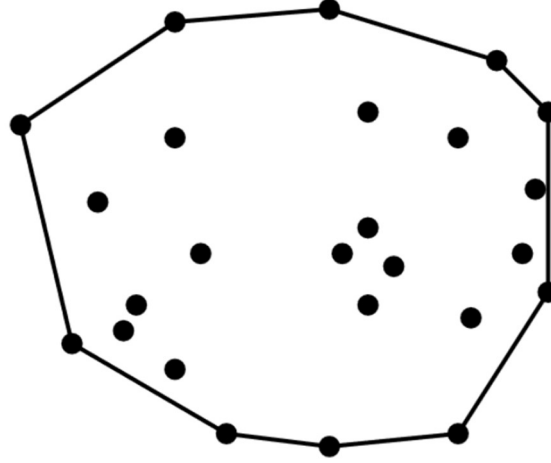
Figure 32 Convex hull H application example on a set of points Q . (Mount, 2012)
