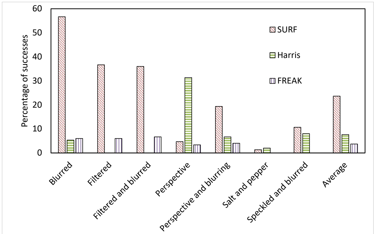
Figure 1 Success rate of Surf, Harris and FREAK in stitching together images issued from a noised dataset described later in 3.7 Results. *(Y Donon et al, 2019)
