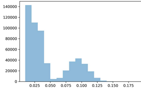
Figure 74 Fragment of coefficient of variation distribution graph [0.01-0.2] containing two clusters (Yann Donon A.)
