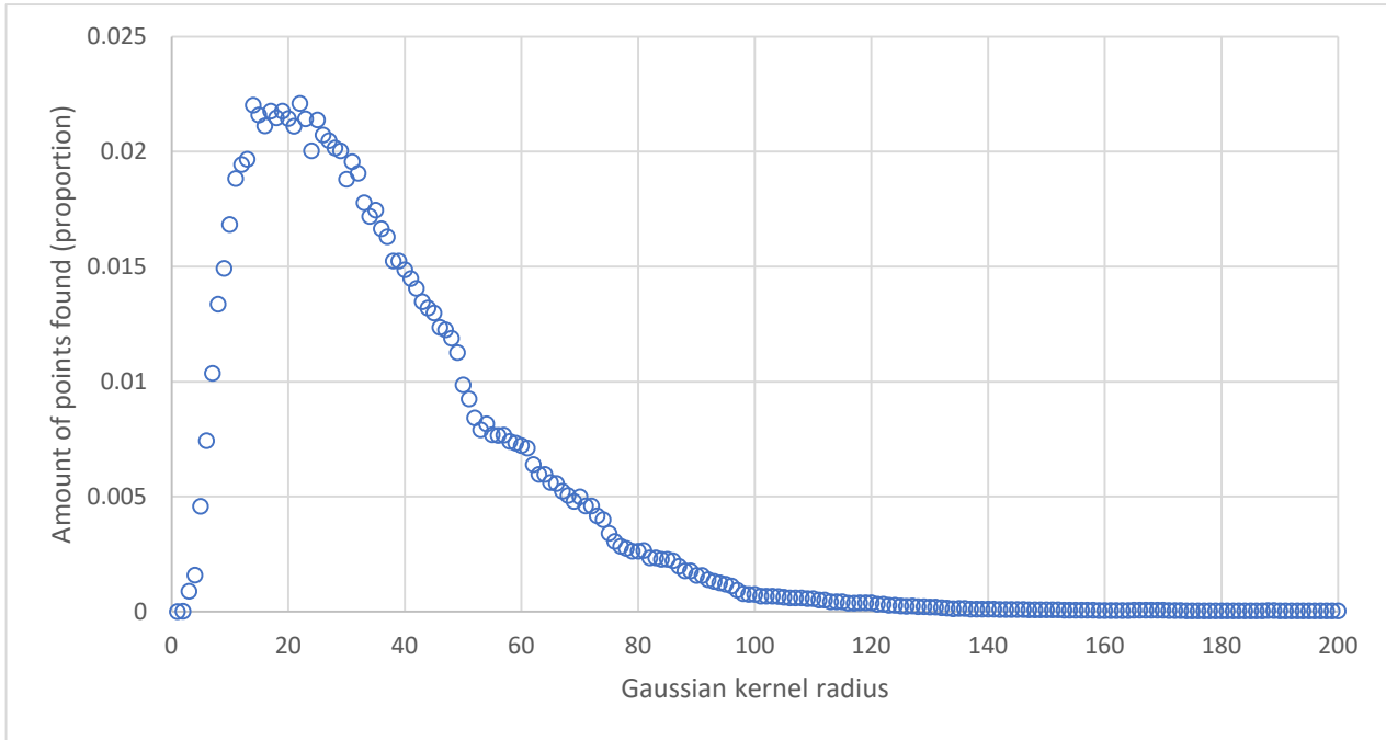
Figure 24 Statistical repetition of points found depending on Gaussian kernel size.
