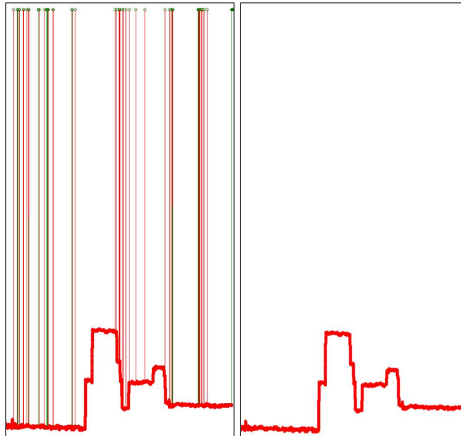
Figure 80 Same fragments before filtering using Grubb's test (left) and after (right) The fragment contains about 50'000 entries, less than 1 % of data were filtered out (Yann Donon A.).
