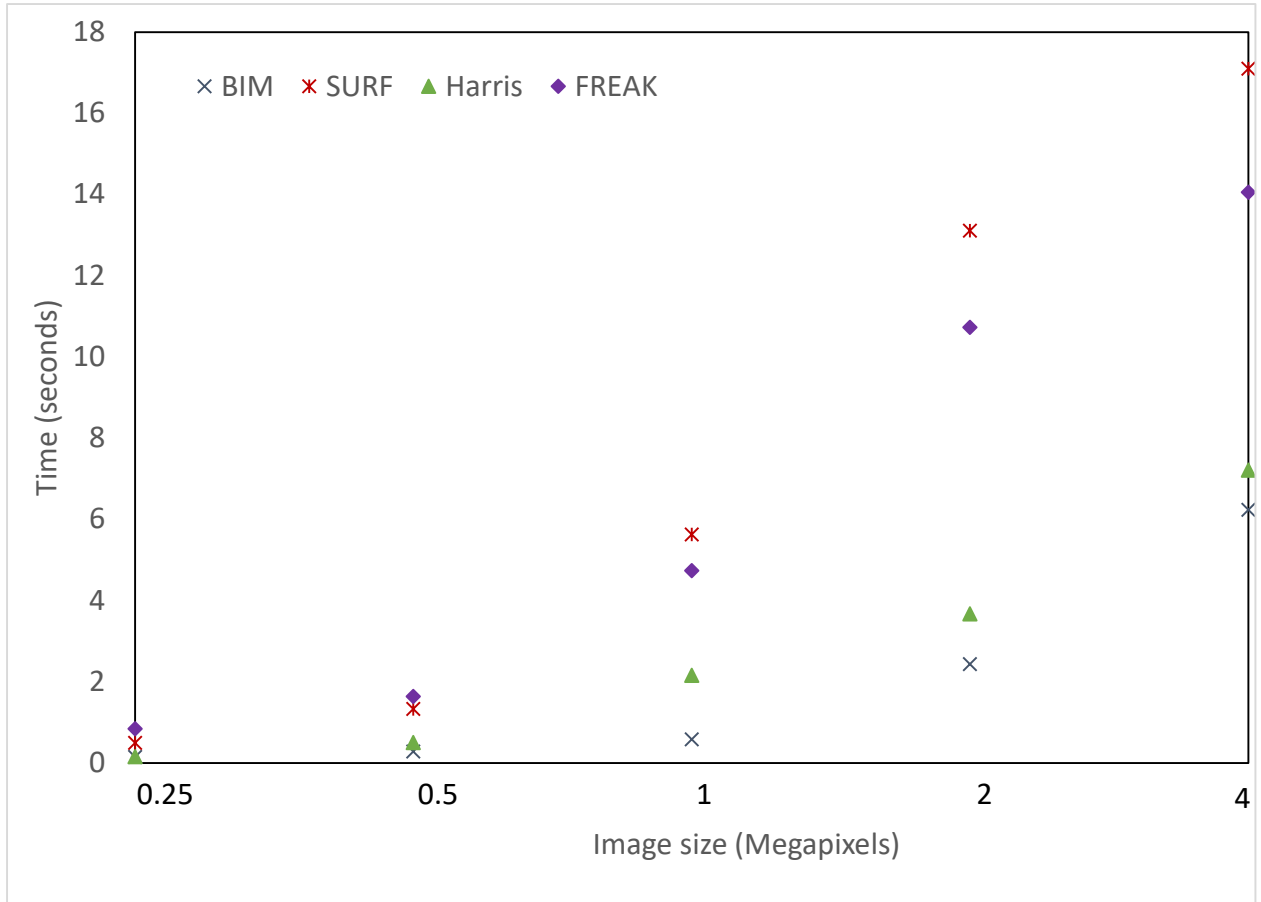
Figure 39 Computation time comparison between the different techniques. In this figure BIM stitching takes significantly less time than with other techniques, independently from image sizes.
