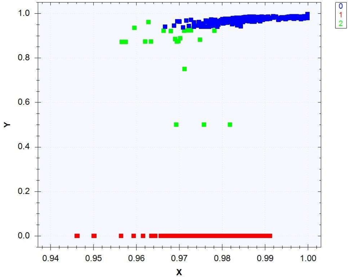
Figure 83 shows the clustering of a thousand windows stochastic matrices, with in blue regular operations, in green human interactions and in red periods of jittering.
