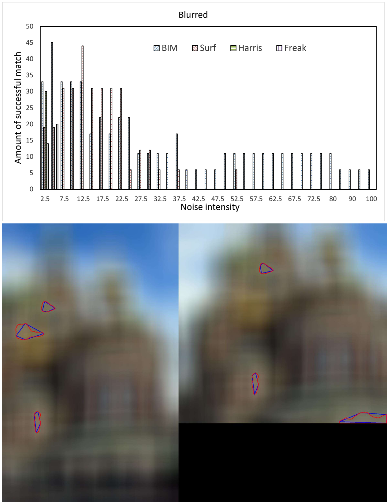
Figure 49 Amount of image successfully stitched depending on blur intensity, with a sample of image at the maximum noise tolerance. In red, key points selected as described in Shape contouring blobs comparison chapter and in blue key points selected as described in Convex hull blobs comparison chapter.
