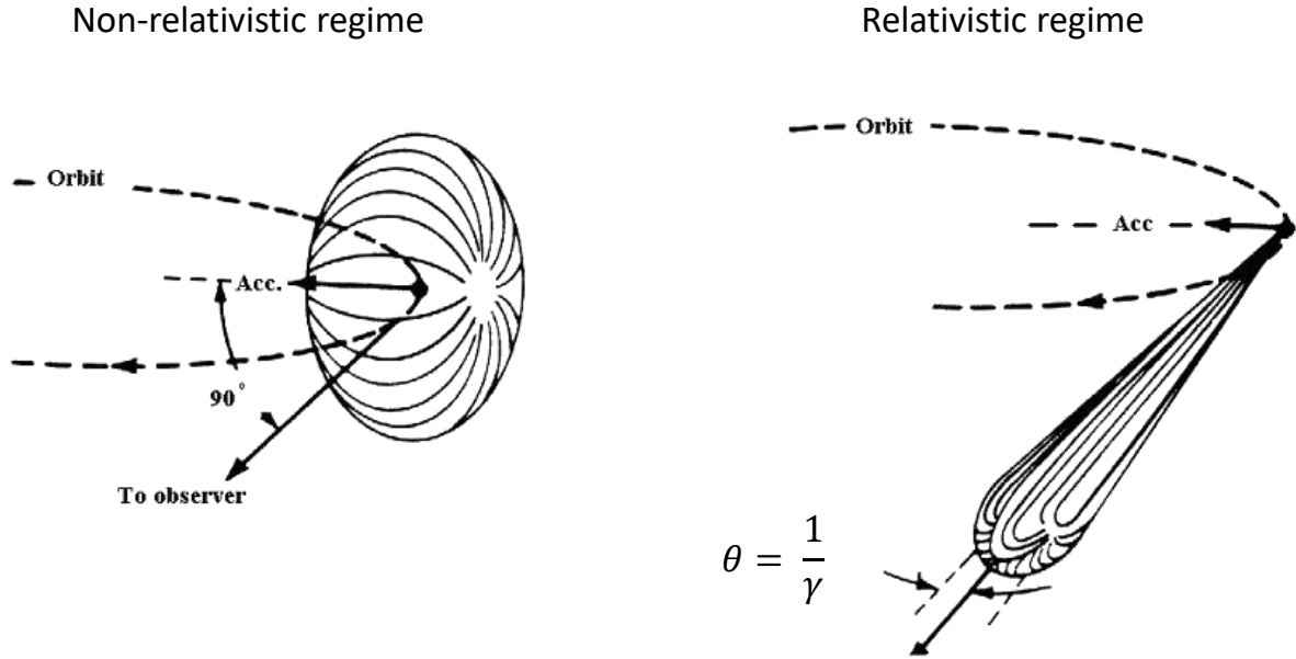
FIGURE 4.1: Qualitative radiation patterns from electrons in a circular orbit at low energy (left) and as distorted by relativistic transformation at high energy (right) [70].
