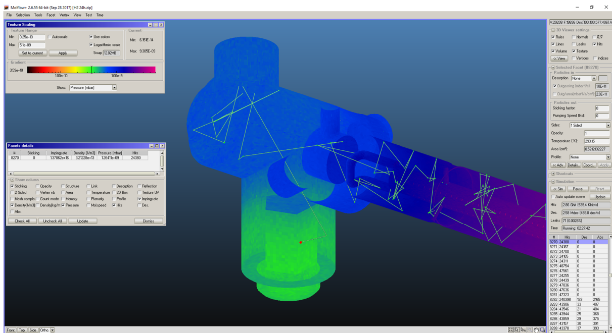
FIGURE 3.1: Example of a Molflow+ Monte Carlo simulation, showing a modelled NEXTor pump installed in BESTEX. The trajectories of each molecule (in green) are traced until being pumped (red dot, on the pump’s surface).
