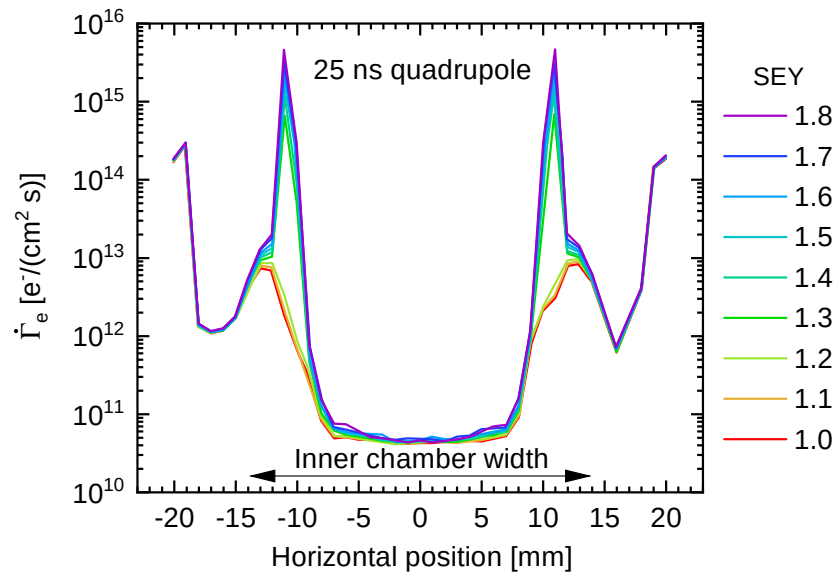
FIGURE 4.54: Horizontal projection of \dot{\Gamma}_e in a quadrupole FCC-hh BS with a 360 T/m magnetic field, as a function of the SEY. Nominal beam parameters. Taken from [74].
