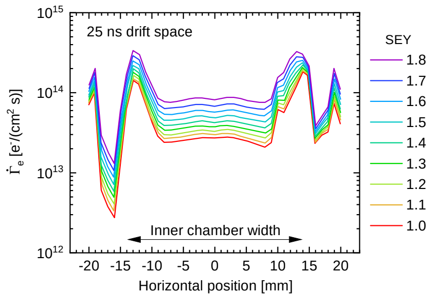
FIGURE 4.55: Horizontal projection of \dot{\Gamma}_e in the FCC-hh BS in the inter-connection area, with no magnetic field, as a function of the SEY. Nominal beam parameters. Absorber slope treated with LASE. Taken from [74].
