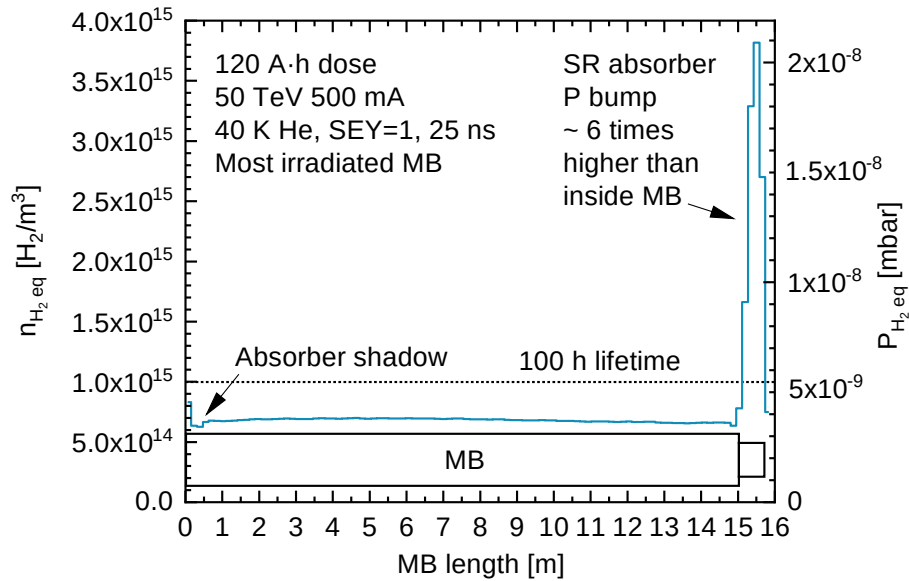
FIGURE 4.58: \text{H}_2 equivalent gas density profile of the most irradiated MB in the arcs, for a 120 Ah beam dose. Calculated for a 50 TeV, 25 ns, non ideal proton beam.
