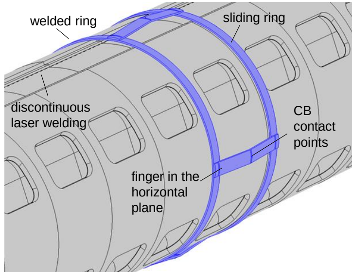
FIGURE 4.36: Supporting system of the FCC-hh BS [79].
