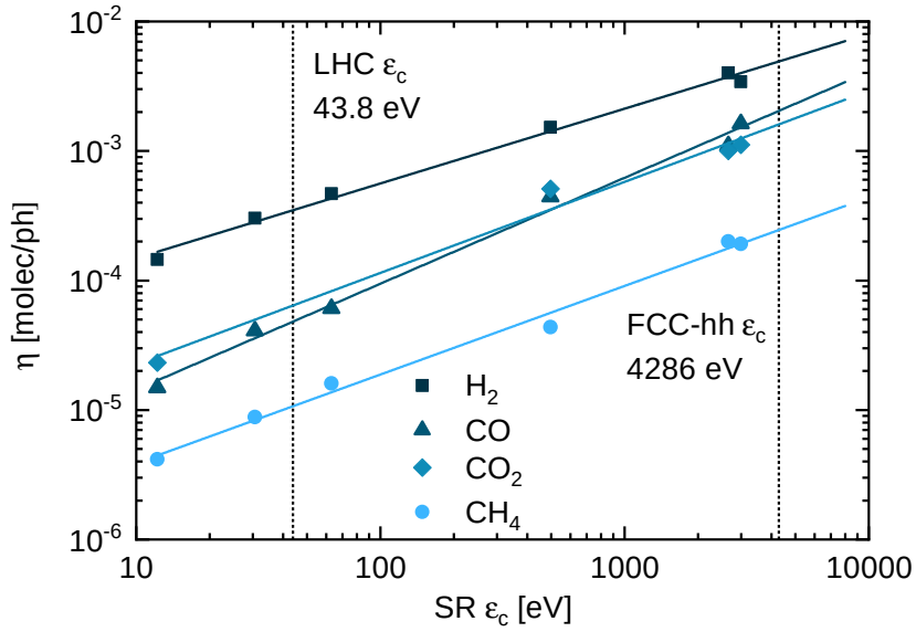
FIGURE 4.50: \eta_{ph} dependence on \epsilon_c for RT baked Cu measured at a common dose of 2.5 \times 10^{20} ph/m [135, 136].
