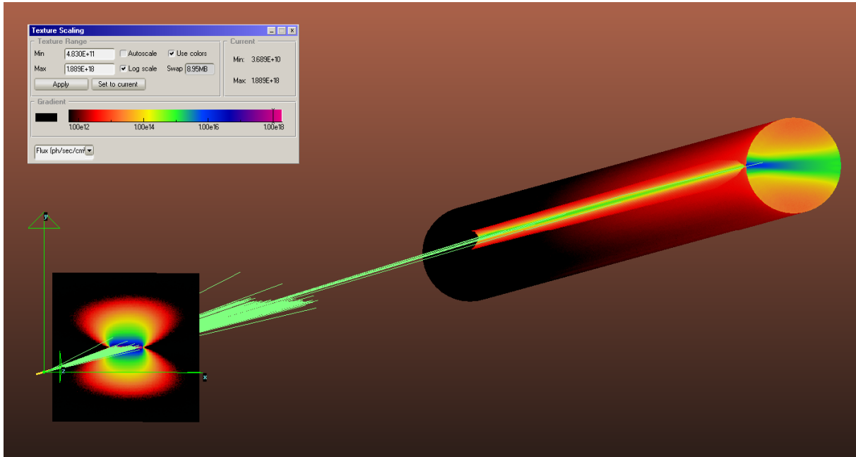
FIGURE 4.49: Recreation in Synrad+ of the DCI PSD experimental setup [134].
