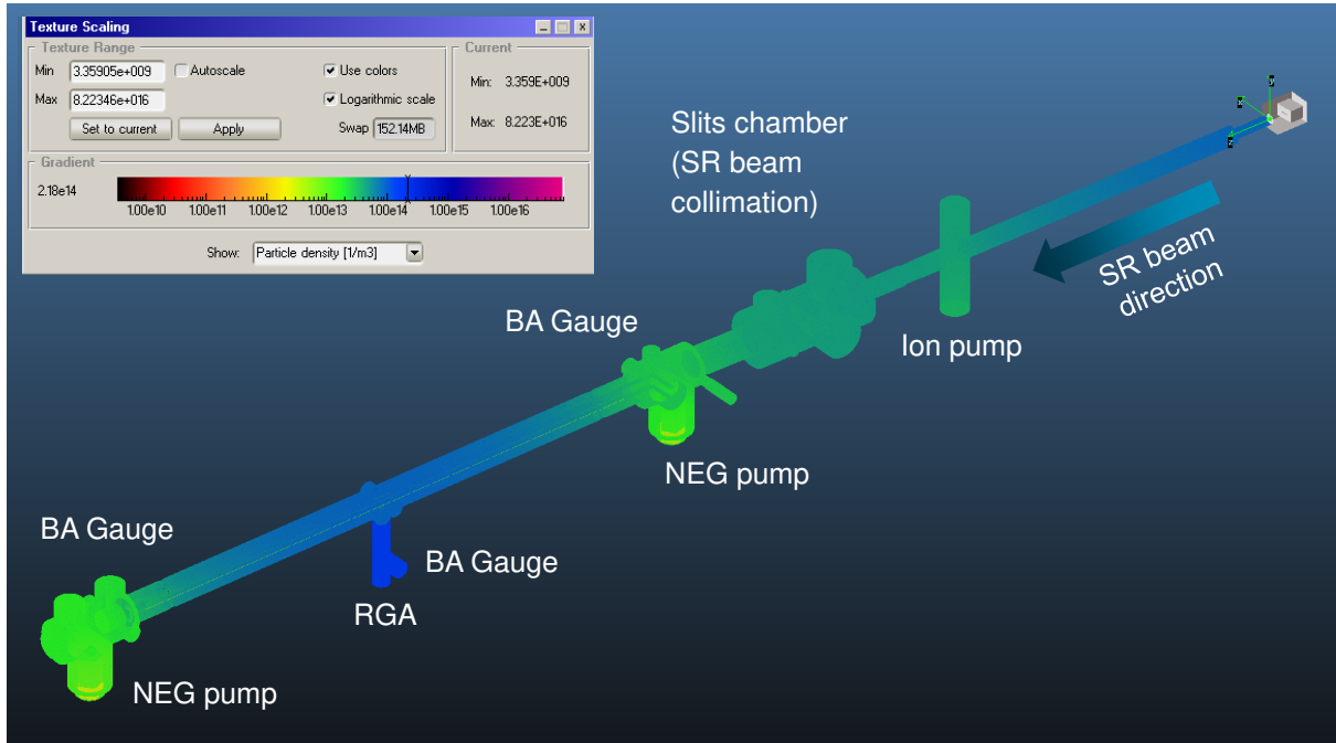
FIGURE 4.60: Simulation of \text{H}_2 molecular density map in BESTEX, after 24 h of beam dose. Arbitrary yield data.
