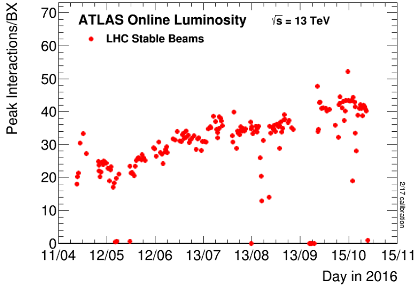
Figure B.10: Maximum number of inelastic collisions per bunch crossing \mu during stable beams in pp collisions at \sqrt{s} = 13 \text{ TeV} in 2016. The inelastic cross-section is taken to be 80 mb.
