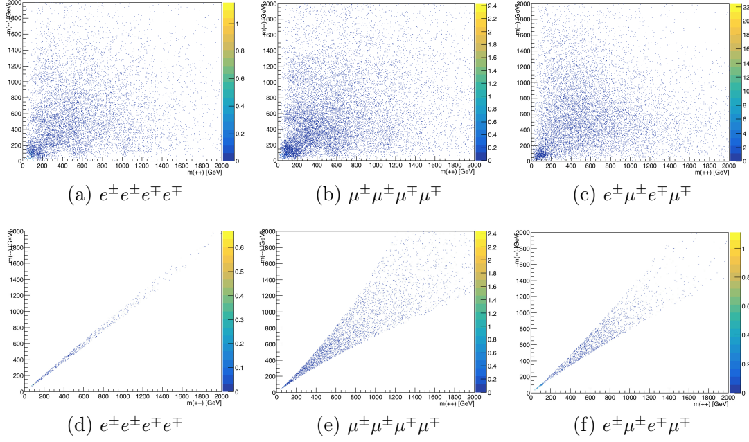
Figure 7.15: Scatter plot of m^{--} versus m^{++} diboson ZZ same-sign masses before the application of the \Delta M/\alpha \times \bar{M}^{\beta} cut (a), (b), (c) and after (d), (e), (f) in the e^{\pm}e^{\pm}e^{\mp}e^{\mp} , \mu^{\pm}\mu^{\pm}\mu^{\mp}\mu^{\mp} and e^{\pm}\mu^{\pm}e^{\mp}\mu^{\mp} channels.
