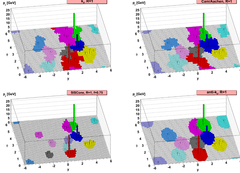
Figure 4.5: Three dimensional ( p_T, y, \phi plane) illustration of a parton-level event clustered with different jet algorithms (in order: k_t , Cam/Aachen, SIScone and anti- k_t ) showing the catchment areas of the resulting hard jets [118].
