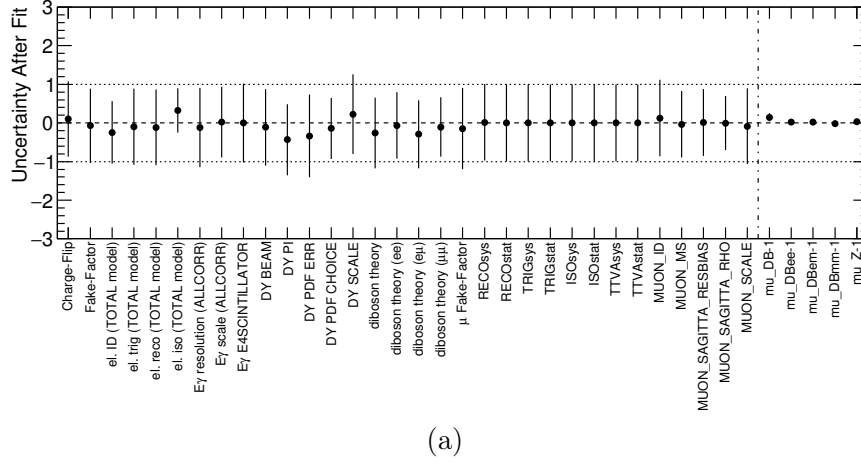
Figure 7.34: Systematic pulls for the combined fit. Values between -1 and 1 indicate the nominal 1 standard deviation band of the uncertainty.
