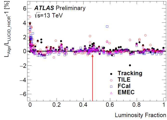
Figure B.12: Fractional difference in run-integrated luminosity between LUCID_HitOR algorithm, the TILE (red circle), EMEC (pink triangle), FCal (blue square) and track-counting (black dot) algorithms as a function of the cumulative delivered luminosity (normalized to 2016 total luminosity).
