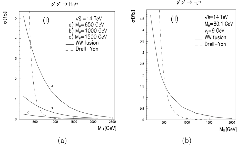
Figure 2.9: Cross-section for doubly-charged Higgs boson production as a function of the H^{\pm\pm} invariant mass for the right-handed (a) and left-handed (b) particles at \sqrt{s} = 14 TeV [58]. Curves are given for different values of M_{W_R} = \{650, 1000, 1500\} GeV and production mechanisms.
