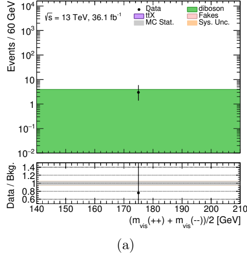
Figure 7.29: Data/MC in the 4LVR in one mass bin only from 150 to 200 GeV.
