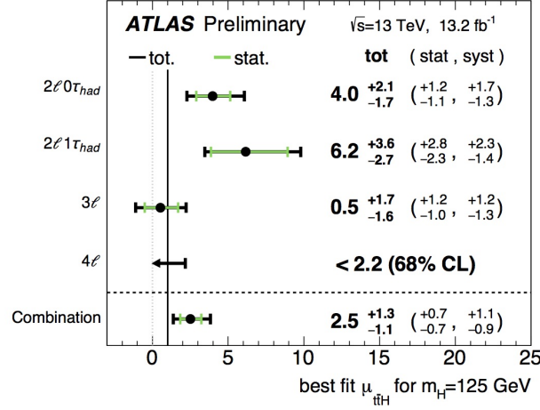
Figure 6.25: Best fit values of the t\bar{t}H signal strength separated into different final states and combined. The SM predicted signal strength is \mu=1 . In the 4\ell channel no events are observed in data and the 68% CL upper limit is shown.
