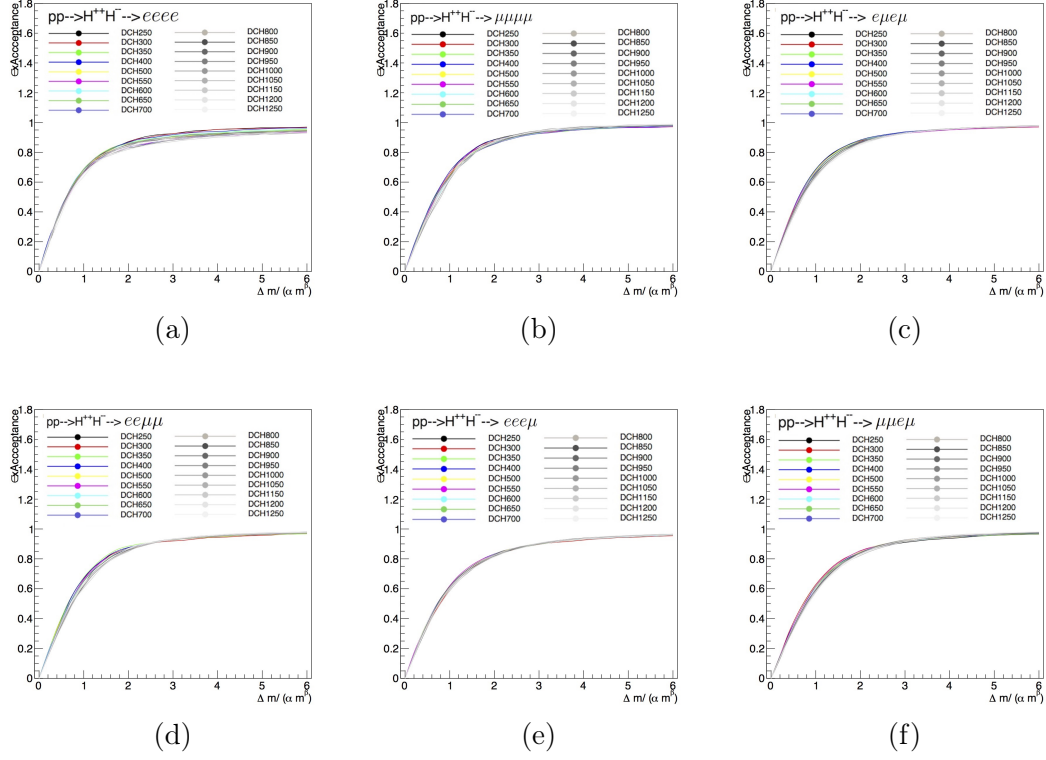
Figure 7.13: Signal efficiency times acceptance as a function of the \Delta M/\alpha \times \bar{M}^\beta cut for the eeee (a), \mu\mu\mu\mu (b), e\mu e\mu (c), ee\mu\mu (d), eee\mu (e) and \mu\mu e\mu (f) channels respectively. Plots are normalized to baseline (signal region definition, trigger requirement and Z veto) selection.
