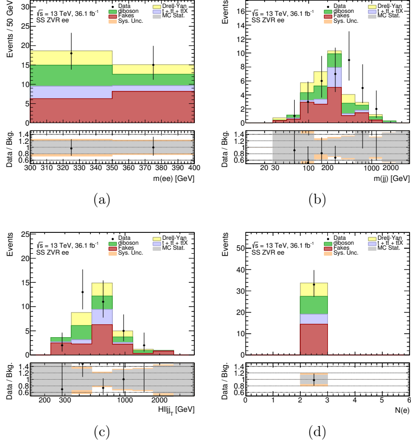
Figure 7.50: Pre-fit distributions for data and SM background predictions in the electron channel validation region: (a) invariant mass of the two leptons, (b) invariant mass of the two leading jets, (c) scalar sum of the p_T of leptons and two leading jets, and (d) total number of events in the region.
