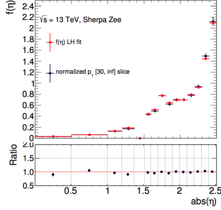
Figure 7.18: Comparison between the true MC 2D charge-flip parametrization (black dots) and the result of the likelihood fit applied to simulation using the 1D×1D parametrization (red dots).
