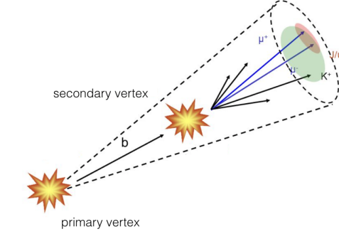
Figure 5.6: Representation of an event containing a non-prompt lepton: a b -hadron is produced in the IP with consequent decay into light quarks jets in secondary displaced vertex. Electrons, or muons, originate from the b -hadron secondary decay and can fake leptons coming directly from the PV.
