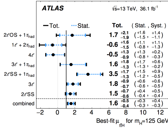
Figure 6.27: Observed best-fit values of the t\bar{t}H signal strength and uncertainties divided into final state category and combined. The individual values for channels \mu are obtained fitting all the signal regions with each channel signal strength floating independently.
