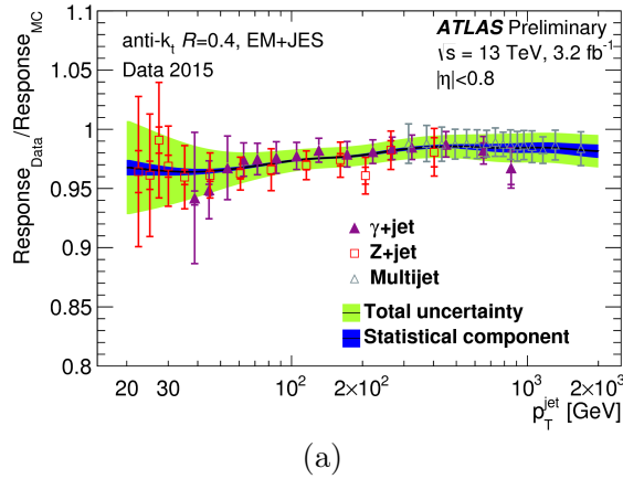
Figure 4.9: (a) jet response ratio as a function of jet p_T [121].
