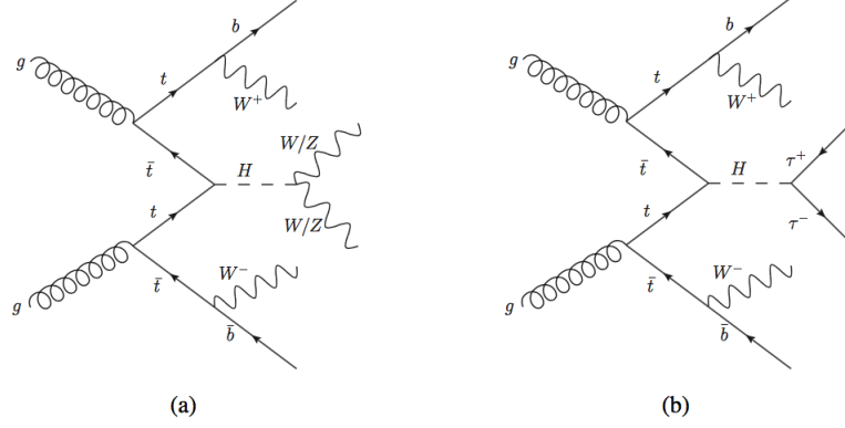
Figure 2.4: Tree-level production mode for the t\bar{t}H process with consequent decays into WW^*, ZZ^* (left) or \tau\bar{\tau} (right).
