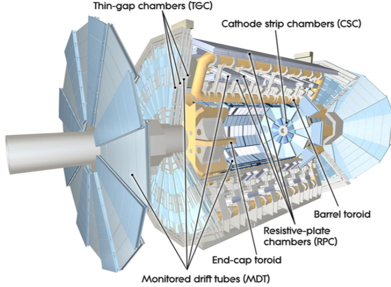
Figure 3.11: View of the ATLAS muon spectrometer [95].
