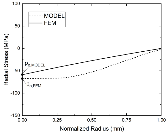
Figure 4.22: Radial stress distribution as a function of the SMA ring normalized radius (configuration #1 in Table 4.8) obtained at T_o = 25\text{ }^{\circ}\text{C} from FEM simulation and analytical model calculation.
