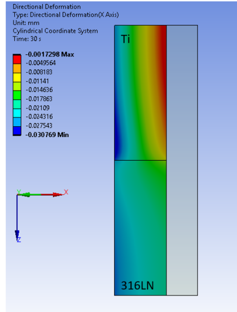
Figure 5.22: Radial displacement (in mm) of the steel and titanium rings at T = 200^{\circ}C .
