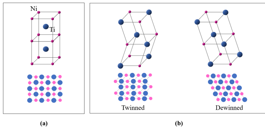
Figure 2.1: Schematic three and two-dimensional representations of the NiTi alloy crystallographic phases: (a) Austenite, (b) Martensite.
