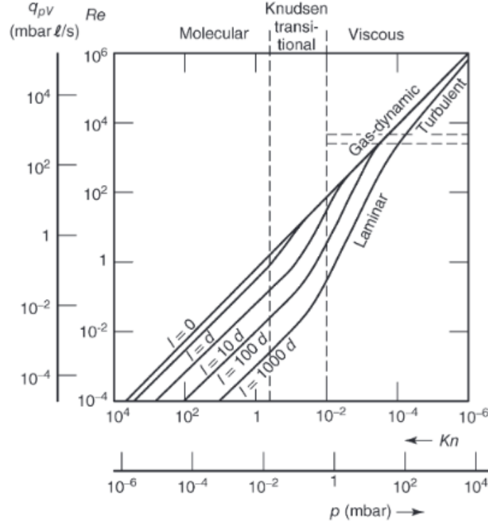
Figure 1.2: Flow types in tubes with circular cross section, diameter d = 1\text{ cm} , and length l as indicated taken as an example. The gas is air at 20^\circ\text{C} . Inlet pressure is taken as abscissa and the outlet pressure is assumed negligible, from [16].
