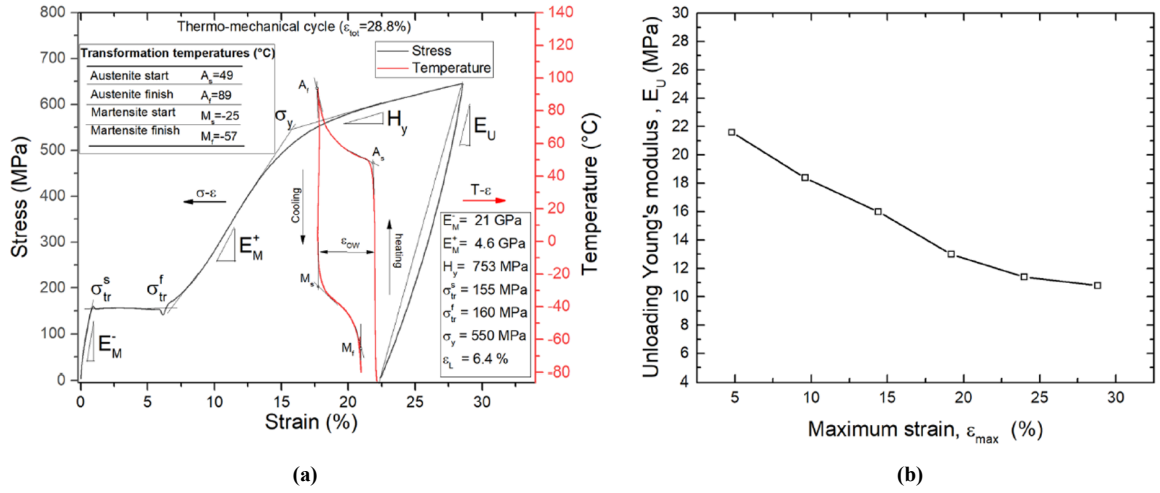
Figure 4.5: Thermo-mechanical properties of the investigated NiTi alloy: (a) isothermal stress-strain curve ( T = -80^\circ\text{C} ) and subsequent strain-temperature curve obtained from a complete thermal cycle between TTs and (b) unloading modulus E_U , as a function of the pre-strain level, \epsilon_{max} .
