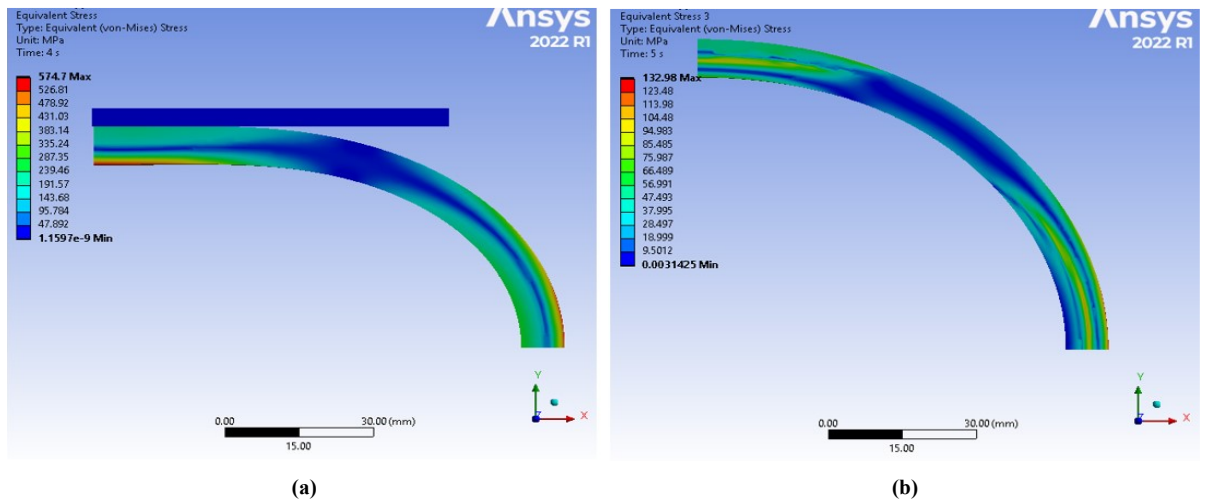
Figure 5.25: Equivalent Stress distribution in the NiTi coupler during ovalization: (a) Maximum loading displacement, w_{max} = 16mm , and (b) Complete unloading.
