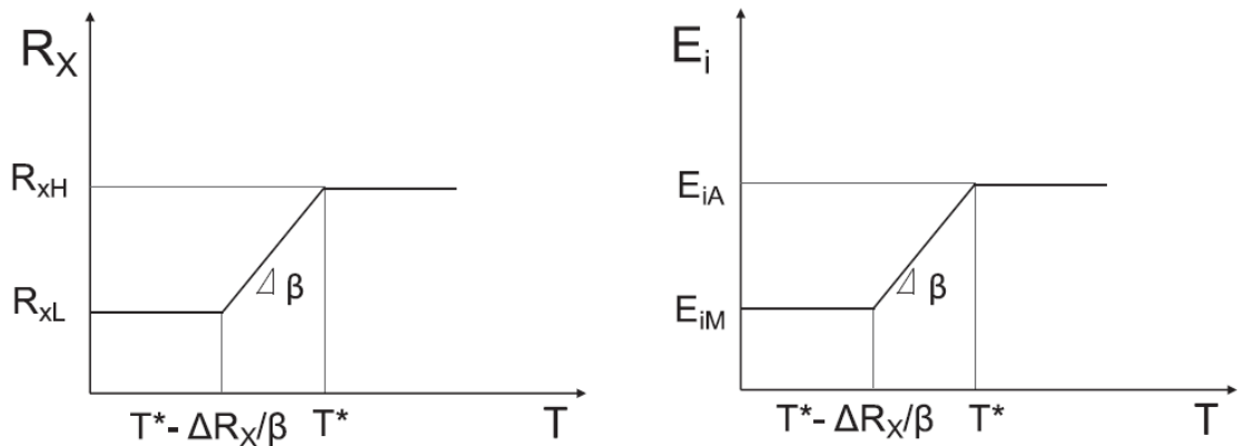
Figure 5.2: Temperature dependence for the elastic domain radius R_X and the initial Young's modulus of martensite E_i , from [9].
