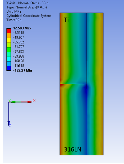
Figure 5.21: Radial stress distribution in the bi-material connection system at T_{room} = 25^{\circ}C .
