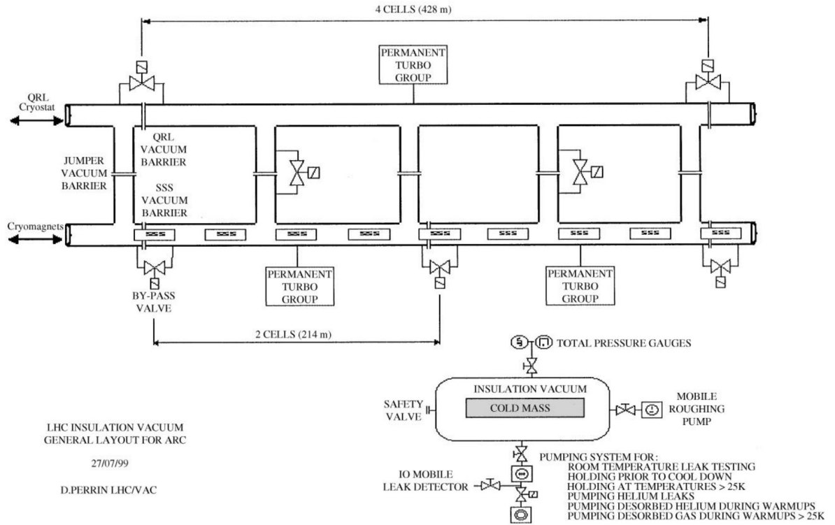
Figure 1.8: Layout of cryogenic insulation vacuum, from [24].
