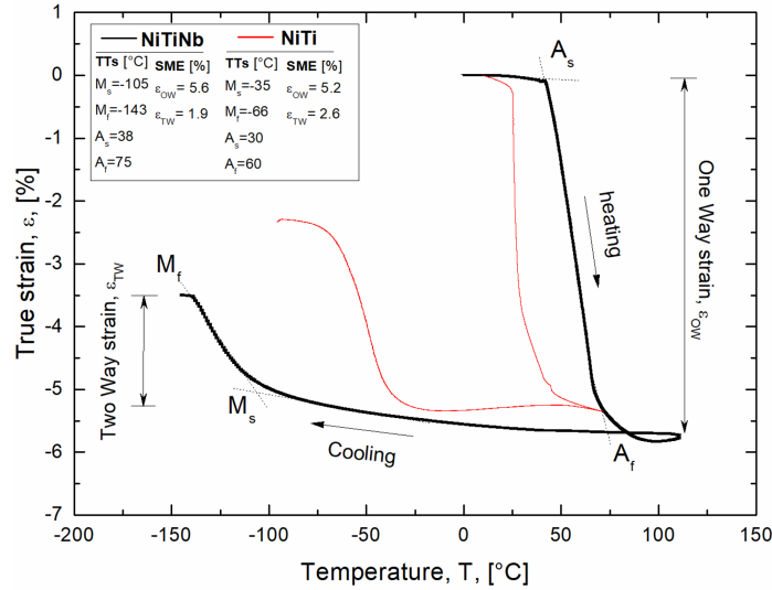
Figure 3.4: Thermo-mechanical properties of the investigated NiTi and NiTiNb alloys: true strain vs temperature ( \epsilon - T ) curve obtained from stress-free ( \sigma = 0 ) thermal cycle between the TTs.
