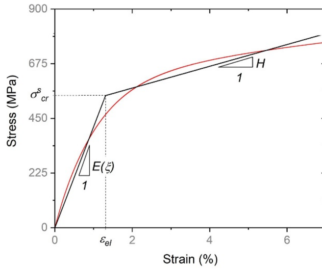
Figure 4.20: Bilinear stress-strain curve used for simulations and identification of model parameters
