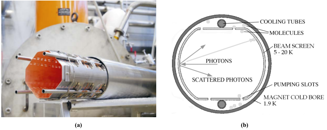
Figure 1.10: Beam screen: (a) Picture of the beam screen prototype for the Q2 quadrupole magnets for High-Luminosity (HL) -LHC, from [22], (b) Schematic representation of actively cooled beam screen in the magnet cold bore, from [24].
