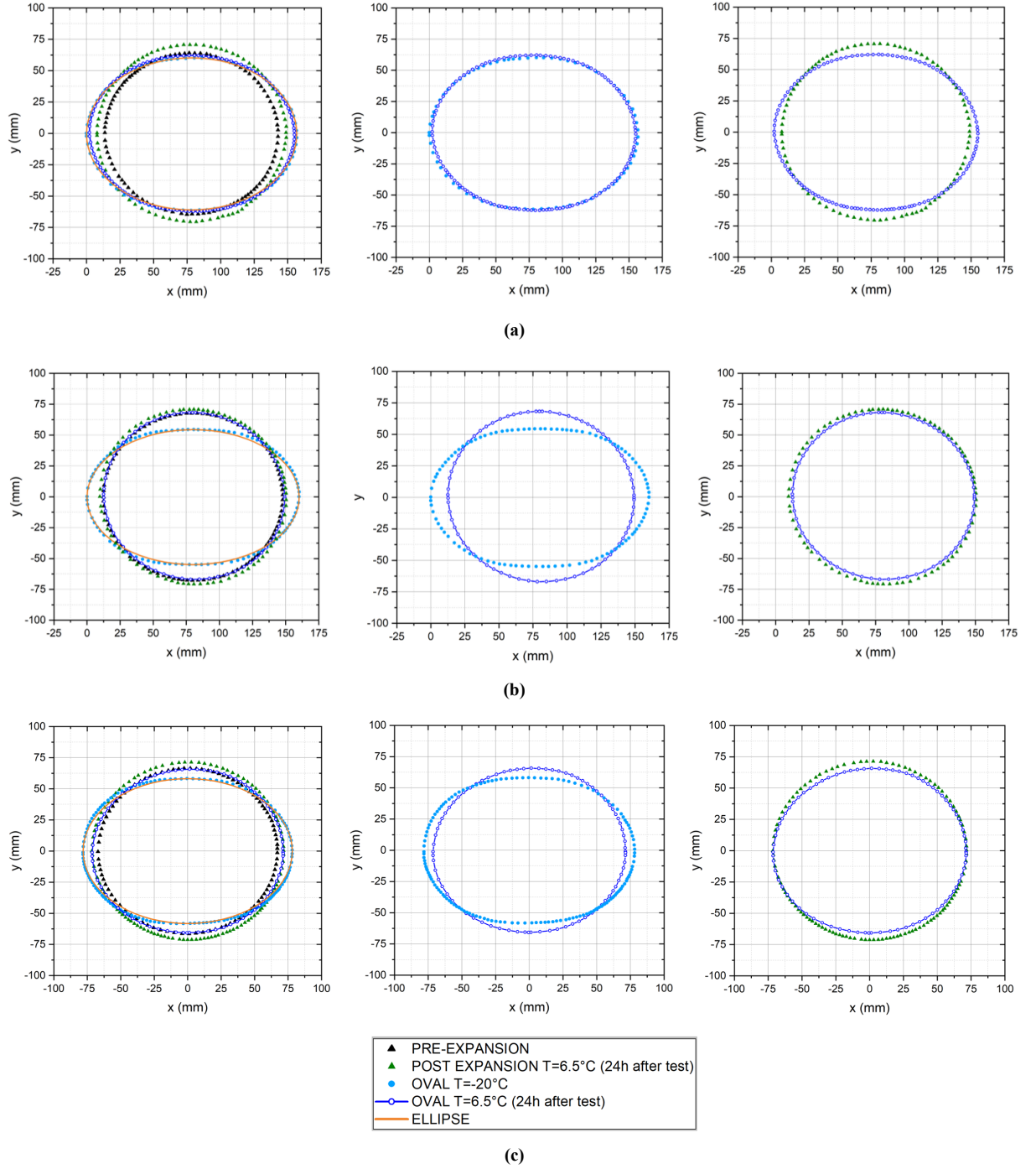
Figure 3.17: Comparison between the internal profile of connectors during the ovalization process for: (a) Connector 1, (b) Connector 2, and (b) Connector 3. The internal profile of each connector is reported into three different graphs: the first graphs shows the profile of the connector in the pre- and post-expansion phase, and after the oval test at T=-20^{\circ}\text{C} with the associated ellipse and 24 h after the oval test at T=6.5^{\circ}\text{C} . The second graph shows a comparison between the two ovals at T=20^{\circ}\text{C} and 24 h after the test at T=6.5^{\circ}\text{C} . The third graph shows a comparison between initial (post-expansion of the ring) and final (oval at T=6.5^{\circ}\text{C} ) shapes of the oval test.
