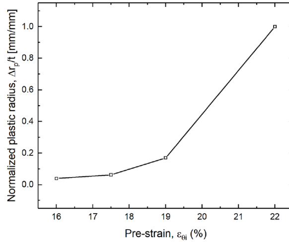
Figure 4.8: Normalized plastic radius, \Delta r_p/t as a function of the prestrain, \epsilon_{\theta i} for ring #9.
