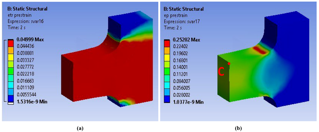
Figure 5.29: Plot of the norm of the transformation and plastic strain tensors in the C-shaped connector at the end of the pre-strain: (a) Norm of the transformation strain tensor, and (b) Norm of the plastic strain tensor.
