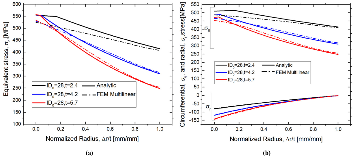
Figure 4.11: Analytical versus FE multilinear predictions of stress distributions along the rings radius for ring type #1, #2, #3 at a fixed pre-strain level: \epsilon_{\theta i} = 16\% : (a) equivalent stress, \sigma_e , and (b) radial, \sigma_r , and circumferential stress, \sigma_\theta .
