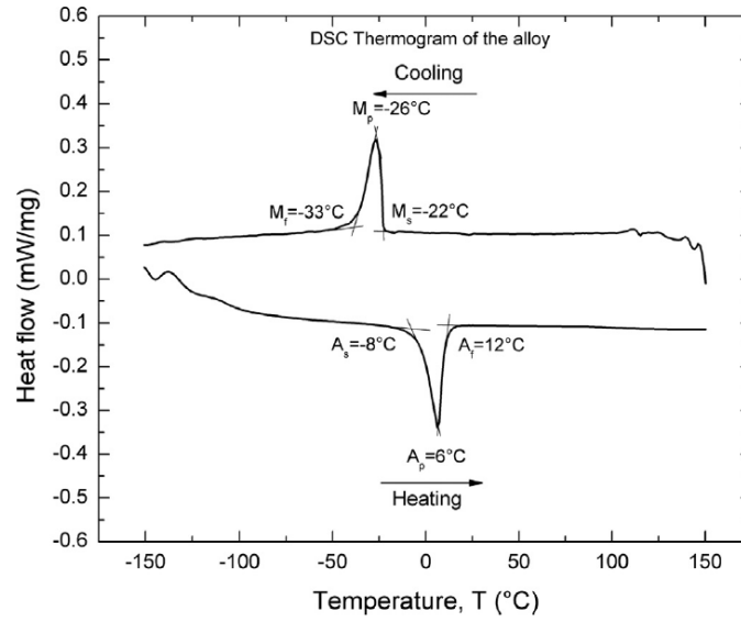
Figure 3.1: Differential Scanning Calorimetry thermogram of the investigated NiTi alloy, from [9].
