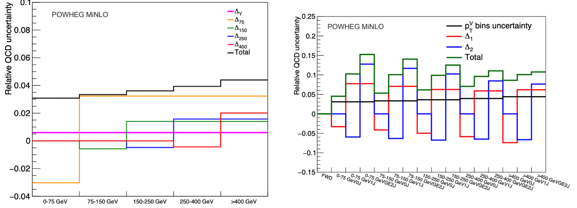
Figure 5.7: Relative QCD scale uncertainties in STXS bins for ZH process (POWHEG).
