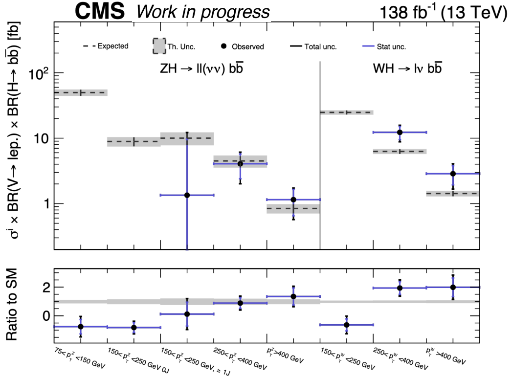
Figure 7.5: Measured values of \sigma\mathcal{B} in STXS bins, combining all years. In the bottom panel, the ratio of the observed results with associated uncertainties to the SM expectations is shown. For the bins where the negative signal strength is measured the observed cross-section values are not reported.
