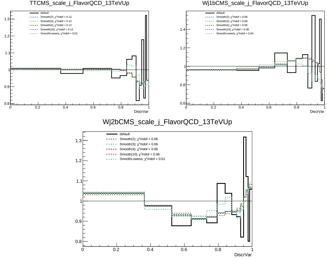
Figure 6.1: Smoothing of up(down) variations for JES systematic uncertainty templates.
