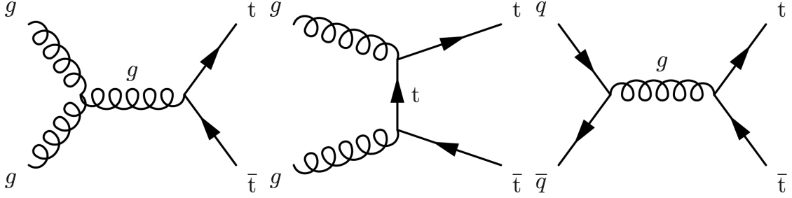
Figure 4.4: t\bar{t} production processes diagrams
