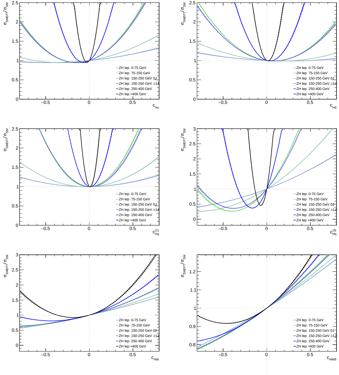
Figure 8.2: Cross-section scaling functions for the modified ZH STXS stage 1.2 bins for each of the O_{Hq}^{(3)} , O_{Hq}^{(1)} , O_{Hu} , O_{Hd} , O_{HW} , O_{HWB} operators. The equations are listed in Table 8.2
