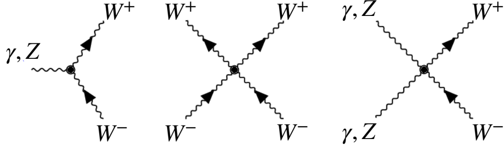
Figure 2.3: EWK self-interaction vertices.
