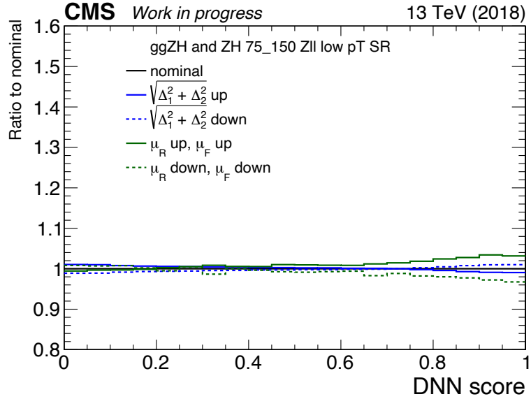
Figure 5.14: Acceptance uncertainties for ZH\ 75 < p_T^V < 150
