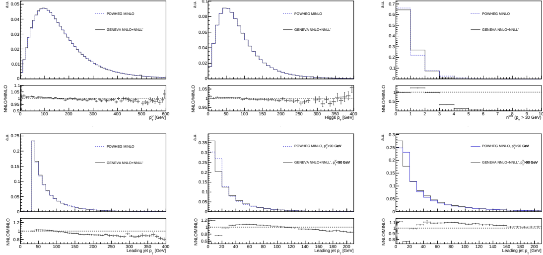
Figure 5.9: Comparison of kinematic distributions of events produced with GENEVA and POWHEG generators. Top row: vector boson p_T distribution on the left, the Higgs boson p_T distribution in the middle and n_{\text{jet}} distribution on the right; bottom row: p_T distribution of the leading jet on the left; p_T distribution of the leading jet for events with p_T^V < 90 GeV in the middle, p_T distribution of the leading jet for events with p_T^V > 90 GeV on the right.
