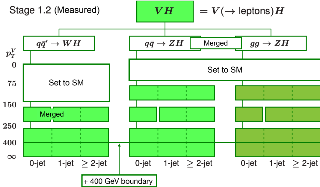
Figure 5.3: VH STXS stage 1.2 scheme adapted to the VH(H \rightarrow b\bar{b}) analysis sensitivity limitations
