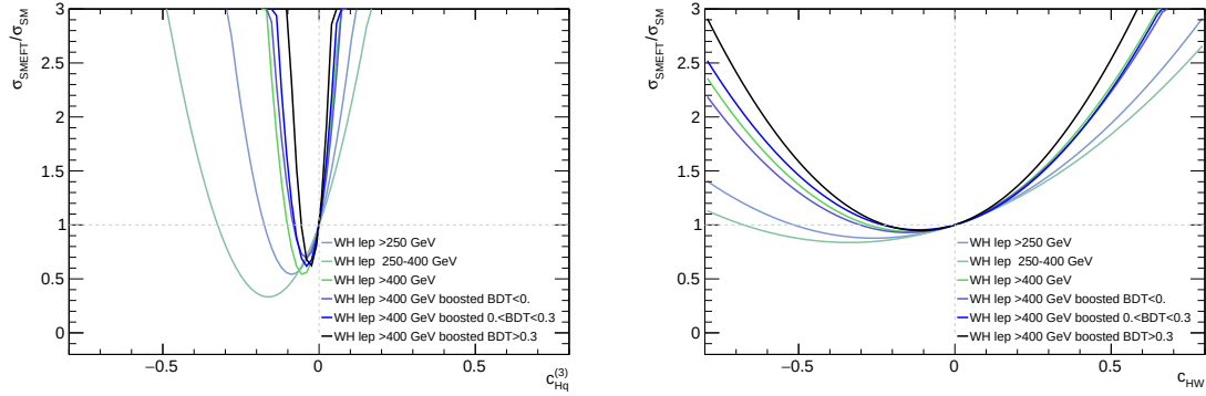
Figure 8.15: Scaling functions for the WH production in p_T^V > 250 GeV, 250 < p_T^V < 400 GeV and p_T^V > 400 GeV bins; in addition the scaling functions are also produced in 3 BDT regions: [-1,0) , [0,0.3) , [0.3,1]
