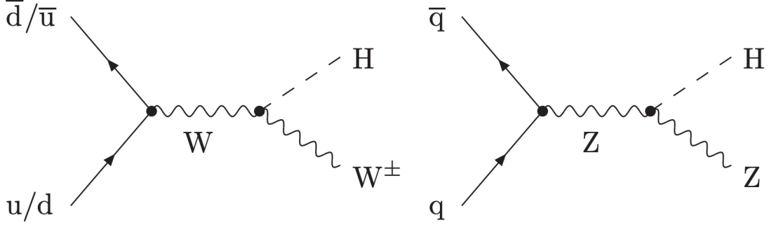
Figure 4.1: qq' \rightarrow WH and qq \rightarrow ZH production processes diagrams
