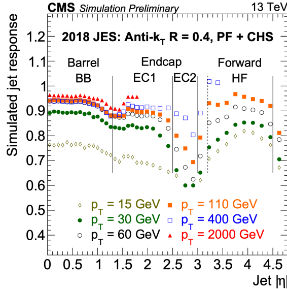
Figure 3.9: The CMS jet energy scale corrections measured in 2018 data-taking period [46].
