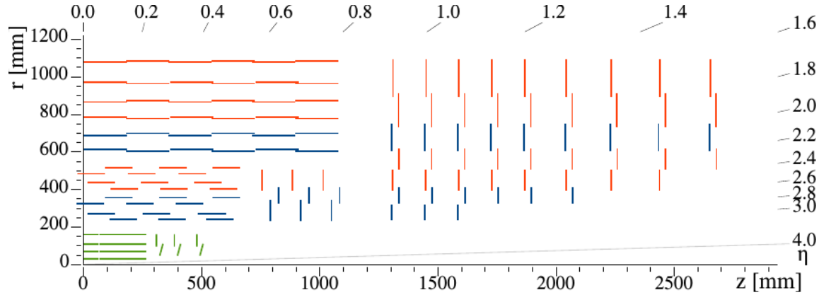
Figure 3.4: The CMS tracking system scheme.
