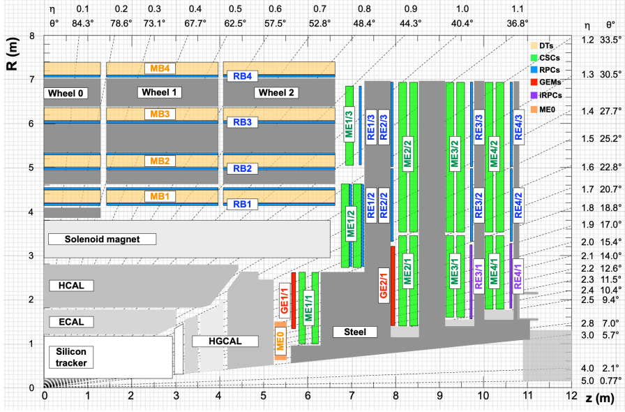
Figure 3.7: The CMS muon system.
