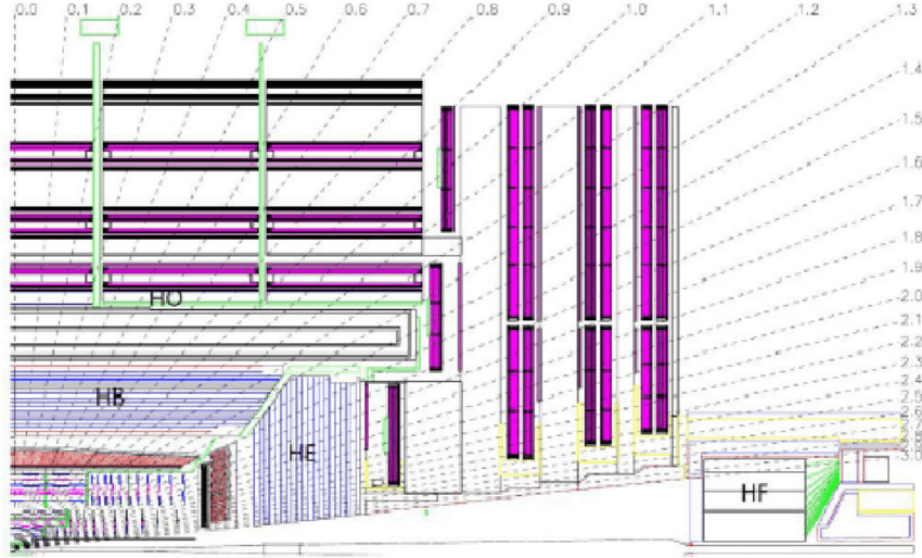
Figure 3.6: The CMS HCAL subdetector.
