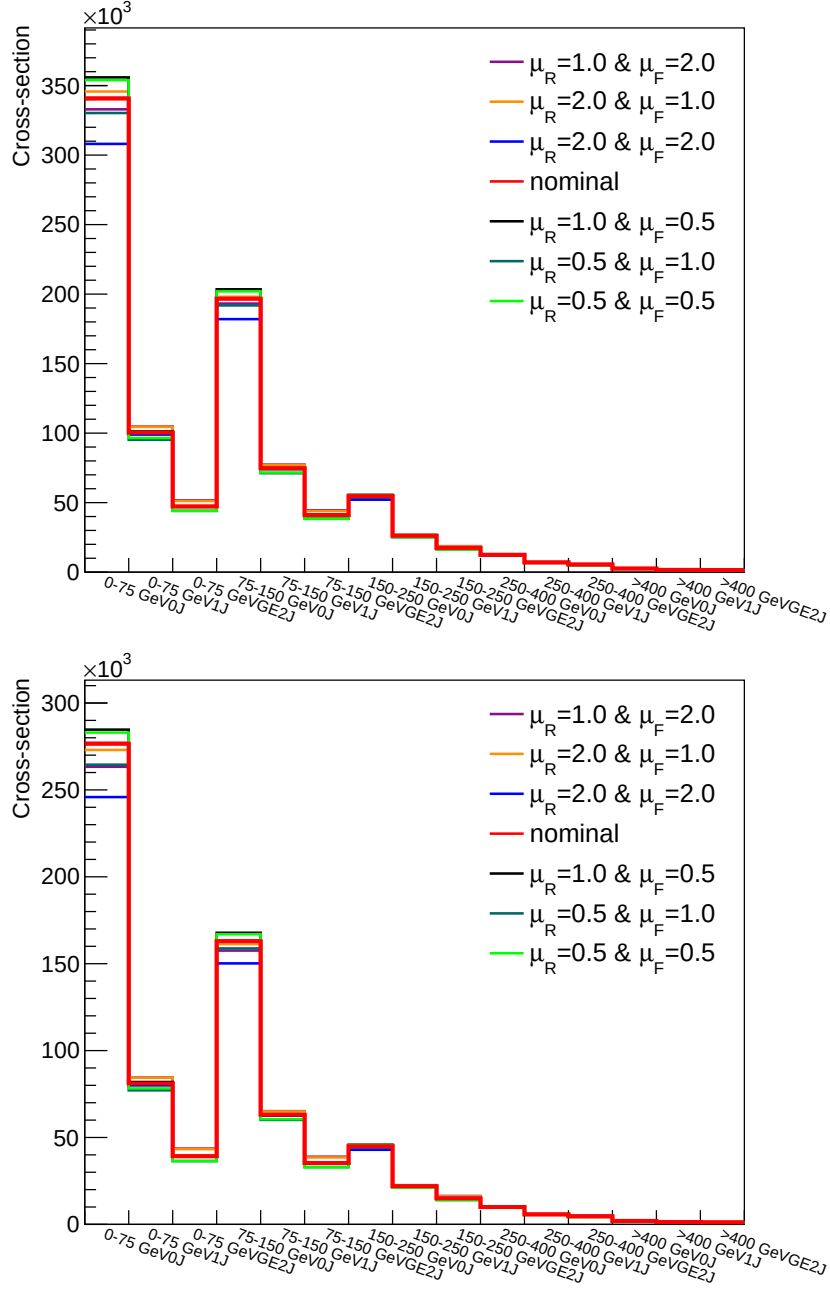
Figure 5.6: Scale variations for WH, qqZH processes.
