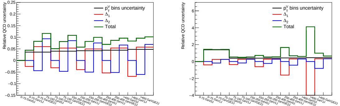
Figure 5.8: Relative QCD scale uncertainties in STXS bins for WH (left) and ggZH (right) processes (POWHEG).
