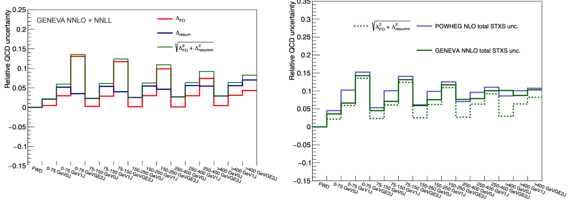
Figure 5.11: Relative FO and resummation uncertainties (left) from GENEVA samples and total uncertainties in comparison with the POWHEG QCD scale uncertainties (right) in STXS bins for VH process.
