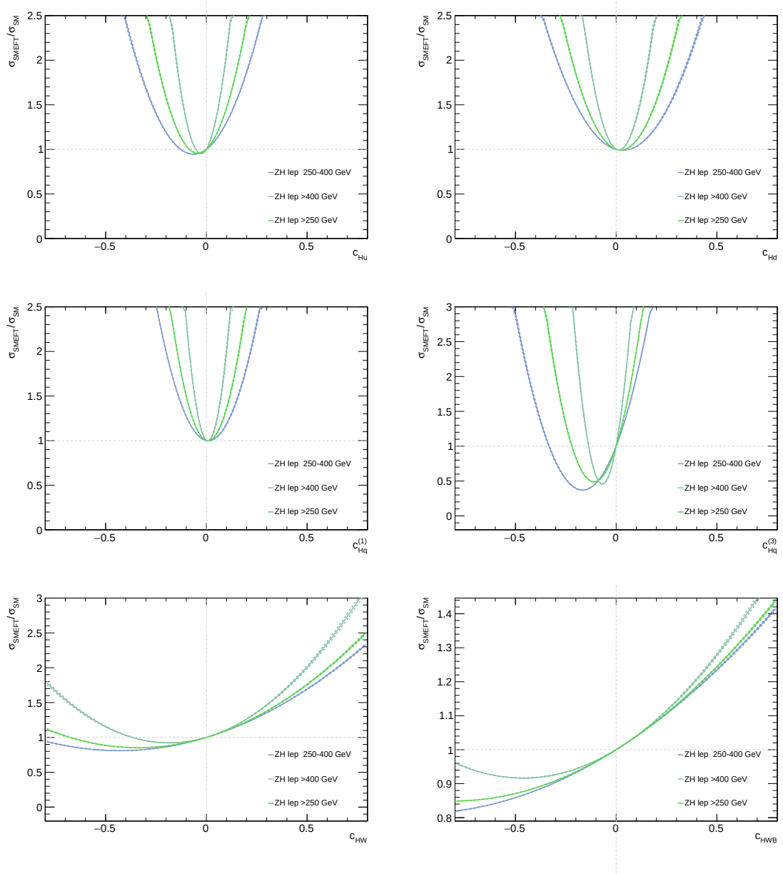
Figure 8.14: Cross-section scaling functions for the ZH STXS stage 1.2 bins
