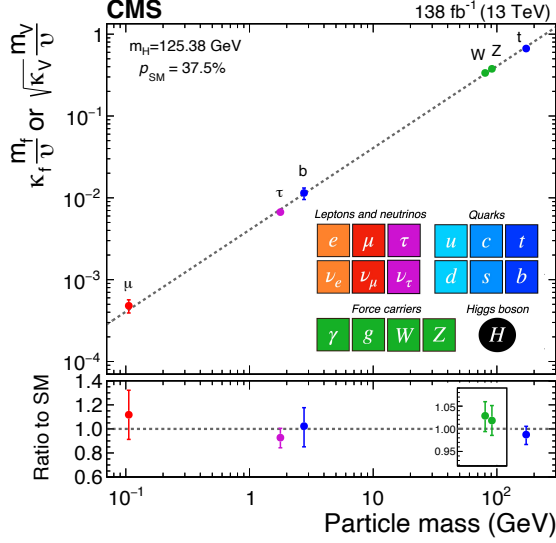
Figure 2.9: SM Higgs boson couplings to fermions and vector bosons measured in CMS [24].
