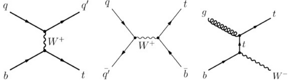
Figure 4.5: Single-top-quark production processes diagrams. From left to right: t-channel, s-channel and tW process.
