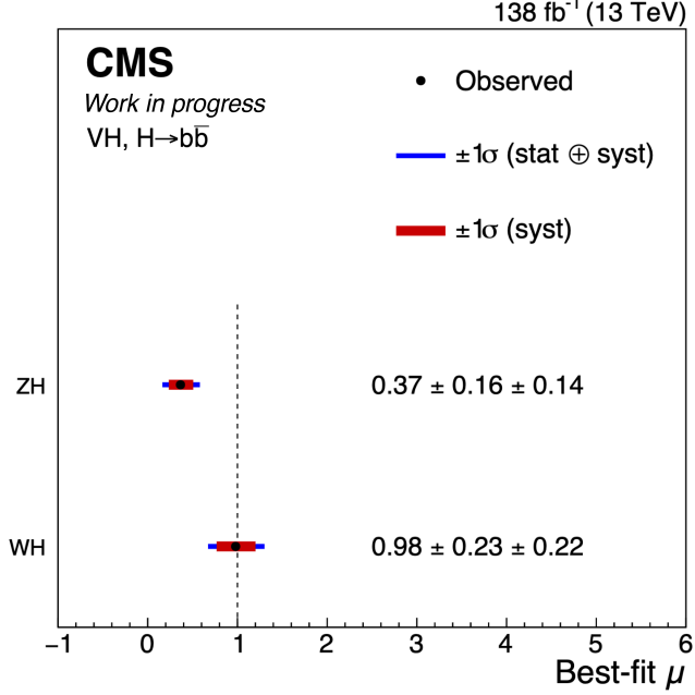
Figure 7.4: Signal strengths for the ZH and WH production modes.
