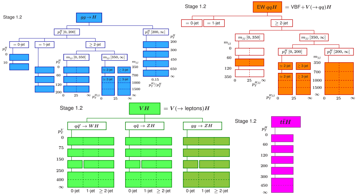
Figure 5.1: STXS categorisation for the leading Higgs production processes.
