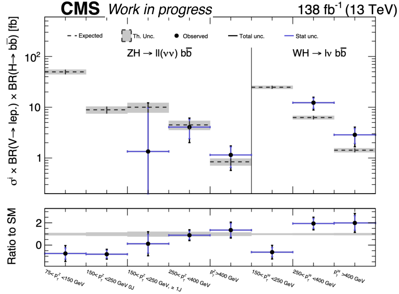
Figure 9.1: Measured values of \sigma\mathcal{B} in STXS bins from the full Run 2 VH(H \rightarrow b\bar{b}) analysis.
