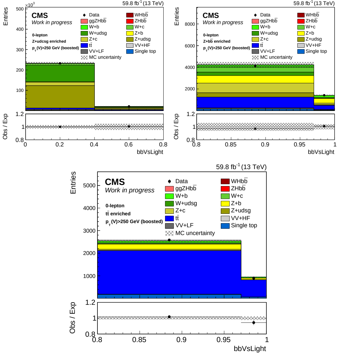
Figure 4.14: Control region post-fit distributions in the boosted analysis in 0-lepton channel. The left, middle and right columns corresponds to the V+LF, V+HF and t\bar{t} control regions respectively.
