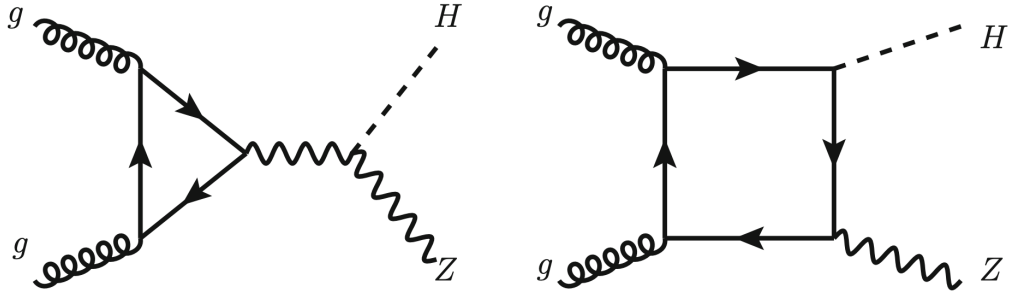
Figure 4.2: ggZH production processes diagram
