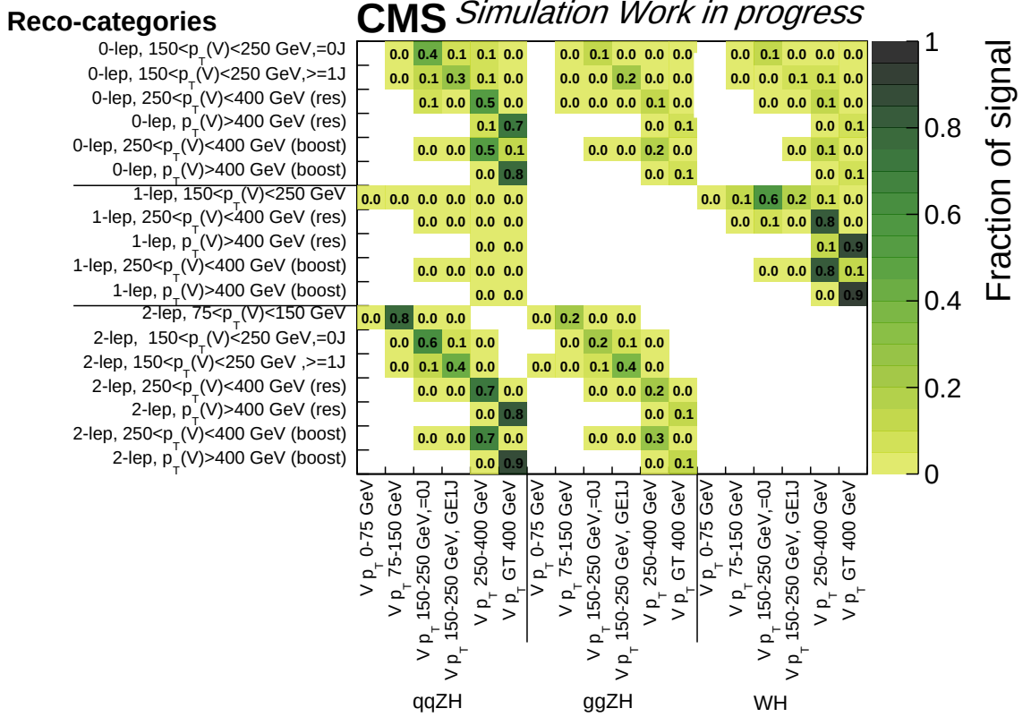
Figure 5.4: STXS signal processes fraction inside reconstruction level analysis signal categories.
