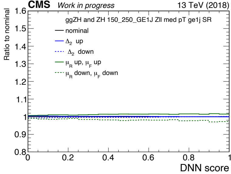
Figure 5.12: Acceptance uncertainties for ZH\ 150 < p_T^V < 250\text{ GeV} \geq 1\text{ jet} process.
