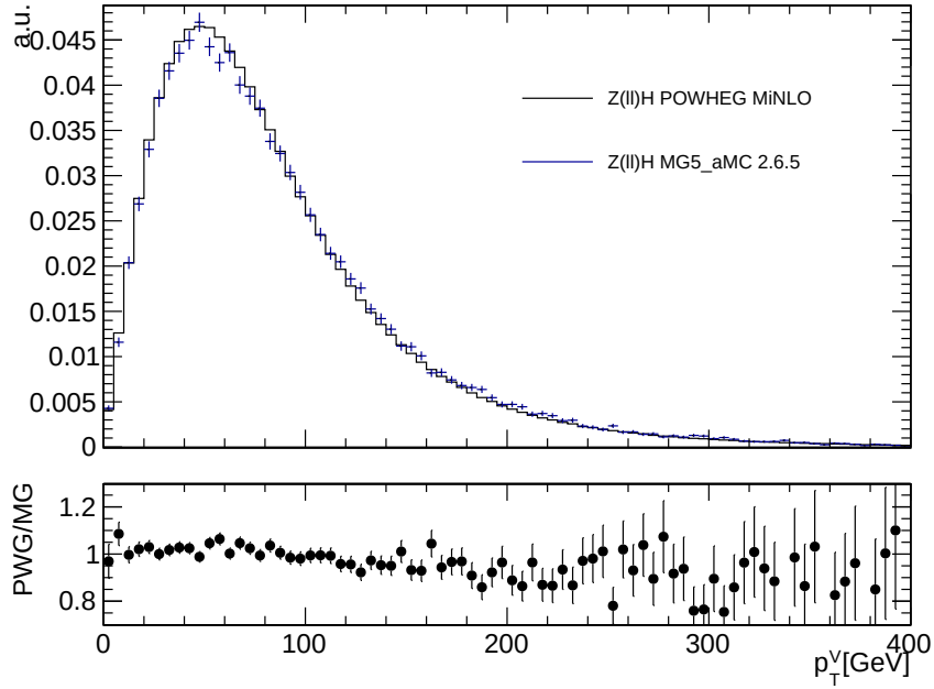
Figure 8.1: p_T^V distribution for ZH(l) Madgraph and POWHEG MiNLO events. The uncertainties shown for each point are statistical.
