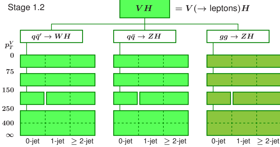
Figure 5.2: STXS bins stage 1.2 VH leptonic
