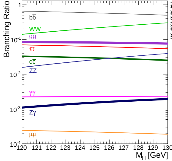
Figure 2.8: SM Higgs boson decay branching fraction predictions [15]
