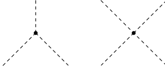
Figure 2.5: Higgs boson self-interaction diagrams
