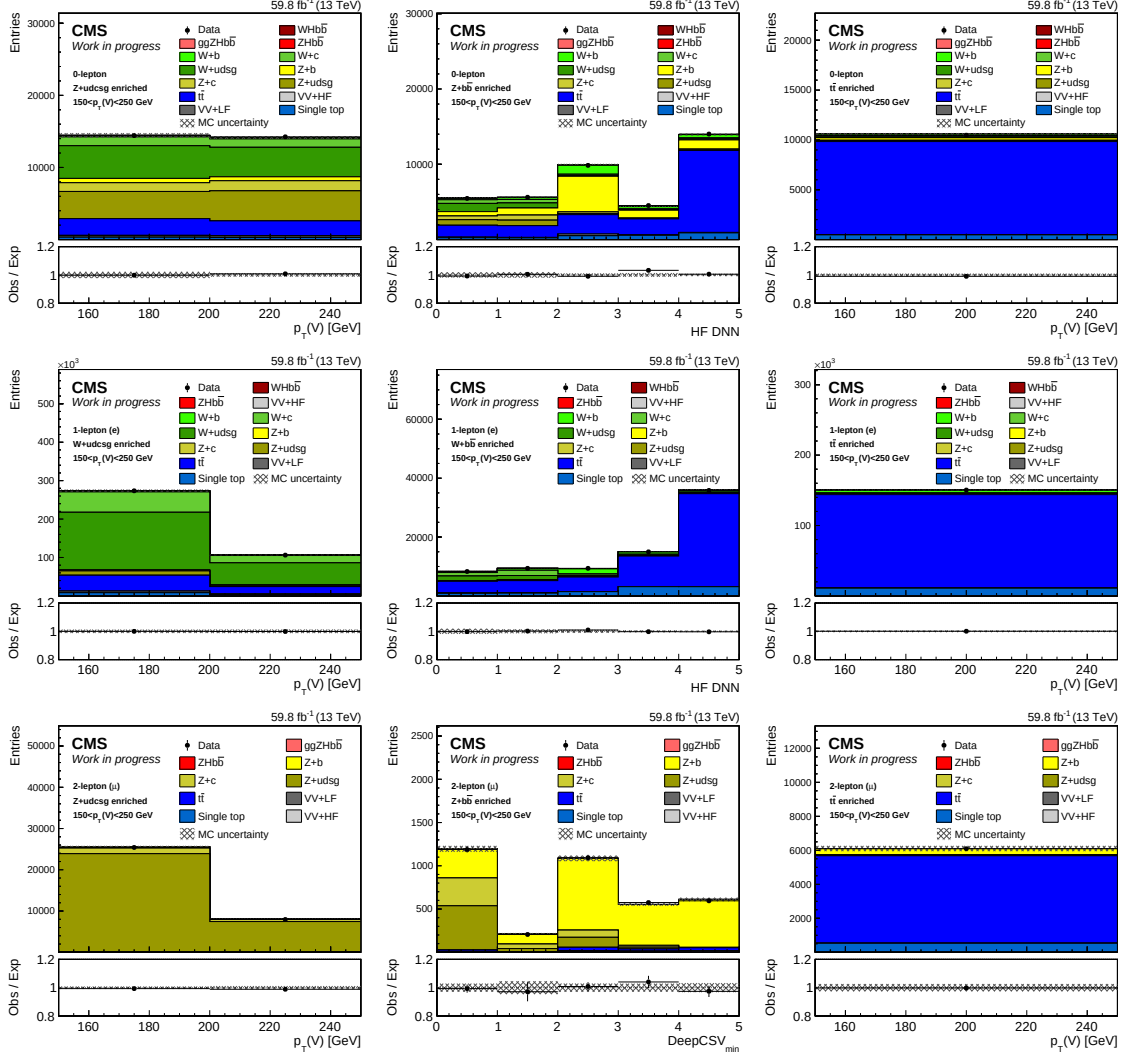
Figure 4.13: Control region post-fit distributions in the resolved analysis. Top, middle and bottom rows corresponds to the 0-lepton, 1-lepton and 2-lepton channels respectively. The left, middle and right columns corresponds to the V+LF, V+HF and t\bar{t} control regions respectively.
