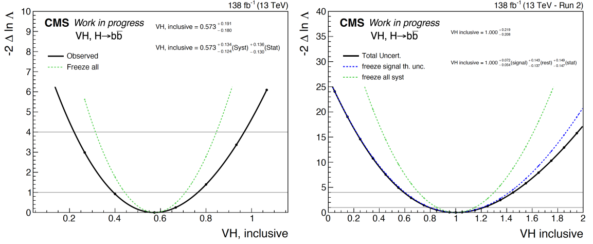
Figure 7.1: Test statistics distributions for inclusive single strength \mu extracted from the full Run 2 fit. The curve where all of the uncertainties are included are shown in black, without theoretical signal uncertainty in violet, and the curve where only statistical uncertainties are included in green.
