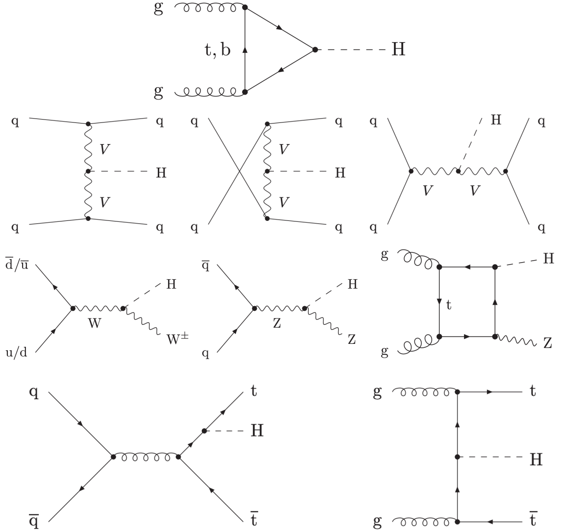
Figure 2.6: Feynman diagrams for the leading Higgs production modes at the LHC [14]. The ggH , VBF, VH and t\bar{t}H Higgs production processes are shown in the first, second, third and bottom rows respectively.
