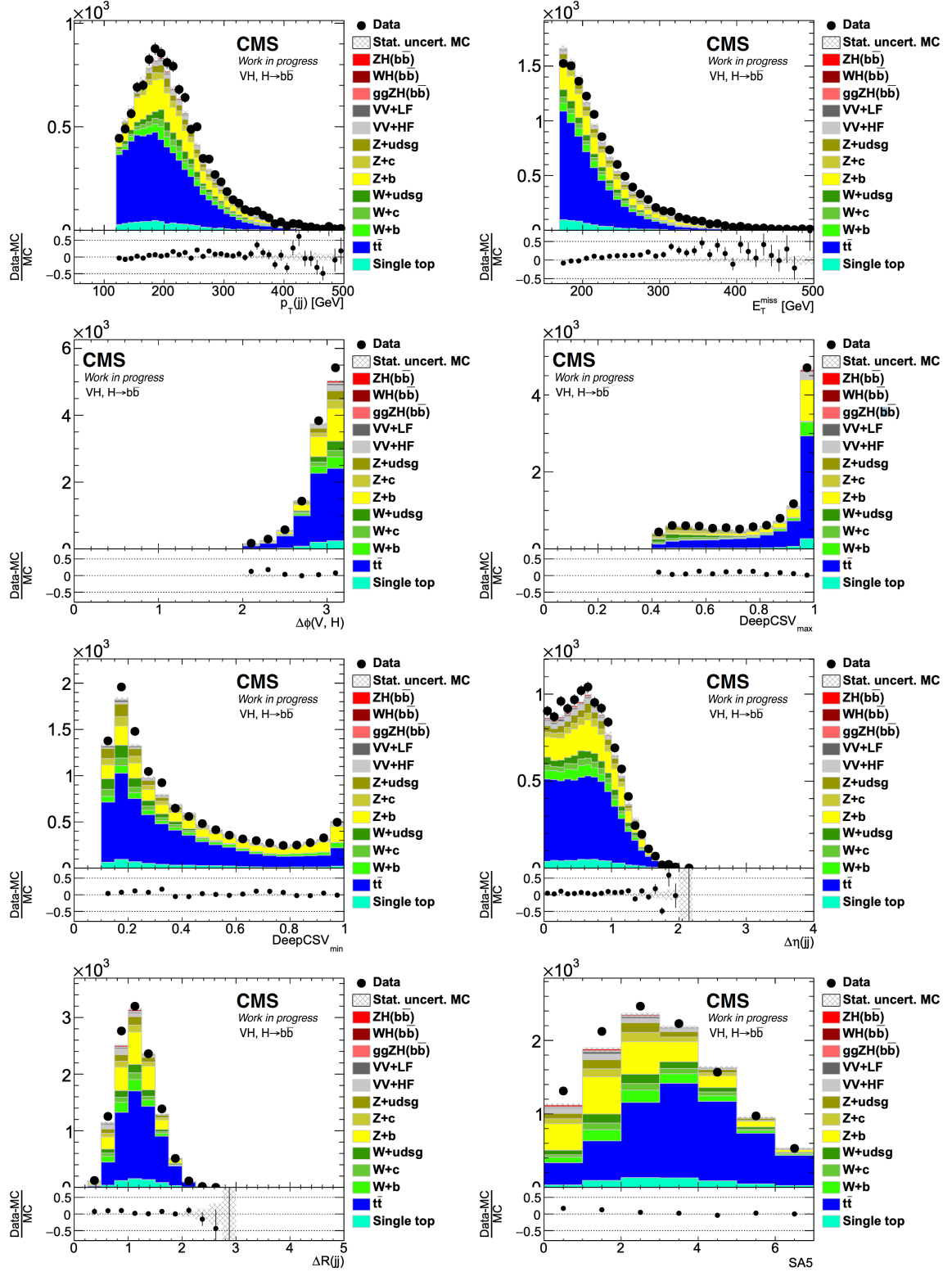
Figure 4.12: 0-lepton signal region pre-fit distribution of MVA input variables
