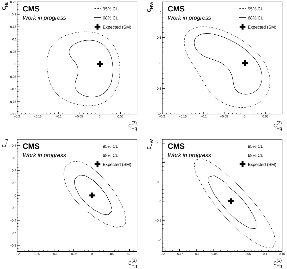
Figure 8.8: The expected 68% and 95% CL contours obtained with the full parametrisation (top row) and linear only (bottom row) for the O_{Hq}^{(3)} vs O_{Hu} (left) and O_{Hq}^{(3)} vs O_{HW} (right) operators.
