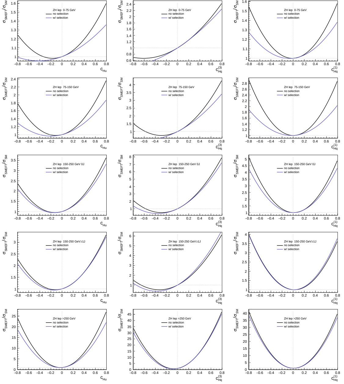
Figure 8.10: Parametrisation derived in STXS stage 1.2 bins with and without acceptance effects taken into account for the c_{Hq}^{(3)} , c_{Hq}^{(1)} , c_{Hu} operators.
