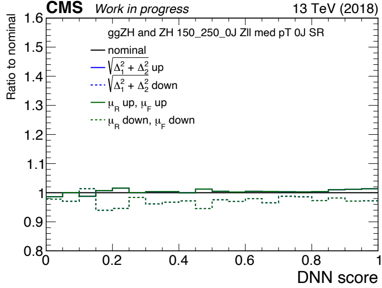
Figure 5.13: Acceptance uncertainties for ZH\ 150 < p_T^V < 250\text{ GeV}\ 0\text{ jets} process.
