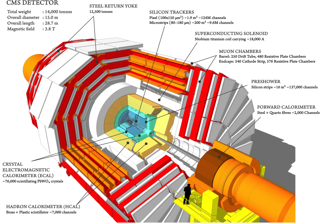
Figure 3.3: The CMS detector general view
