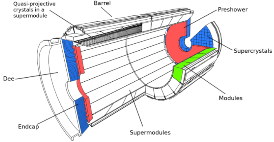
Figure 3.5: The CMS ECAL subdetector.
