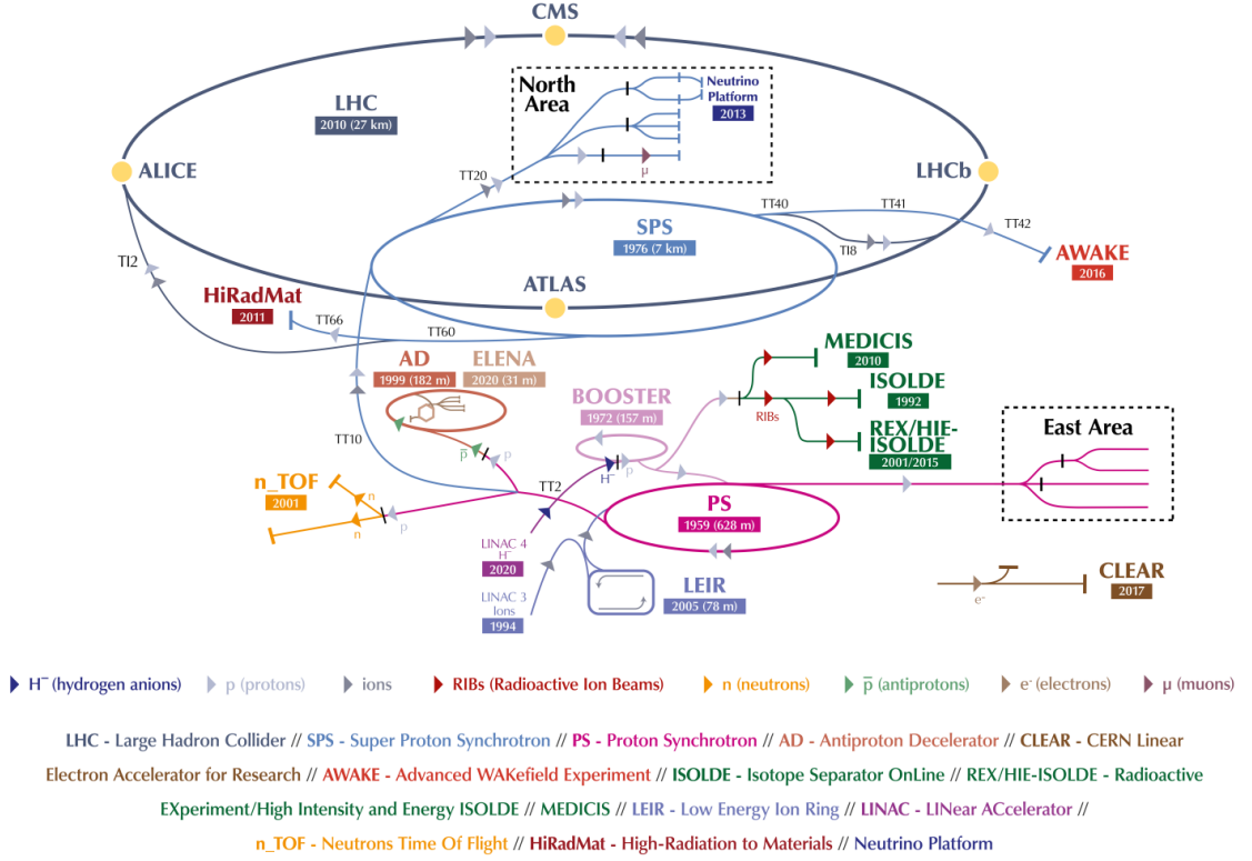
Figure 3.1: The LHC acceleration complex scheme.
