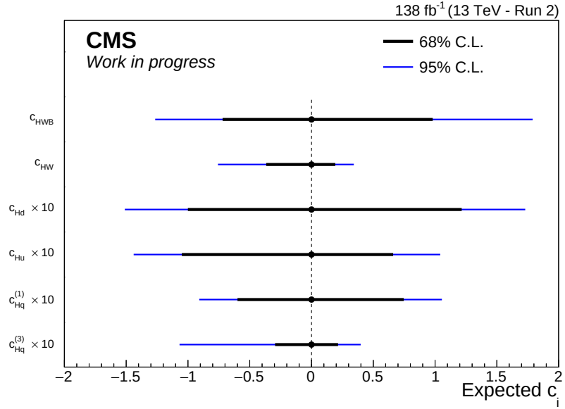
Figure 9.2: Expected 68% and 95% CL intervals obtained with linear-plus-quadratic parametrisation.
