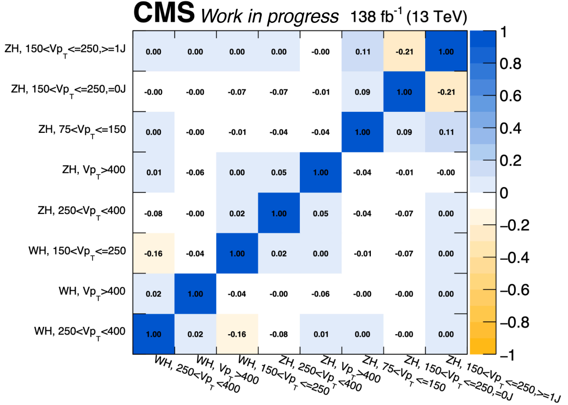
Figure 7.6: Observed correlations between the STXS parameters of interest.
