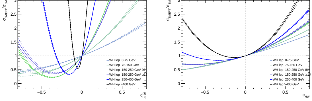
Figure 8.3: Cross-section scaling functions for the modified WH STXS stage 1.2 bins for the O_{Hq}^{(3)} , O_{HW} operators. The functions are listed in Table 8.2
