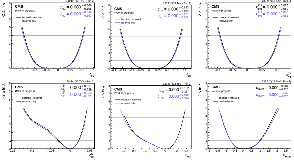
Figure 8.9: The likelihood curves for the six dim-6 SMEFT operators considered in this work. The violet line corresponds to the limits extracted from the resolved analysis only and the black line shows the combined analysis results. The SMEFT parametrisation includes both linear and quadratic terms. The fits are performed by considering EFT effects for a single operator.
