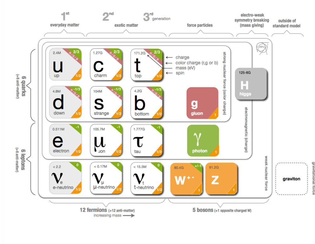
Figure 2.1: The SM particle content.
