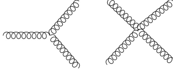
Figure 2.2: Gluon self interaction diagrams.
