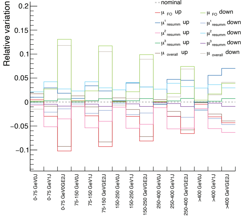
Figure 5.10: Scale variations in GENEVA NNLL'+NNLO simulation
