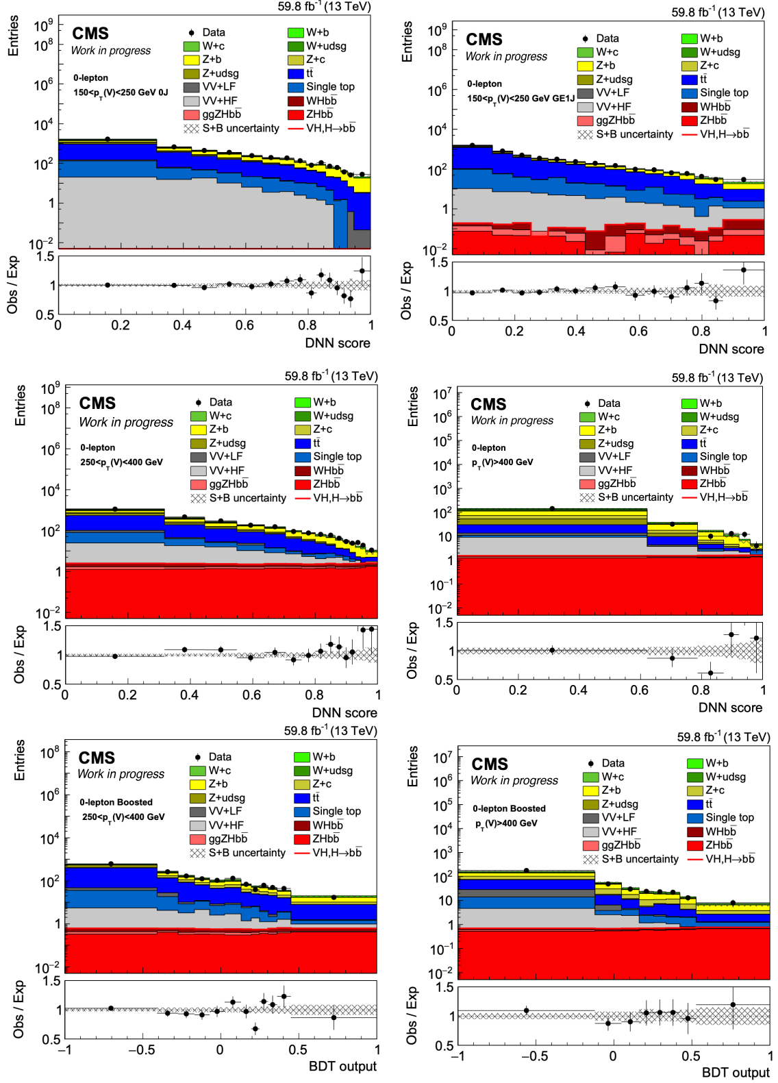
Figure 7.7: Signal regions post-fit distributions for 0-lepton channel signal regions in the 2018 analysis.
