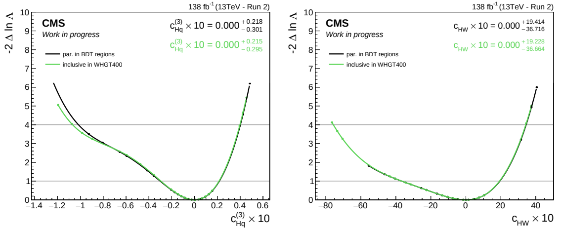
Figure 8.16: Likelihood-scans shapes obtained with the parametrisation derived inclusively for p_T^V > 400 GeV bin and with additional separation based on BDT output region.
