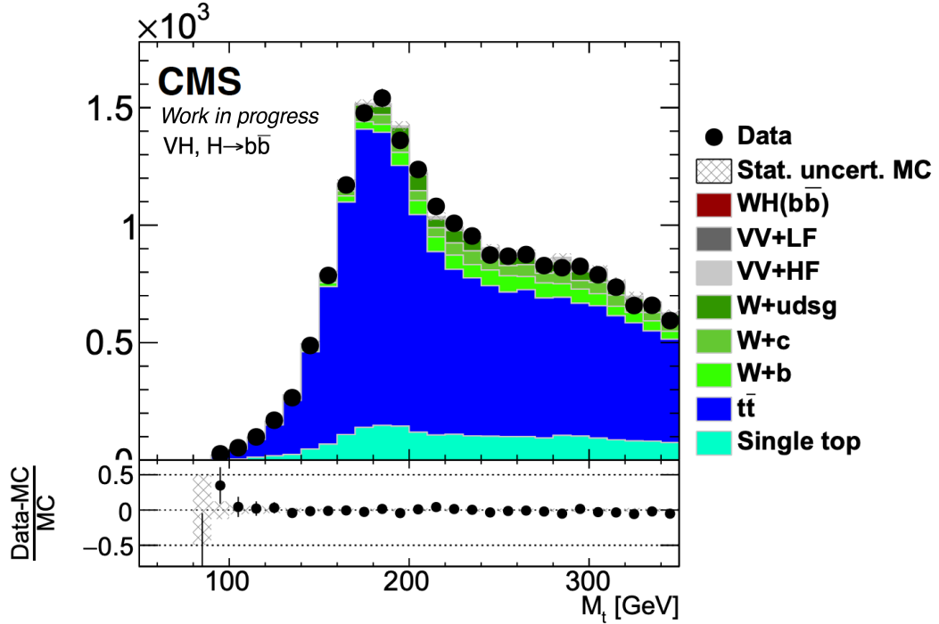
Figure 4.8: Top-quark mass distribution reconstructed in 1-lepton signal region
