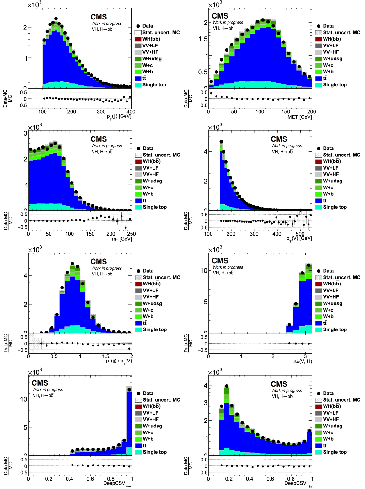
Figure 4.11: 1-lepton signal region pre-fit distribution of MVA input variables
