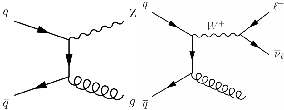
Figure 4.3: V +jets production processes diagrams
