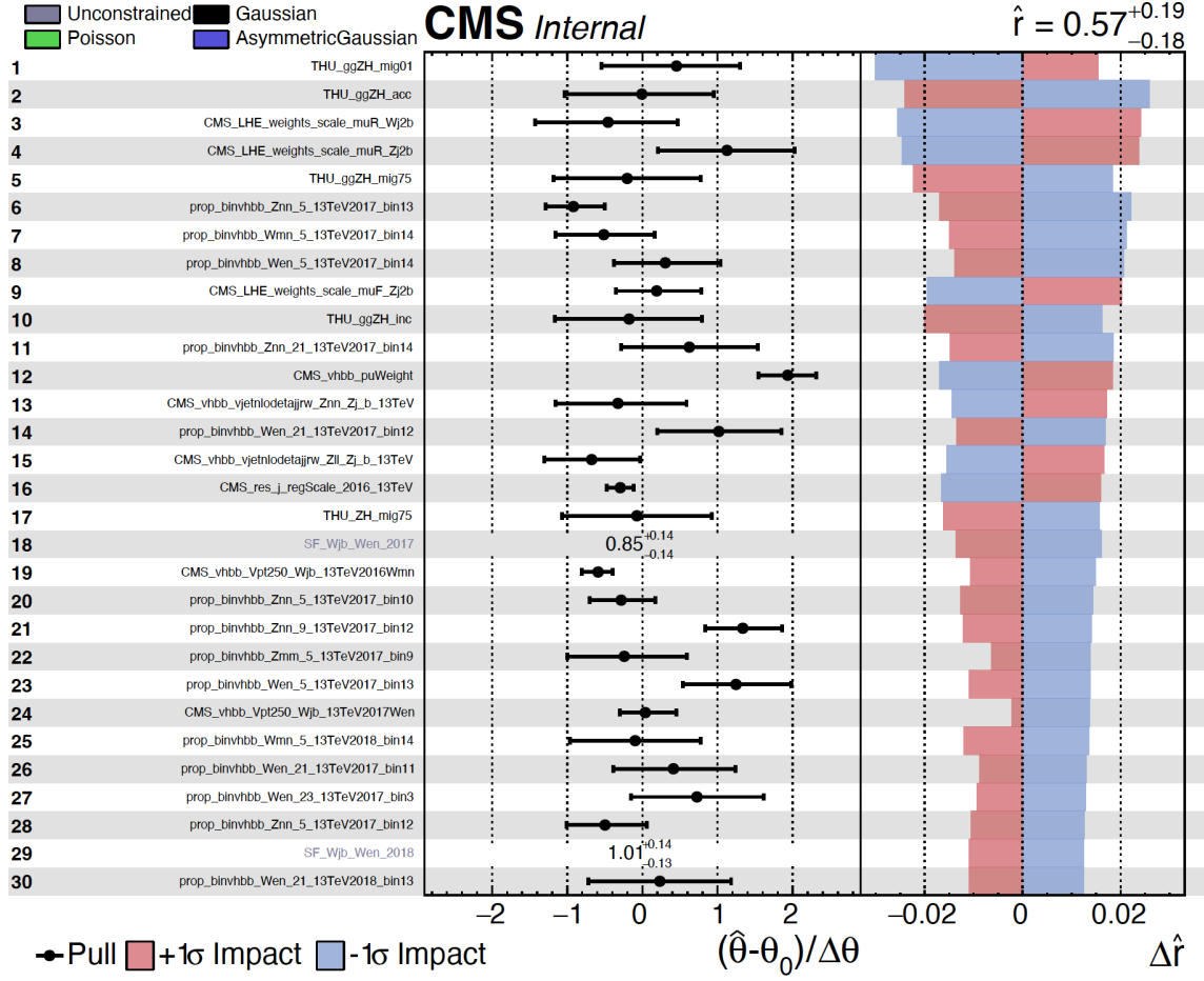
Figure 7.2: Pulls and constraints for the most impactful nuisances in the full Run 2 inclusive fit.
