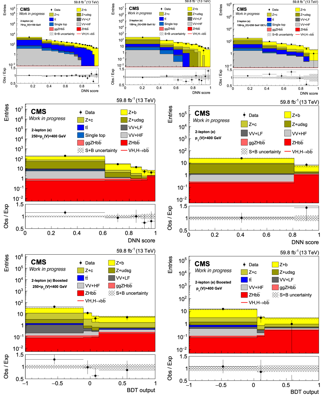
Figure 7.9: Signal regions post-fit distributions for 2-lepton channel signal regions in the 2018 analysis.
