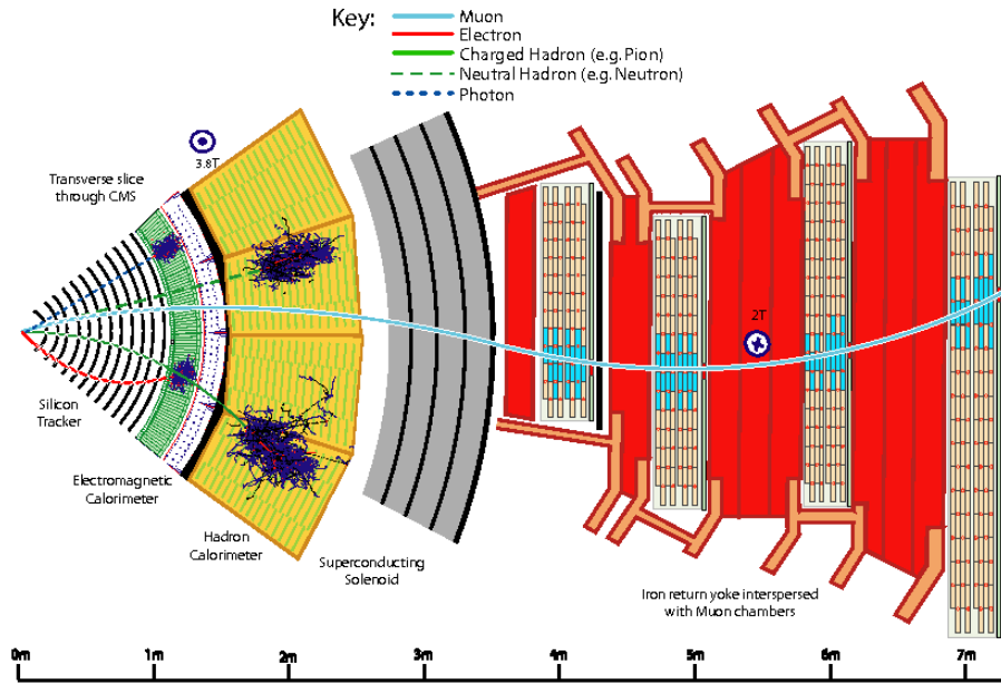
Figure 3.8: The CMS particle flow
