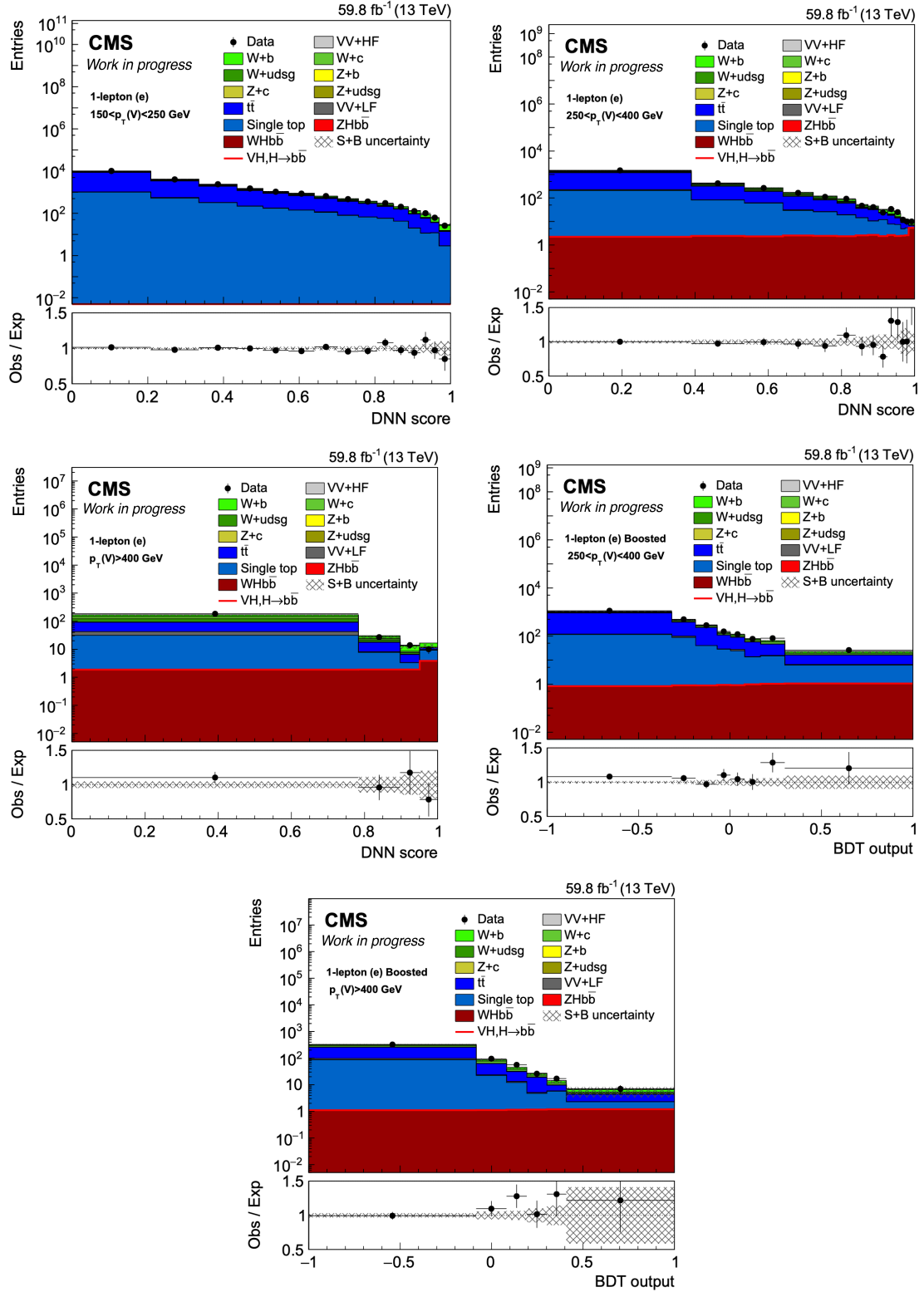
Figure 7.8: Signal regions post-fit distributions for 1-lepton channel signal regions in the 2018 analysis.
