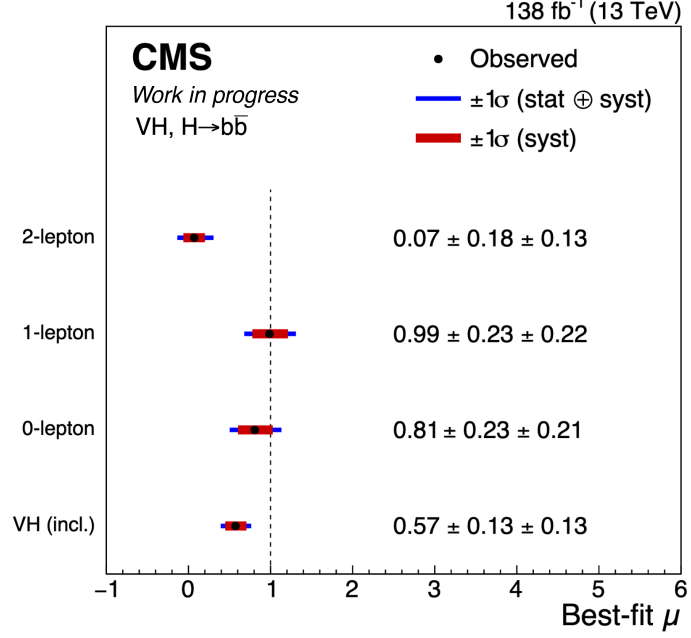
Figure 7.3: Observed signal strengths for the 0-lepton, 1-lepton and 2-lepton channels, as well as the combined signal strength.
