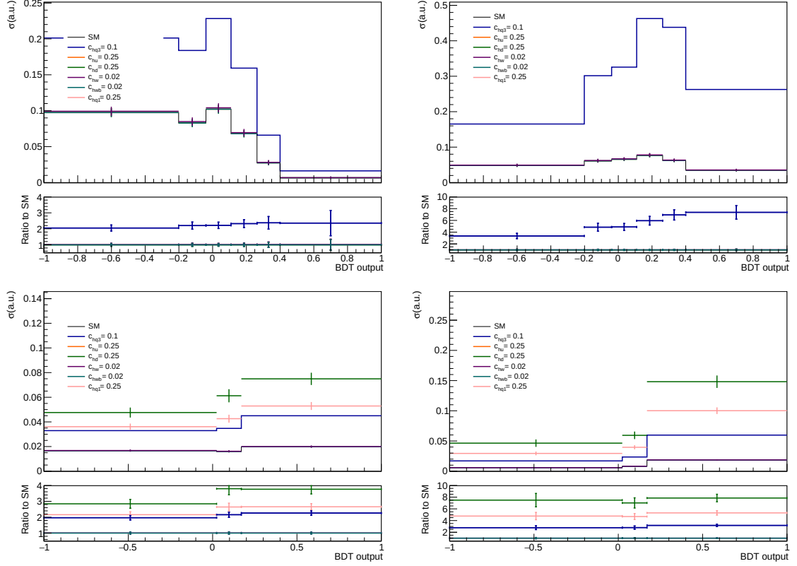
Figure 8.12: BDT output distribution for boosted category under EFT variations for WH (upper row) and ZH (lower row), in 250 < p_T^V < 400 (left) and p_T^V > 400 GeV (right) GeV STXS bins.
