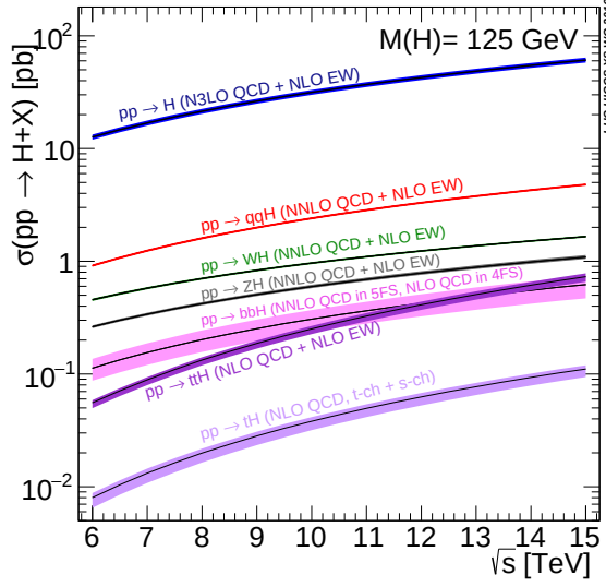
Figure 2.7: SM Higgs boson production predictions [15]
