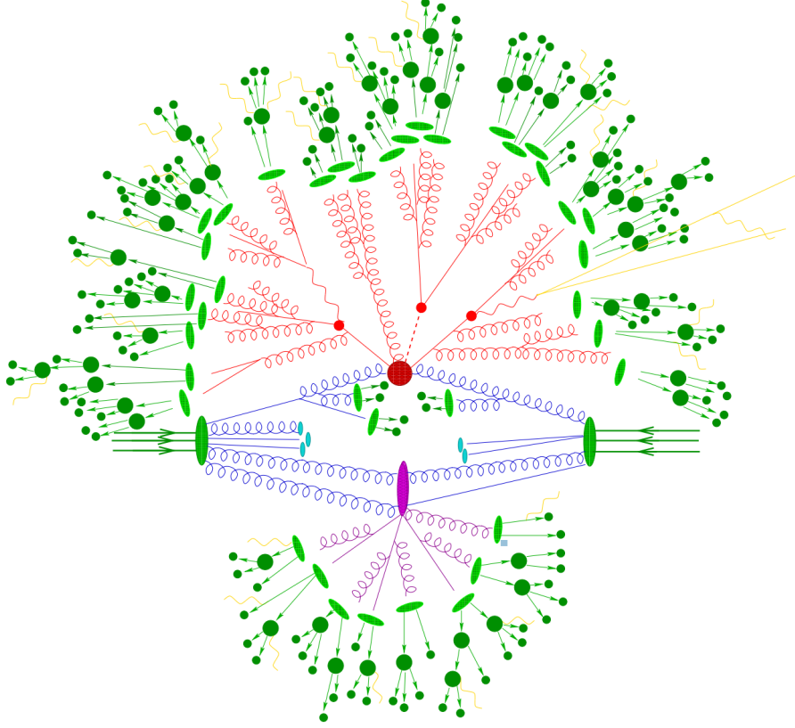
Figure 3.10: The proton-proton collision visualisation including the hard interaction, the parton shower and the hadronization processes [51].
