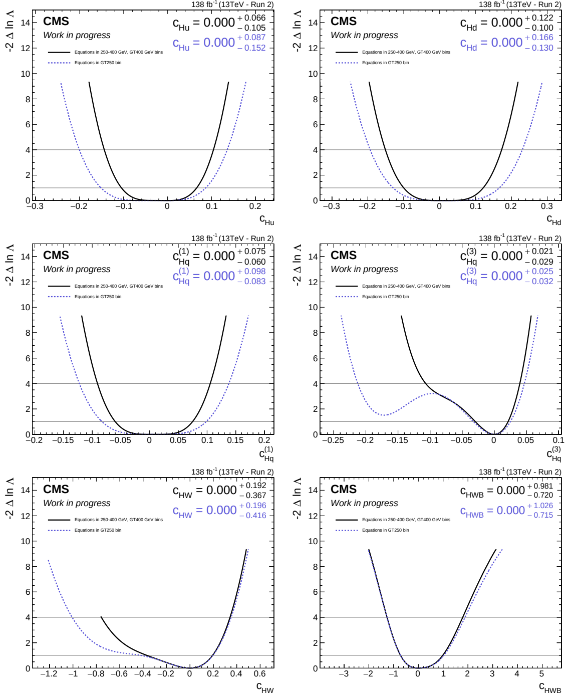
Figure 8.13: The likelihood curves for the full set of operators with the parametrisation derived for the default STXS 1.2 scheme in violet and the modified scheme in black.
