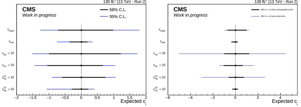
Figure 8.5: Expected 68% and 95% CL intervals obtained with linear-plus-quadratic parametrisation are shown in the left plot. The comparison of 68% CL derived with the full parametrisation and linear only is shown in the right plot.
