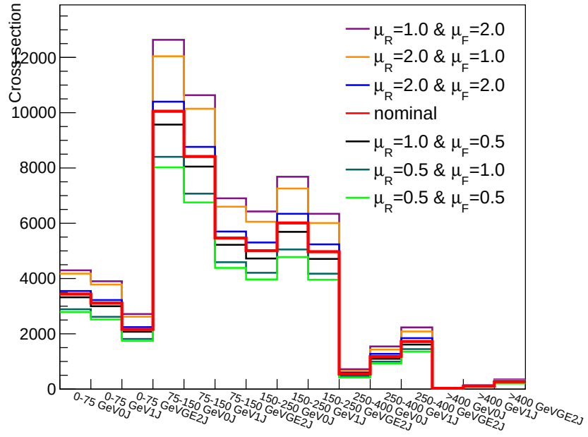
Figure 5.5: Scale variations for ggZH process.
