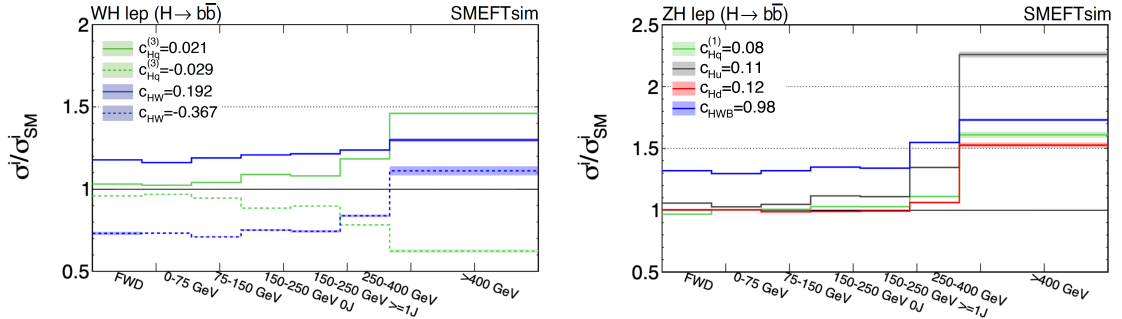
Figure 8.6: The modified STXS stage 1.2 for WH (left) and ZH (right) processes with the SMEFT parameters set at upper 68% CL boundaries.
