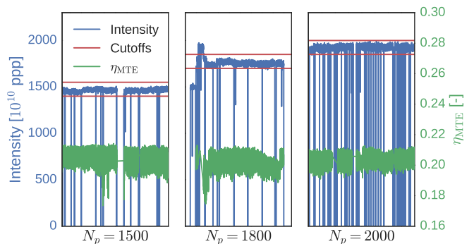
FIG. 3: PS intensity over time, shown together with the cuts in intensity, and \eta_{\text{MTE}} .
